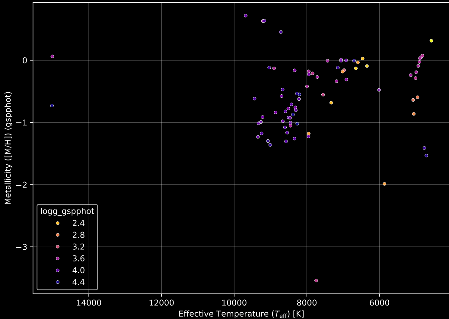
Gaia Cluster: [Kronberger_81] Stellar Population Parameters (n= 79)
