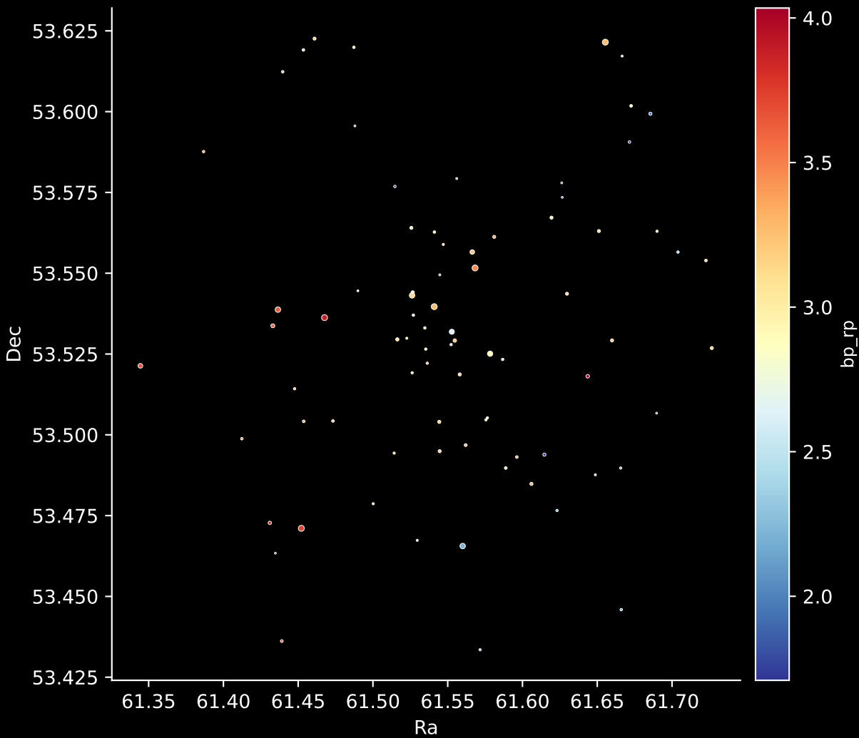
Gaia Cluster: [Kronberger_81] Stars: 79
