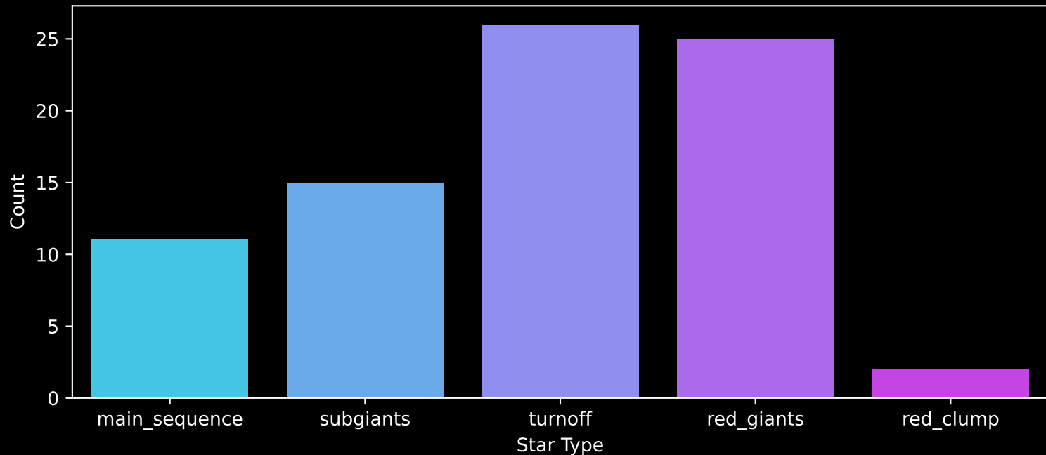
Gaia Cluster: [Kronberger_81] Count plot of Star Type
