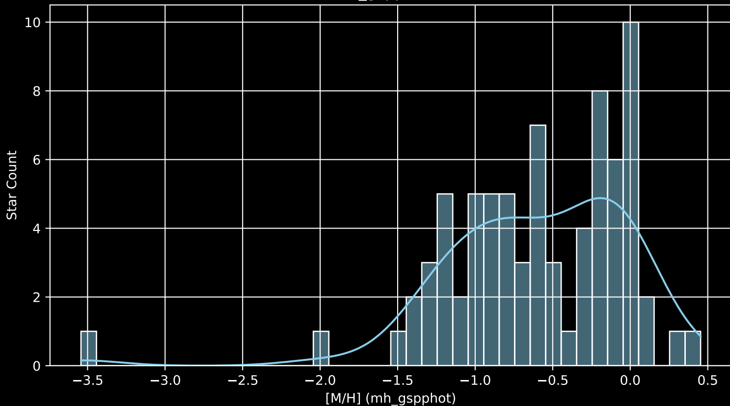
Gaia Cluster: [Kronberger_81 [M/H] (mh_gspphot) (n= 76)
