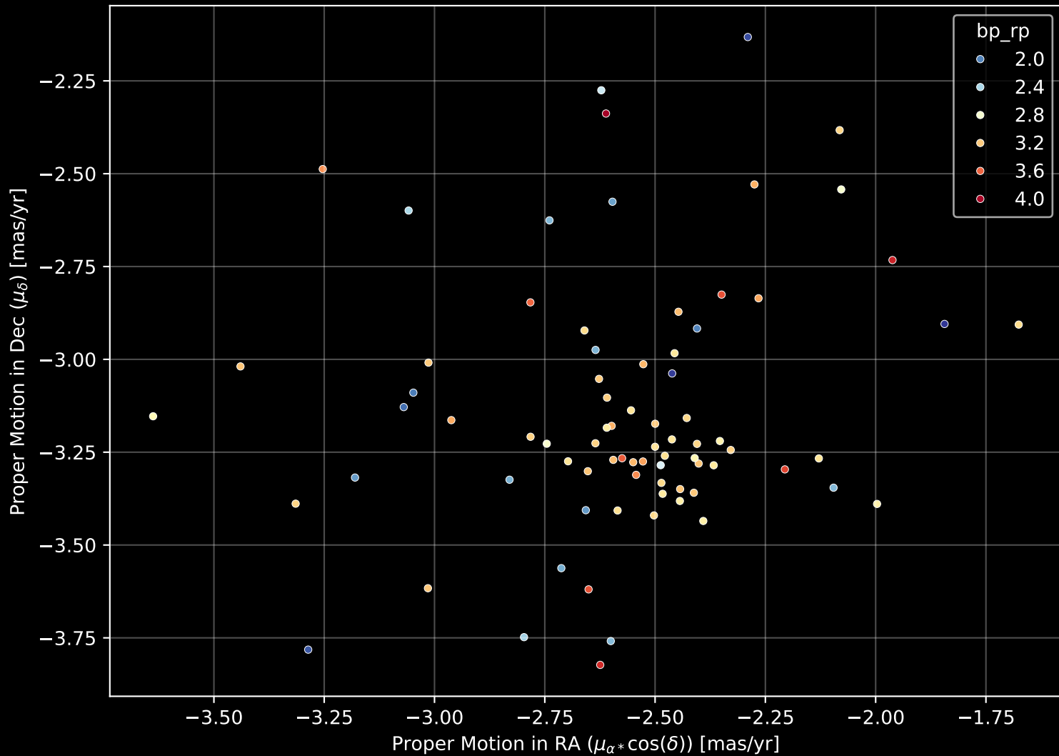
Gaia Cluster: [Kronberger_81] Proper Motion Diagram (n= 79)
