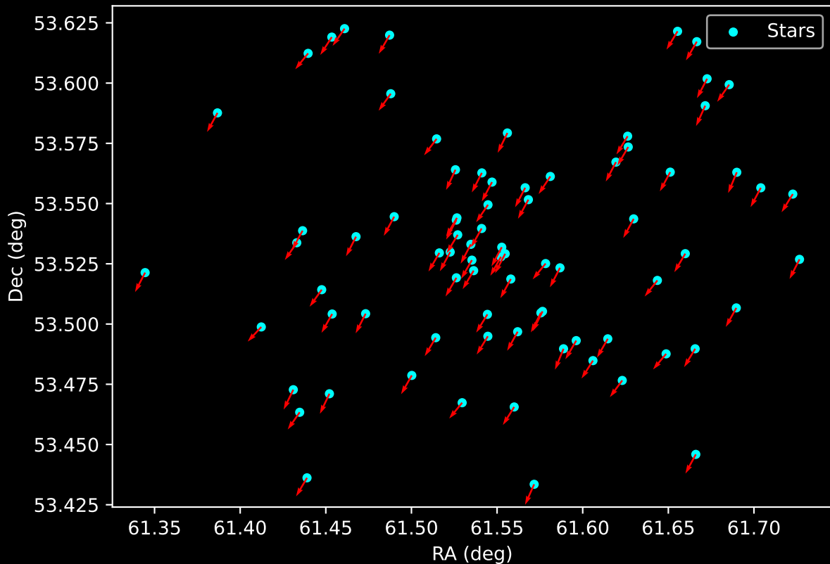
Gaia Cluster: [Kronberger_81] Proper Motion Vectors for Gaia Star Field (n= 79)
