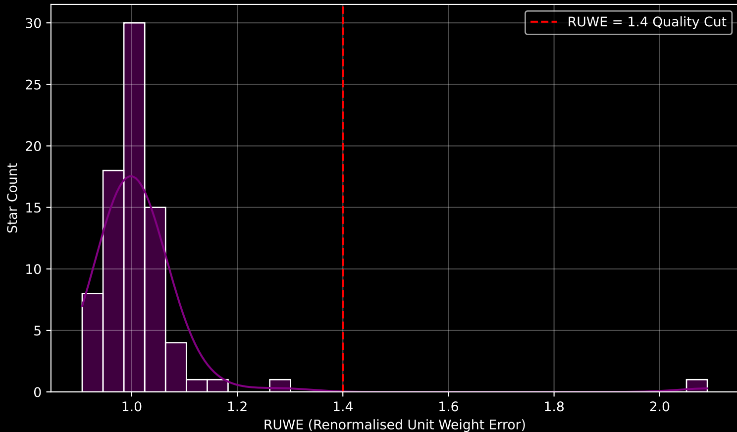
Gaia Cluster: [Kronberger_81] RUWE Distribution (n= 79)
