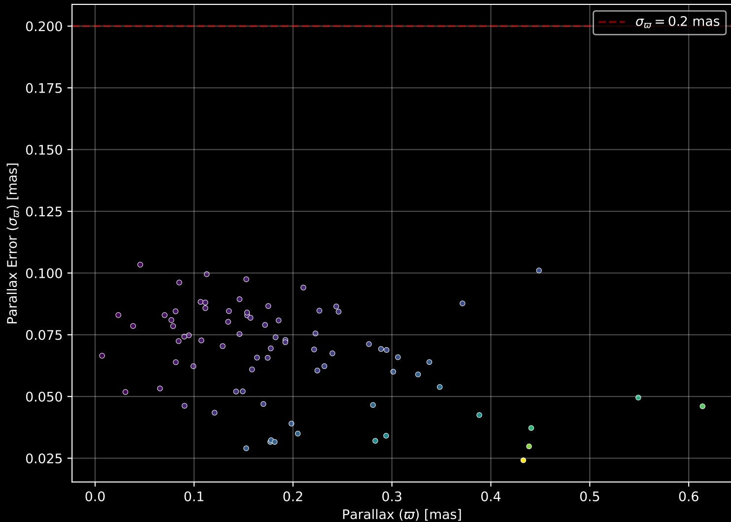
Gaia Cluster: [Kronberger_81] Parallax Quality (n= 79)
