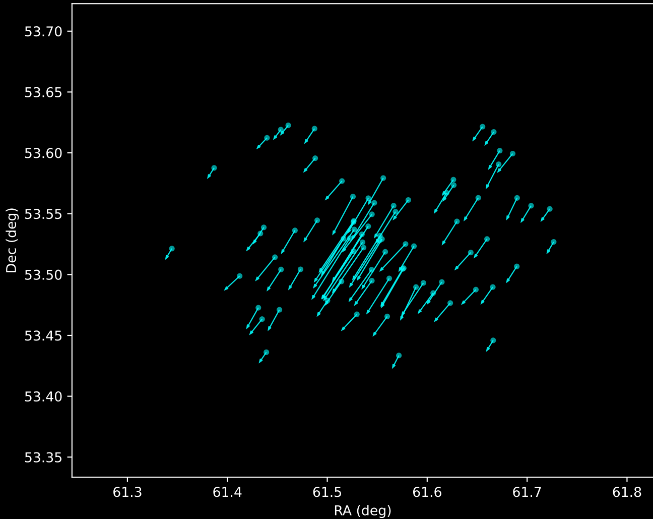
Gaia DR3 Noise Stream Proper Motion Vectors (n=79)
