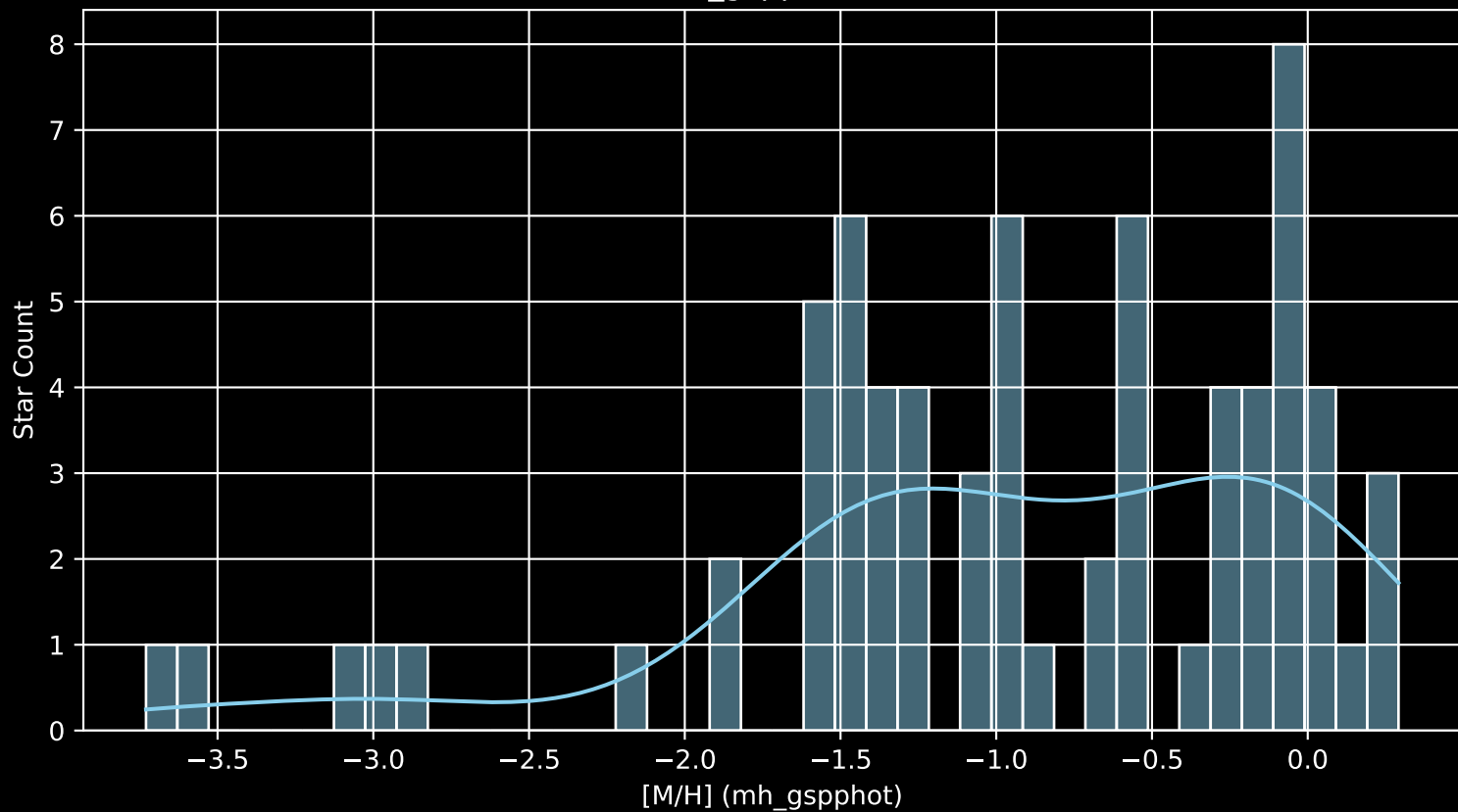
Gaia Cluster: [Kronberger_84 [M/H] (mh_gspphot) (n= 70)
