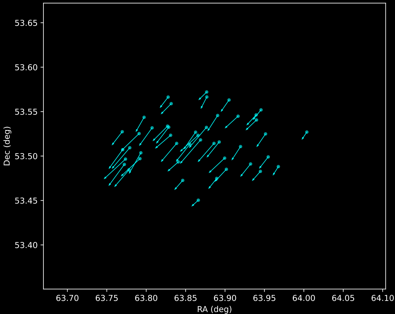
Gaia DR3 Noise Stream Proper Motion Vectors (n=45)
