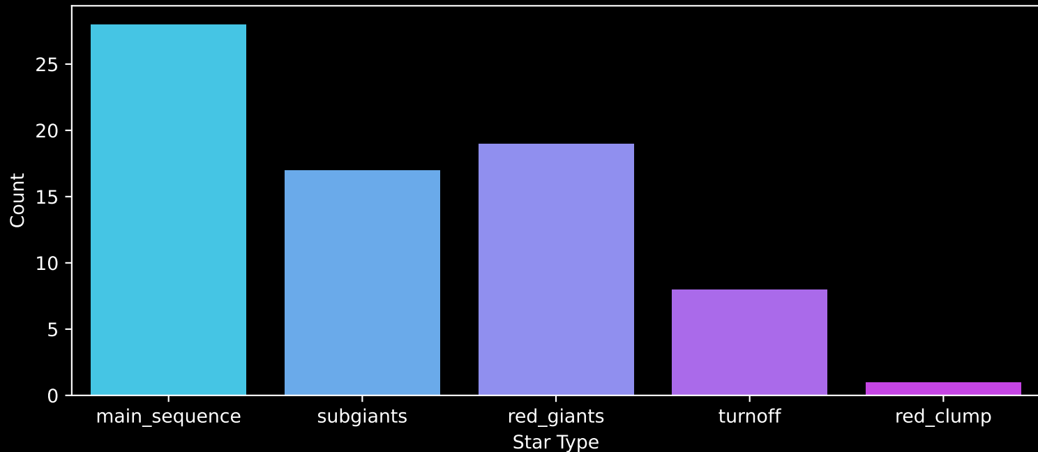
Gaia Cluster: [Kronberger_84] Count plot of Star Type
