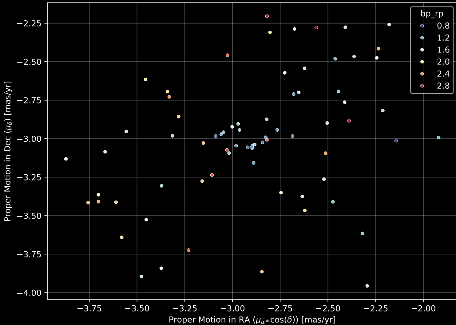
Gaia Cluster: [Kronberger_84] Proper Motion Diagram (n= 73)
