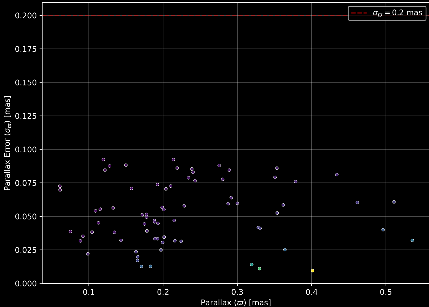
Gaia Cluster: [Kronberger_84] Parallax Quality (n= 73)
