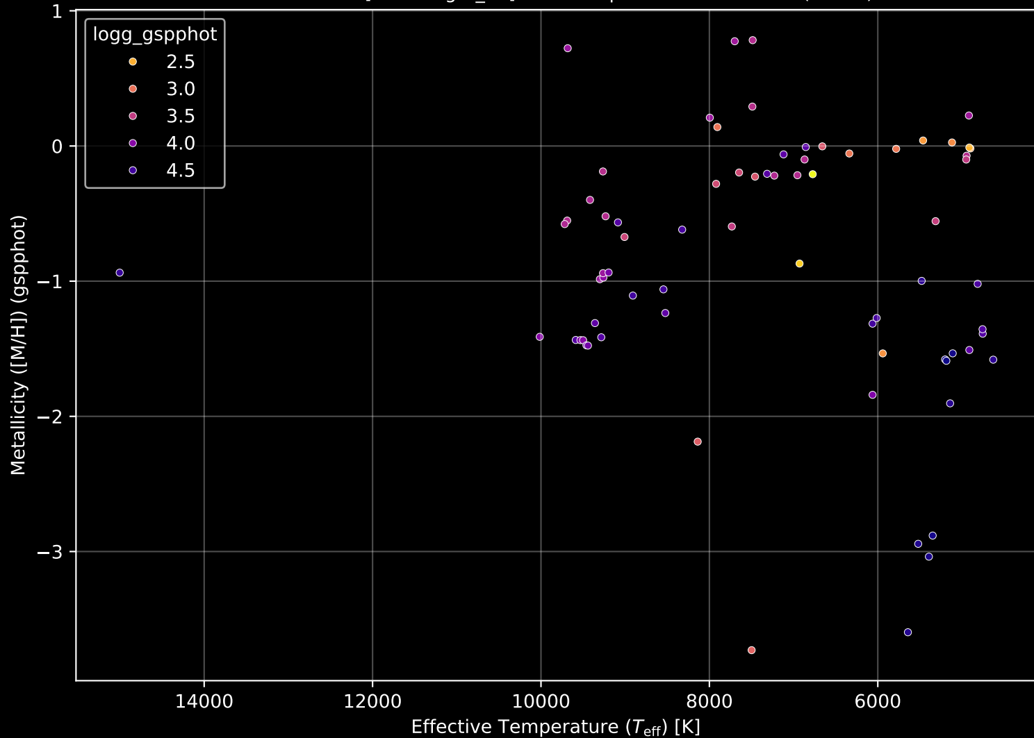
Gaia Cluster: [Kronberger_84] Stellar Population Parameters (n= 73)
