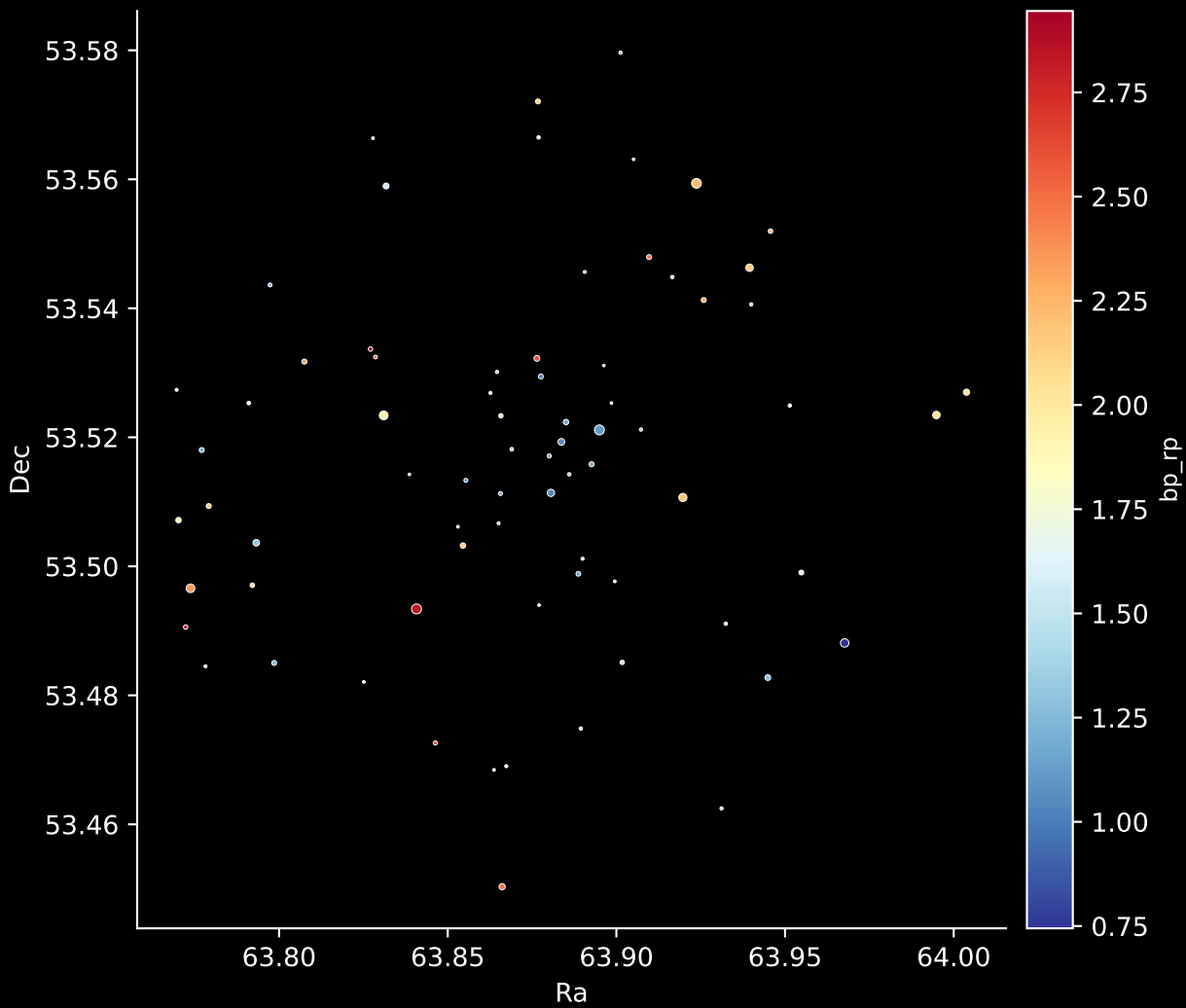
Gaia Cluster: [Kronberger_84] Stars: 73
