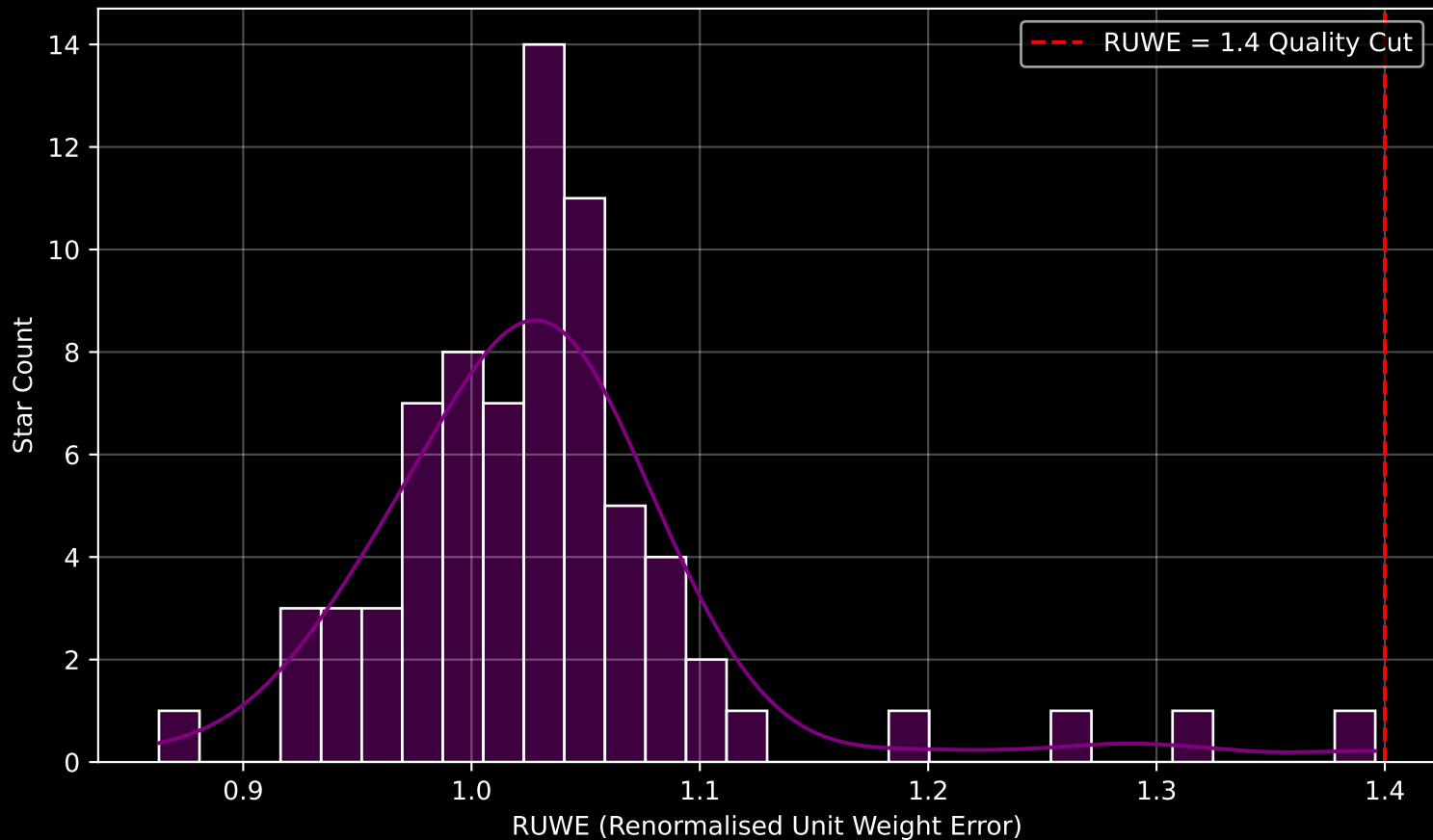
Gaia Cluster: [Kronberger_84] RUWE Distribution (n= 73)
