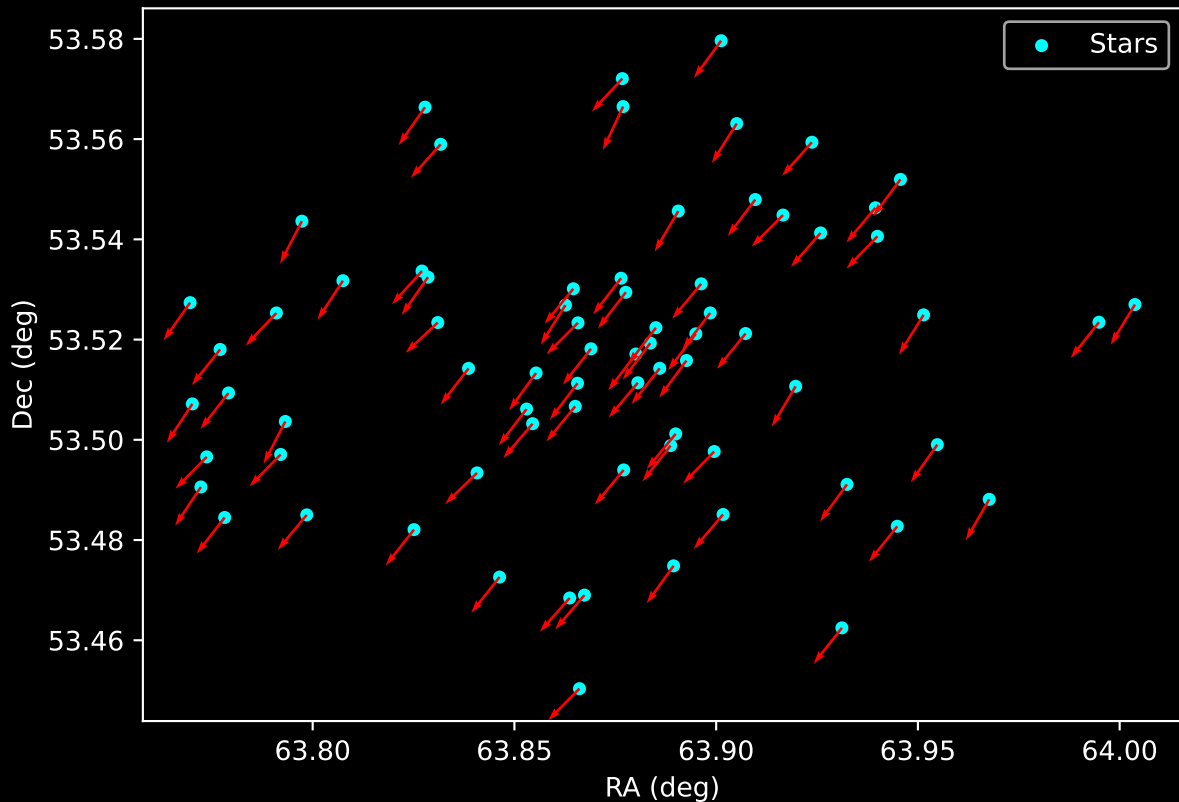
Gaia Cluster: [Kronberger_84] Proper Motion Vectors for Gaia Star Field (n= 73)
