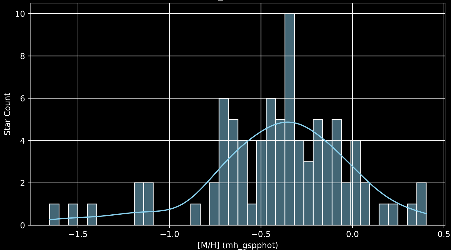
Gaia Cluster: [Loden_1194 [M/H] (mh_gspphot) (n= 85)
