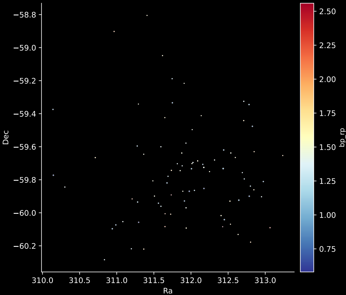
Gaia Cluster: [Loden_1194] Stars: 85
