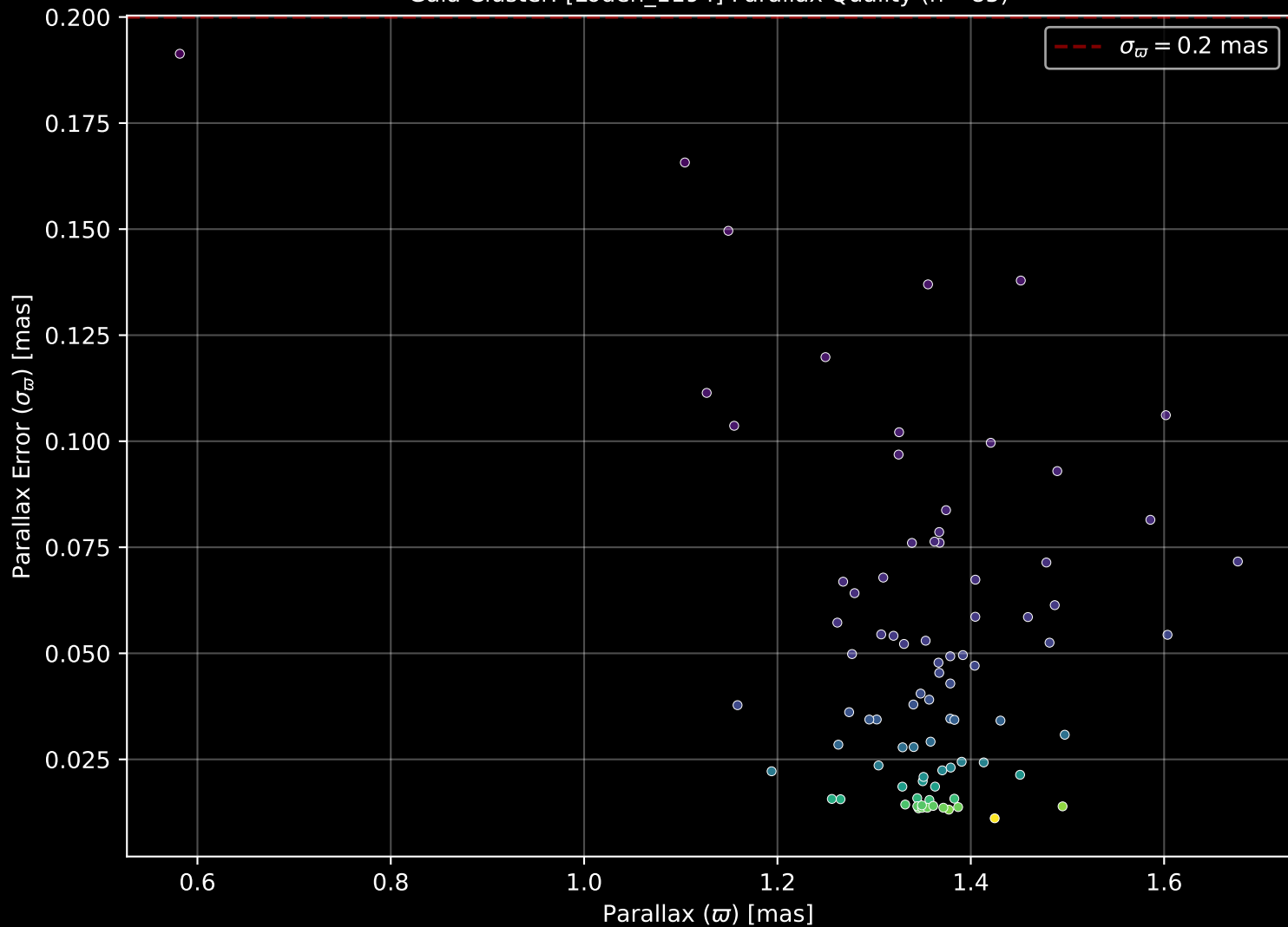
Gaia Cluster: [Loden_1194] Parallax Quality (n= 85)
