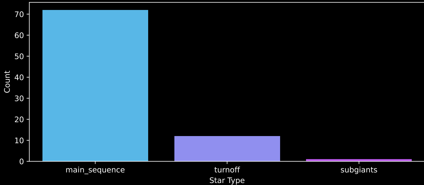
Gaia Cluster: [Loden_1194] Count plot of Star Type
