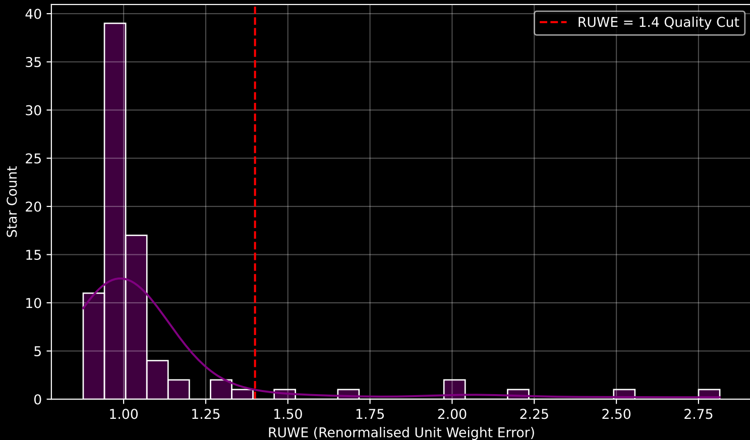
Gaia Cluster: [Loden_1194] RUWE Distribution (n= 83)
