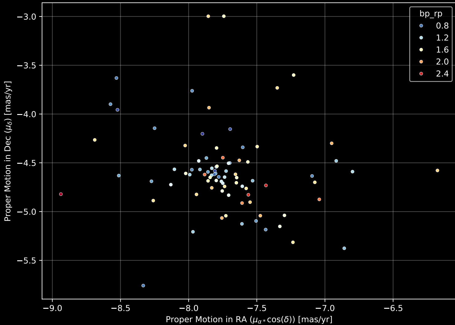
Gaia Cluster: [Loden_1194] Proper Motion Diagram (n= 85)
