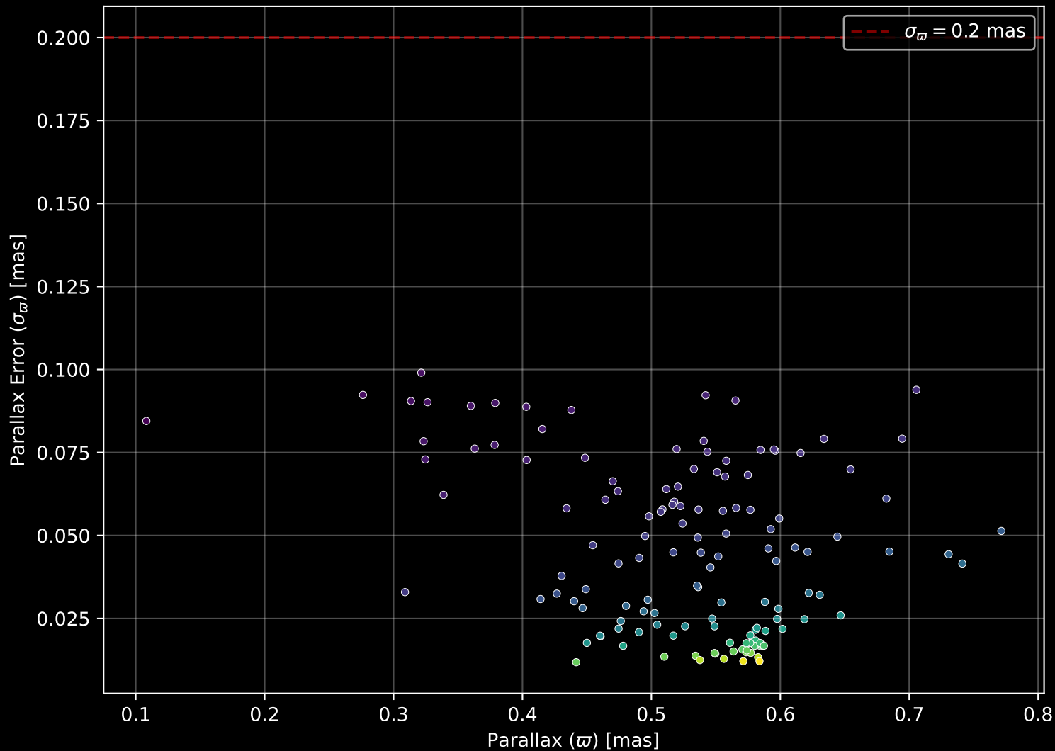
Gaia Cluster: [Loden_372] Parallax Quality (n= 137)
