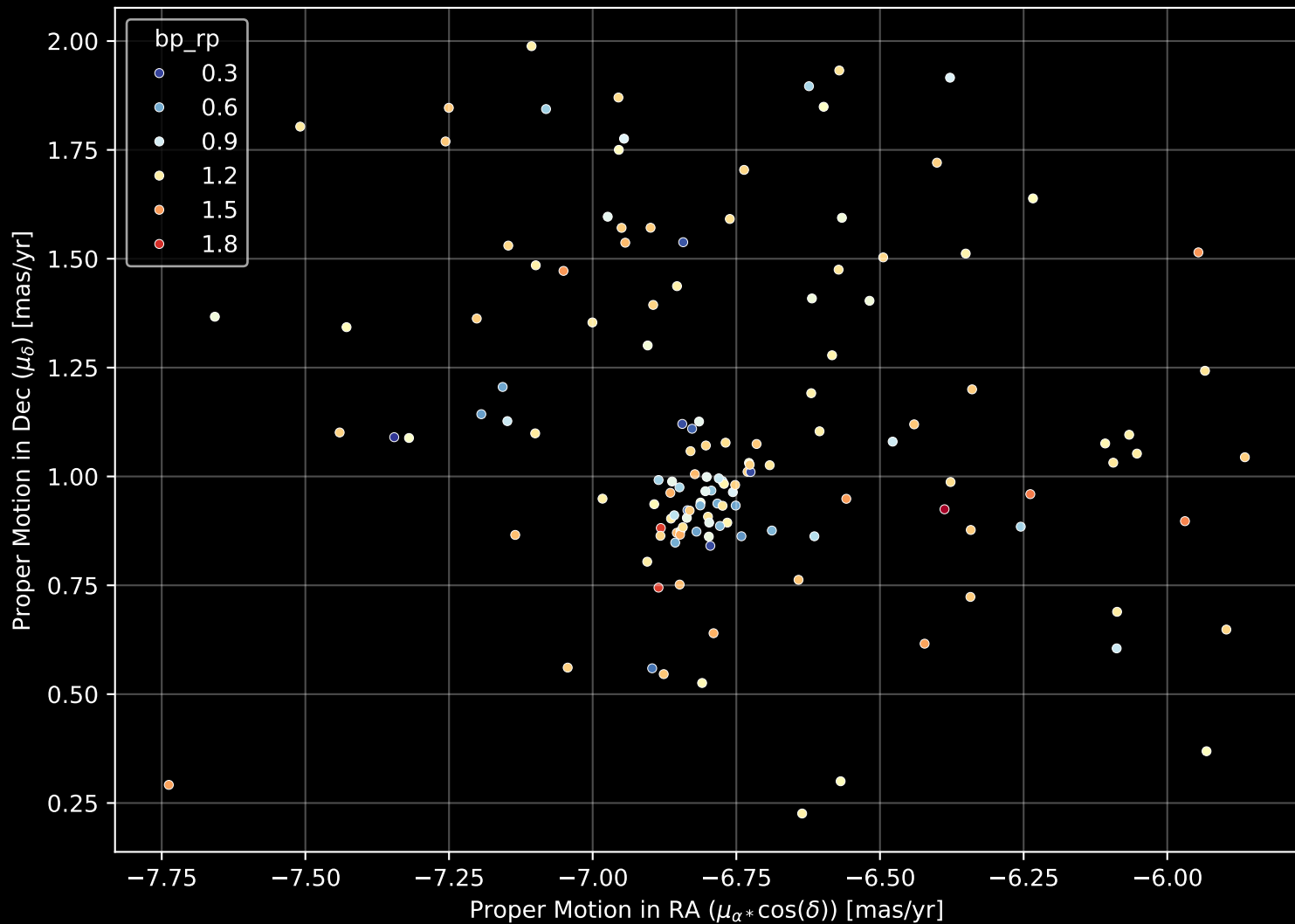
Gaia Cluster: [Loden_372] Proper Motion Diagram (n= 137)
