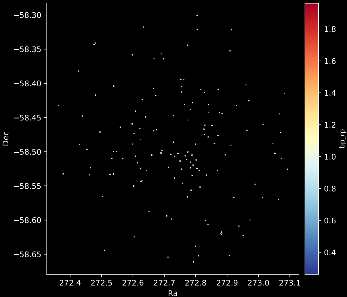
Gaia Cluster: [Loden_372] Stars: 137
