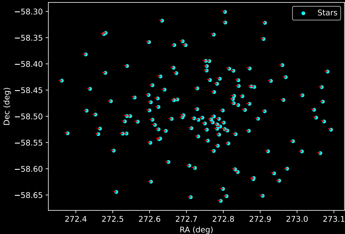
Gaia Cluster: [Loden_372] Proper Motion Vectors for Gaia Star Field (n= 137)
