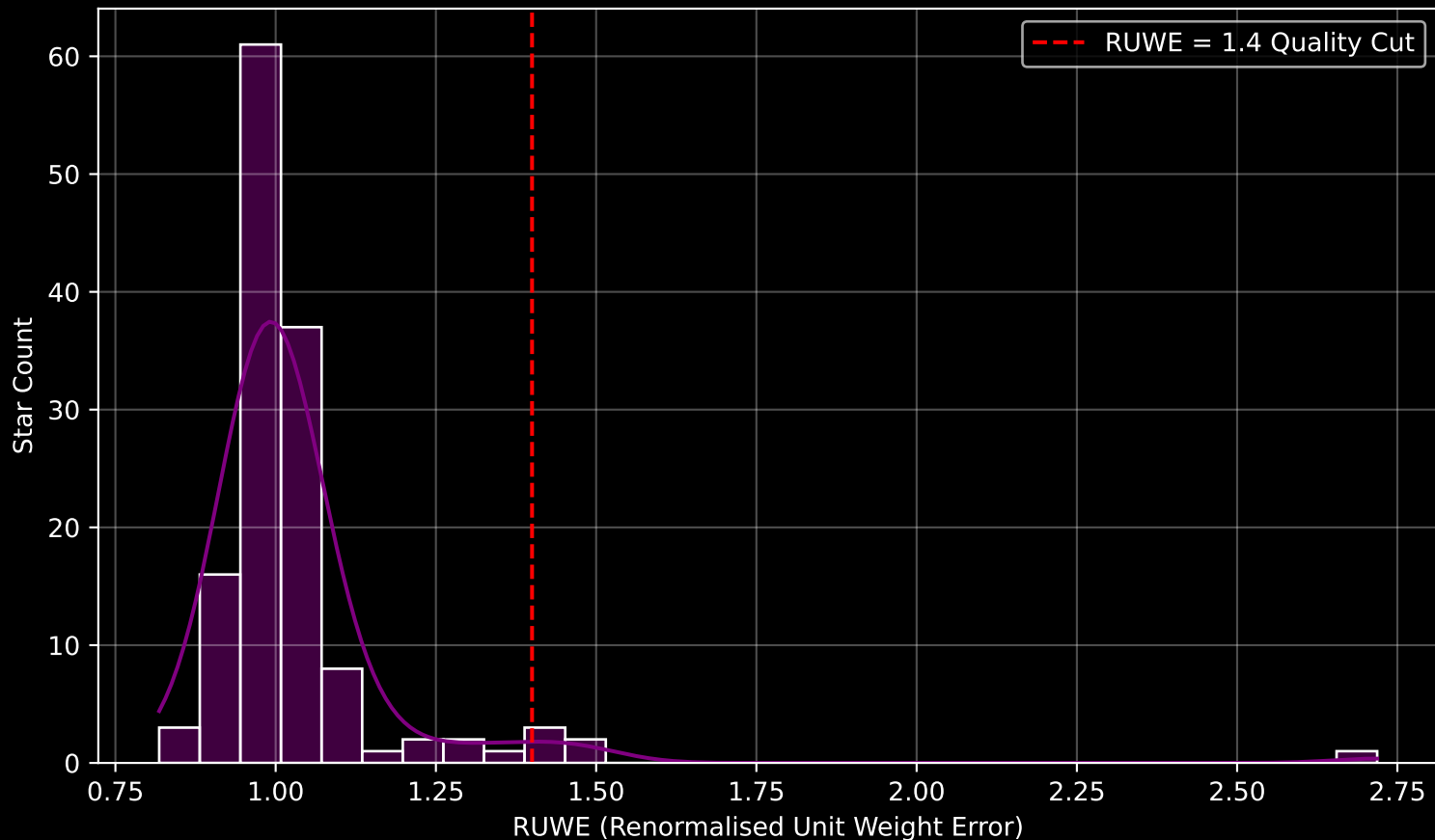
Gaia Cluster: [Loden_372] RUWE Distribution (n= 137)
