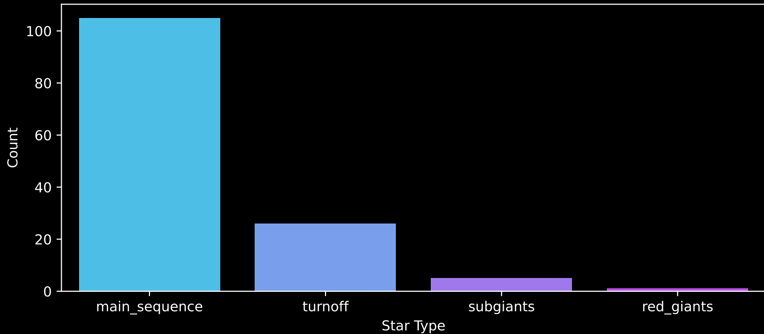
Gaia Cluster: [Loden_372] Count plot of Star Type
