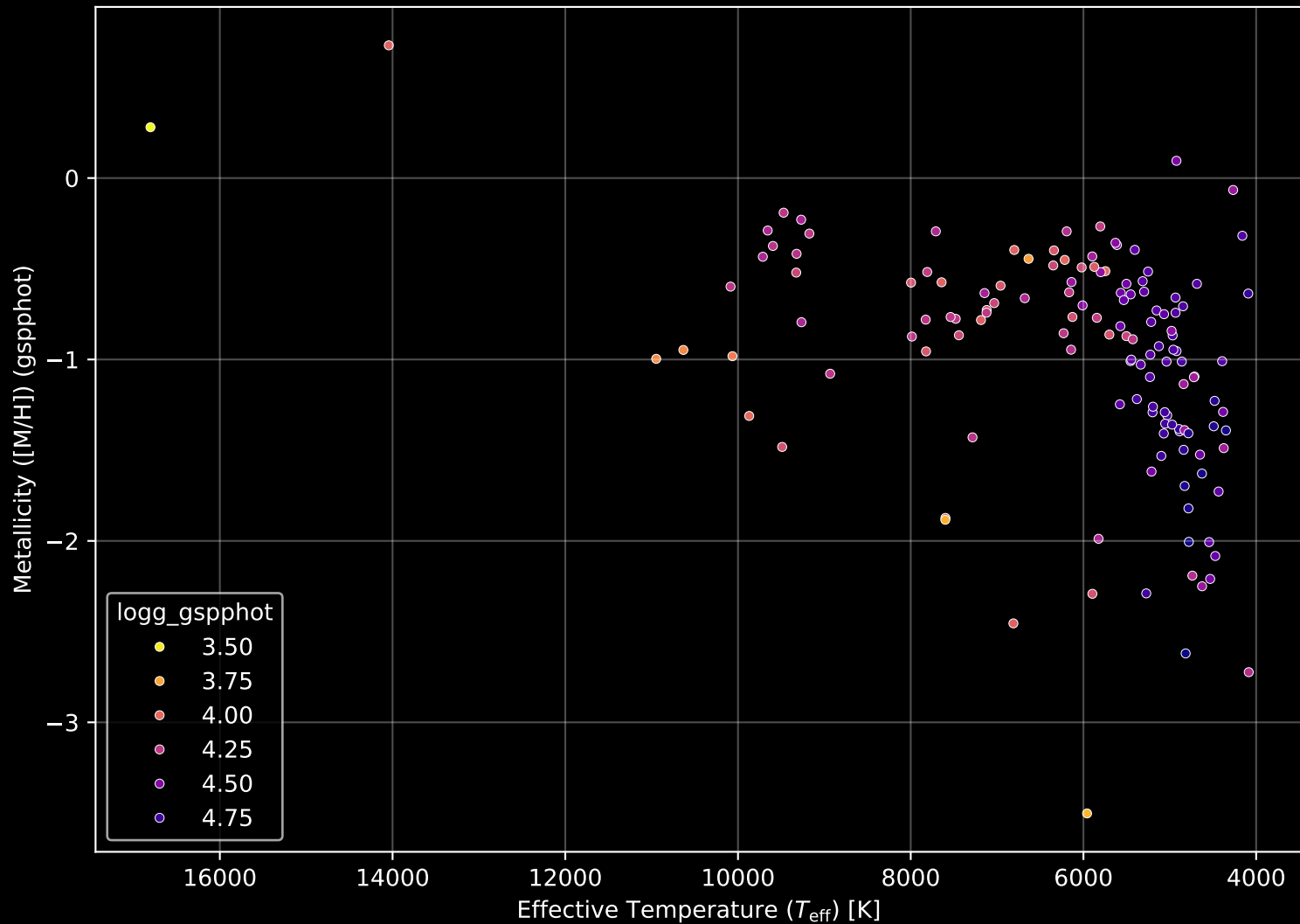
Gaia Cluster: [Loden_372] Stellar Population Parameters (n= 137)
