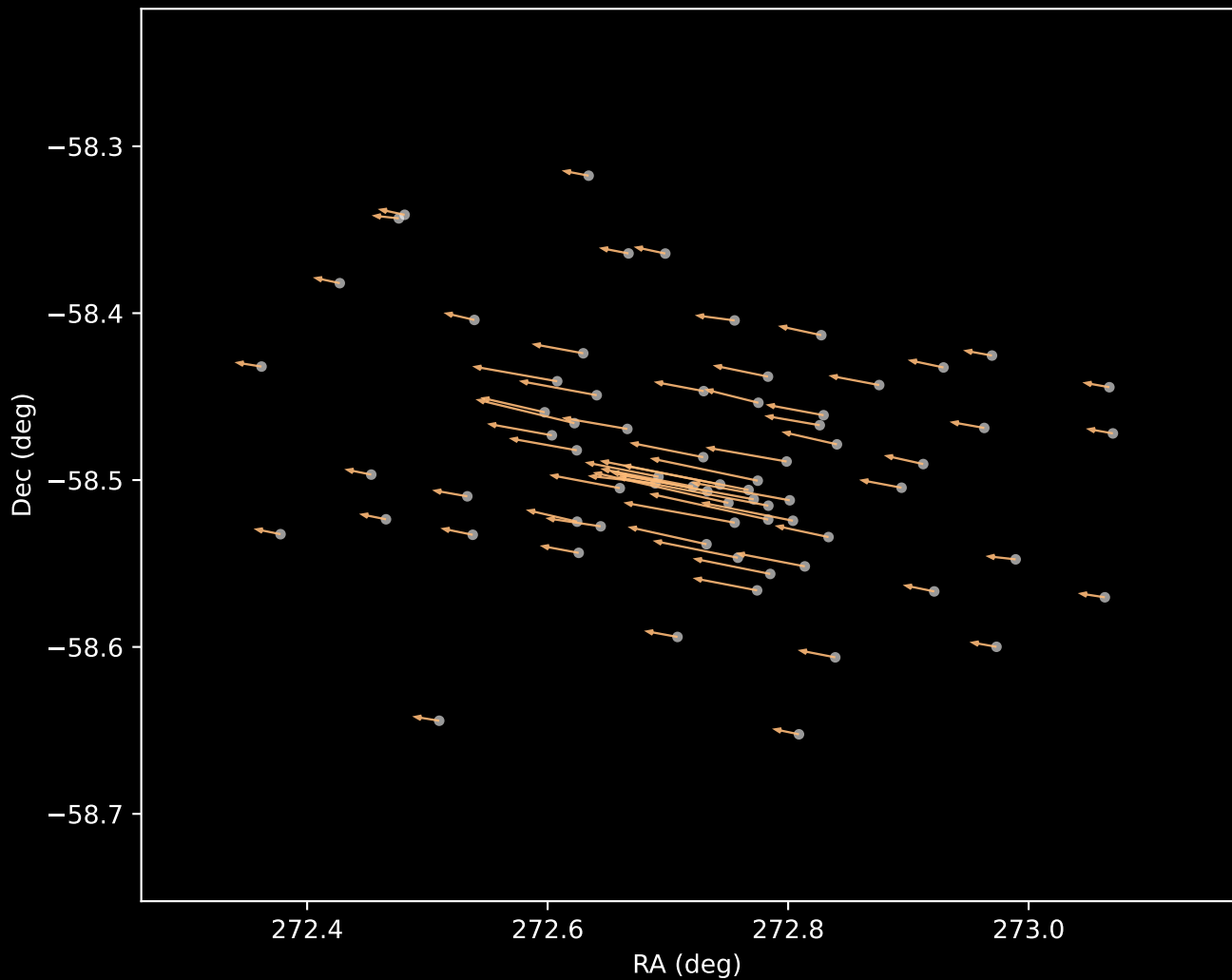
Gaia DR3 Cluster 3 Proper Motion Vectors (n=71)
