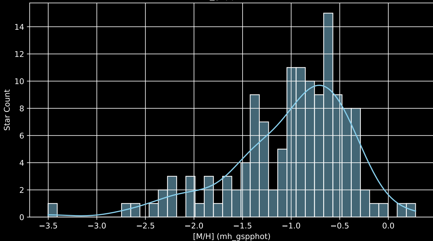
Gaia Cluster: [Loden_372 [M/H] (mh_gspphot) (n= 136)
