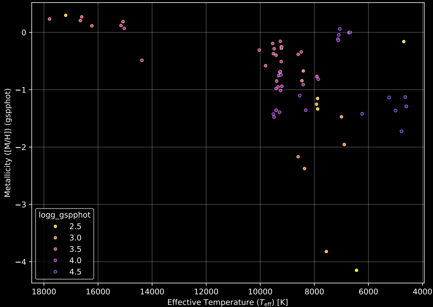
Gaia Cluster: [Lynga_14] Stellar Population Parameters (n= 64)
