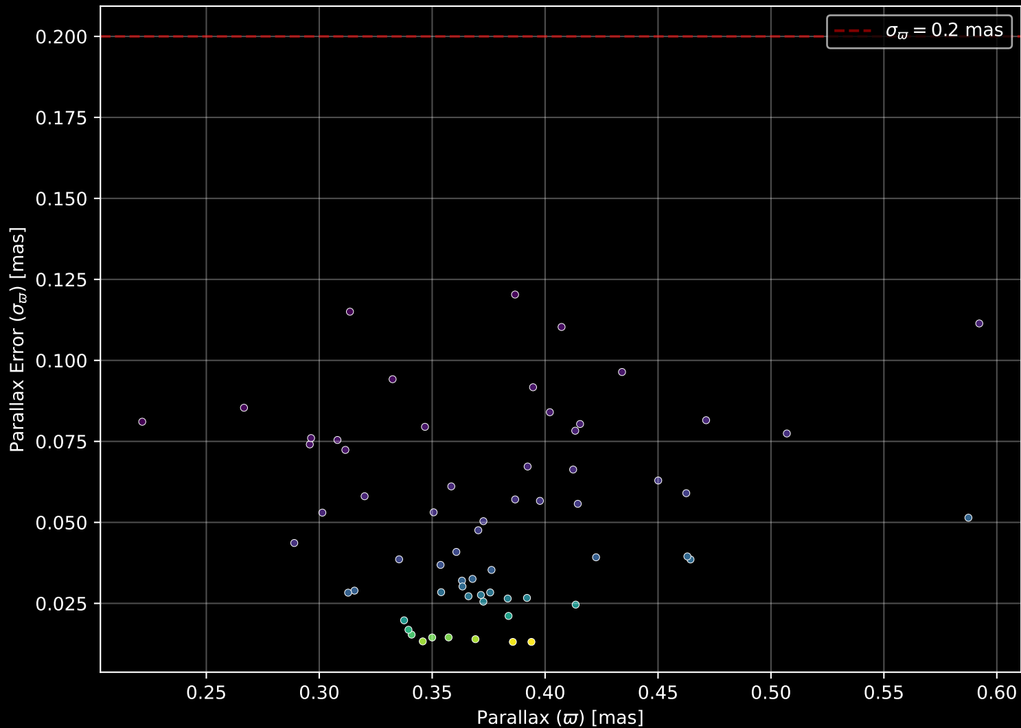
Gaia Cluster: [Lynga_14] Parallax Quality (n= 64)
