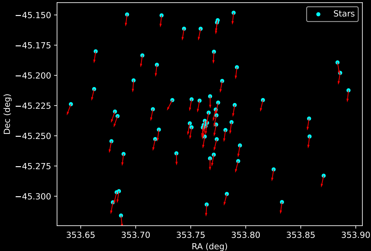
Gaia Cluster: [Lynga_14] Proper Motion Vectors for Gaia Star Field (n= 64)
