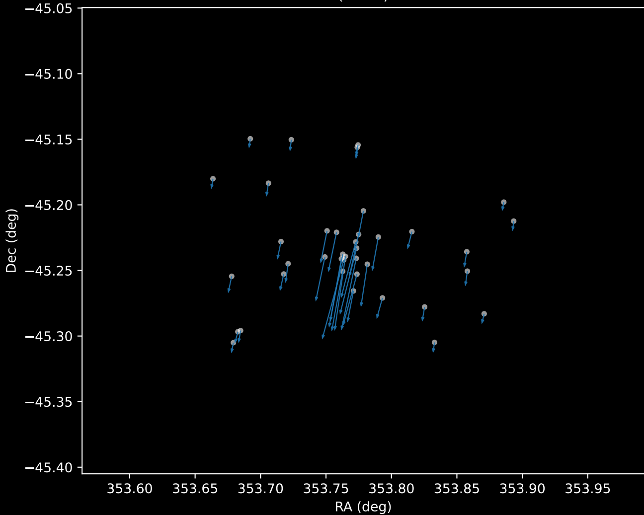
Gaia DR3 Cluster 0 Proper Motion Vectors (n=39)
