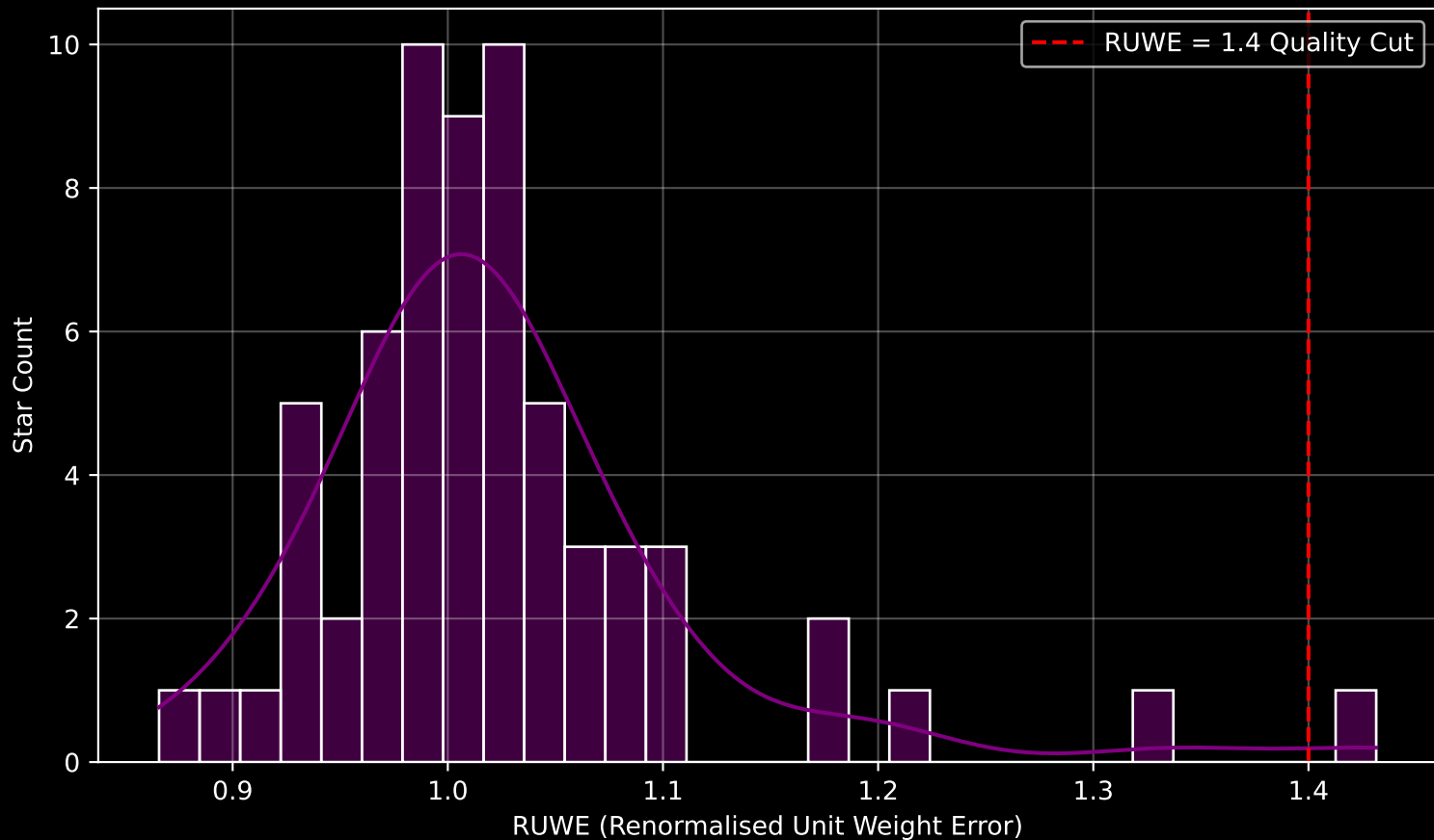
Gaia Cluster: [Lynga_14] RUWE Distribution (n= 64)
