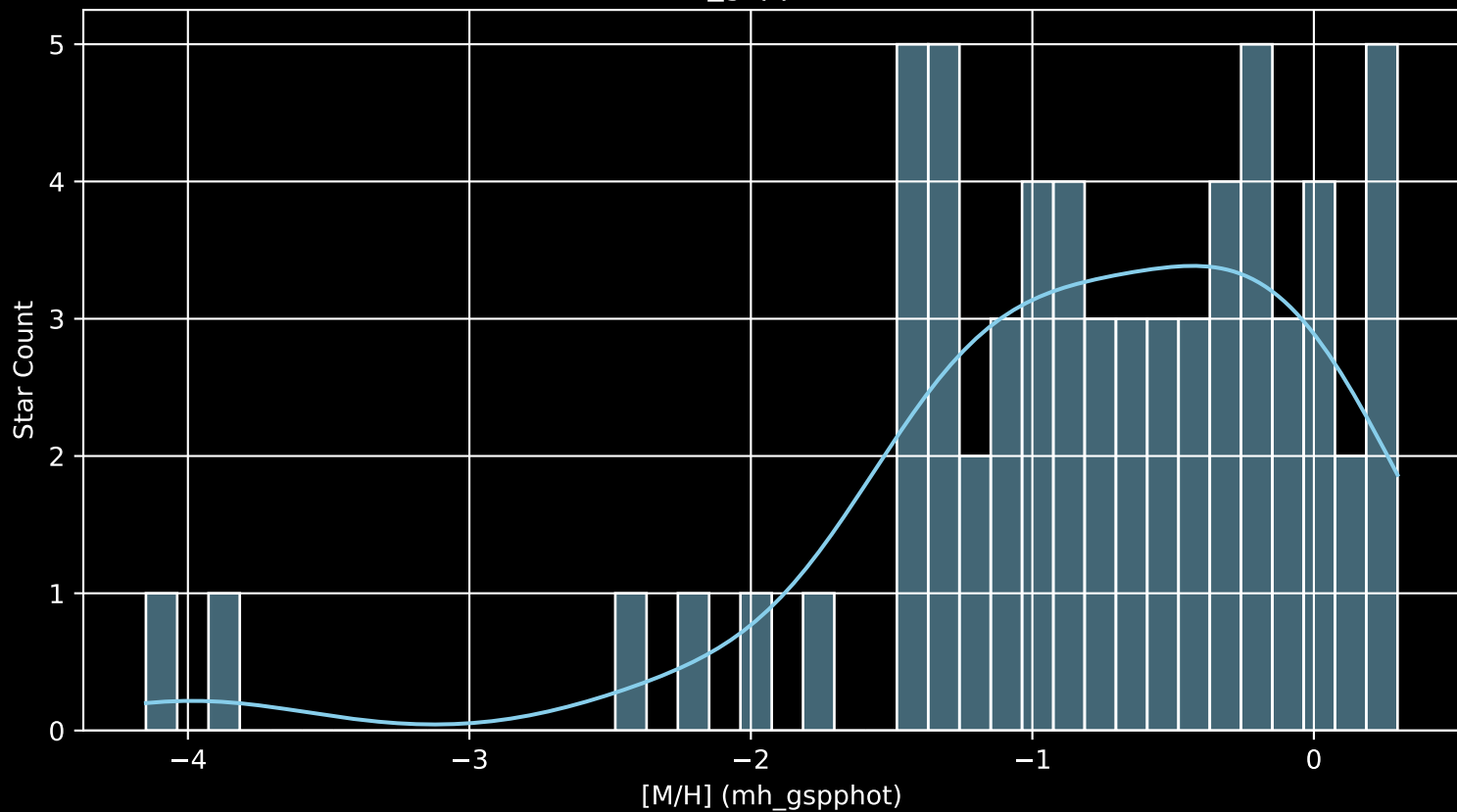
Gaia Cluster: [Lynga_14 [M/H] (mh_gspphot) (n= 64)
