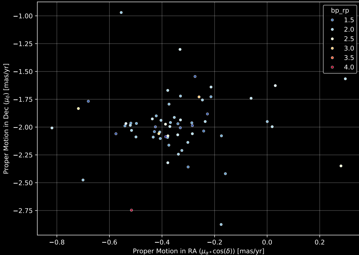
Gaia Cluster: [Lynga_14] Proper Motion Diagram (n= 64)
