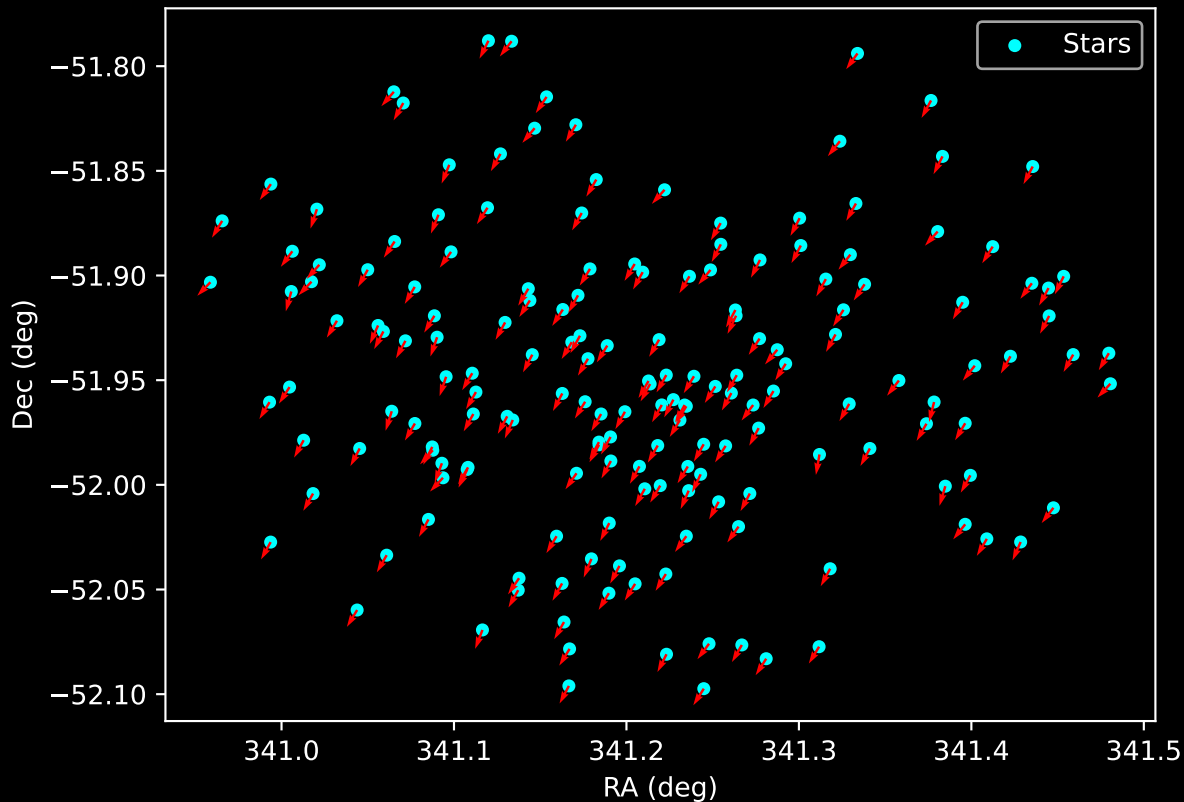
Gaia Cluster: [Lynga_6] Proper Motion Vectors for Gaia Star Field (n= 175)
