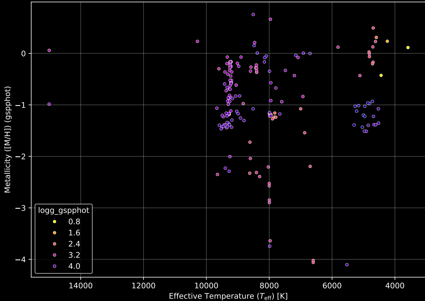
Gaia Cluster: [Lynga_6] Stellar Population Parameters (n= 175)
