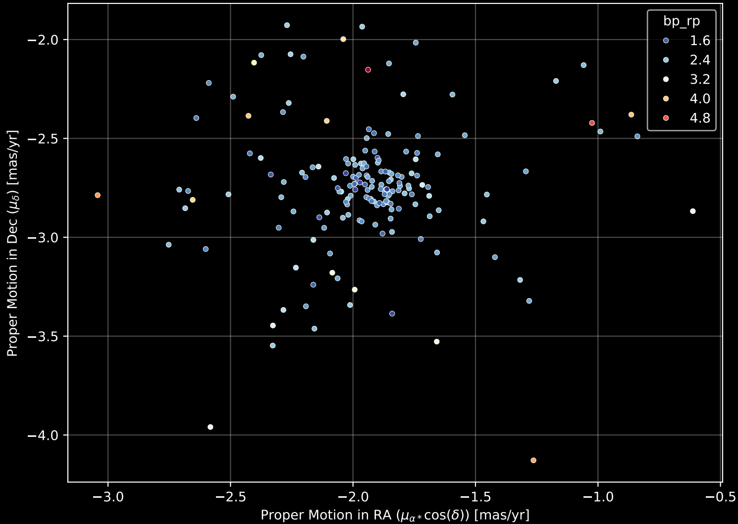
Gaia Cluster: [Lynga_6] Proper Motion Diagram (n= 175)
