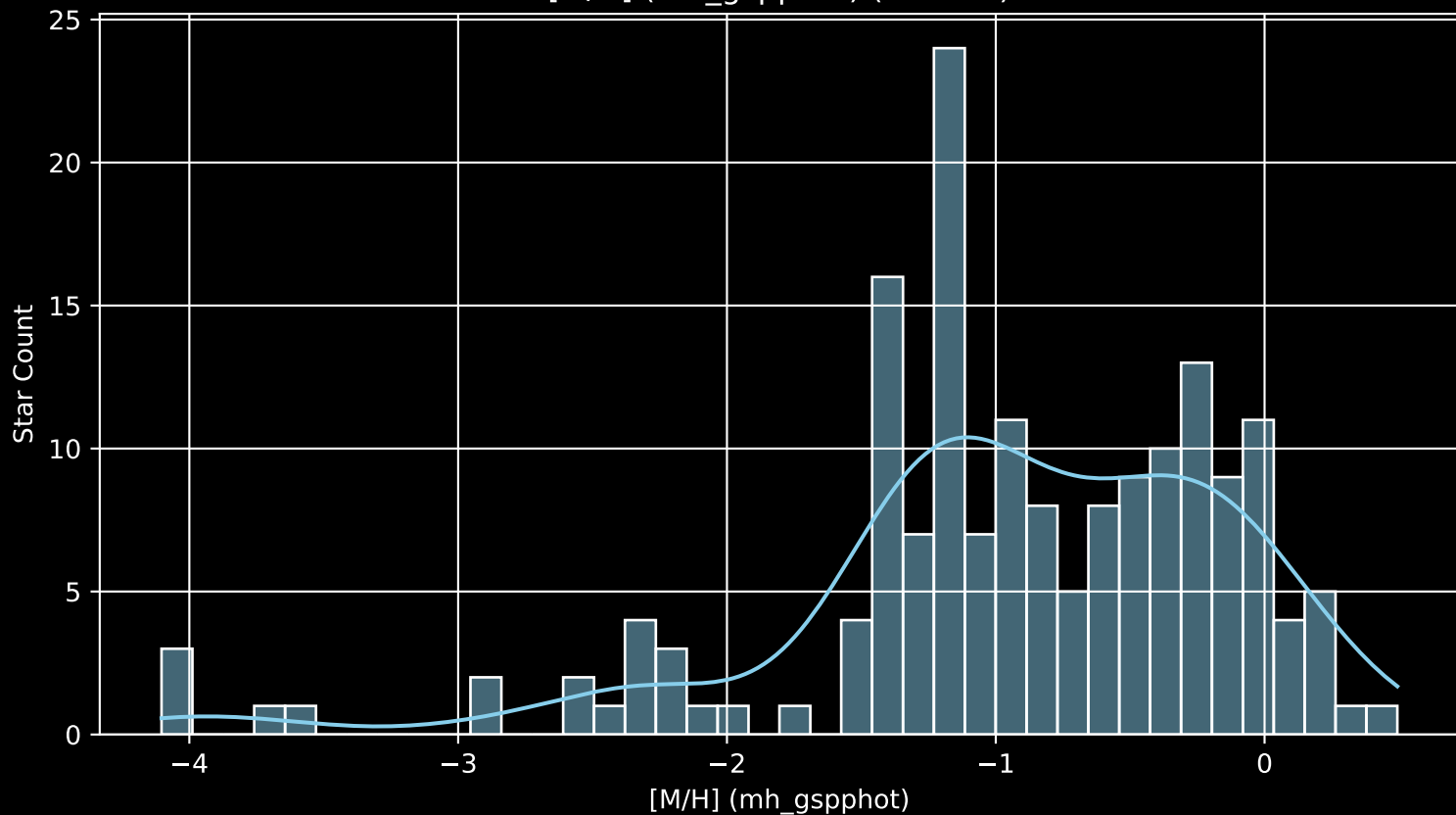
Gaia Cluster: [Lynga_6 [M/H] (mh_gspphot) (n= 173)
