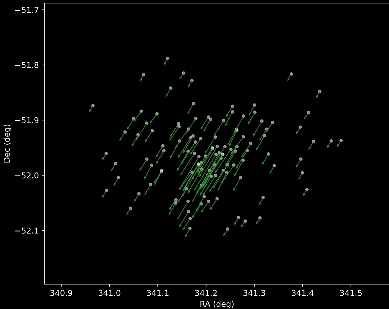
Gaia DR3 Cluster 4 Proper Motion Vectors (n=114)
