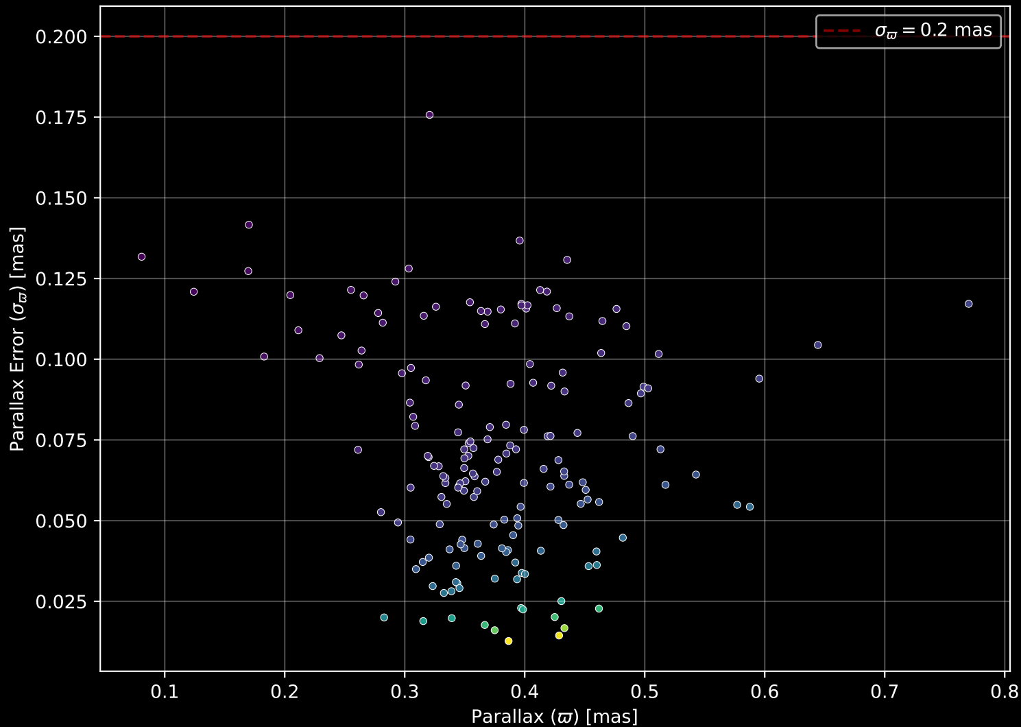
Gaia Cluster: [Lynga_6] Parallax Quality (n= 175)
