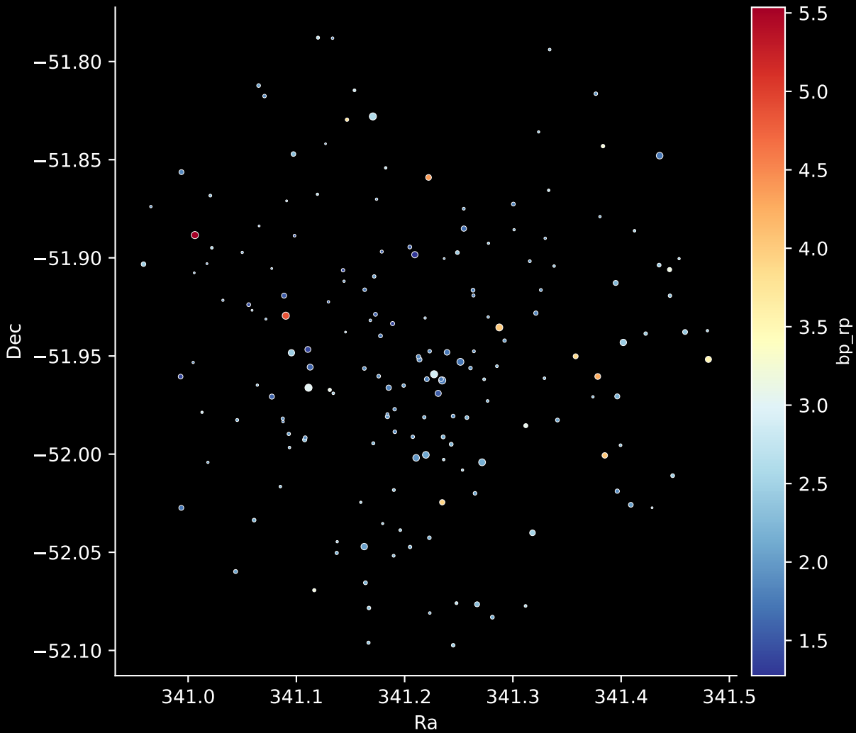
Gaia Cluster: [Lynga_6] Stars: 175
