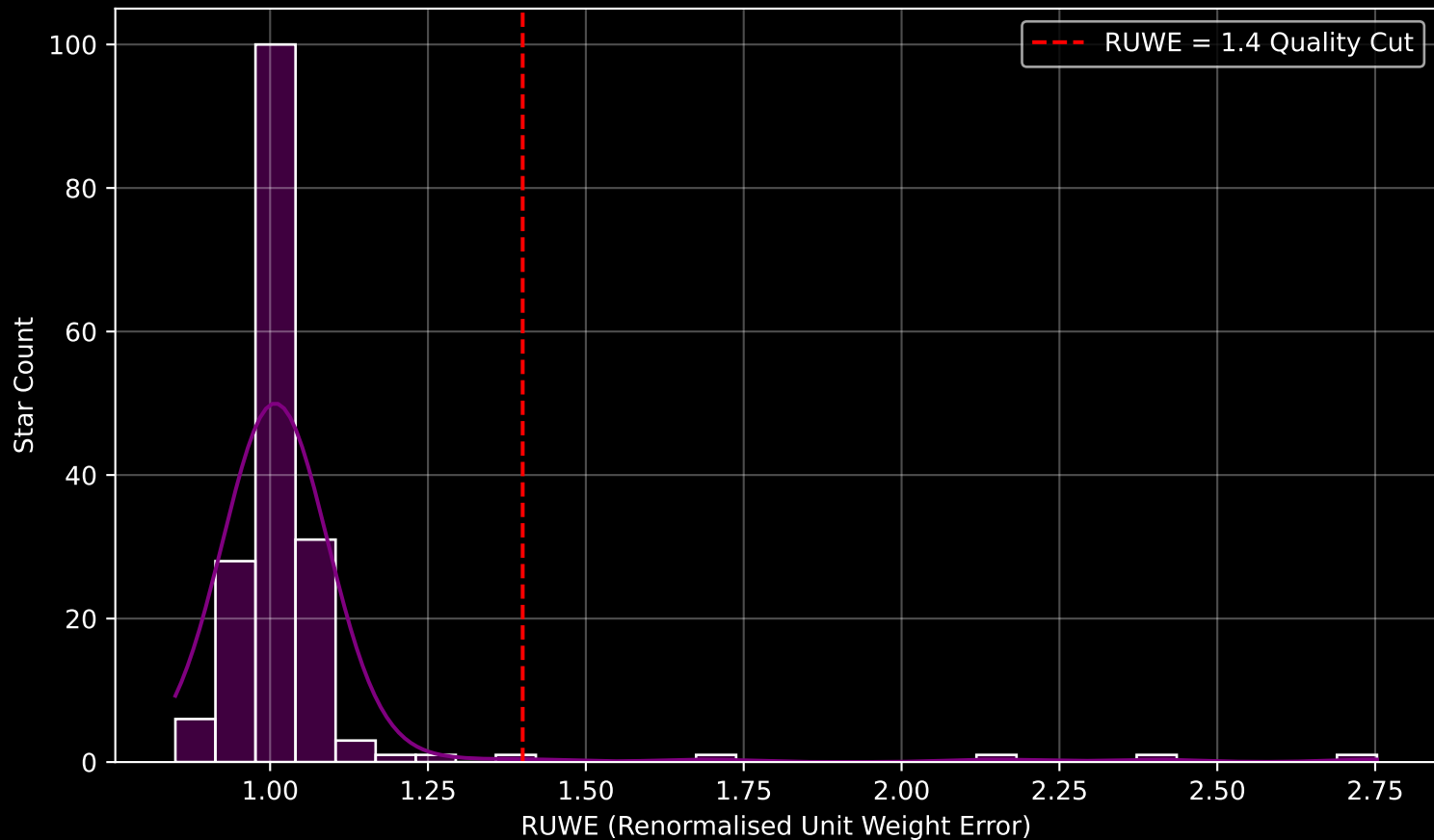
Gaia Cluster: [Lynga_6] RUWE Distribution (n= 175)
