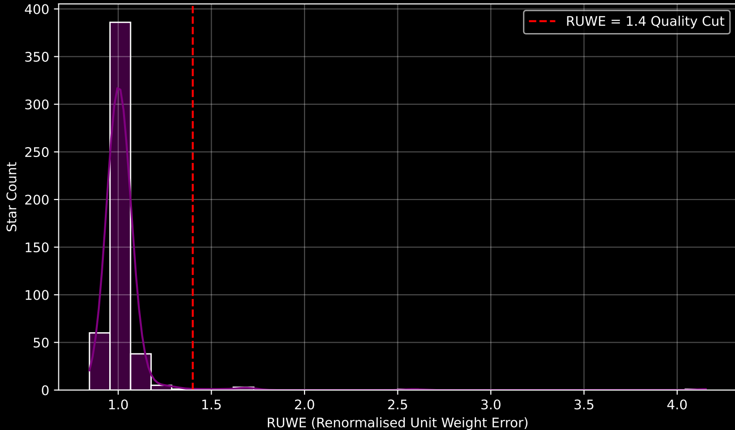
Gaia Cluster: [Lynga_9] RUWE Distribution (n= 497)
