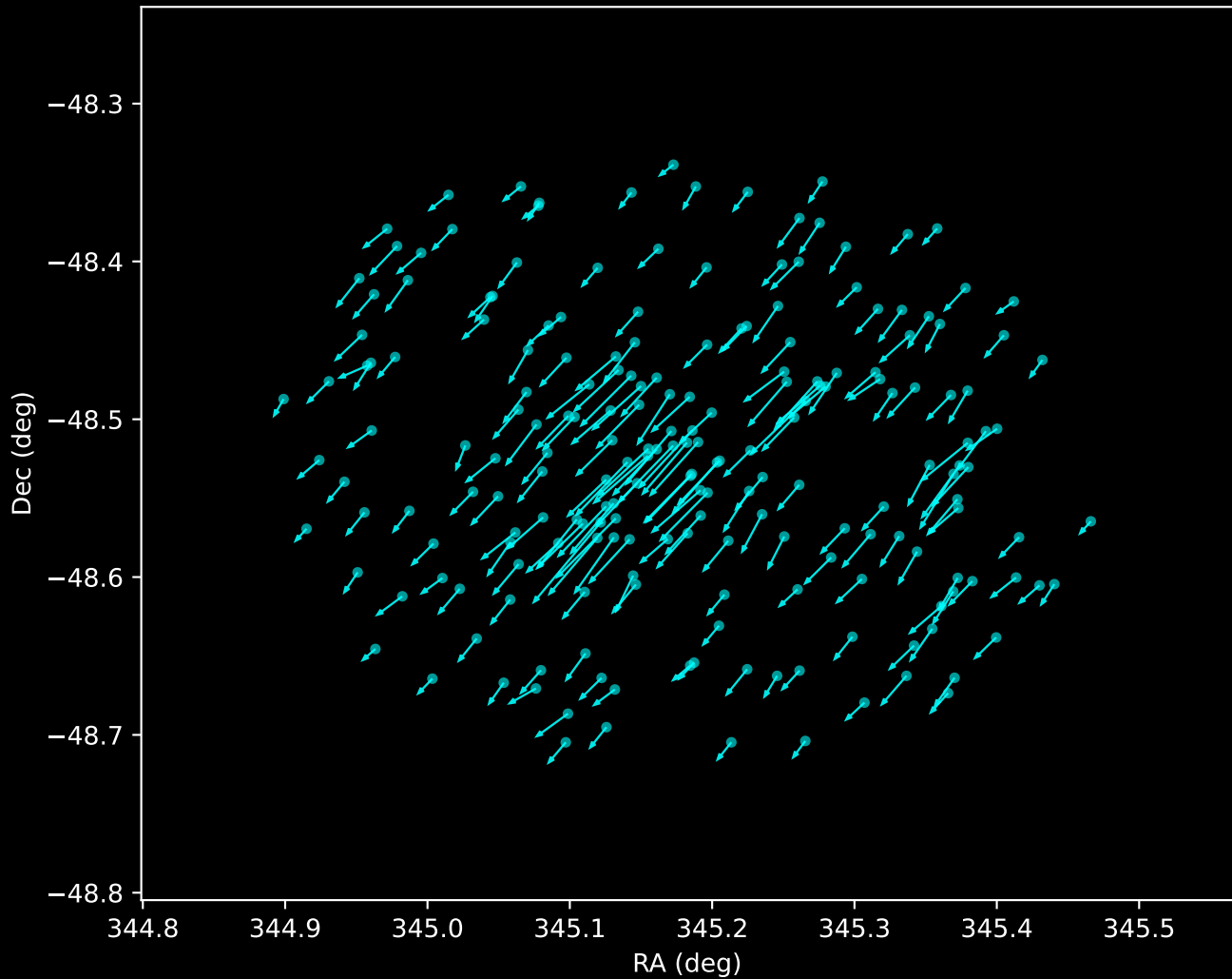
Gaia DR3 Noise Stream Proper Motion Vectors (n=205)
