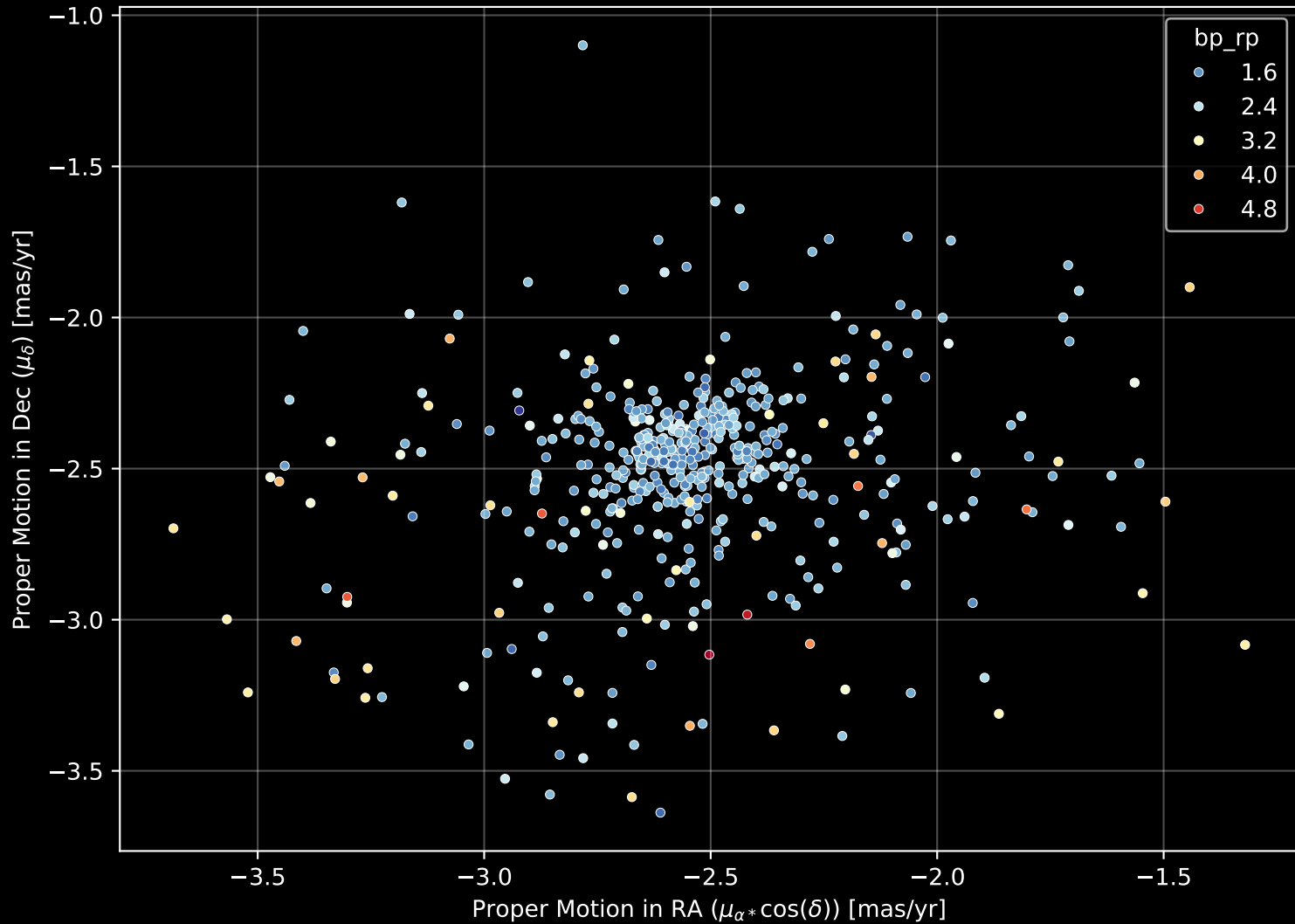
Gaia Cluster: [Lynga_9] Proper Motion Diagram (n= 497)
