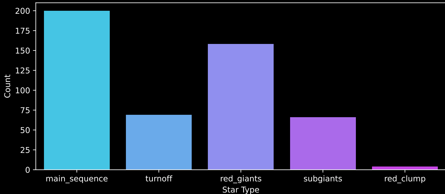
Gaia Cluster: [Lynga_9] Count plot of Star Type
