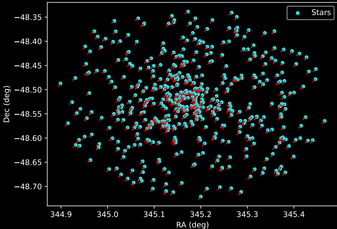
Gaia Cluster: [Lynga_9] Proper Motion Vectors for Gaia Star Field (n= 497)
