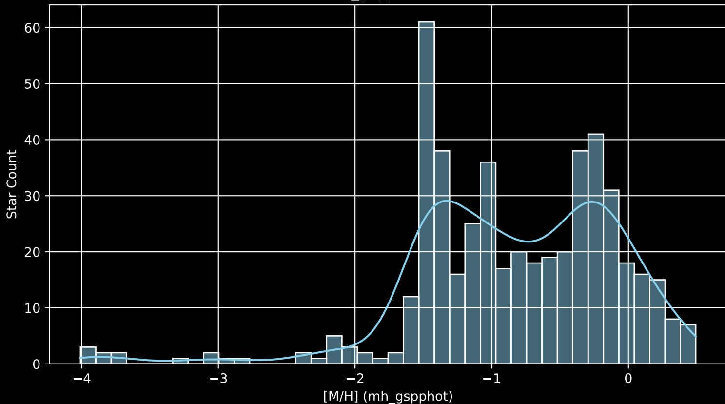
Gaia Cluster: [Lynga_9 [M/H] (mh_gspphot) (n= 484)
