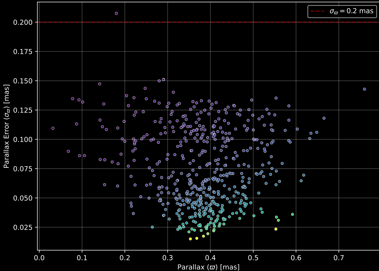
Gaia Cluster: [Lynga_9] Parallax Quality (n= 497)
