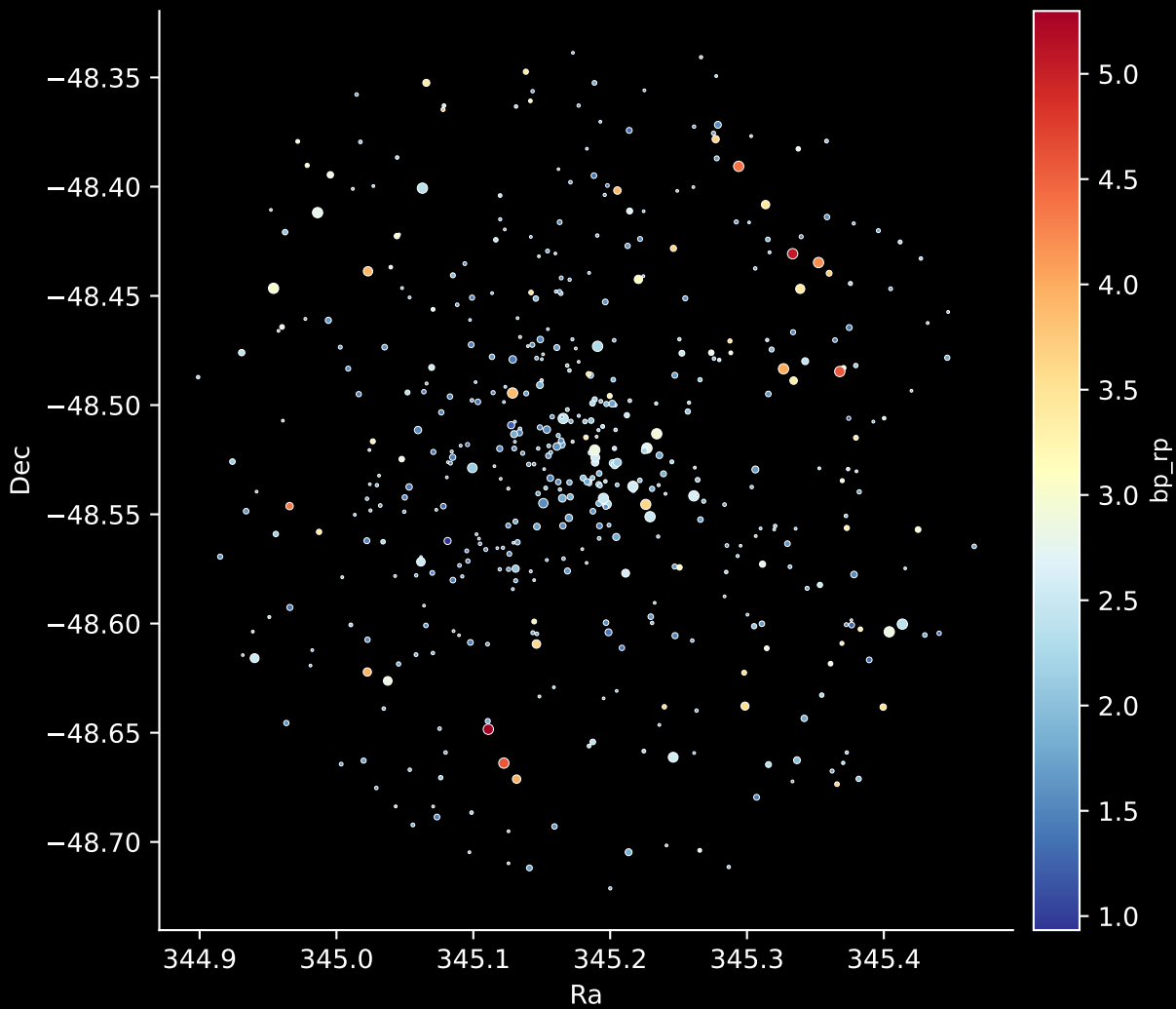
Gaia Cluster: [Lynga_9] Stars: 497
