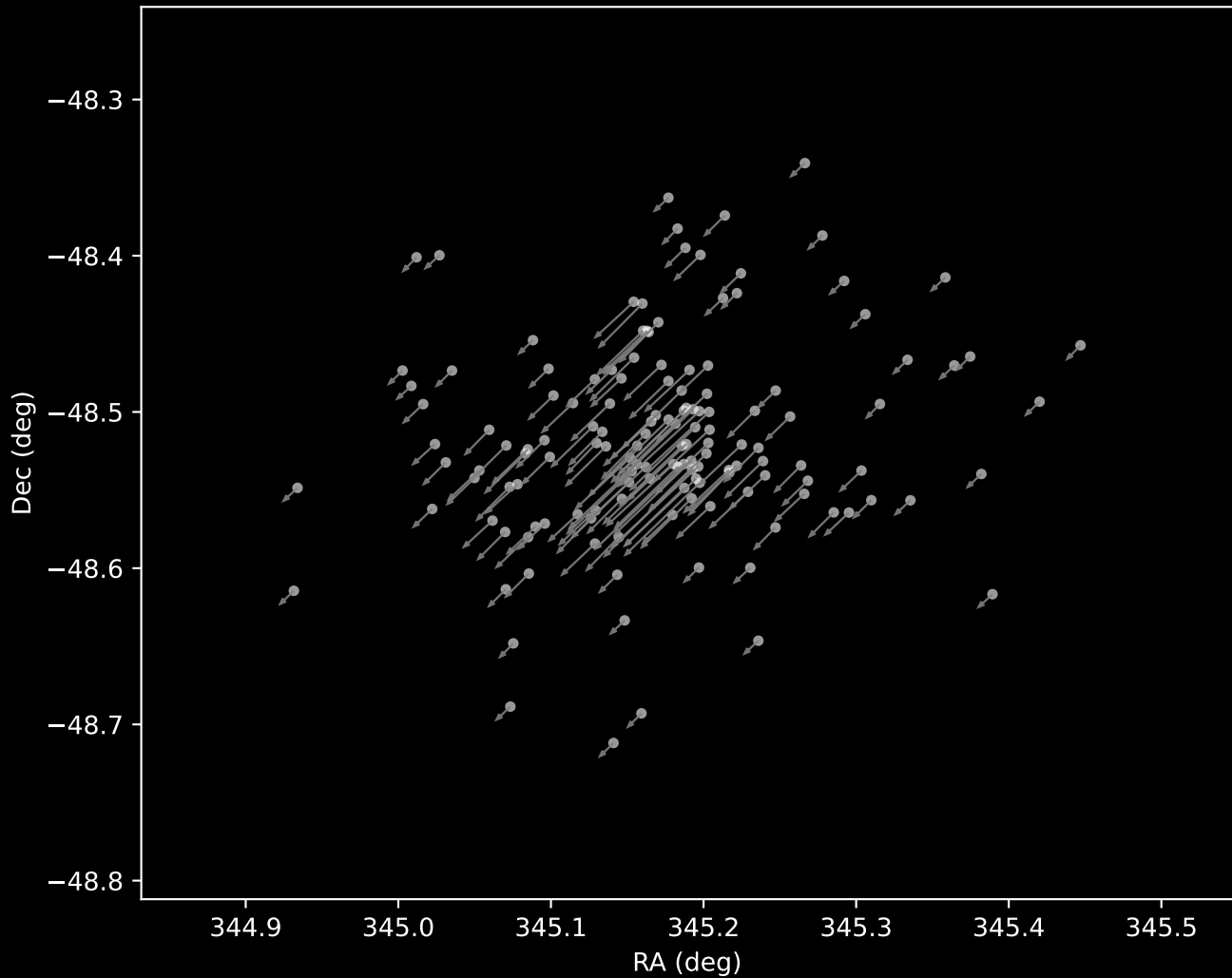
Gaia DR3 Cluster 14 Proper Motion Vectors (n=144)
