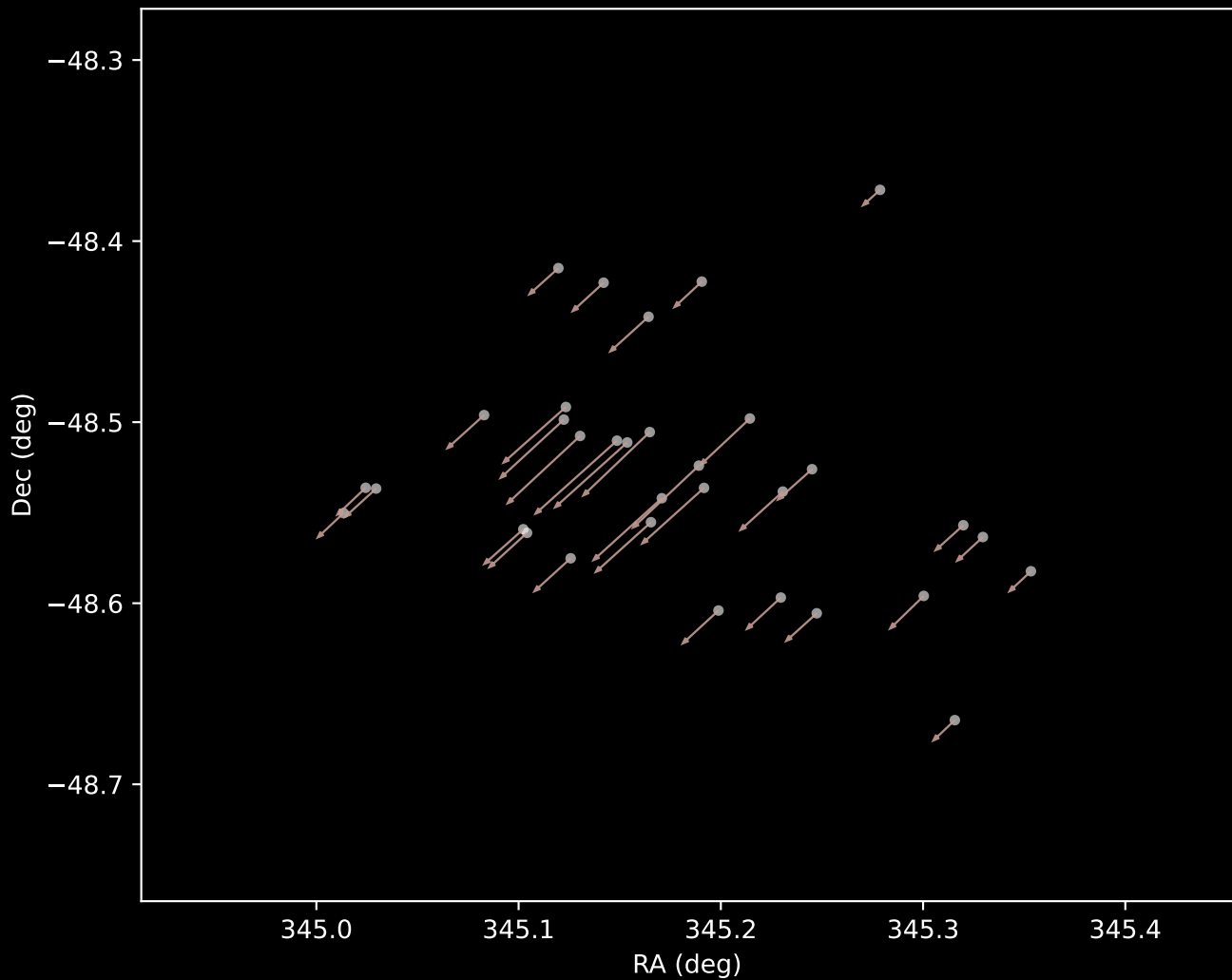
Gaia DR3 Cluster 11 Proper Motion Vectors (n=33)
