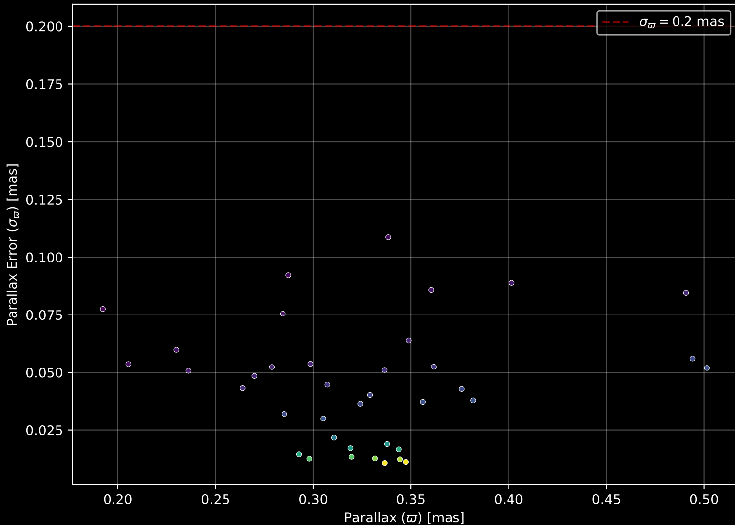
Gaia Cluster: [Markarian_50] Parallax Quality (n= 38)
