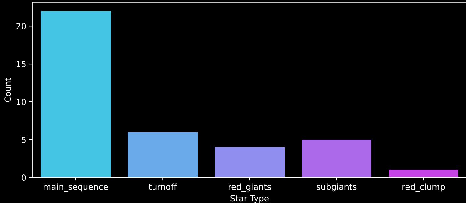
Gaia Cluster: [Markarian_50] Count plot of Star Type
