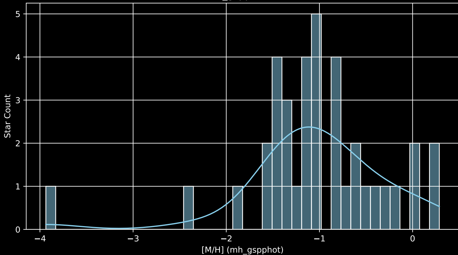
Gaia Cluster: [Markarian_50 [M/H] (mh_gspphot) (n= 37)
