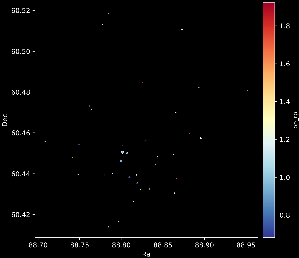
Gaia Cluster: [Markarian_50] Stars: 38
