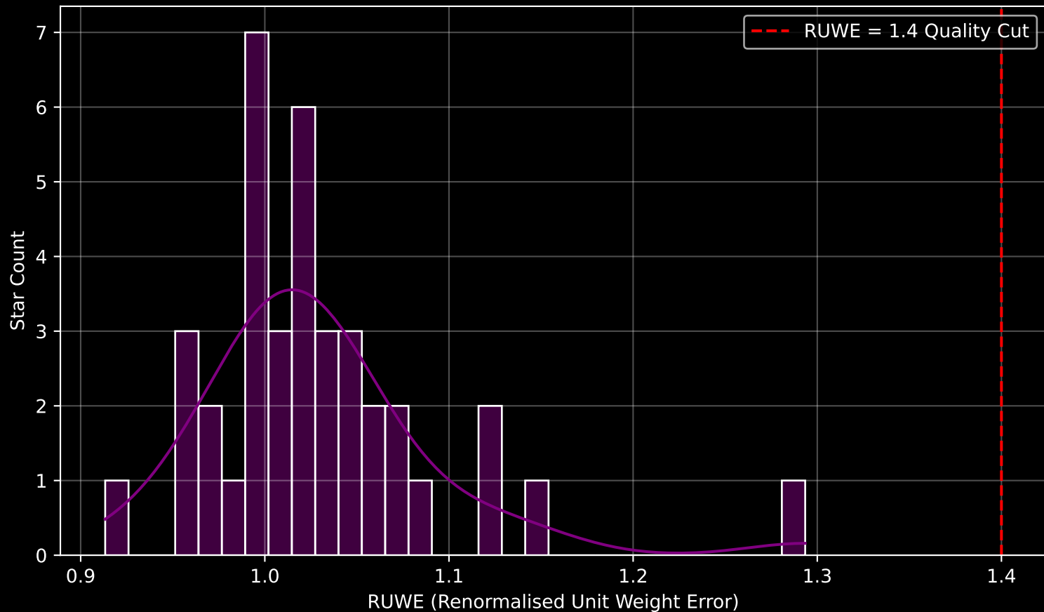
Gaia Cluster: [Markarian_50] RUWE Distribution (n= 38)
