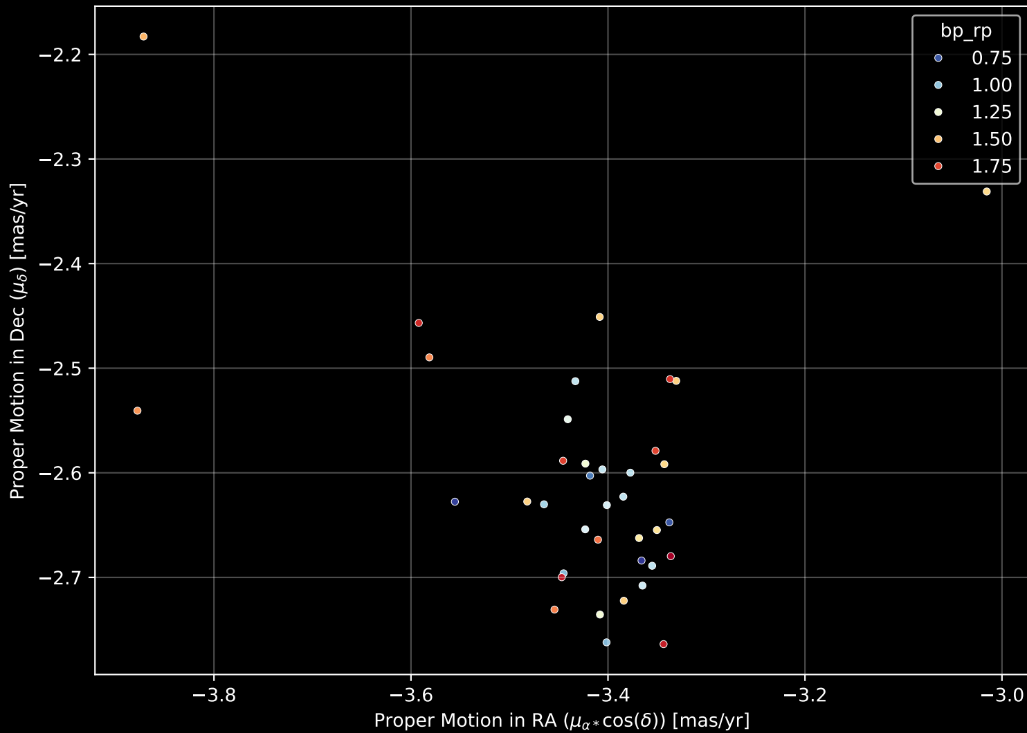
Gaia Cluster: [Markarian_50] Proper Motion Diagram (n= 38)
