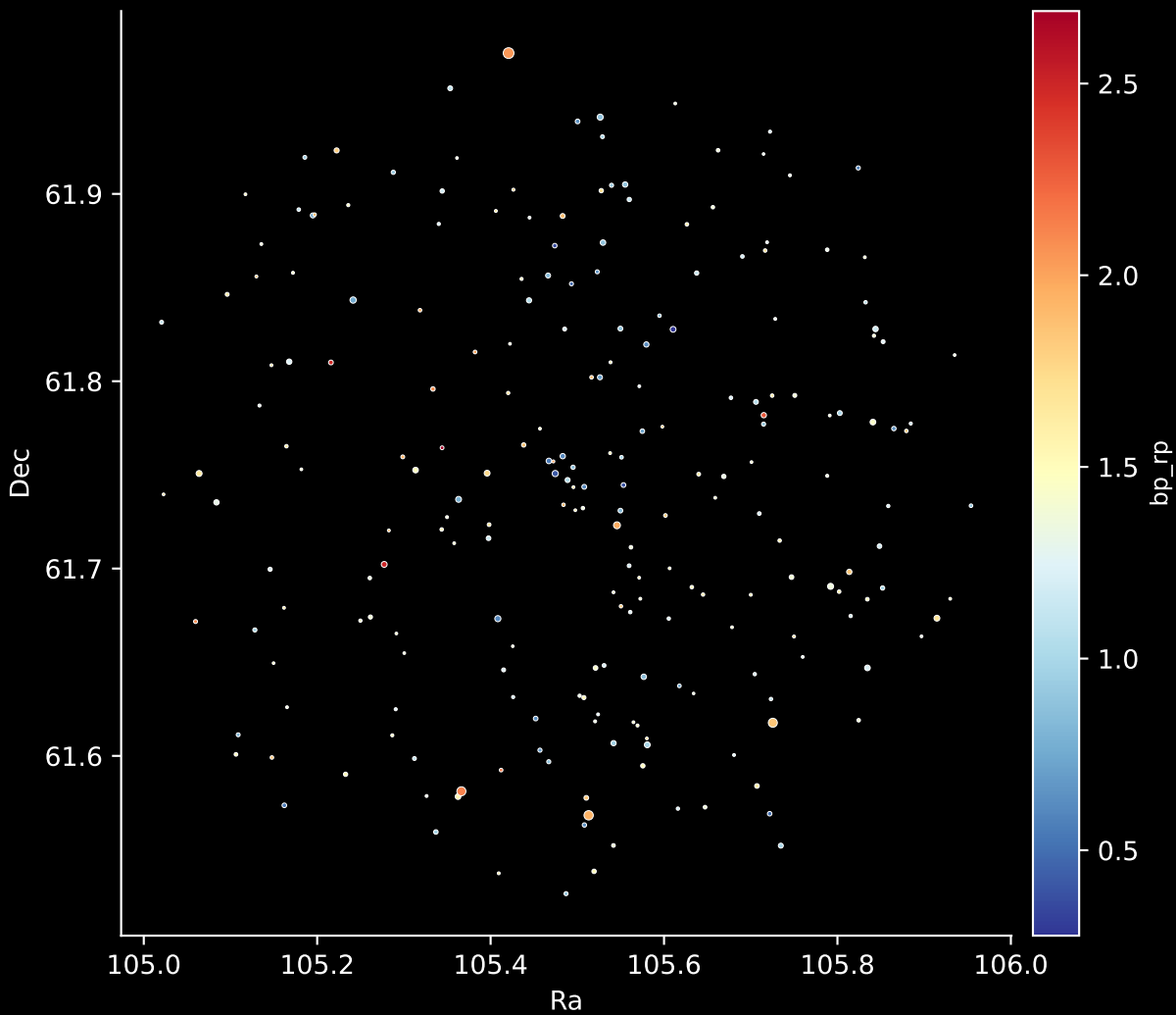
Gaia Cluster: [Mayer_1] Stars: 224
