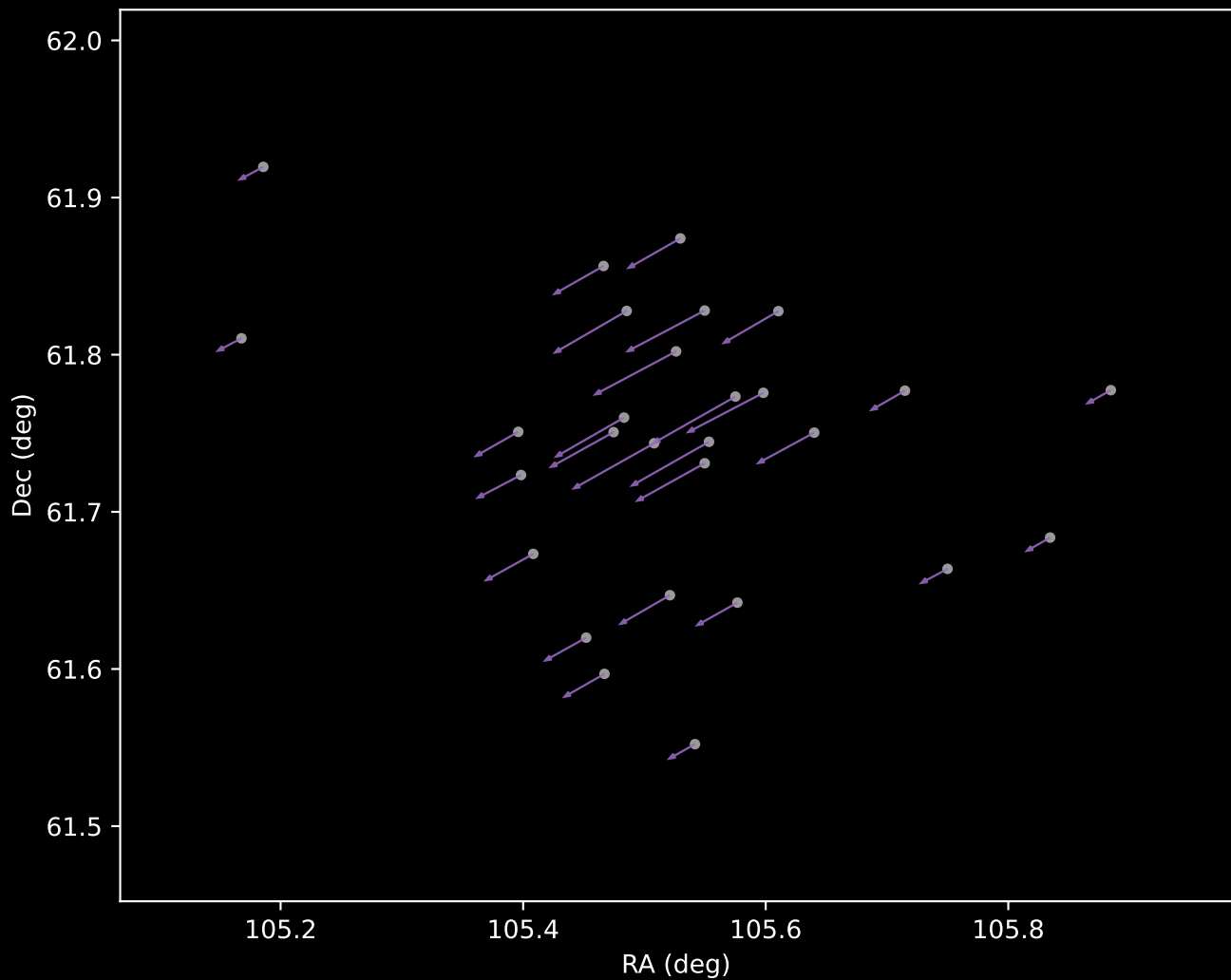
Gaia DR3 Cluster 8 Proper Motion Vectors (n=28)
