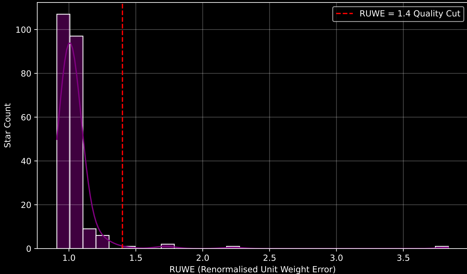
Gaia Cluster: [Mayer_1] RUWE Distribution (n= 224)
