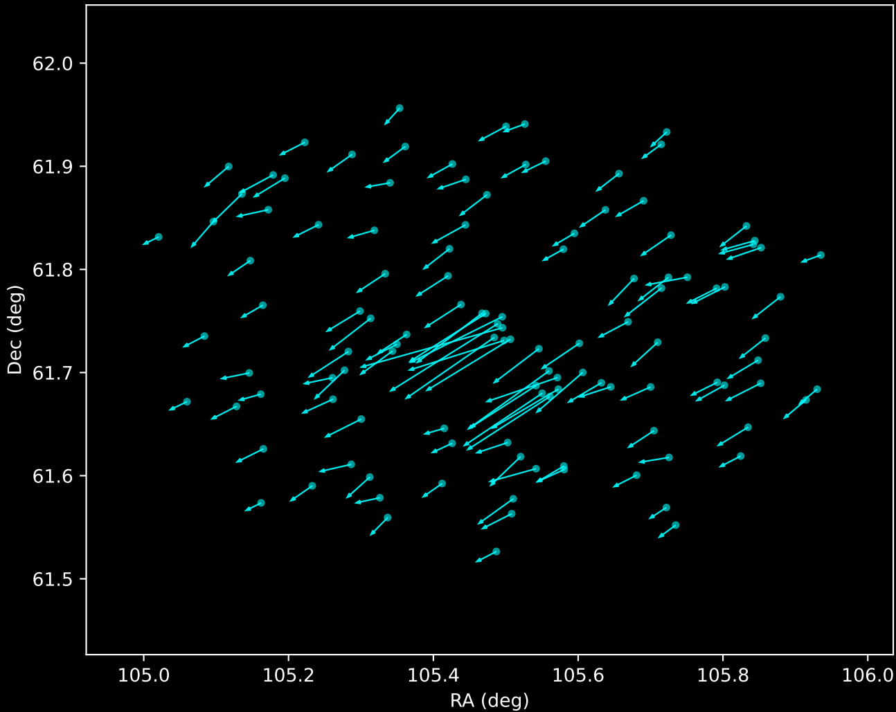
Gaia DR3 Noise Stream Proper Motion Vectors (n=117)
