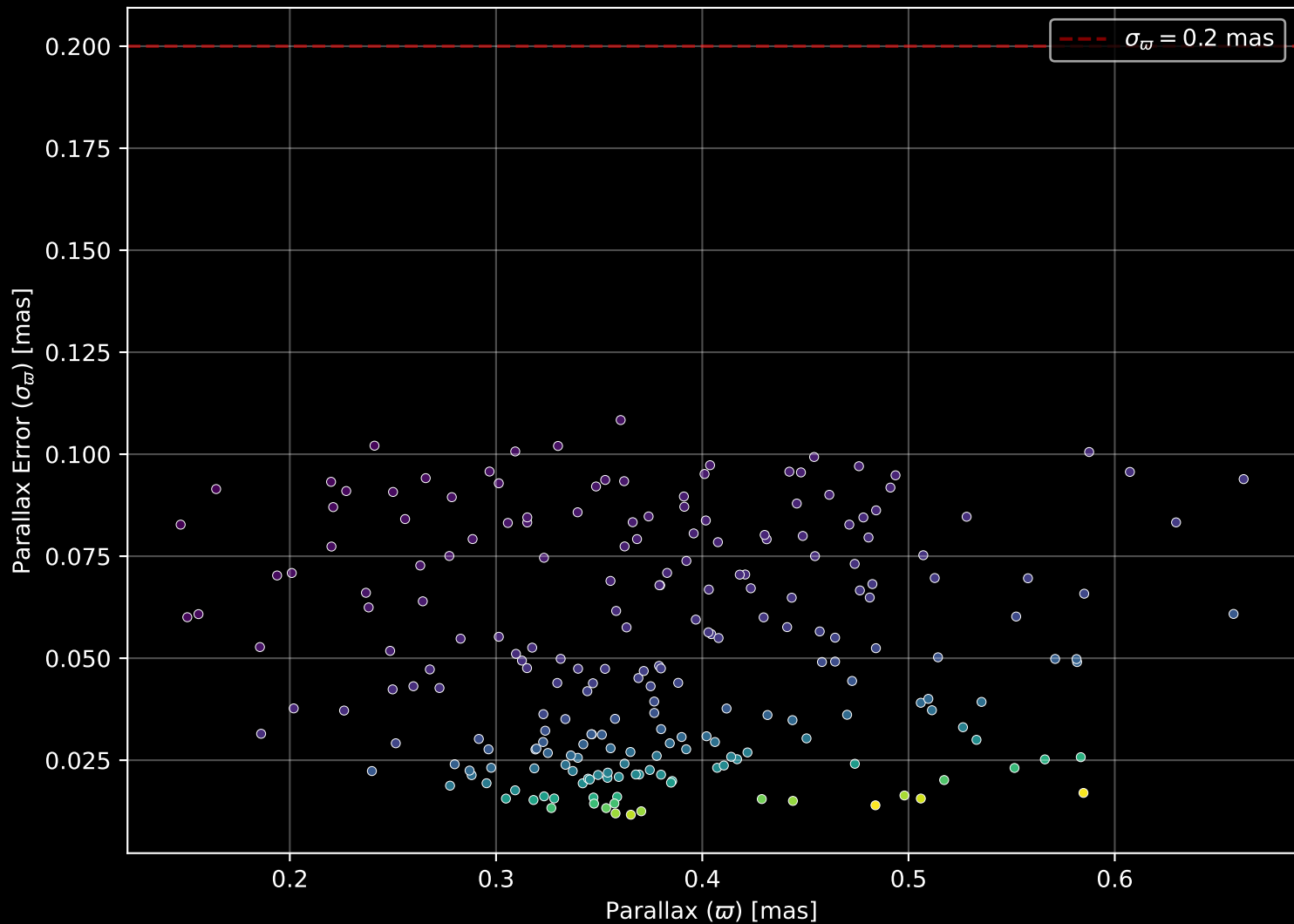
Gaia Cluster: [Mayer_1] Parallax Quality (n= 224)
