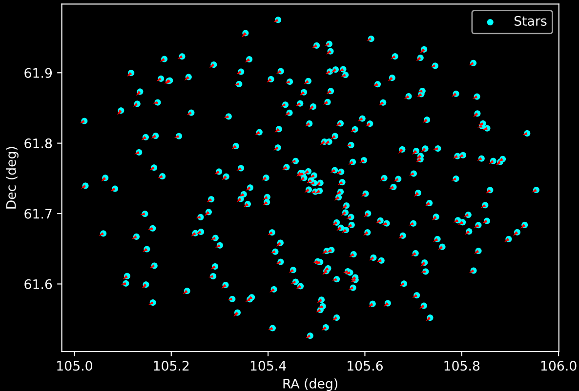
Gaia Cluster: [Mayer_1] Proper Motion Vectors for Gaia Star Field (n= 224)
