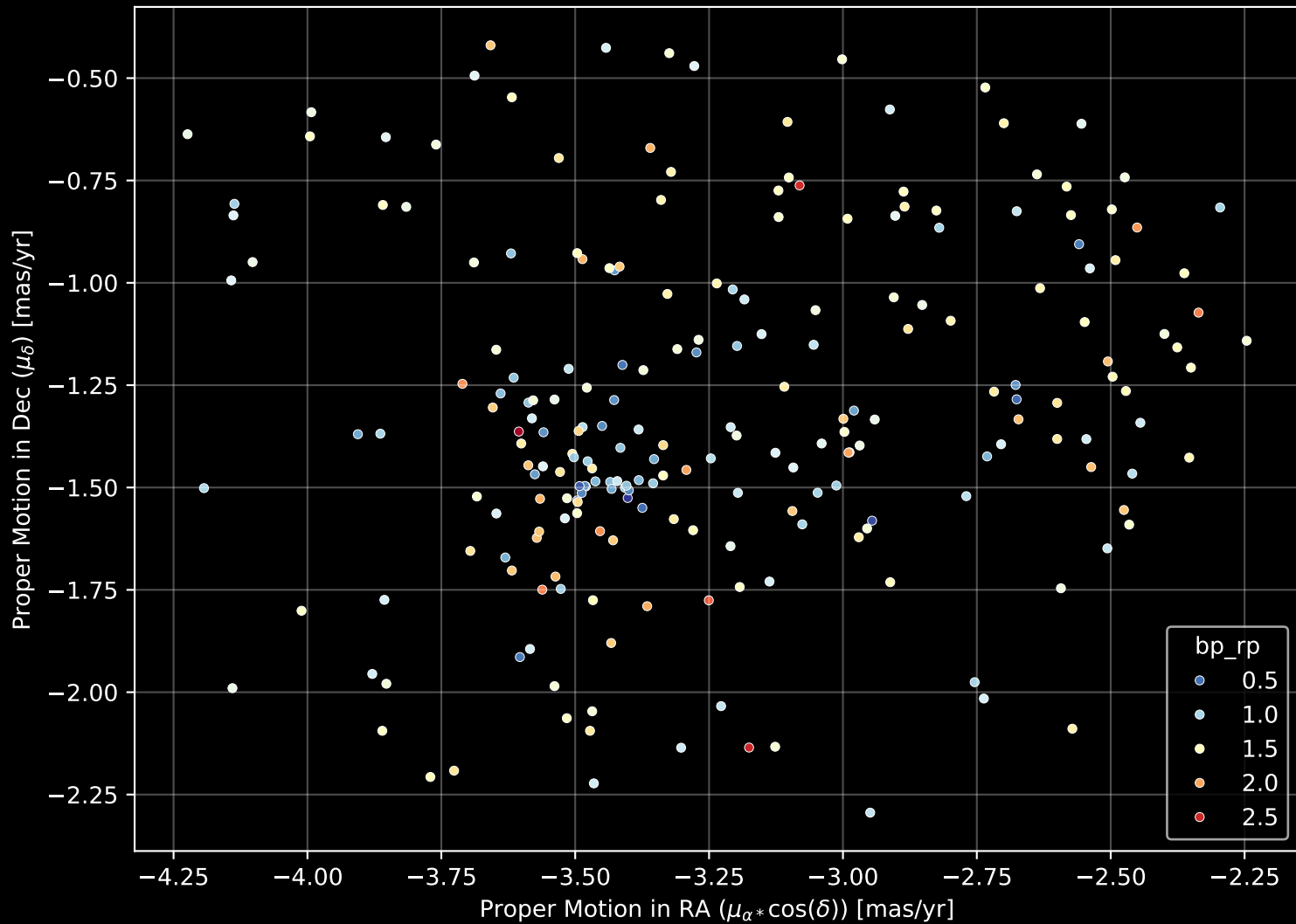
Gaia Cluster: [Mayer_1] Proper Motion Diagram (n= 224)
