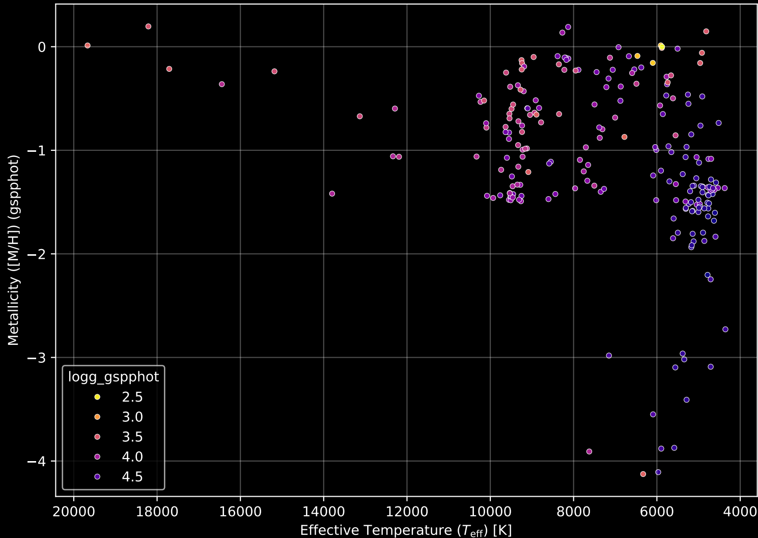
Gaia Cluster: [Mayer_1] Stellar Population Parameters (n= 224)
