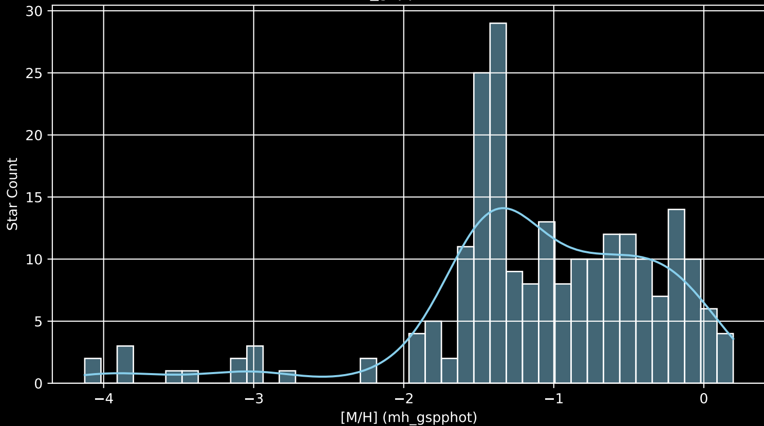
Gaia Cluster: [Mayer_1 [M/H] (mh_gspphot) (n= 224)
