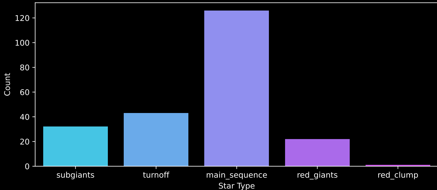
Gaia Cluster: [Mayer_1] Count plot of Star Type
