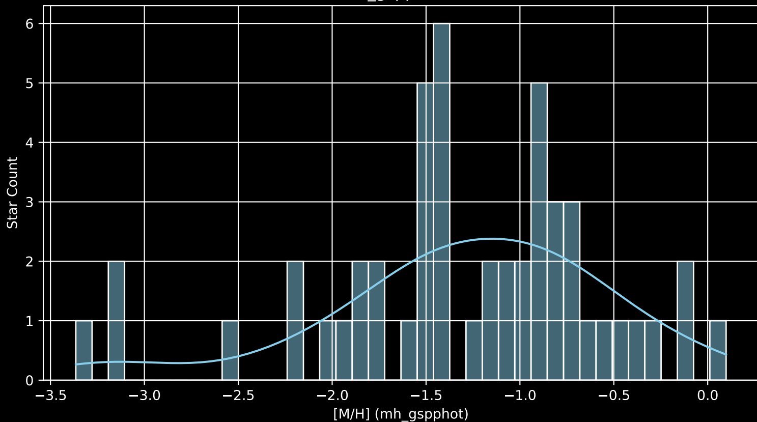
Gaia Cluster: [Mayer_3 [M/H] (mh_gspphot) (n= 50)
