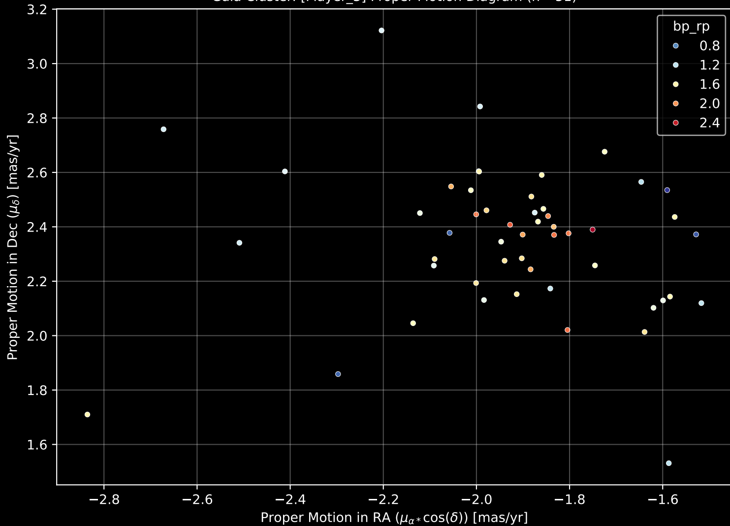
Gaia Cluster: [Mayer_3] Proper Motion Diagram (n= 51)
