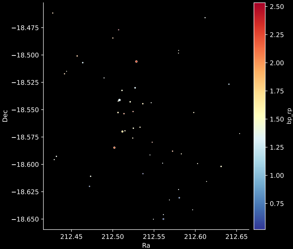
Gaia Cluster: [Mayer_3] Stars: 51
