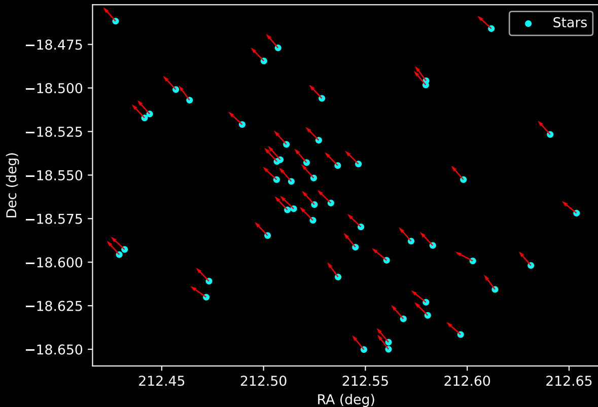
Gaia Cluster: [Mayer_3] Proper Motion Vectors for Gaia Star Field (n= 51)
