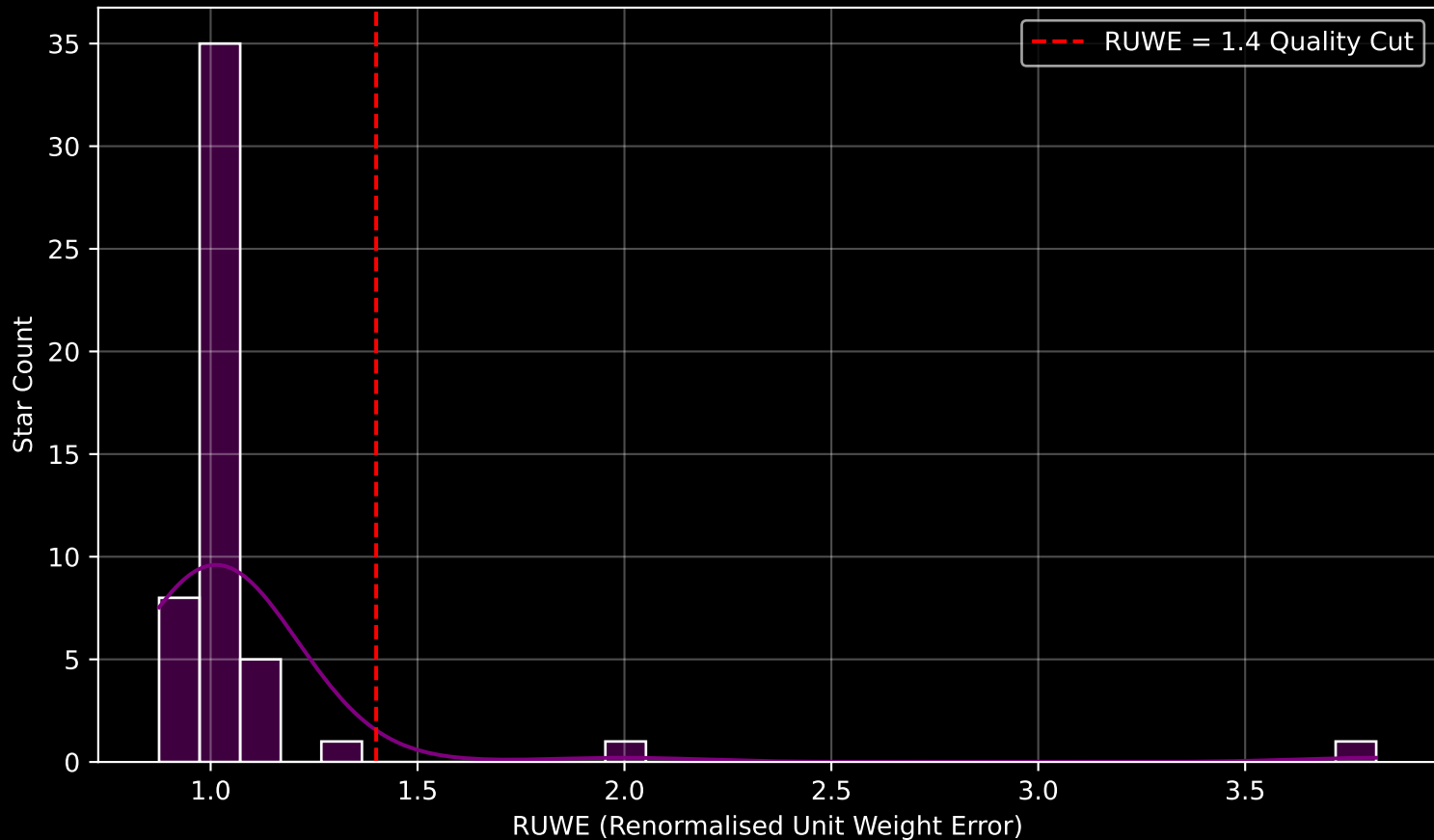
Gaia Cluster: [Mayer_3] RUWE Distribution (n= 51)
