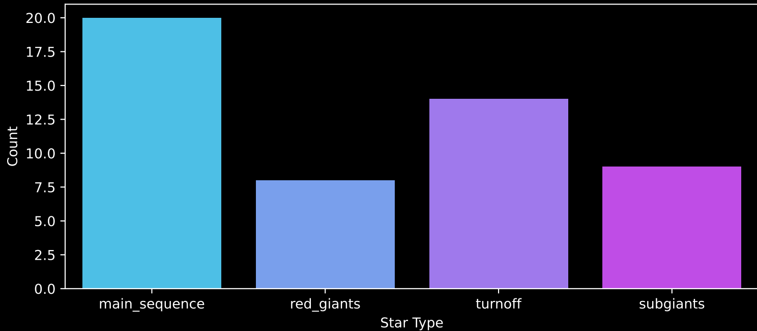
Gaia Cluster: [Mayer_3] Count plot of Star Type
