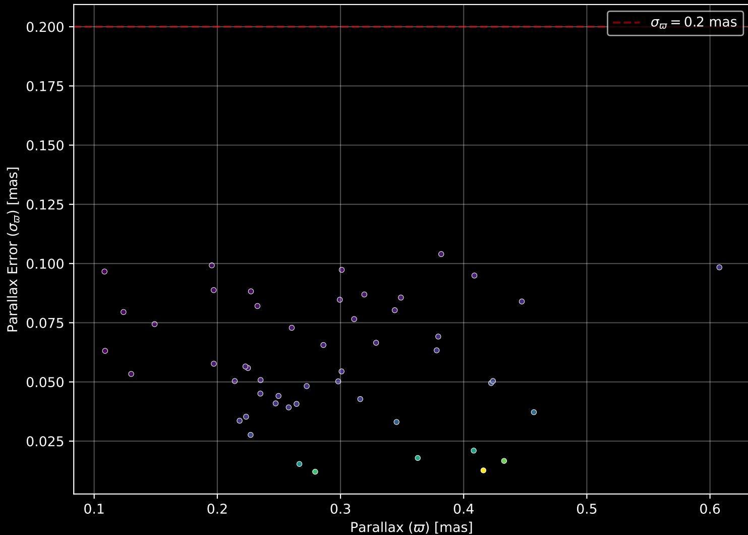
Gaia Cluster: [Mayer_3] Parallax Quality (n= 51)
