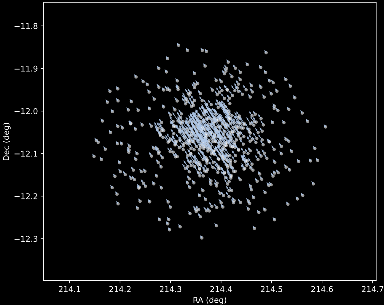
Gaia DR3 Cluster 1 Proper Motion Vectors (n=579)
