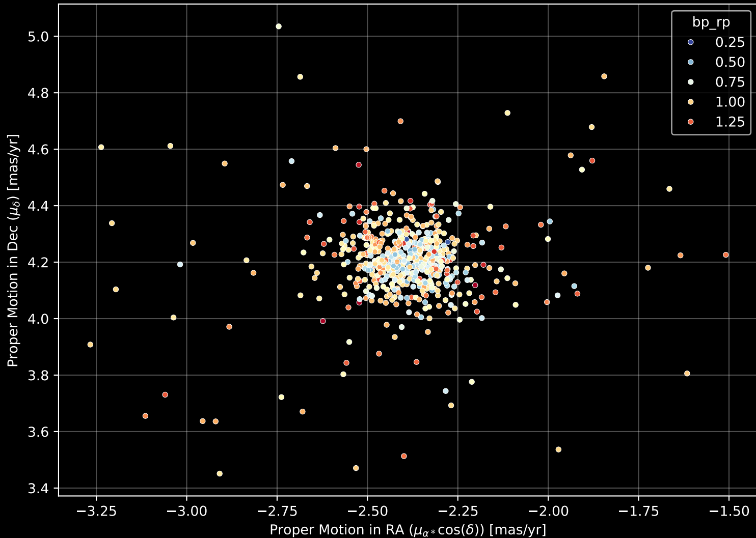
Gaia Cluster: [Melotte_71] Proper Motion Diagram (n= 639)
