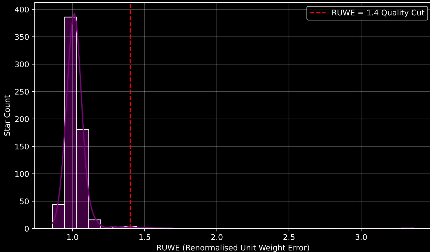
Gaia Cluster: [Melotte_71] RUWE Distribution (n= 639)
