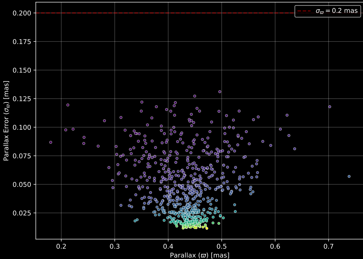
Gaia Cluster: [Melotte_71] Parallax Quality (n= 639)
