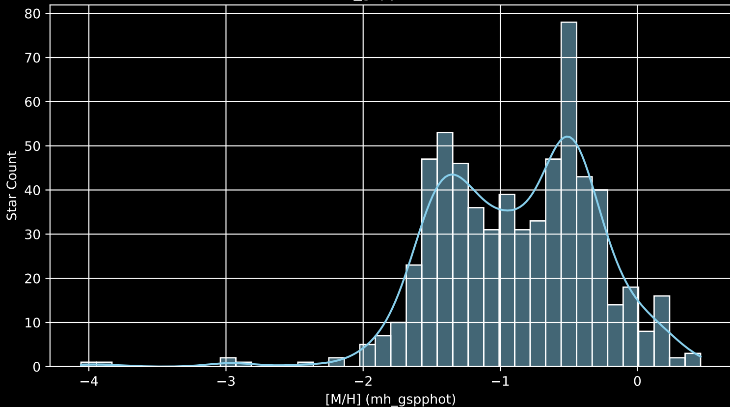
Gaia Cluster: [Melotte_71 [M/H] (mh_gspphot) (n= 638)
