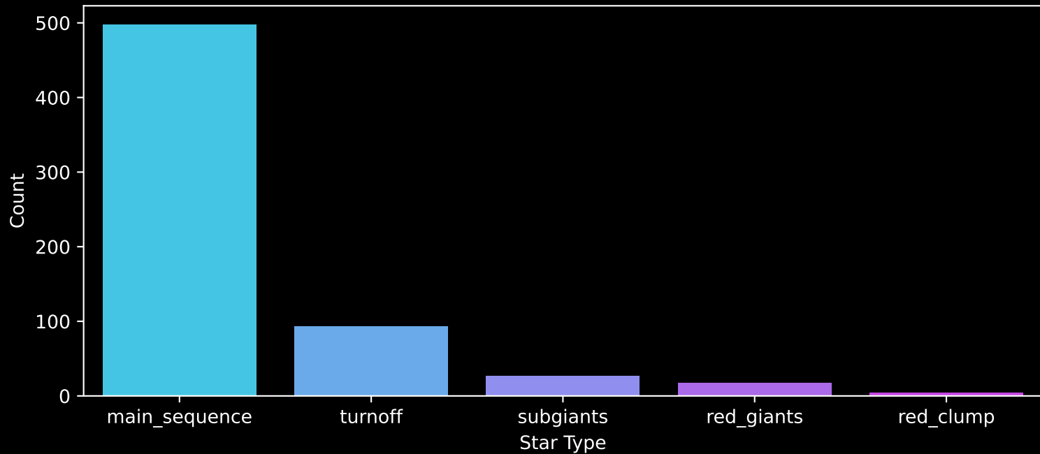
Gaia Cluster: [Melotte_71] Count plot of Star Type
