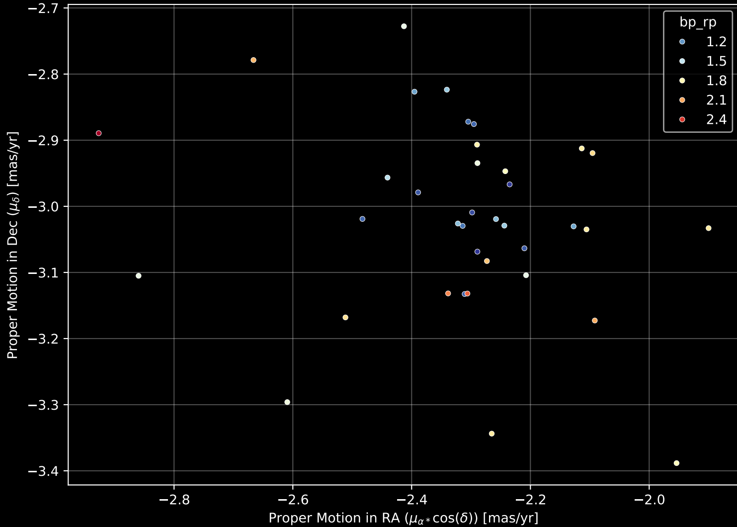
Gaia Cluster: [Moffat_1] Proper Motion Diagram (n= 37)
