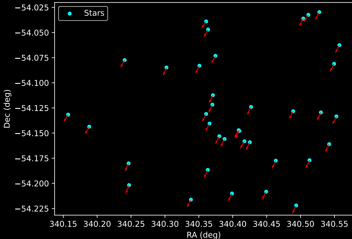
Gaia Cluster: [Moffat_1] Proper Motion Vectors for Gaia Star Field (n= 37)
