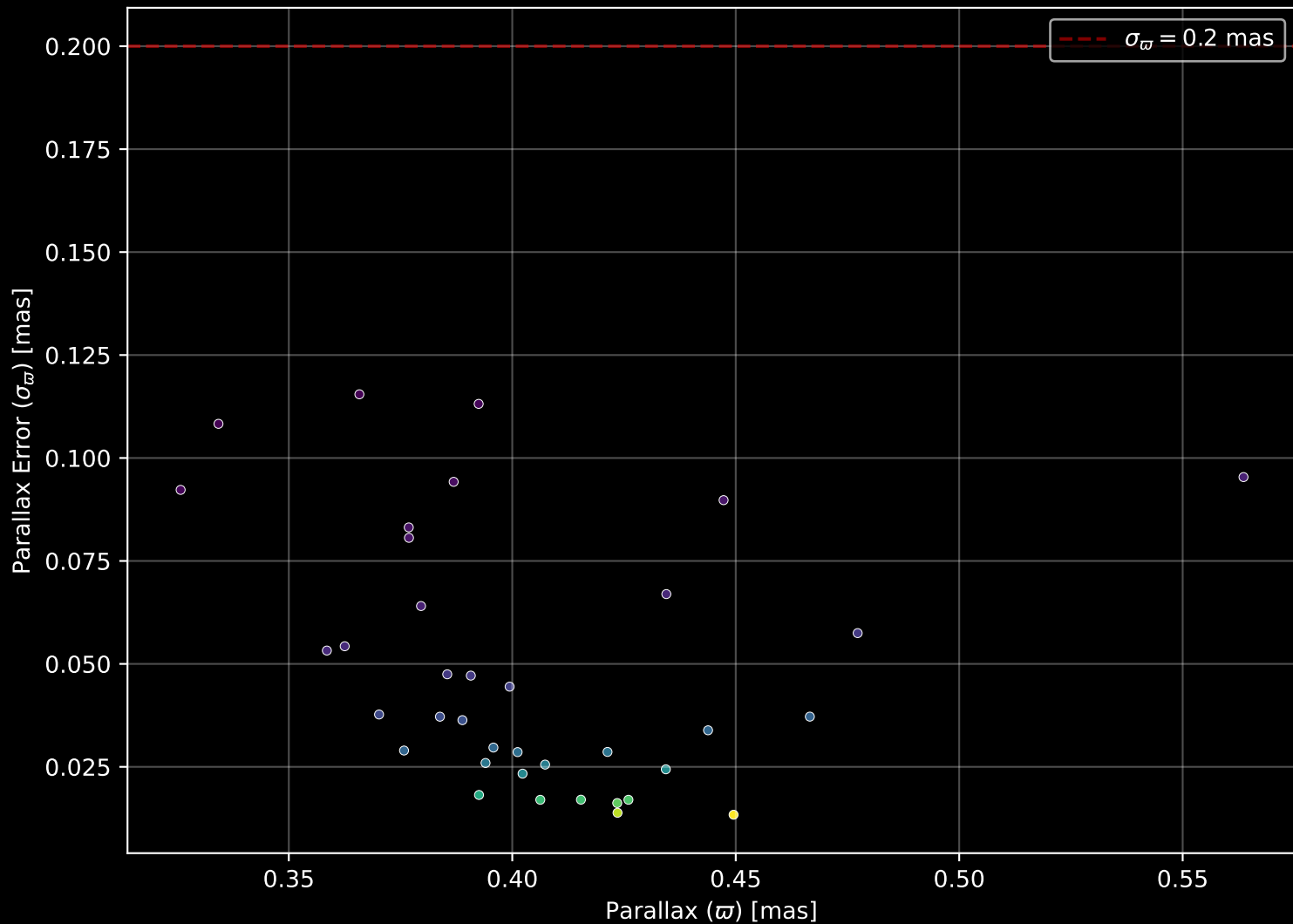
Gaia Cluster: [Moffat_1] Parallax Quality (n= 37)
