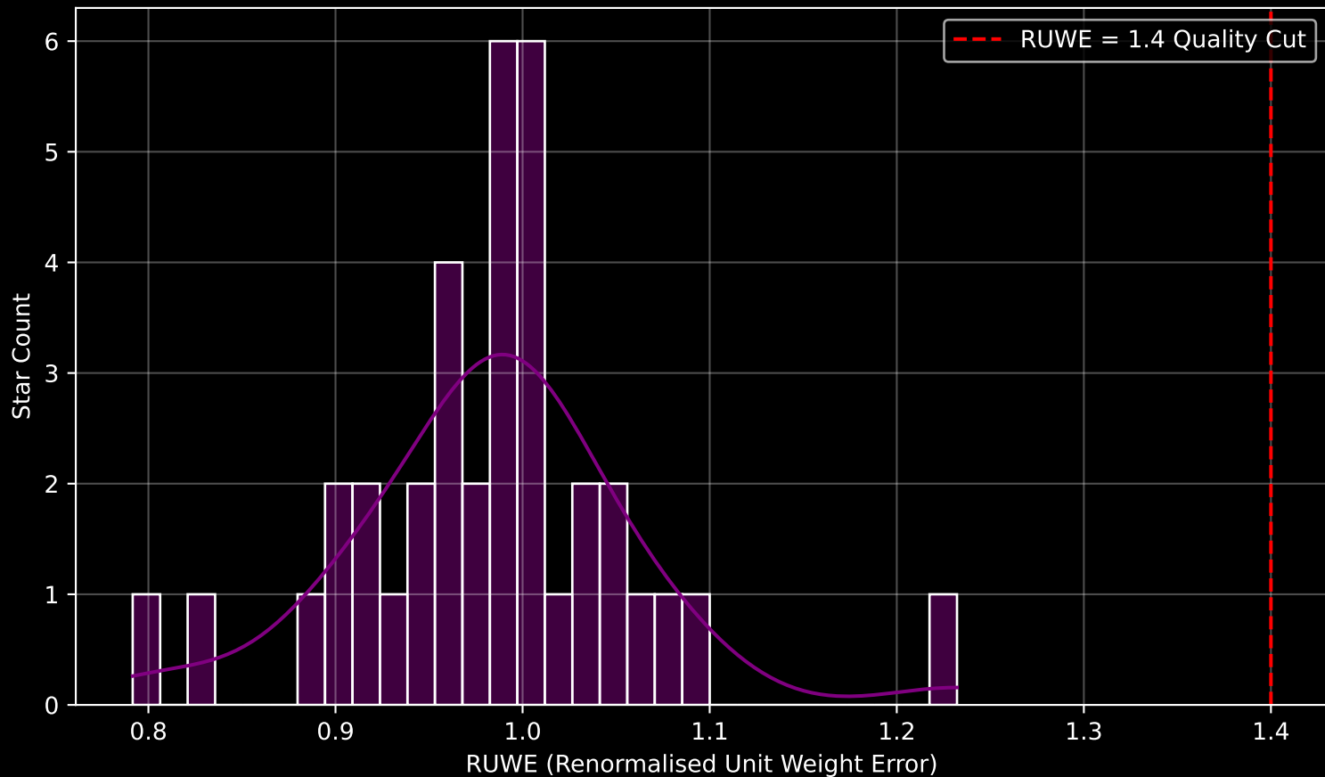
Gaia Cluster: [Moffat_1] RUWE Distribution (n= 37)
