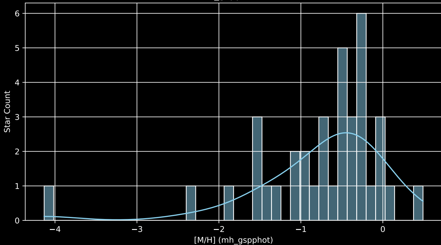
Gaia Cluster: [Moffat_1 [M/H] (mh_gspphot) (n= 37)
