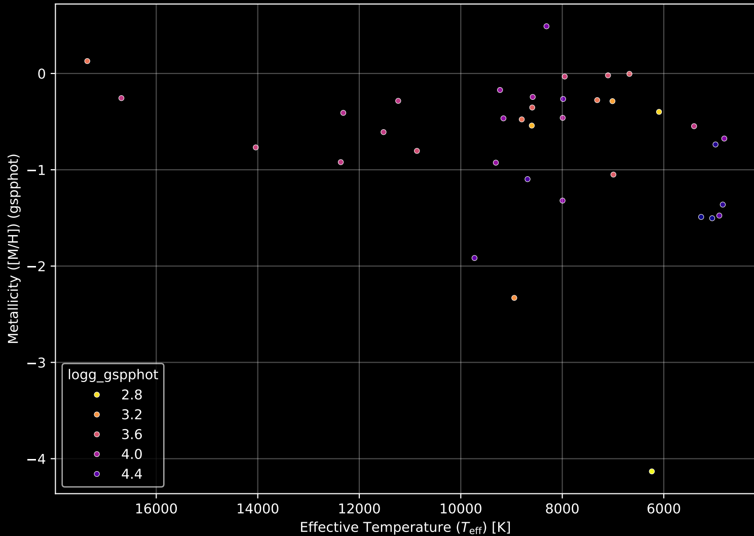
Gaia Cluster: [Moffat_1] Stellar Population Parameters (n= 37)
