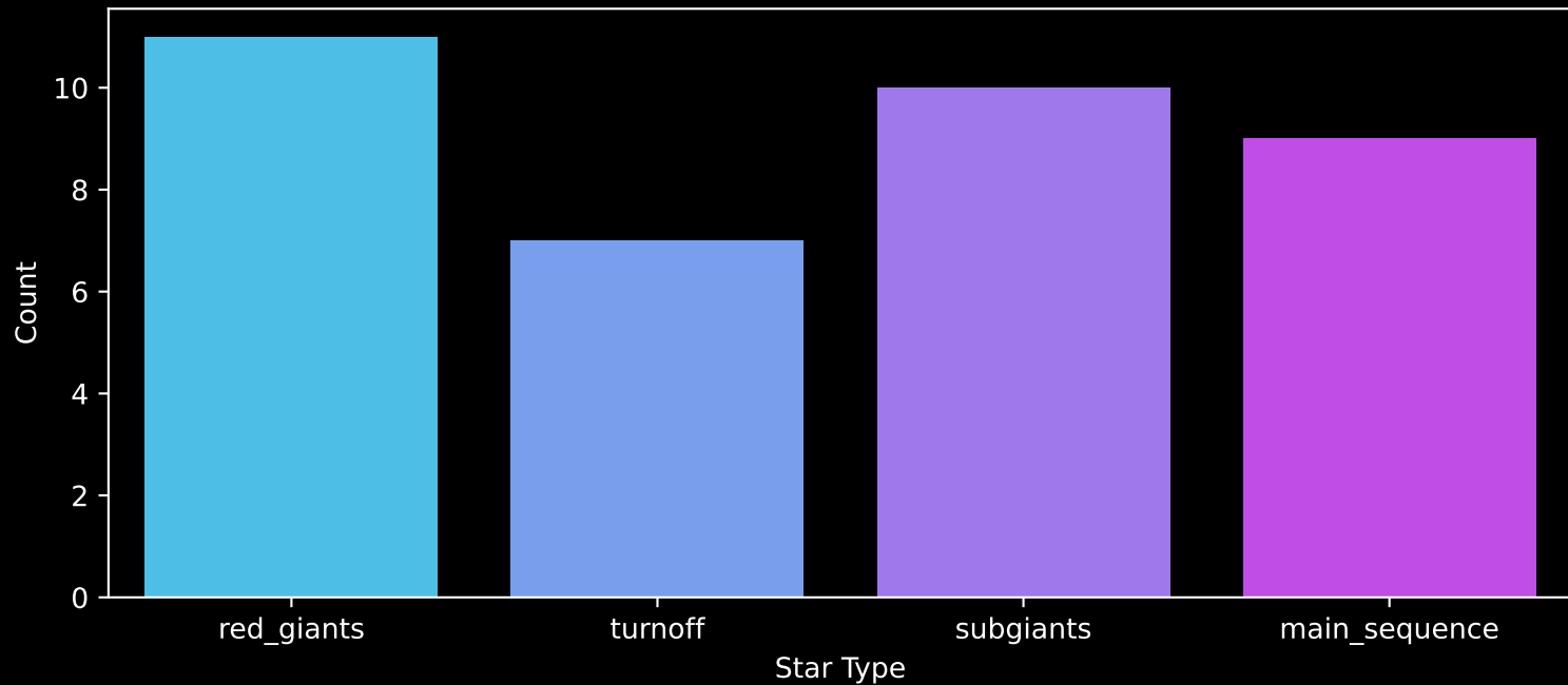
Gaia Cluster: [Moffat_1] Count plot of Star Type
