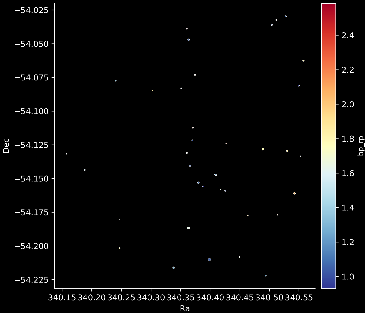
Gaia Cluster: [Moffat_1] Stars: 37
