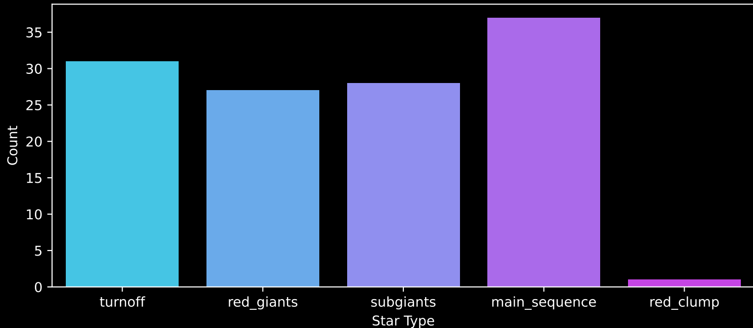
Gaia Cluster: [Muzzio_1] Count plot of Star Type
