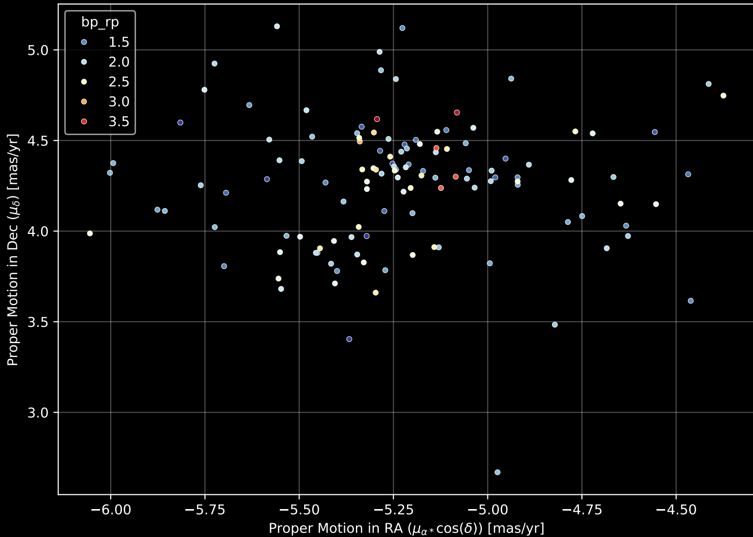
Gaia Cluster: [Muzzio_1] Proper Motion Diagram (n= 124)
