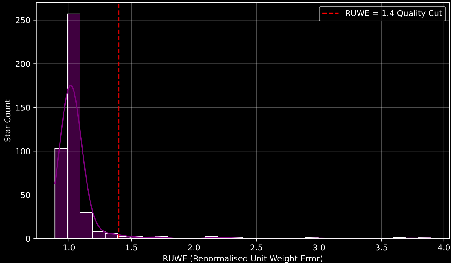
Gaia Cluster: [NGC_1027] RUWE Distribution (n= 417)
