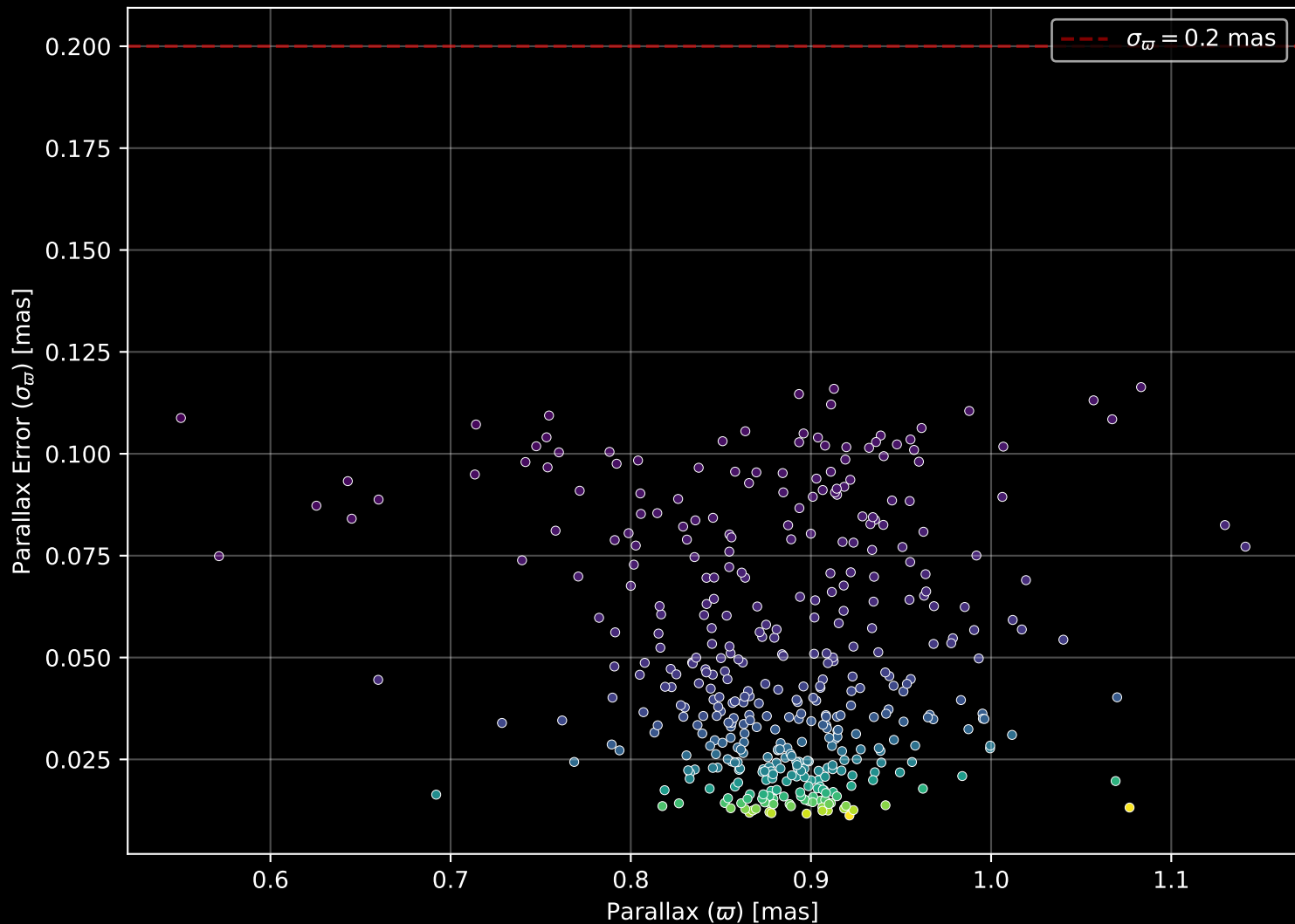
Gaia Cluster: [NGC_1027] Parallax Quality (n= 417)
