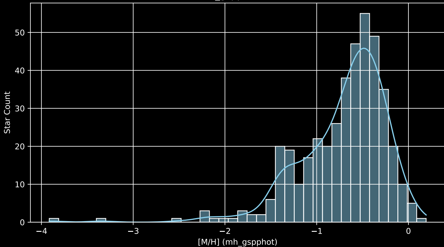
Gaia Cluster: [NGC_1027 [M/H] (mh_gspphot) (n= 416)
