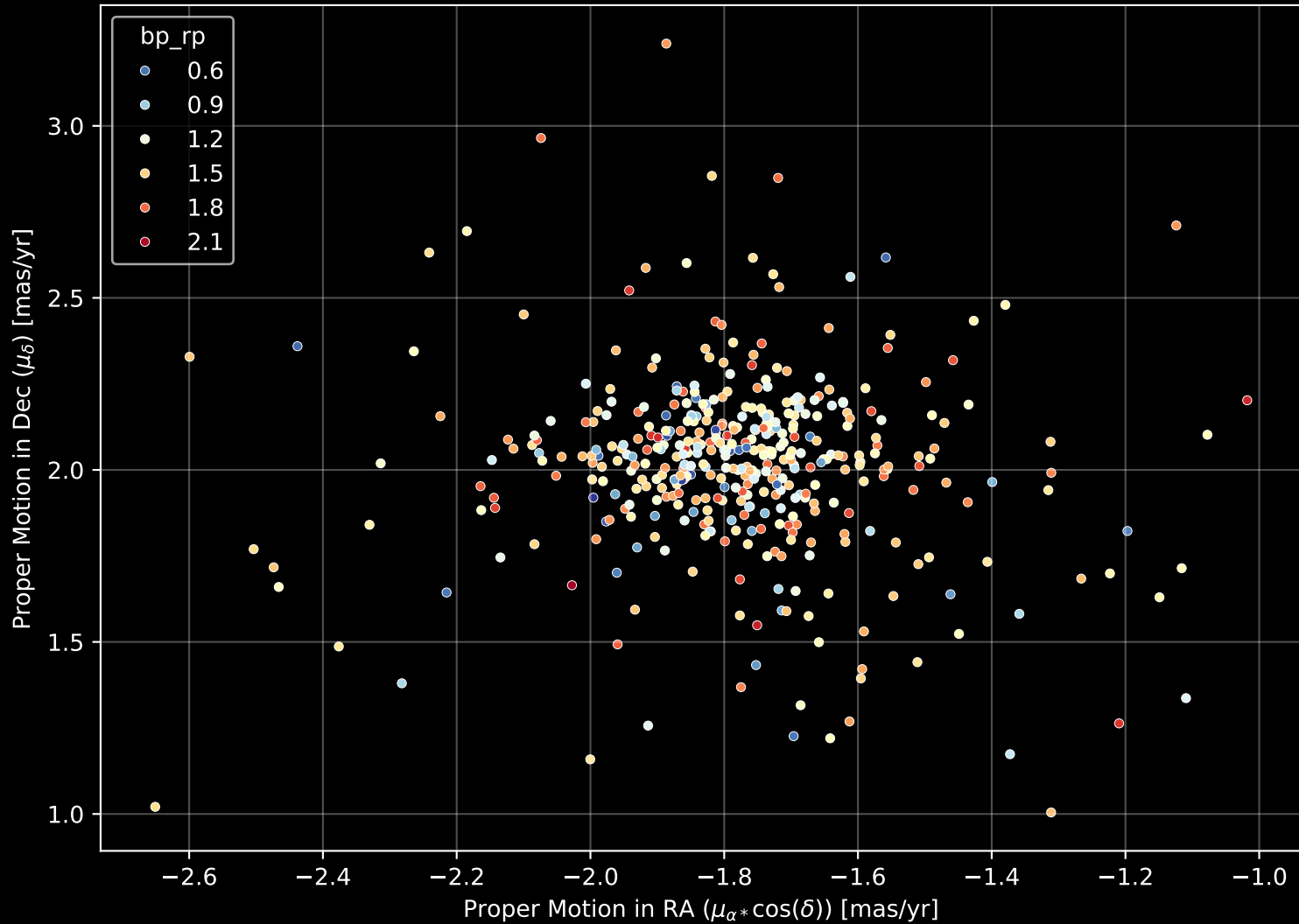
Gaia Cluster: [NGC_1027] Proper Motion Diagram (n= 417)
