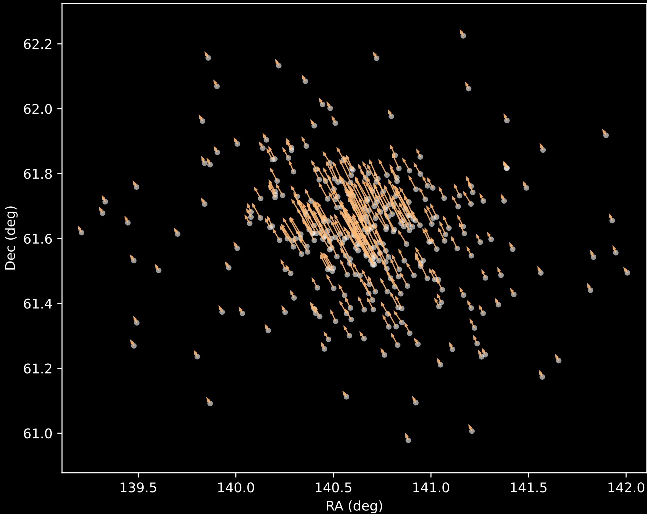
Gaia DR3 Cluster 3 Proper Motion Vectors (n=325)
