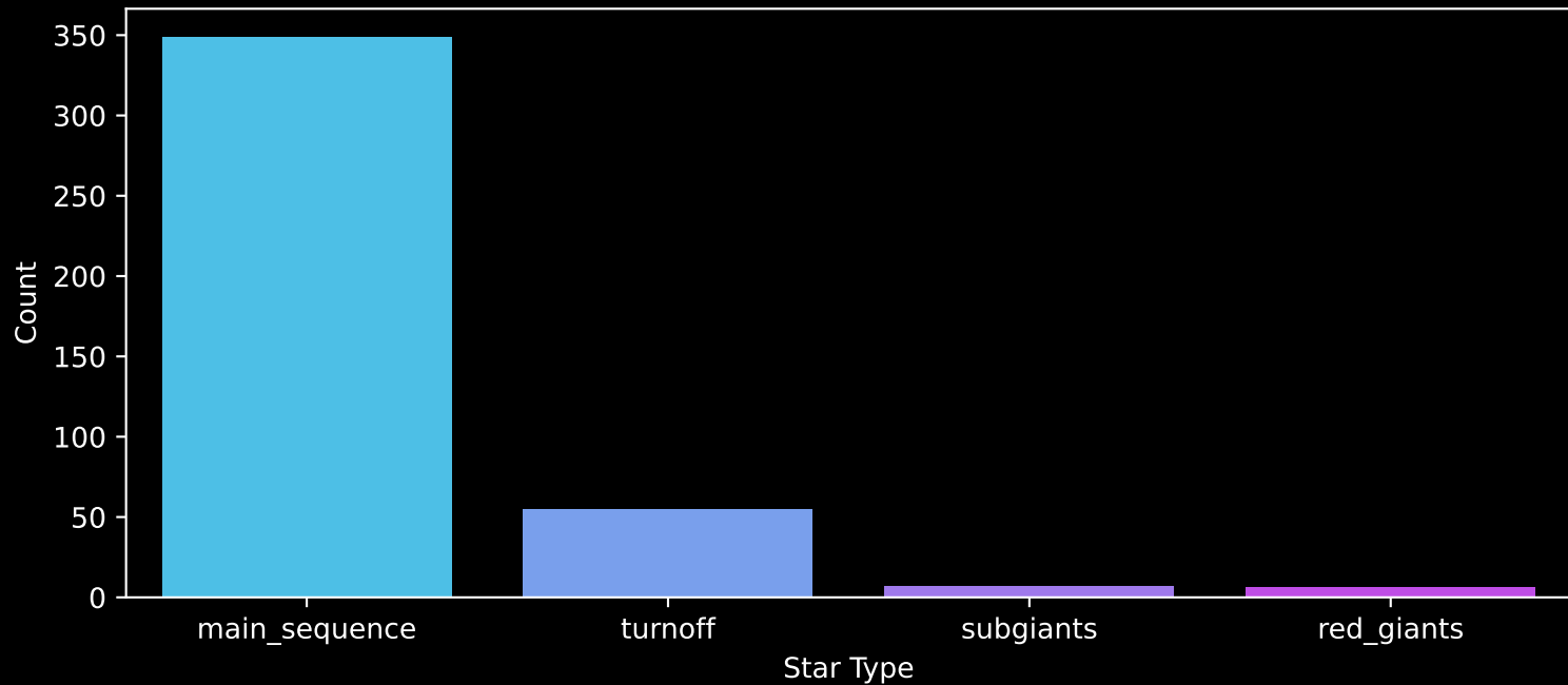
Gaia Cluster: [NGC_1027] Count plot of Star Type
