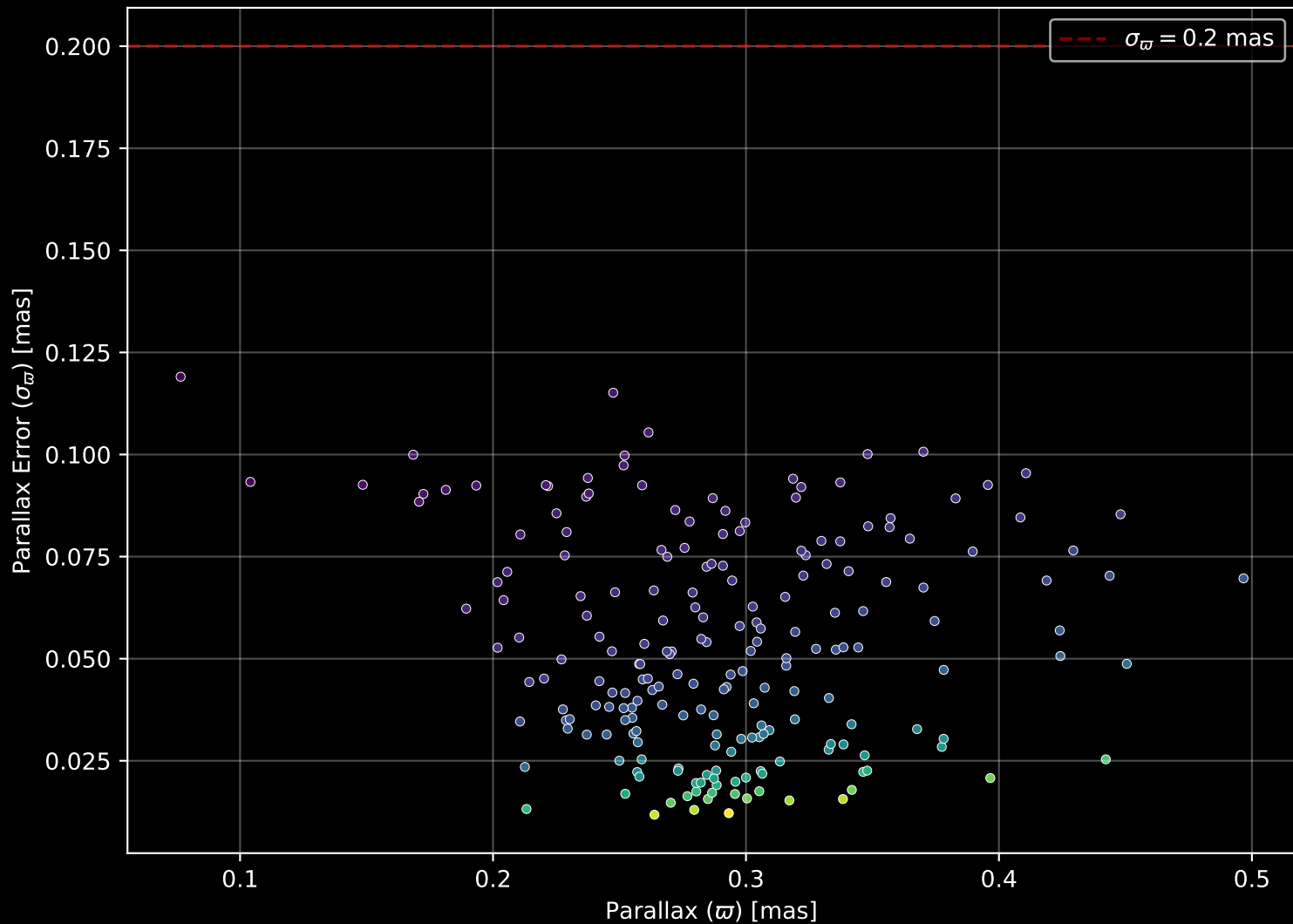
Gaia Cluster: [NGC_103] Parallax Quality (n= 207)
