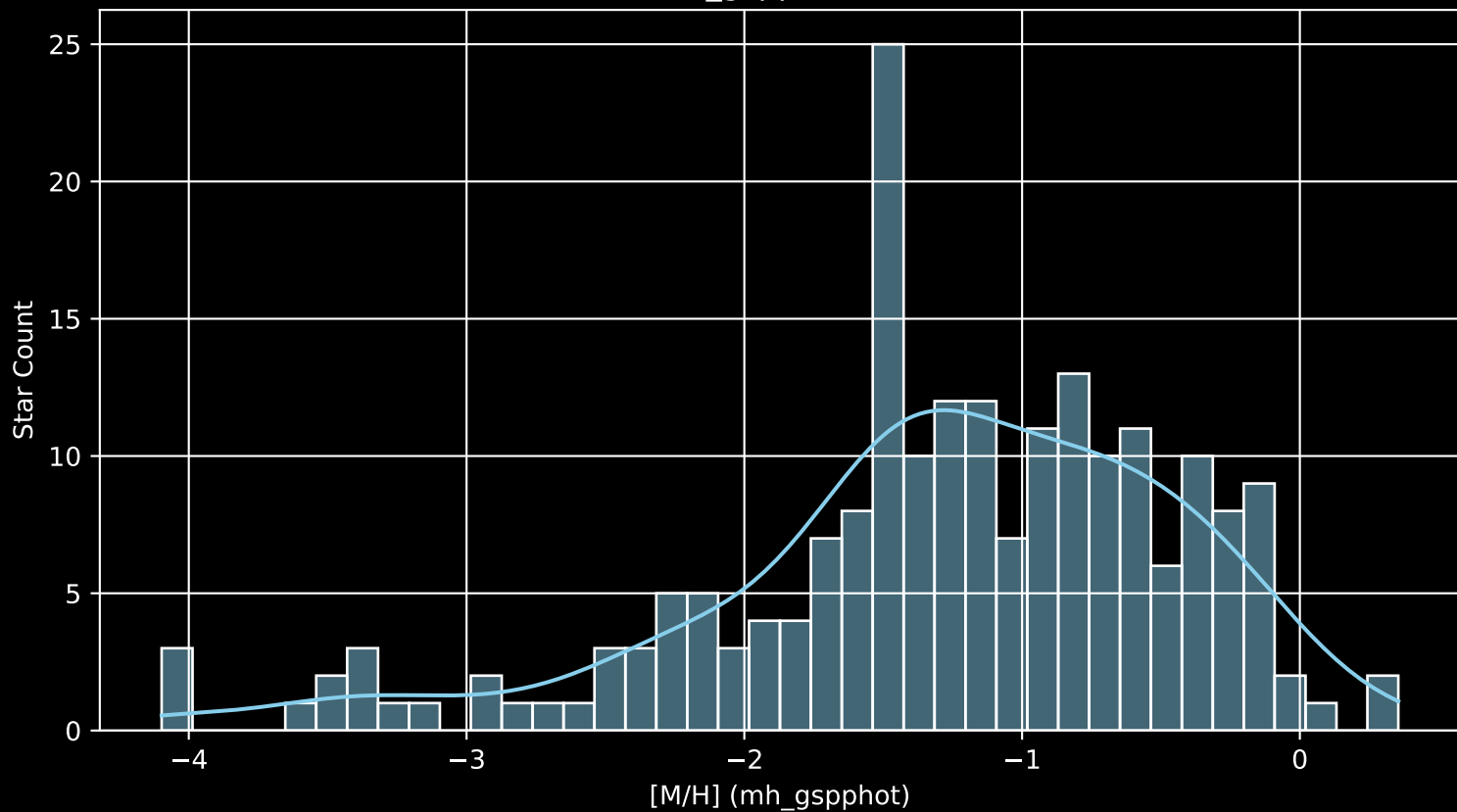
Gaia Cluster: [NGC_103 [M/H] (mh_gspphot) (n= 207)
