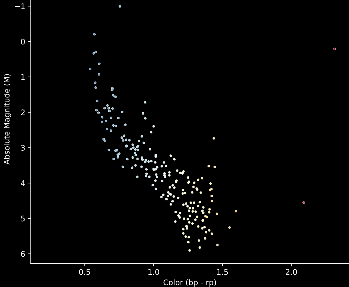
Gaia Cluster: [NGC_103] Stars (n= 207) Hertzsprung-Russel Diagram
