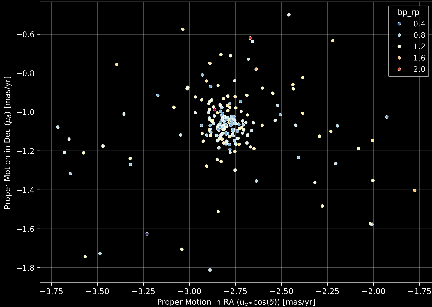
Gaia Cluster: [NGC_103] Proper Motion Diagram (n= 207)
