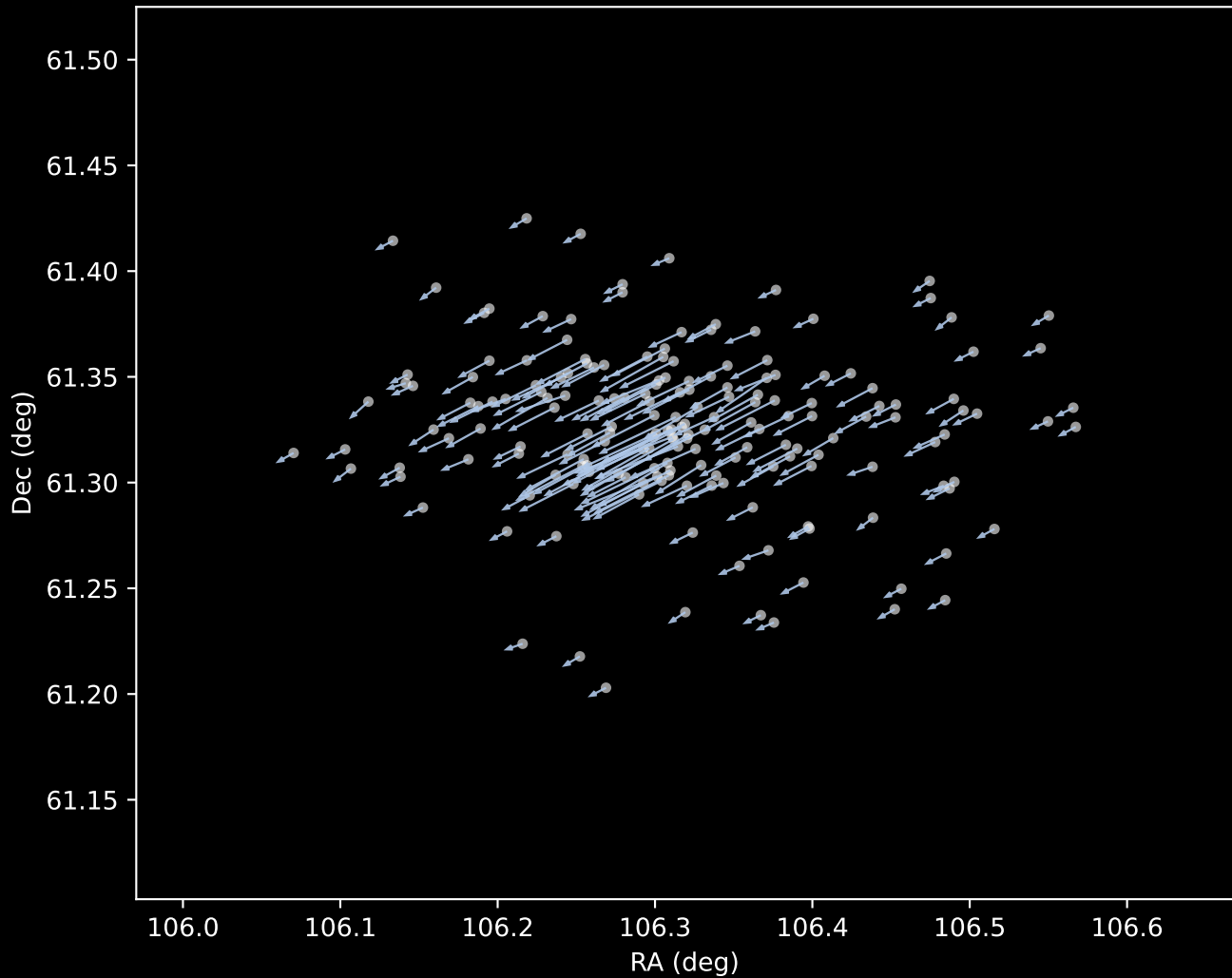
Gaia DR3 Cluster 1 Proper Motion Vectors (n=183)
