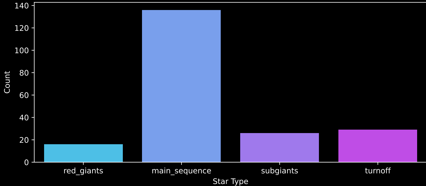
Gaia Cluster: [NGC_103] Count plot of Star Type
