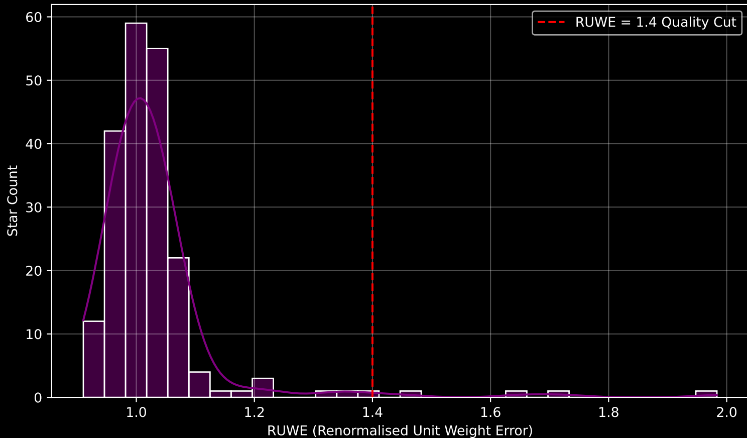
Gaia Cluster: [NGC_103] RUWE Distribution (n= 206)
