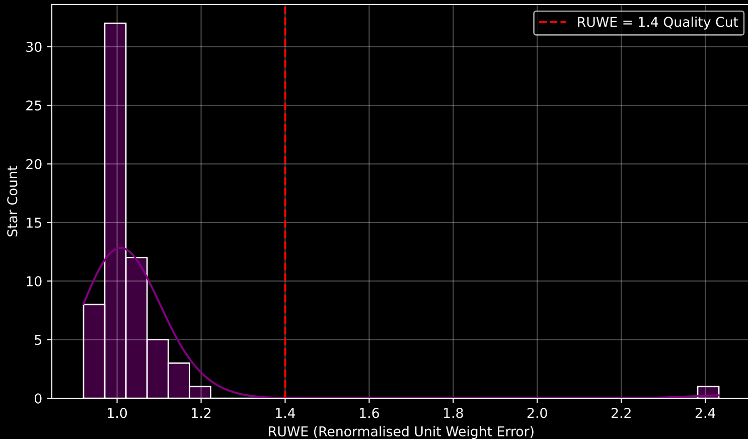
Gaia Cluster: [NGC_1220] RUWE Distribution (n= 62)
