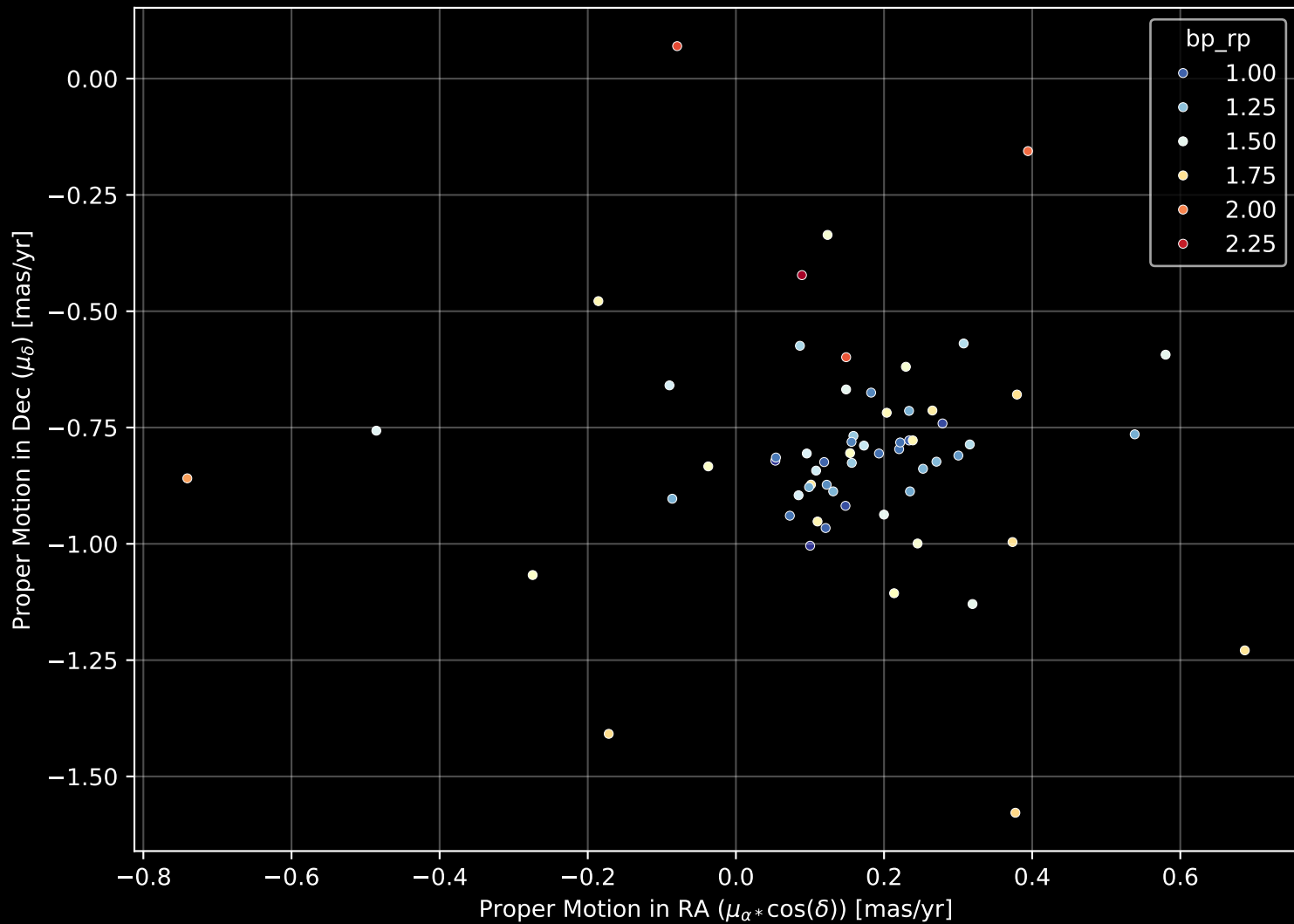
Gaia Cluster: [NGC_1220] Proper Motion Diagram (n= 62)
