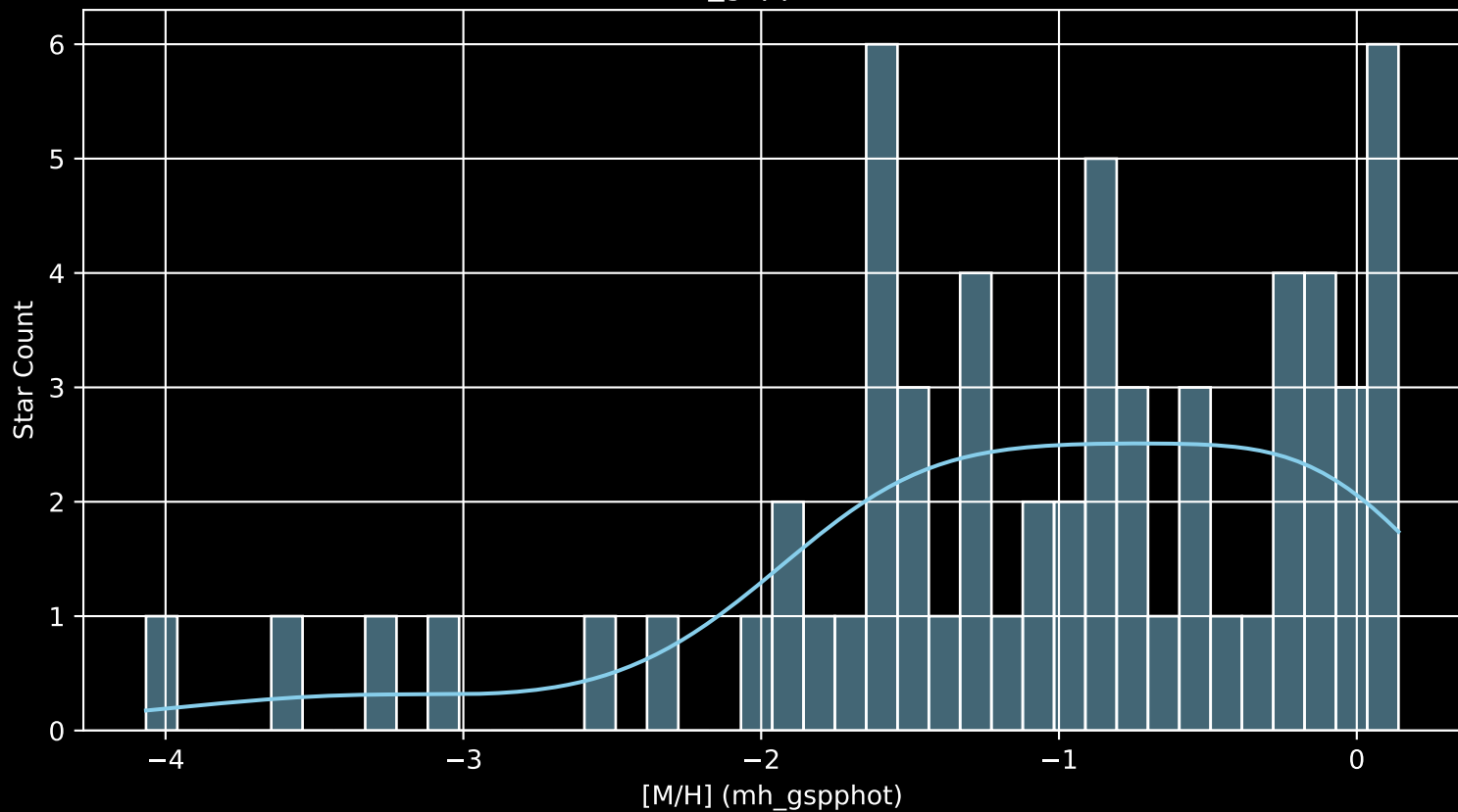
Gaia Cluster: [NGC_1220 [M/H] (mh_gspphot) (n= 61)
