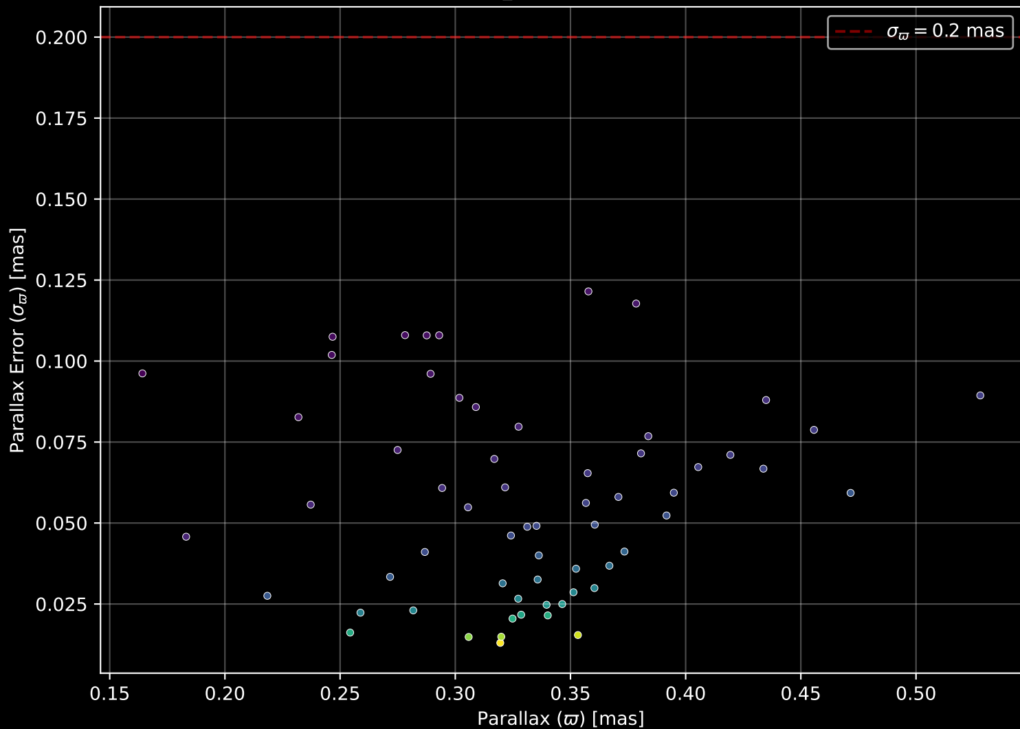
Gaia Cluster: [NGC_1220] Parallax Quality (n= 62)
