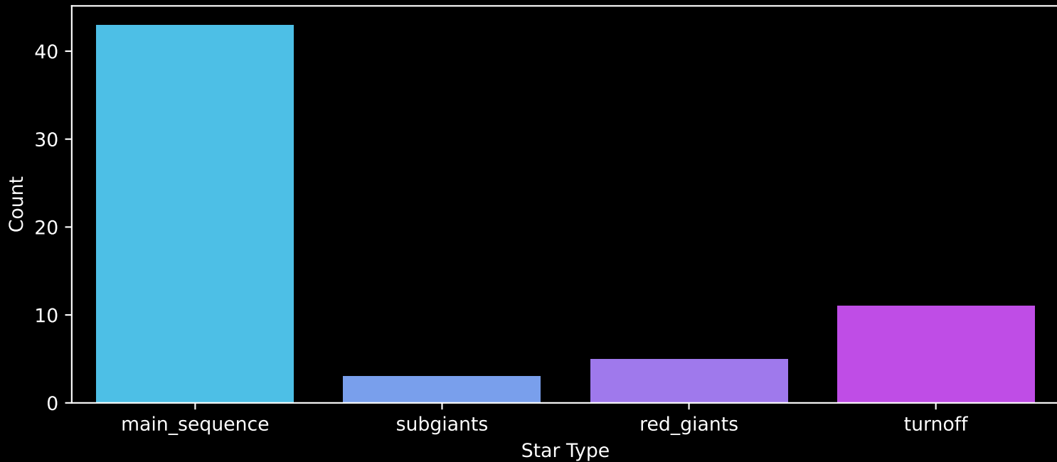
Gaia Cluster: [NGC_1220] Count plot of Star Type
