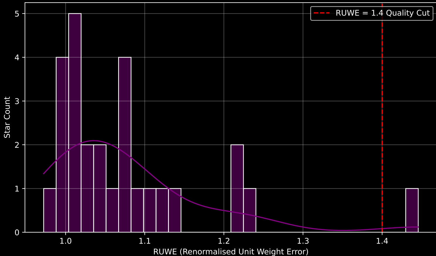
Gaia Cluster: [NGC_1333] RUWE Distribution (n= 27)
