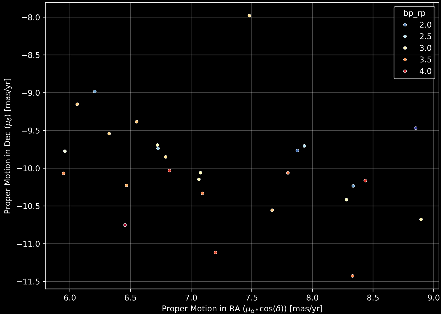
Gaia Cluster: [NGC_1333] Proper Motion Diagram (n= 27)
