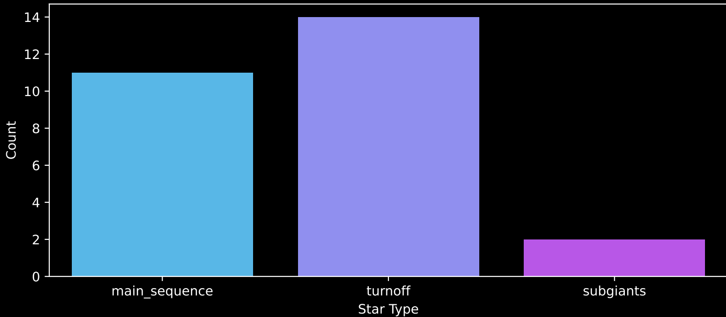
Gaia Cluster: [NGC_1333] Count plot of Star Type
