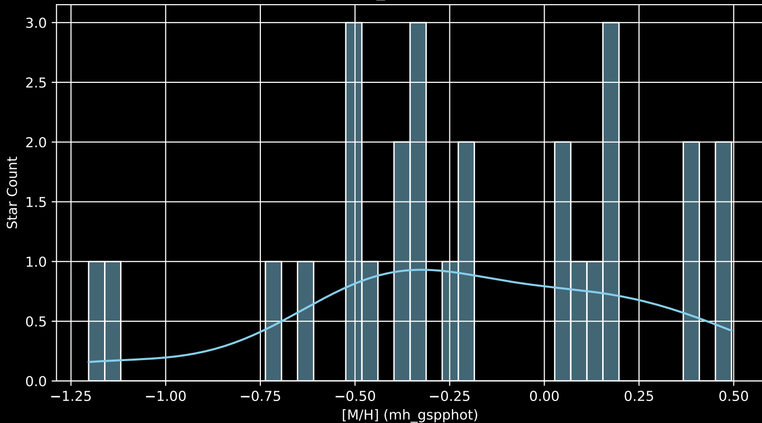
Gaia Cluster: [NGC_1333 [M/H] (mh_gspphot) (n= 27)
