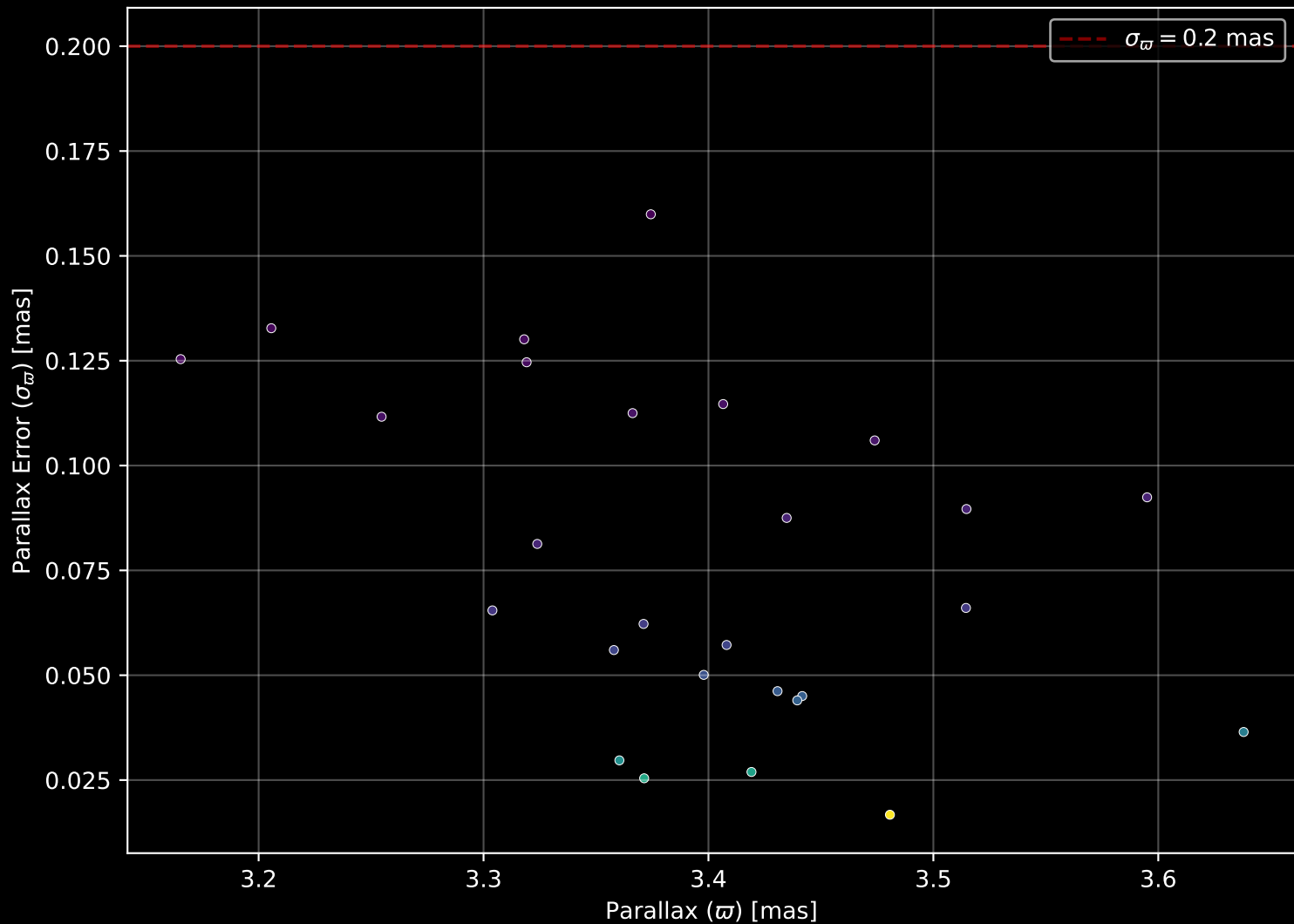
Gaia Cluster: [NGC_1333] Parallax Quality (n= 27)
