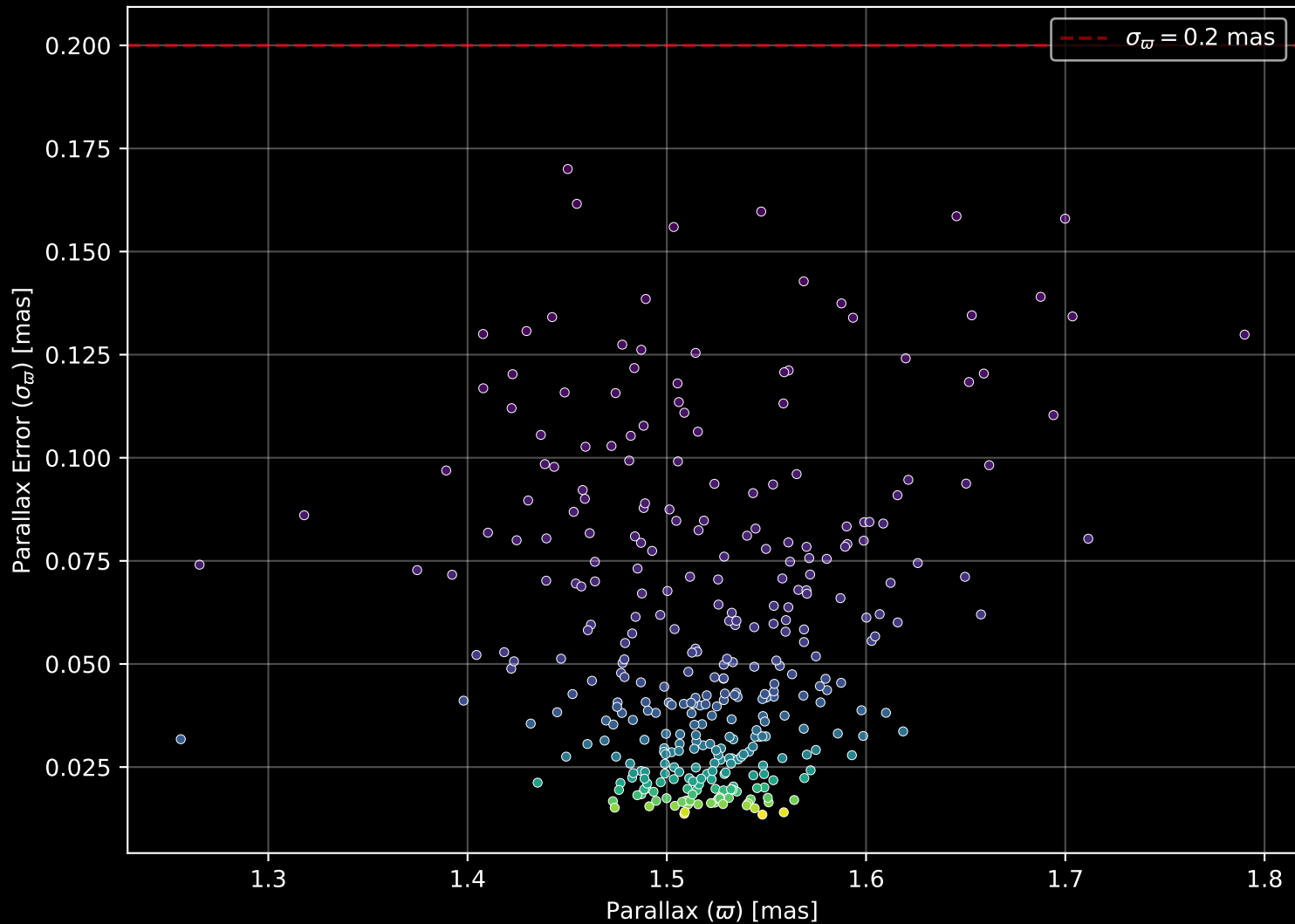
Gaia Cluster: [NGC_1342] Parallax Quality (n= 339)
