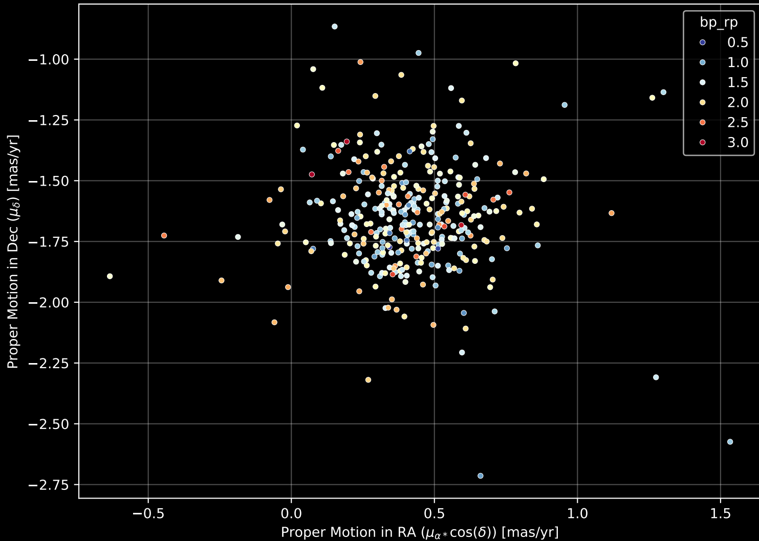
Gaia Cluster: [NGC_1342] Proper Motion Diagram (n= 339)
