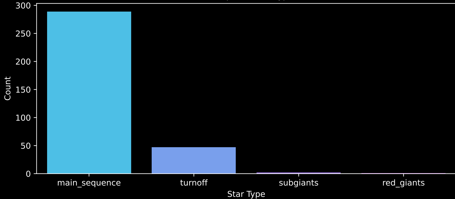
Gaia Cluster: [NGC_1342] Count plot of Star Type
