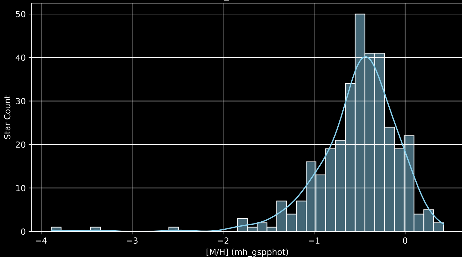
Gaia Cluster: [NGC_1342 [M/H] (mh_gspphot) (n= 339)
