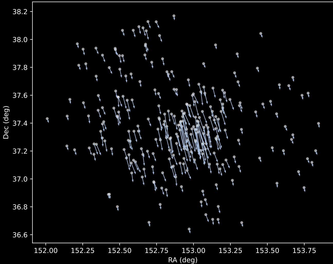
Gaia DR3 Cluster 1 Proper Motion Vectors (n=258)
