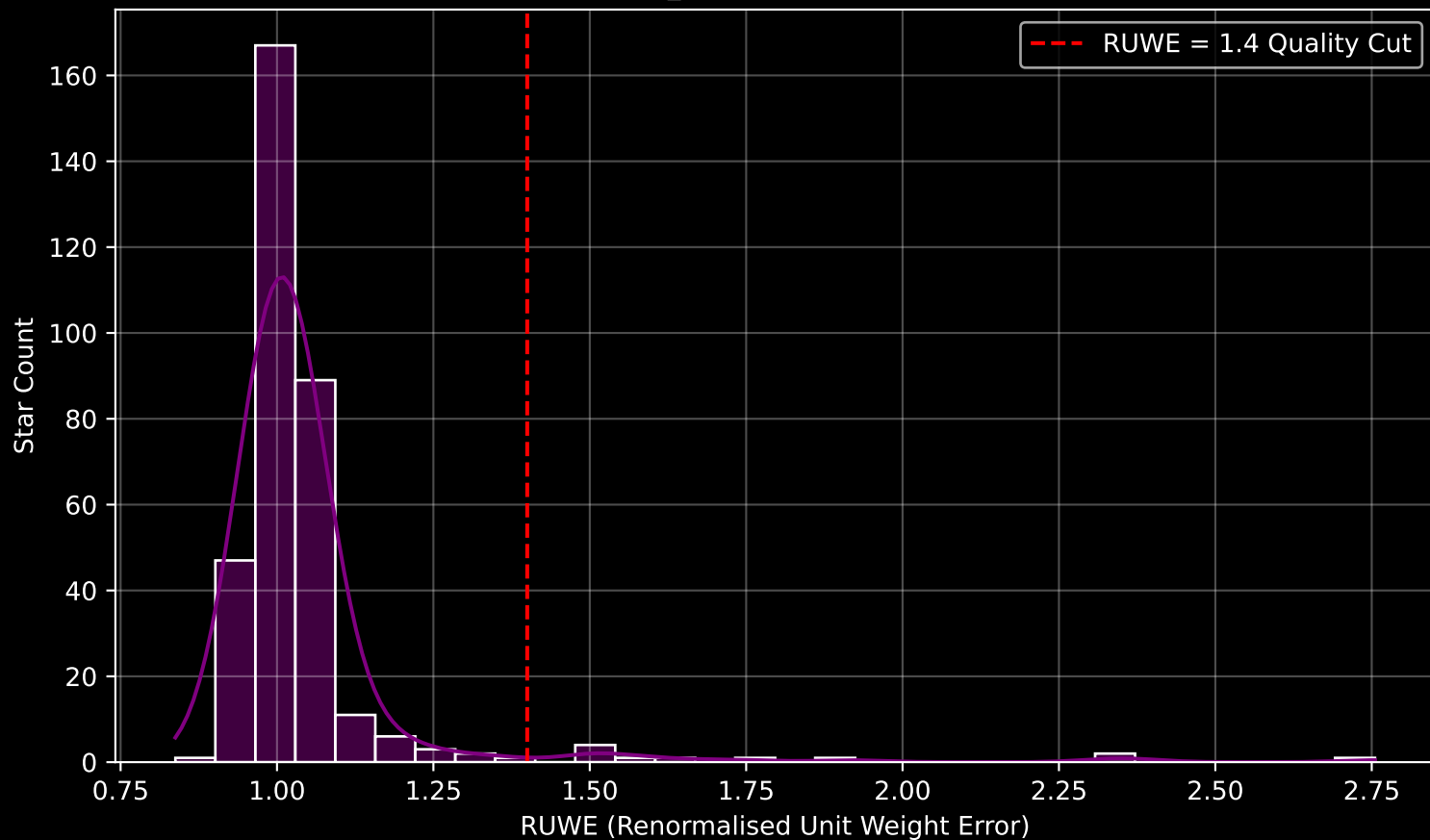
Gaia Cluster: [NGC_1342] RUWE Distribution (n= 338)
