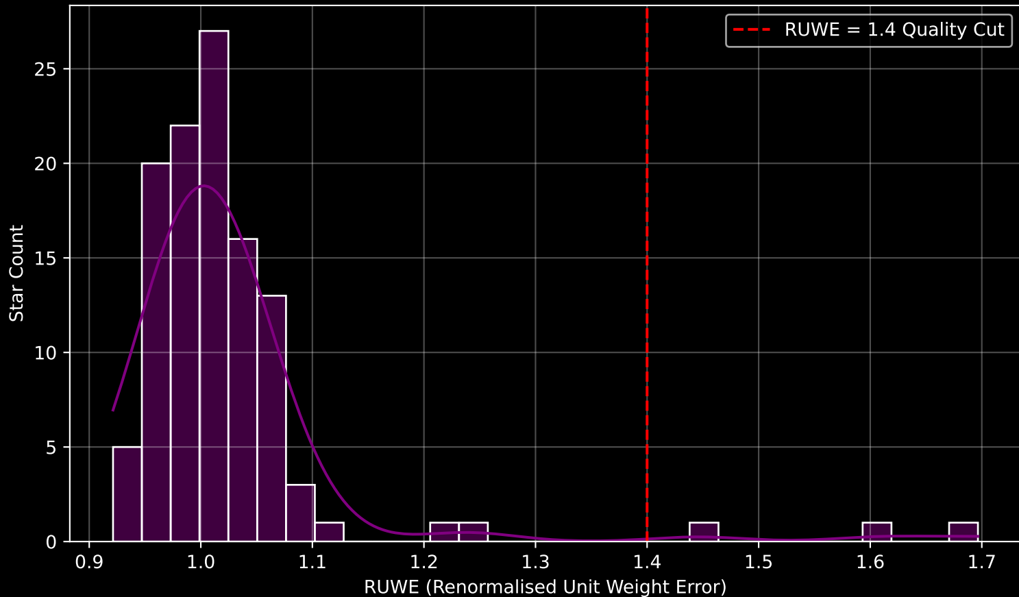
Gaia Cluster: [NGC_136] RUWE Distribution (n= 112)
