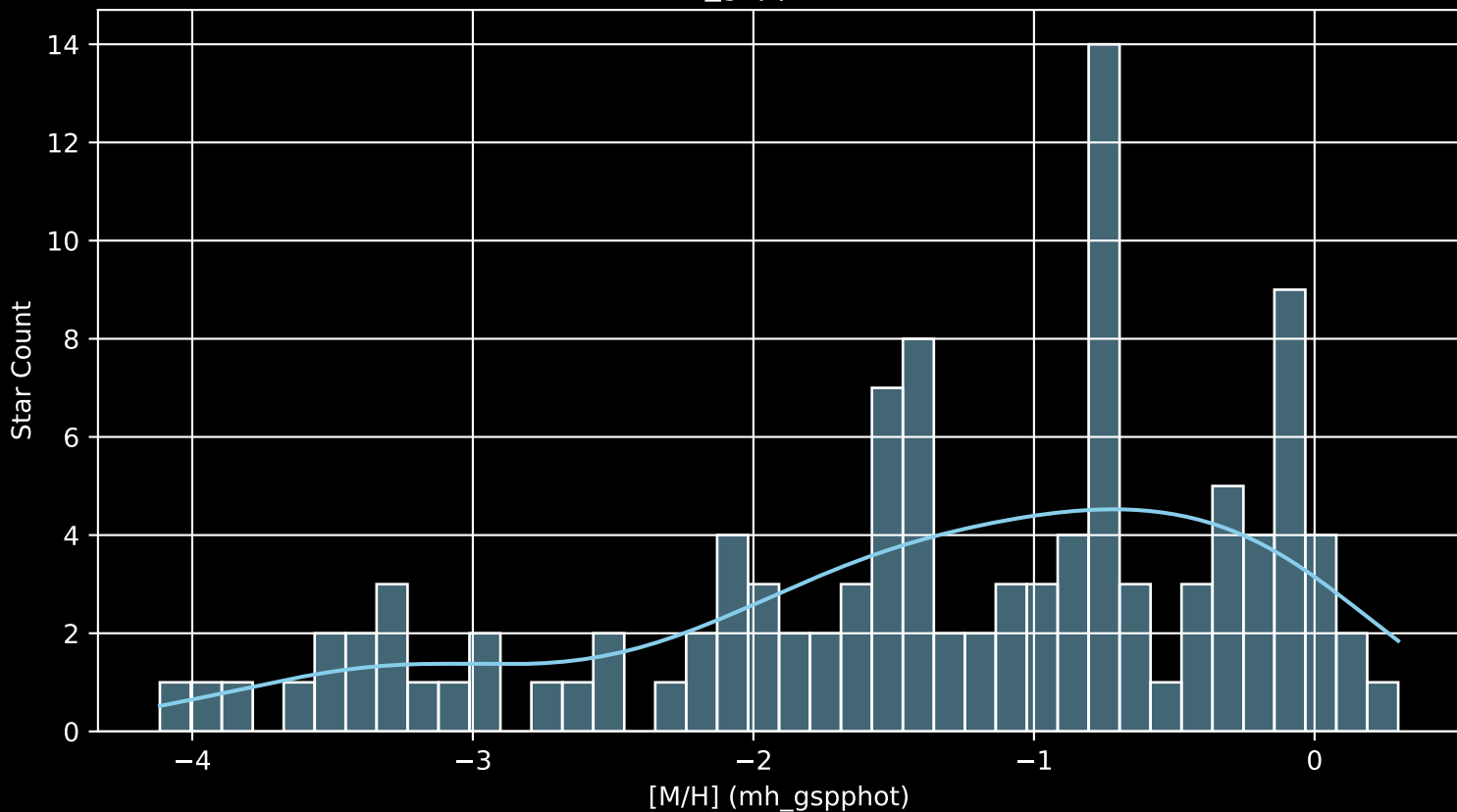
Gaia Cluster: [NGC_136 [M/H] (mh_gspphot) (n= 111)
