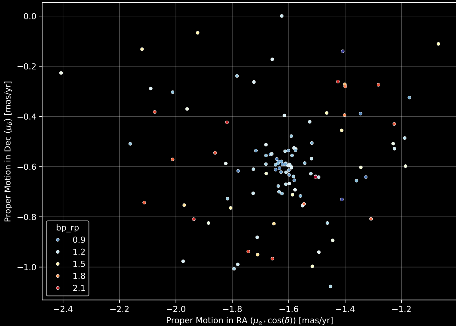
Gaia Cluster: [NGC_136] Proper Motion Diagram (n= 112)
