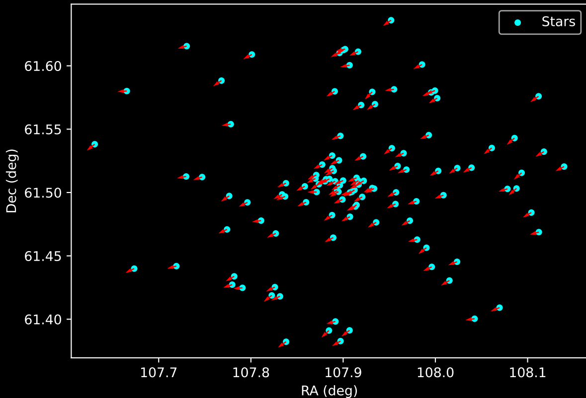
Gaia Cluster: [NGC_136] Proper Motion Vectors for Gaia Star Field (n= 112)
