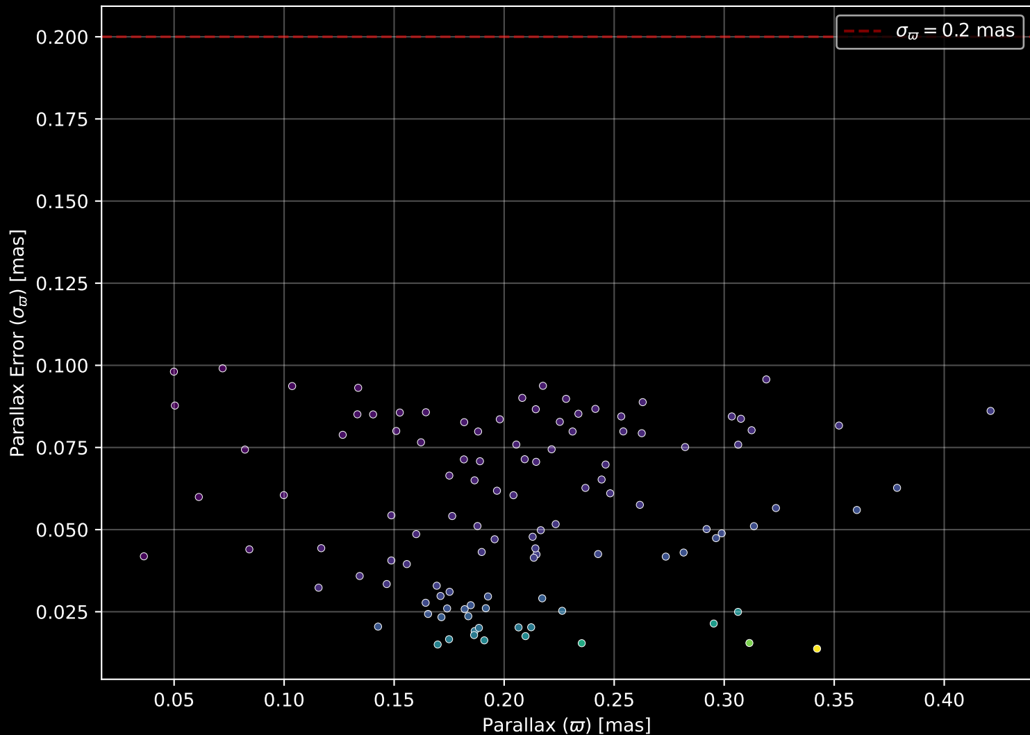
Gaia Cluster: [NGC_136] Parallax Quality (n= 112)
