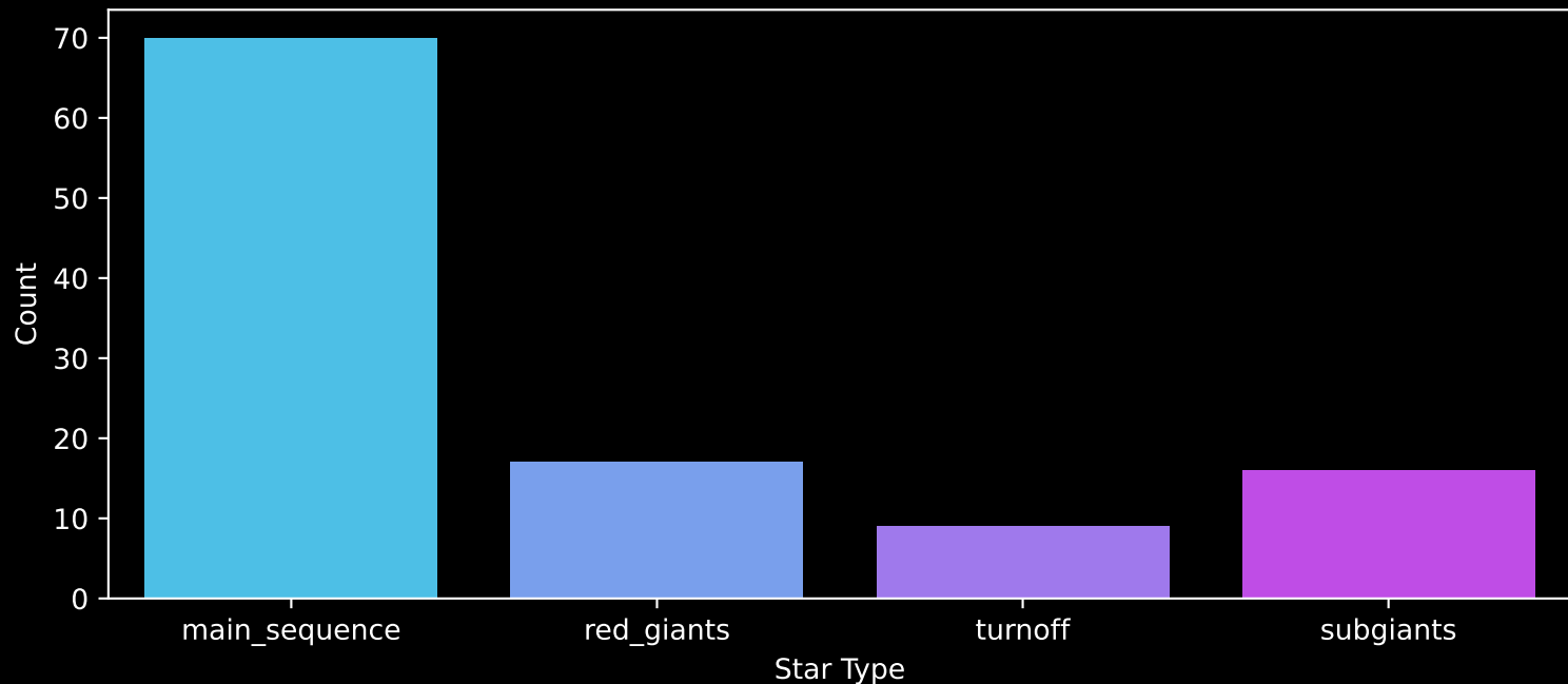
Gaia Cluster: [NGC_136] Count plot of Star Type
