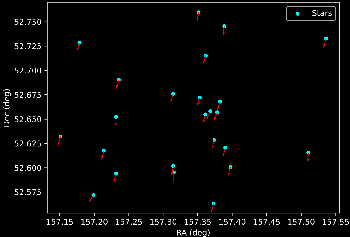
Gaia Cluster: [NGC_1444] Proper Motion Vectors for Gaia Star Field (n= 24)
