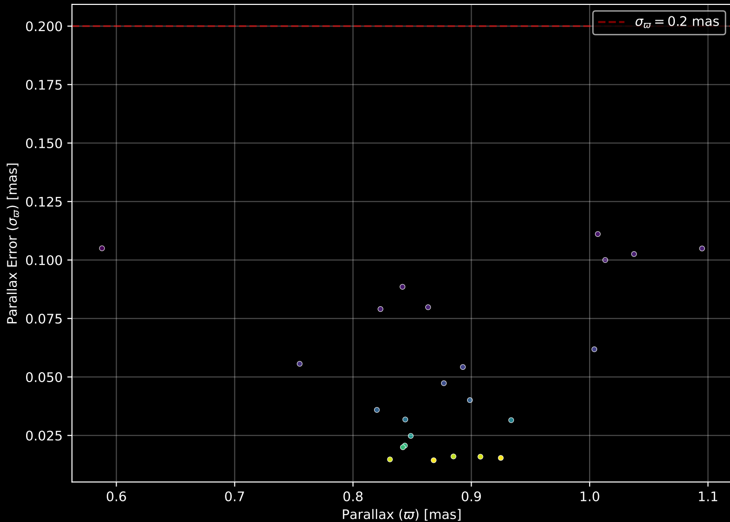
Gaia Cluster: [NGC_1444] Parallax Quality (n= 24)
