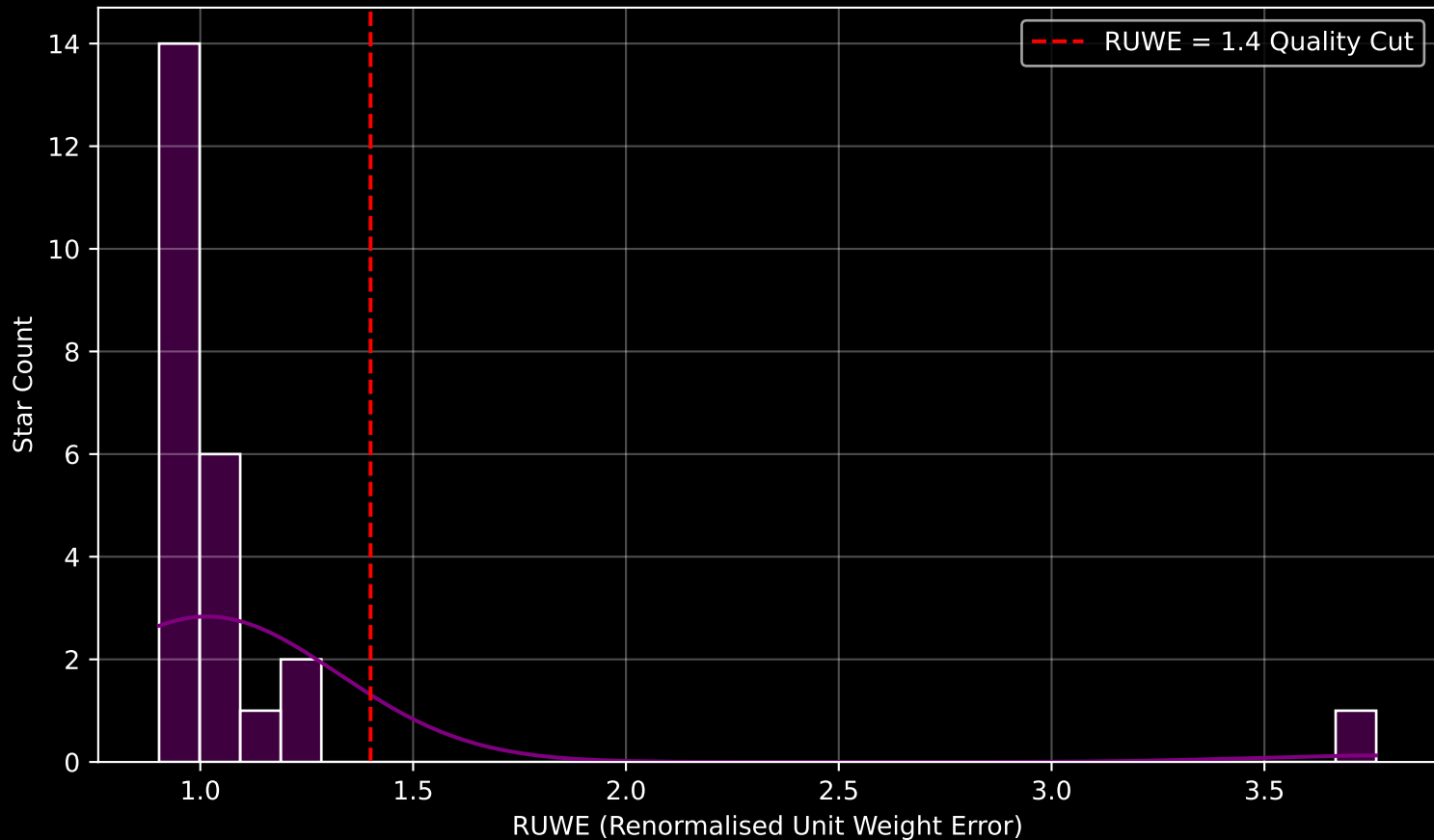
Gaia Cluster: [NGC_1444] RUWE Distribution (n= 24)
