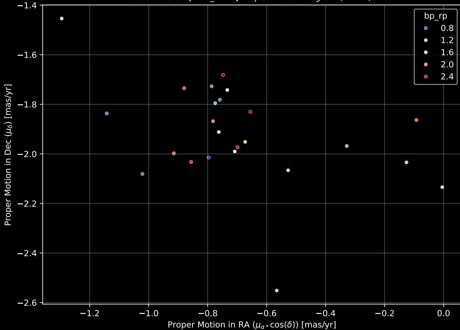
Gaia Cluster: [NGC_1444] Proper Motion Diagram (n= 24)
