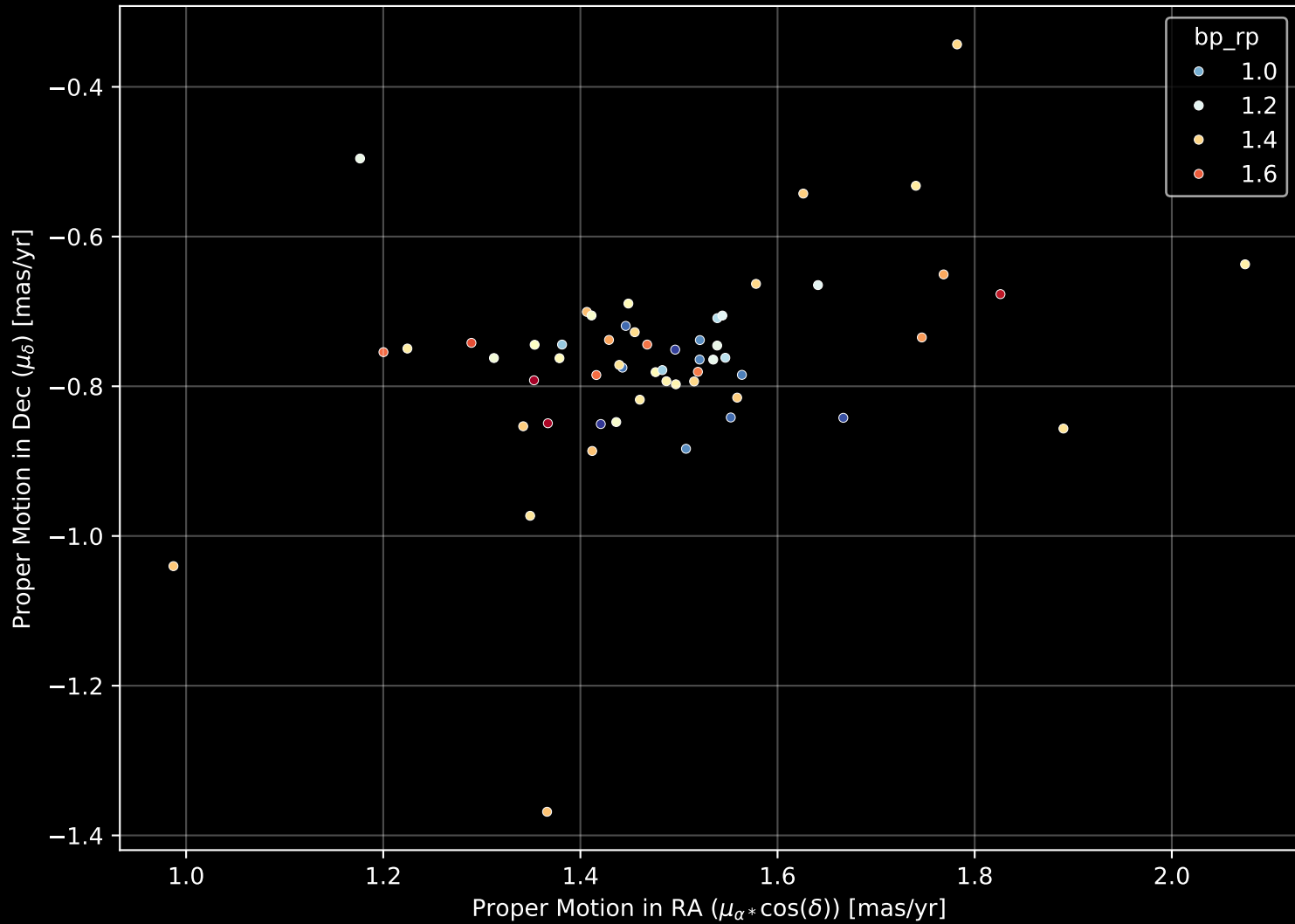
Gaia Cluster: [NGC_1496] Proper Motion Diagram (n= 57)
