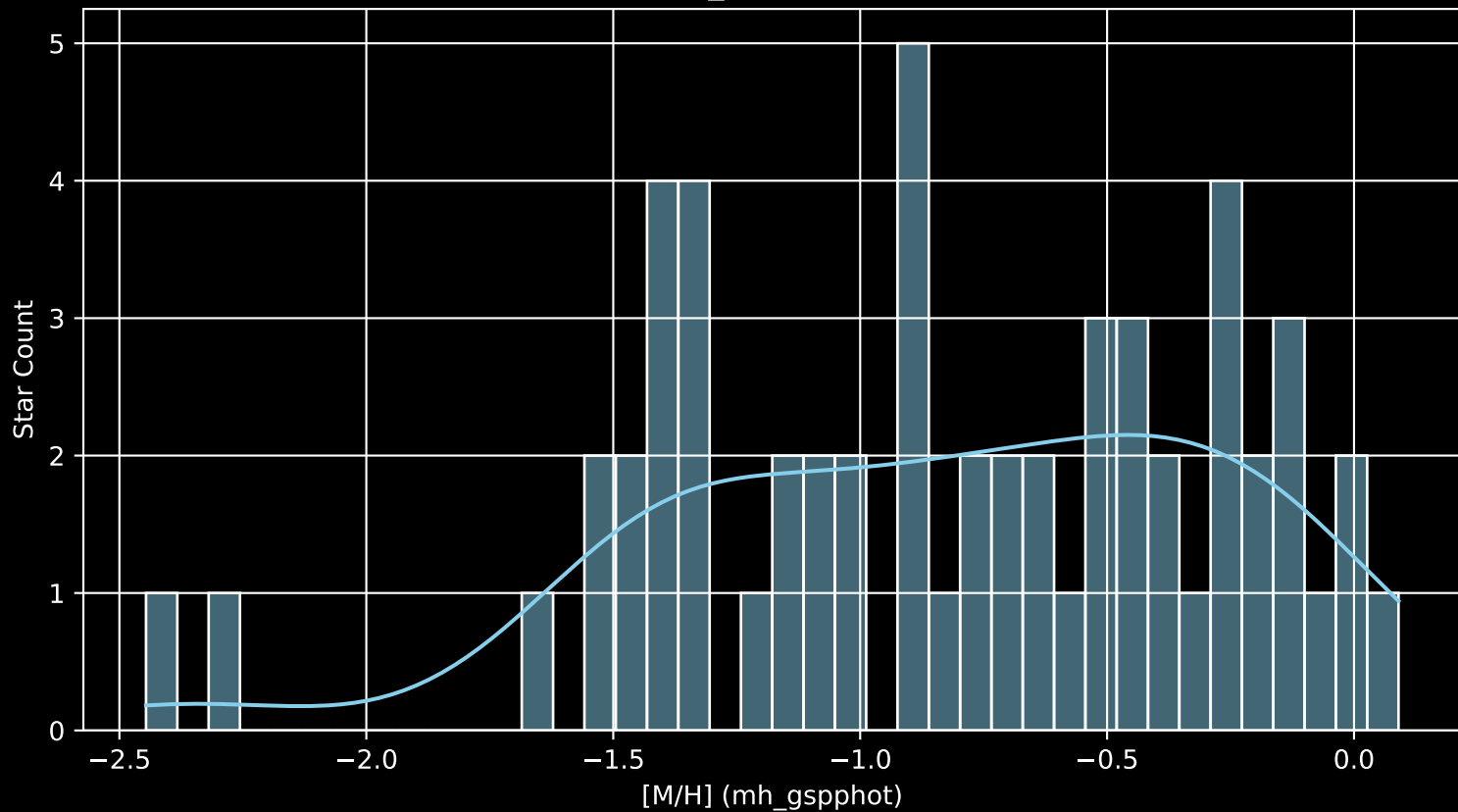
Gaia Cluster: [NGC_1496 [M/H] (mh_gspphot) (n= 57)
