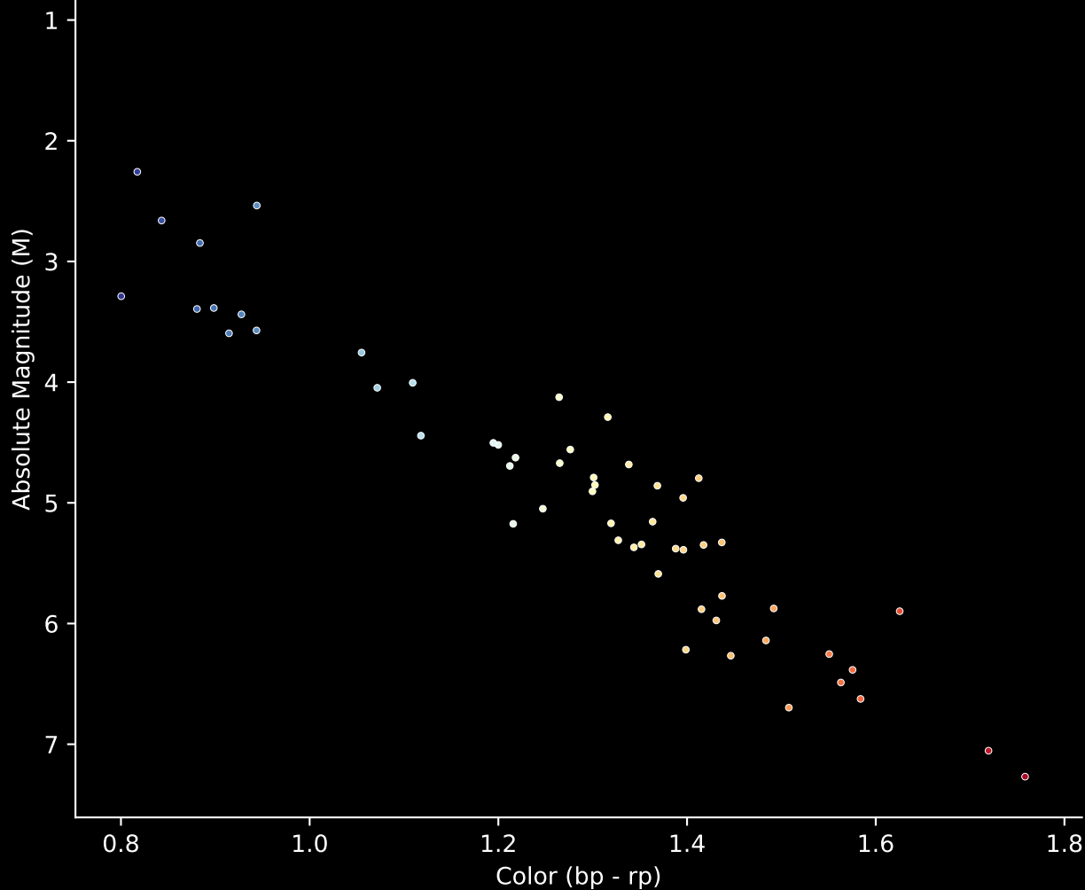
Gaia Cluster: [NGC_1496] Stars (n= 57) Hertzsprung-Russel Diagram
