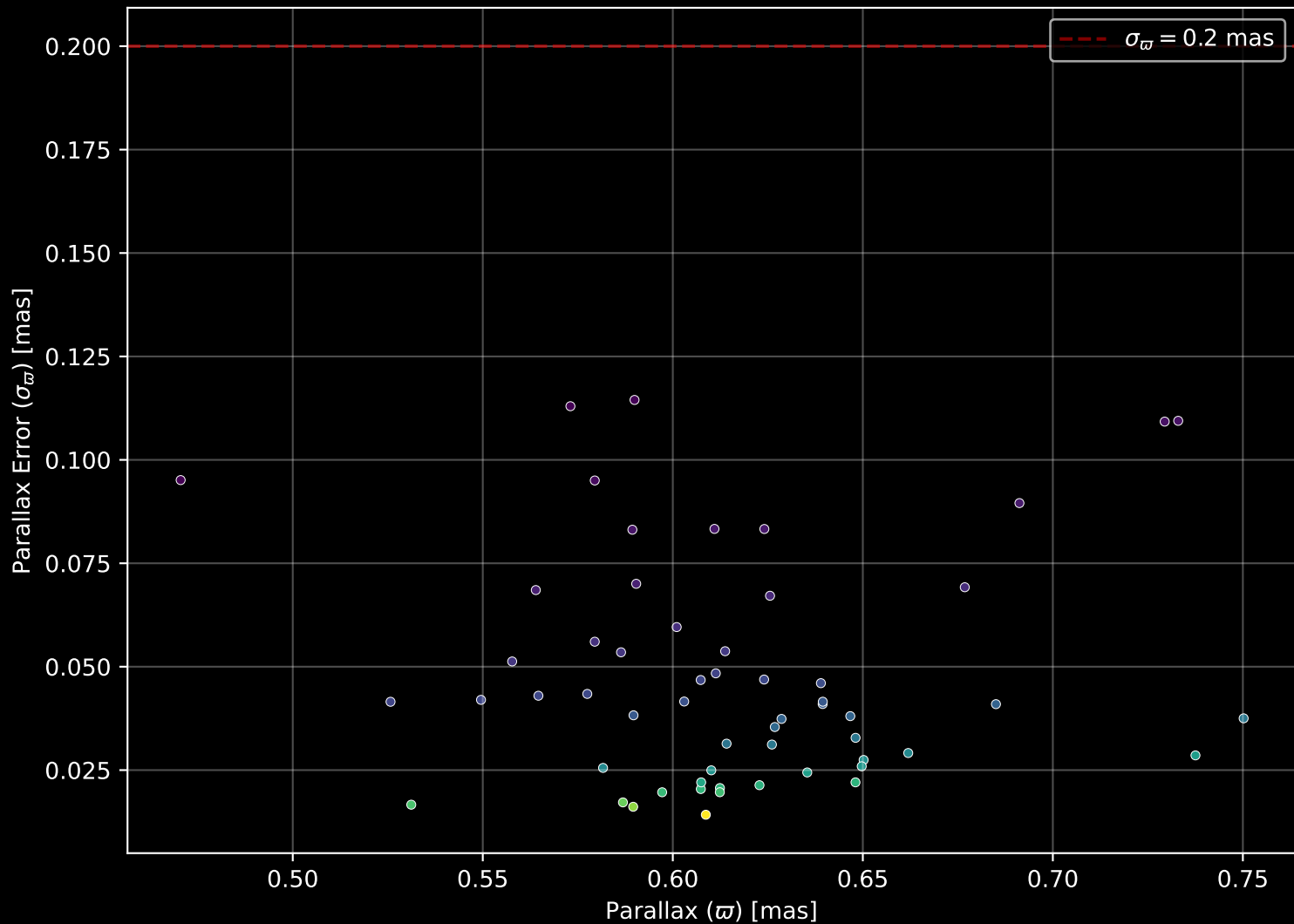
Gaia Cluster: [NGC 1496] Parallax Quality (n= 57)
