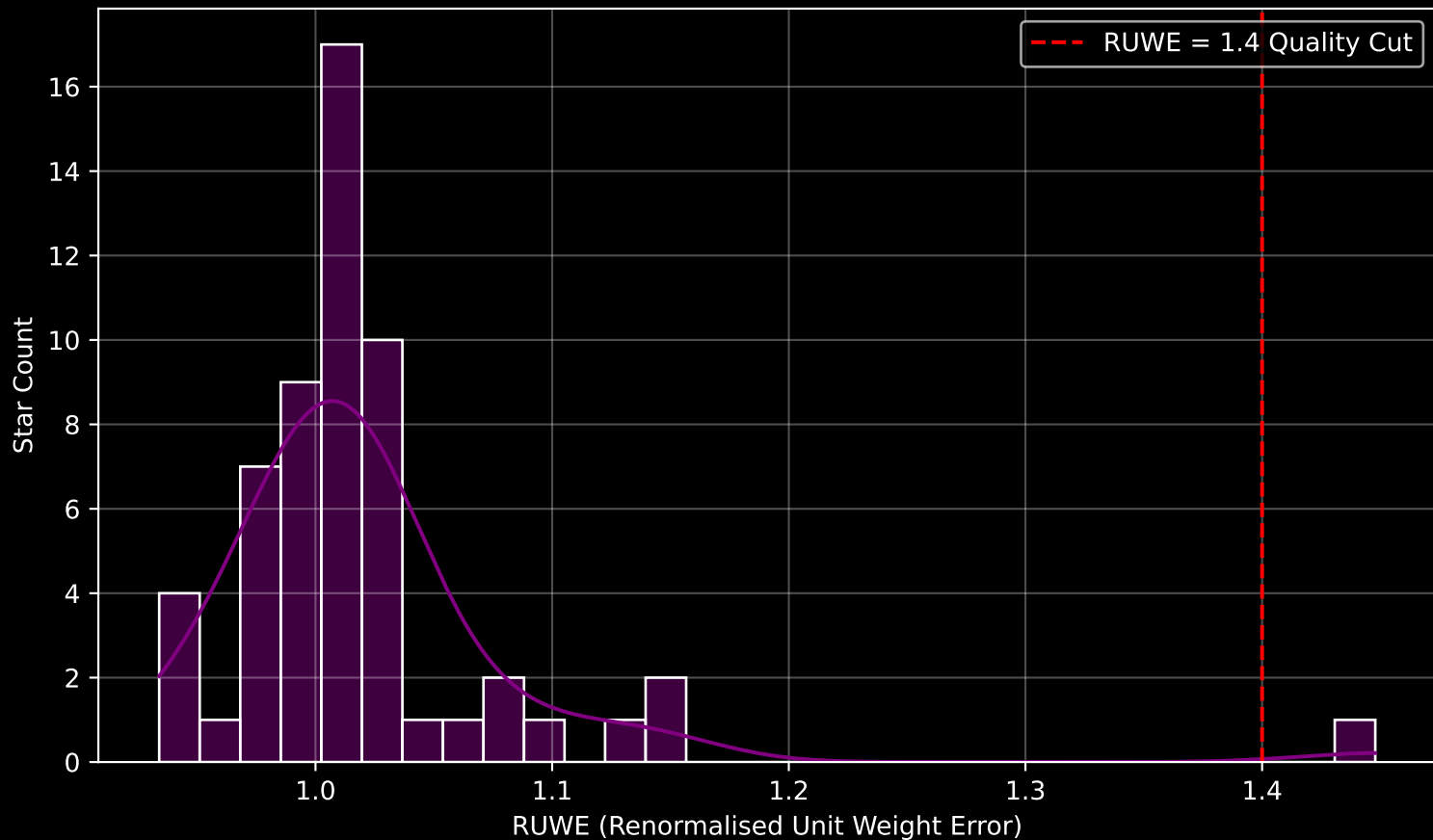
Gaia Cluster: [NGC_1496] RUWE Distribution (n= 57)
