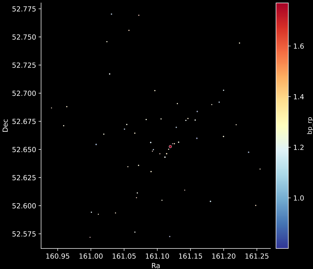
Gaia Cluster: [NGC_1496] Stars: 57
