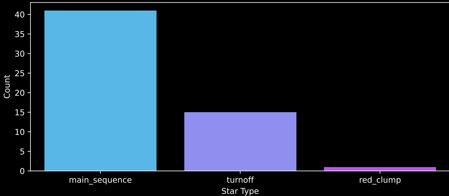
Gaia Cluster: [NGC_1496] Count plot of Star Type
