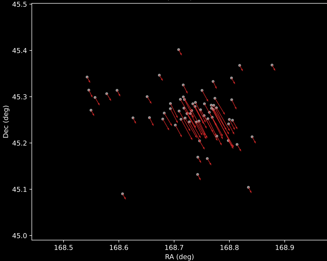
Gaia DR3 Cluster 6 Proper Motion Vectors (n=64)
