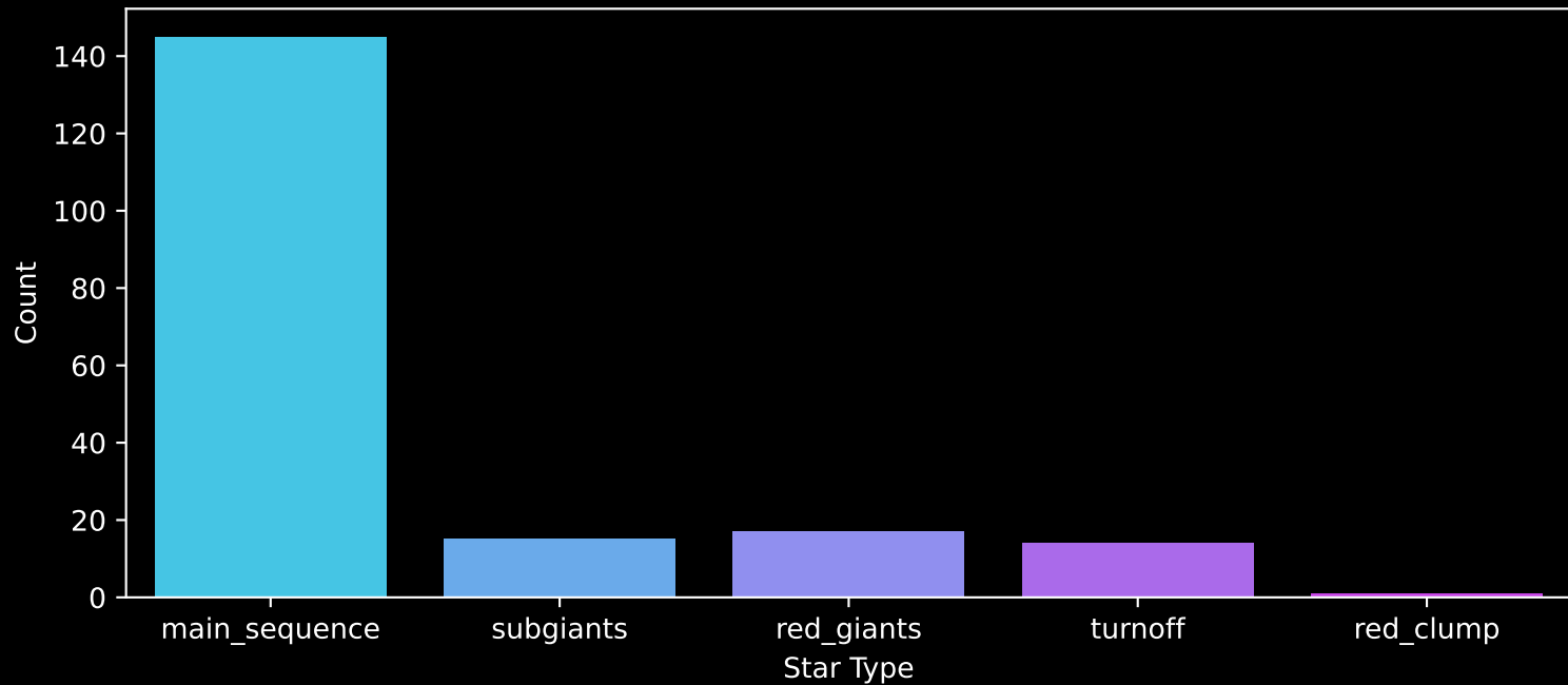
Gaia Cluster: [NGC_1605] Count plot of Star Type
