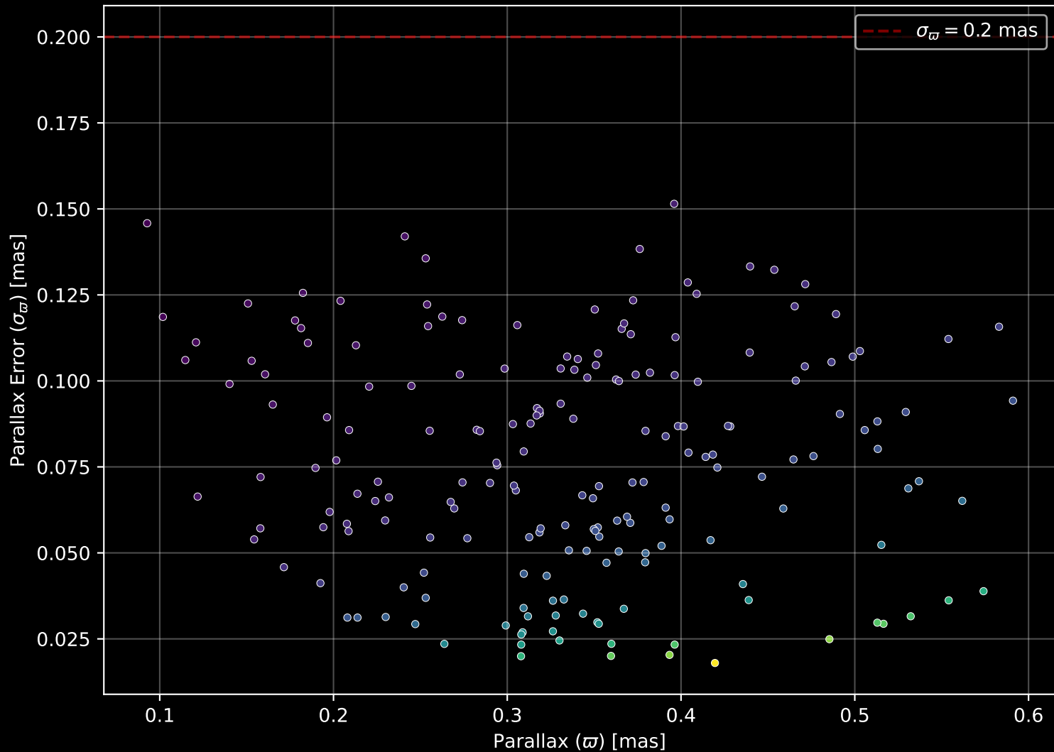
Gaia Cluster: [NGC_1605] Parallax Quality (n= 192)
