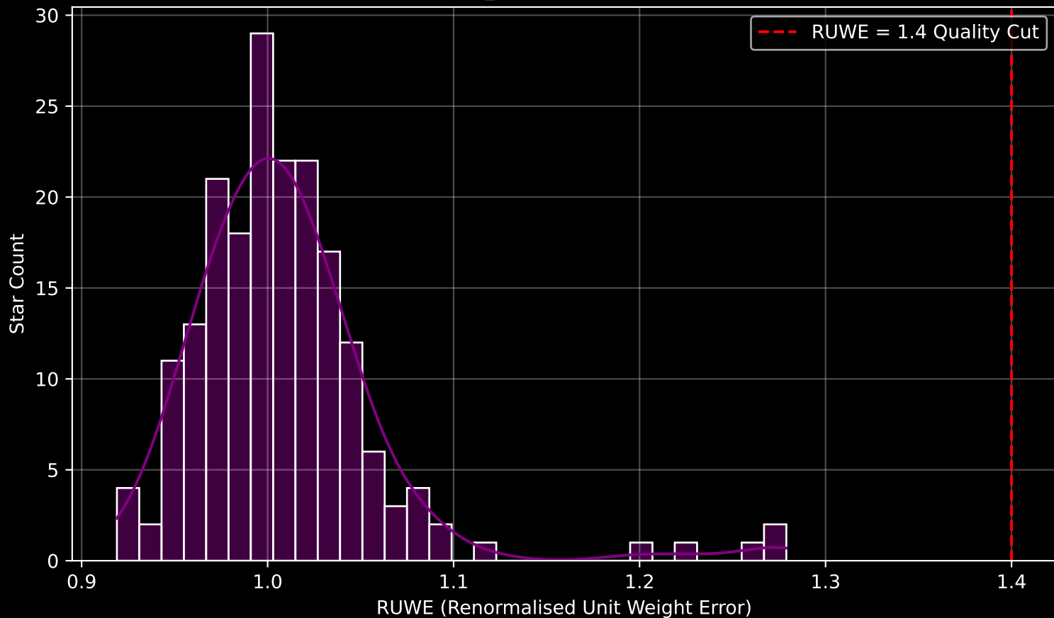
Gaia Cluster: [NGC_1605] RUWE Distribution (n= 192)
