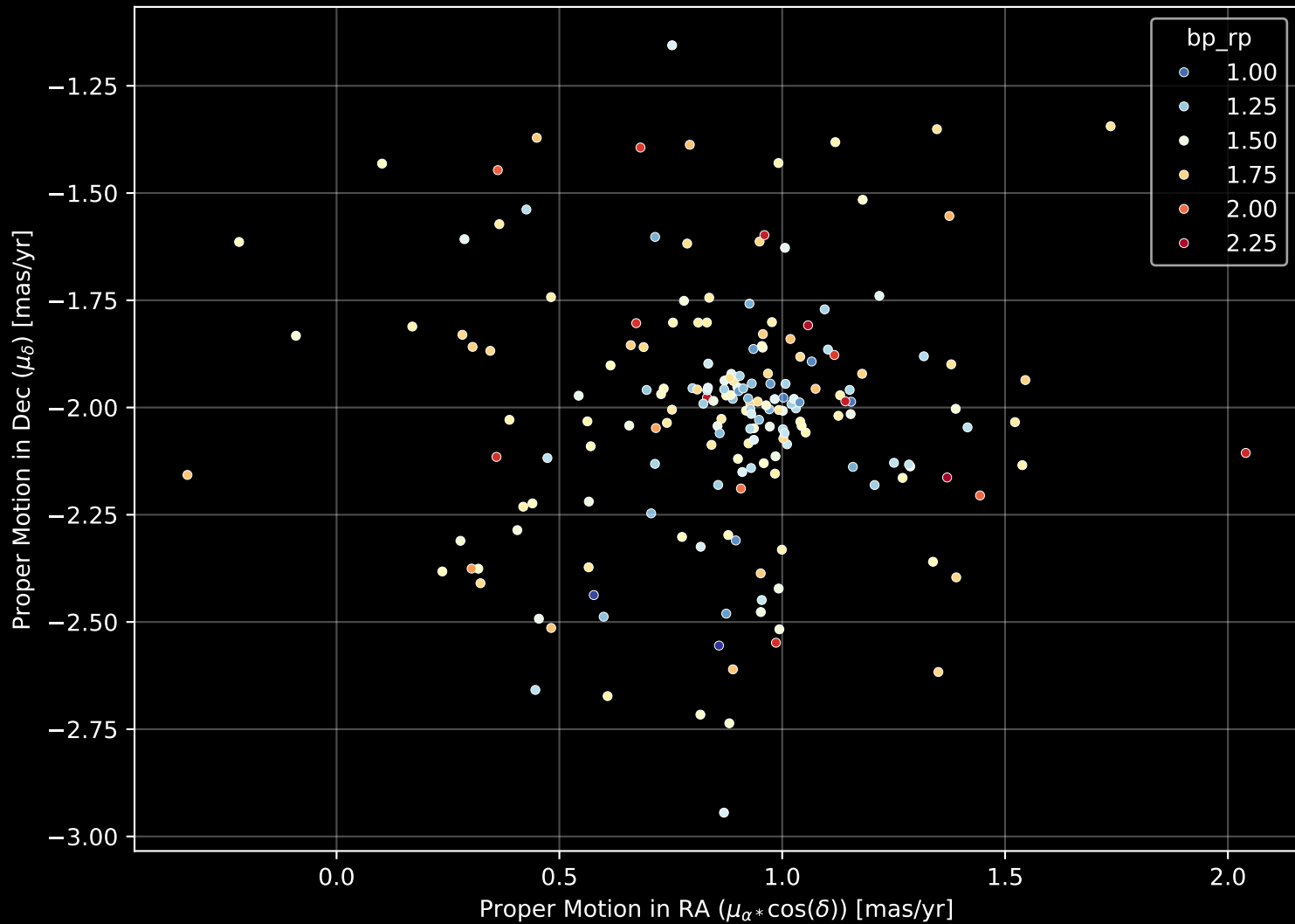
Gaia Cluster: [NGC_1605] Proper Motion Diagram (n= 192)
