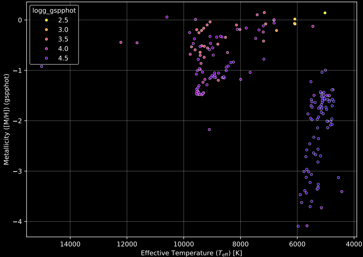
Gaia Cluster: [NGC_1605] Stellar Population Parameters (n= 192)
