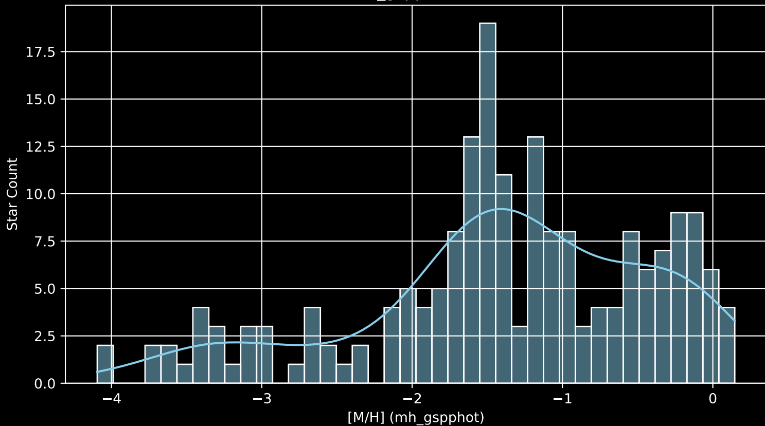
Gaia Cluster: [NGC_1605 [M/H] (mh_gspphot) (n= 192)
