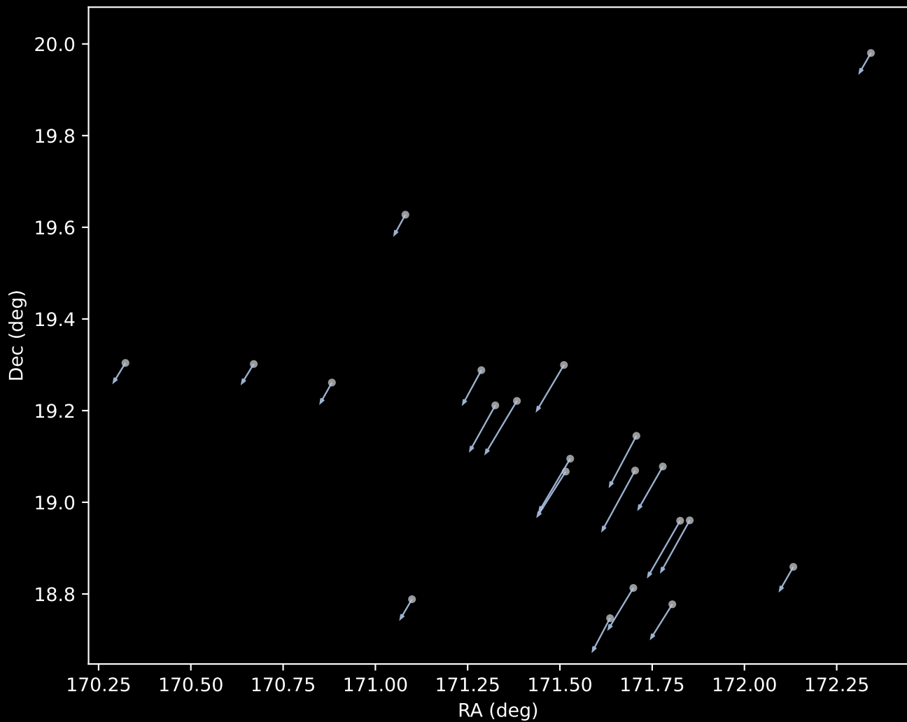
Gaia DR3 Cluster 21 Proper Motion Vectors (n=21)
