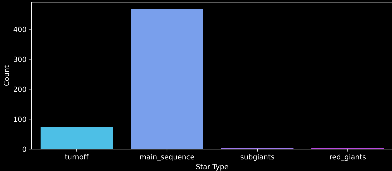
Gaia Cluster: [NGC_1647] Count plot of Star Type
