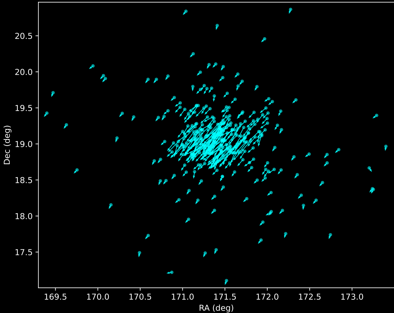
Gaia DR3 Noise Stream Proper Motion Vectors (n=290)
