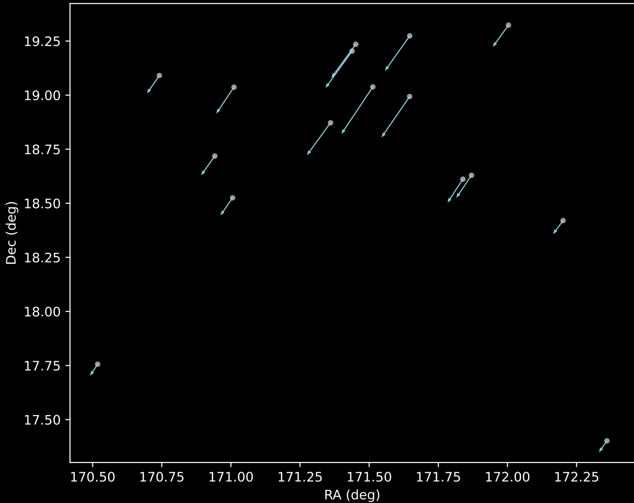
Gaia DR3 Cluster 19 Proper Motion Vectors (n=16)
