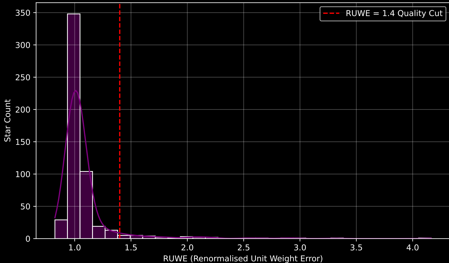
Gaia Cluster: [NGC_1647] RUWE Distribution (n= 543)
