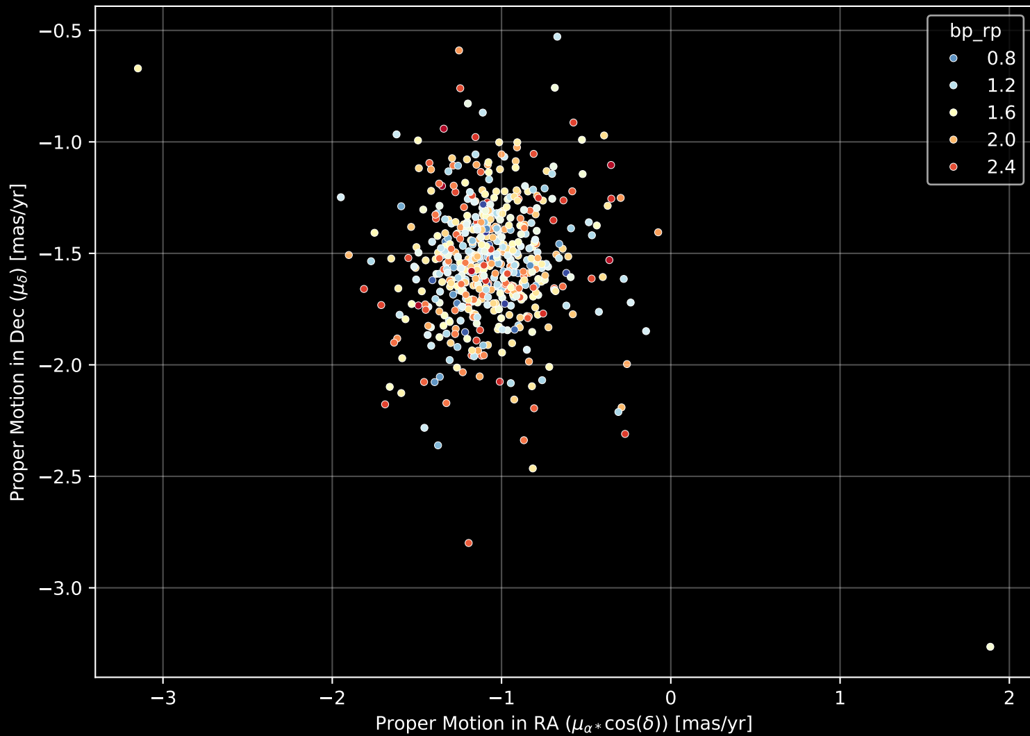
Gaia Cluster: [NGC_1647] Proper Motion Diagram (n= 547)
