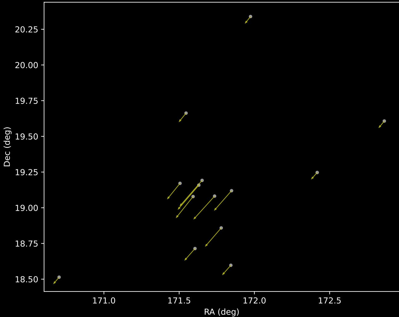
Gaia DR3 Cluster 16 Proper Motion Vectors (n=14)
