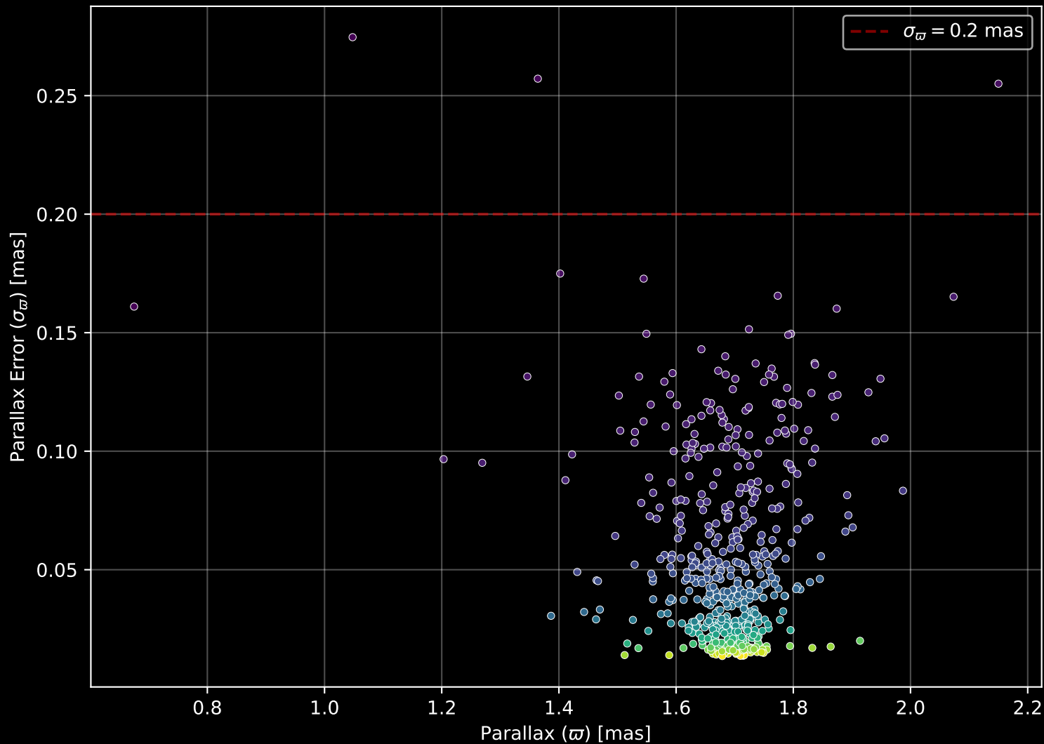
Gaia Cluster: [NGC_1647] Parallax Quality (n= 547)
