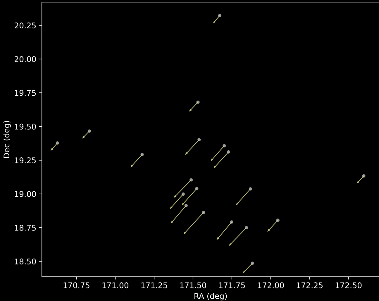
Gaia DR3 Cluster 17 Proper Motion Vectors (n=19)
