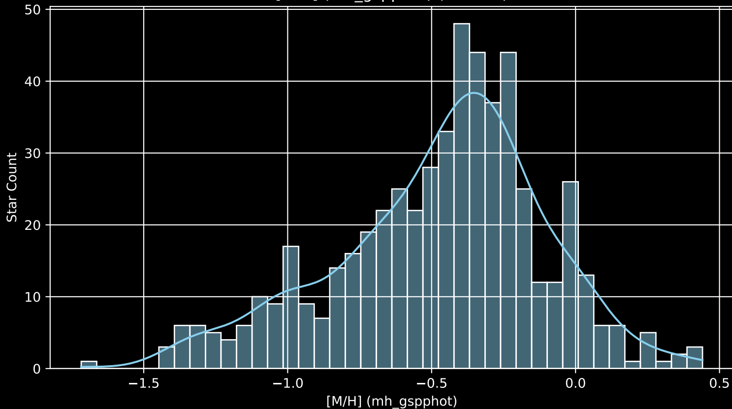
Gaia Cluster: [NGC_1647 [M/H] (mh_gspphot) (n= 547)
