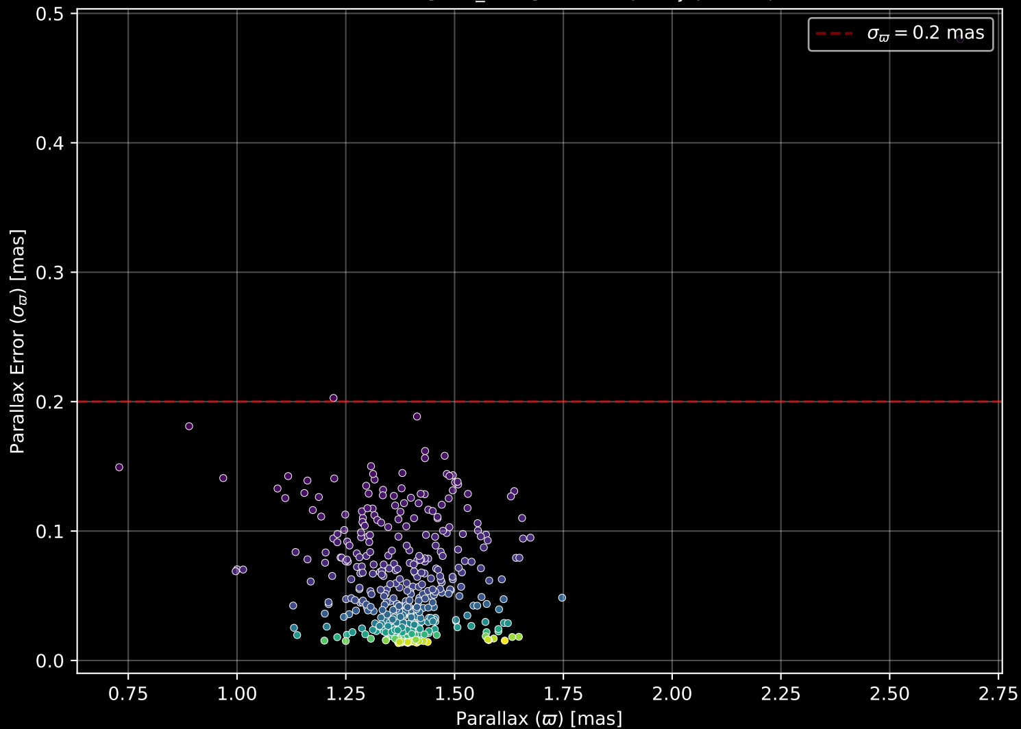
Gaia Cluster: [NGC_1750] Parallax Quality (n= 433)
