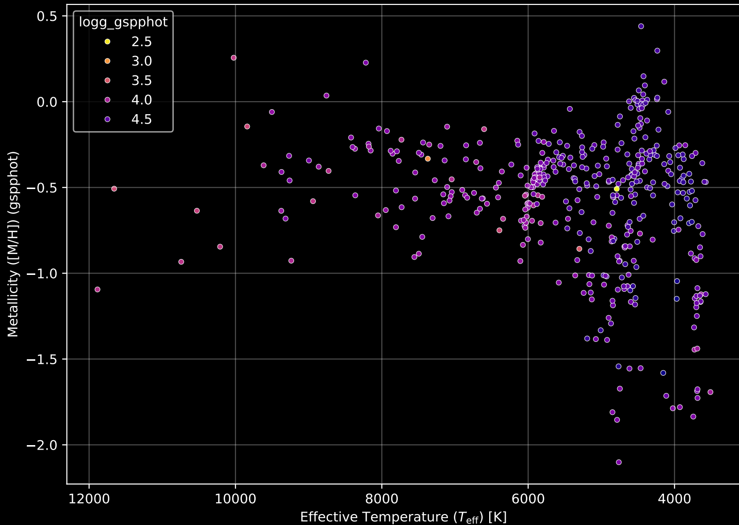
Gaia Cluster: [NGC_1750] Stellar Population Parameters (n= 433)
