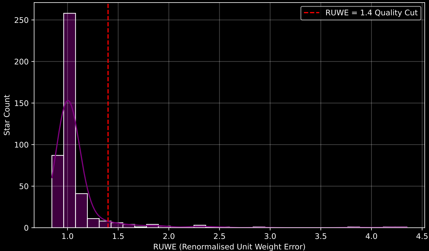
Gaia Cluster: [NGC_1750] RUWE Distribution (n= 431)
