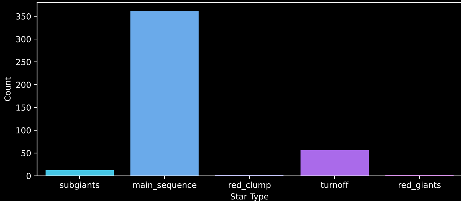
Gaia Cluster: [NGC_1750] Count plot of Star Type
