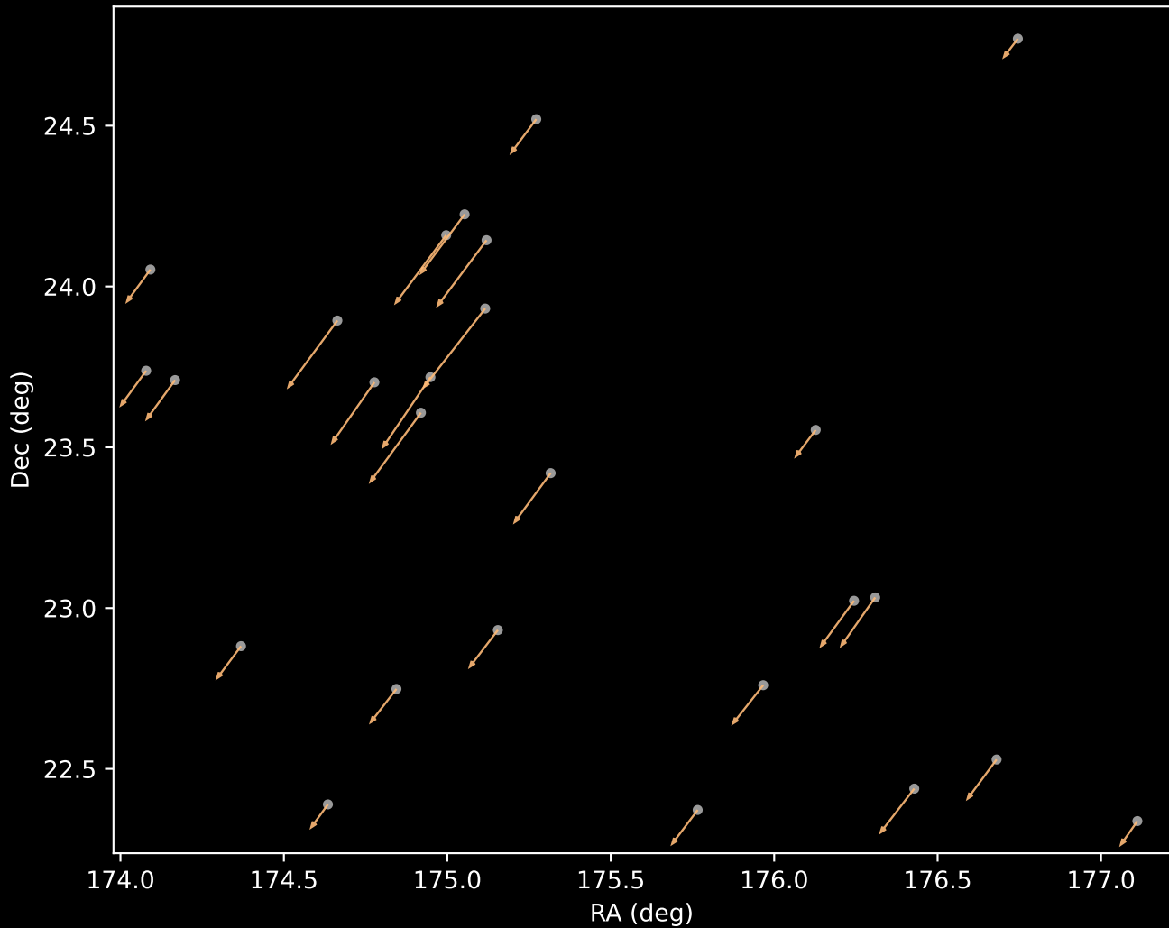
Gaia DR3 Cluster 3 Proper Motion Vectors (n=26)
