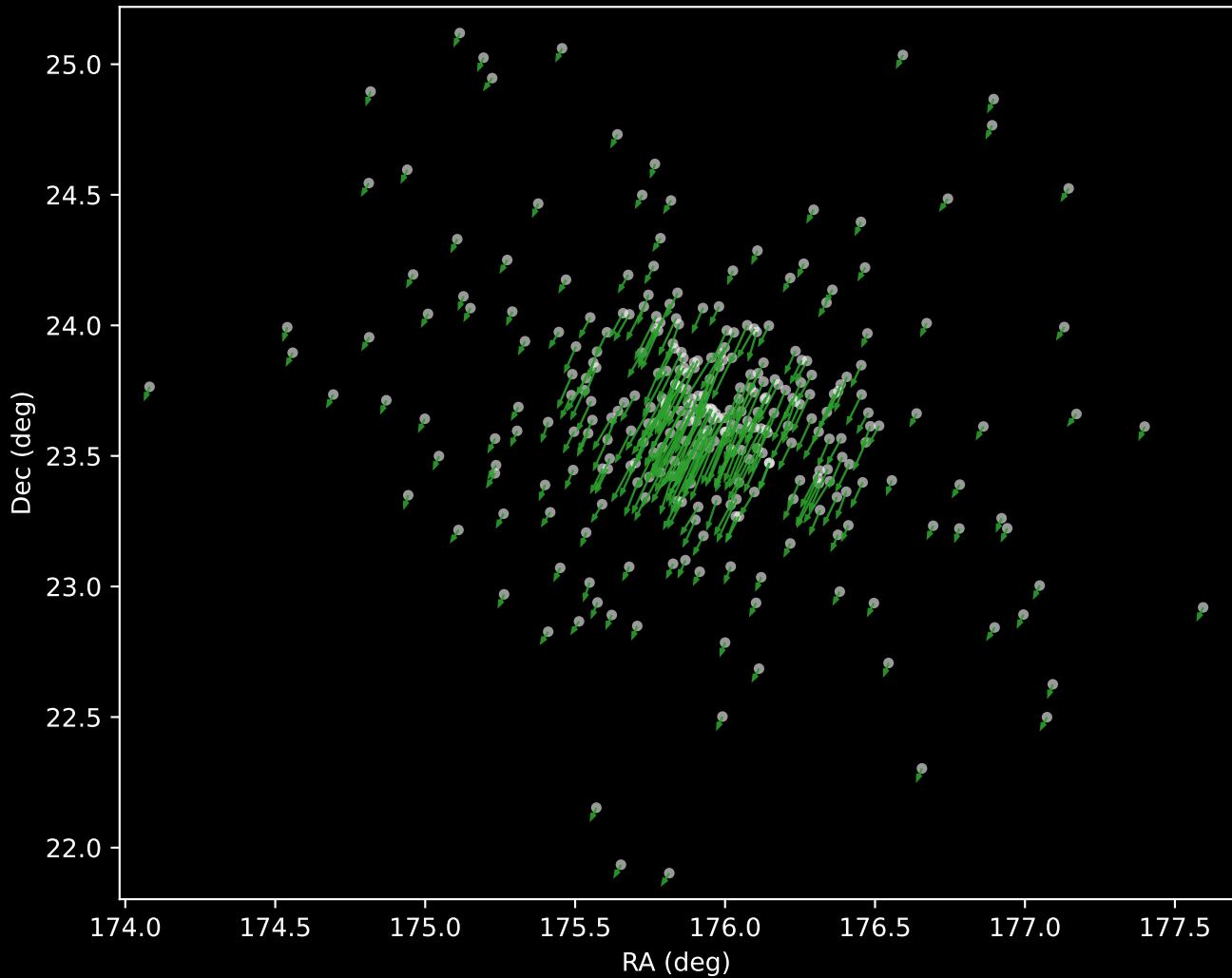
Gaia DR3 Cluster 4 Proper Motion Vectors (n=308)
