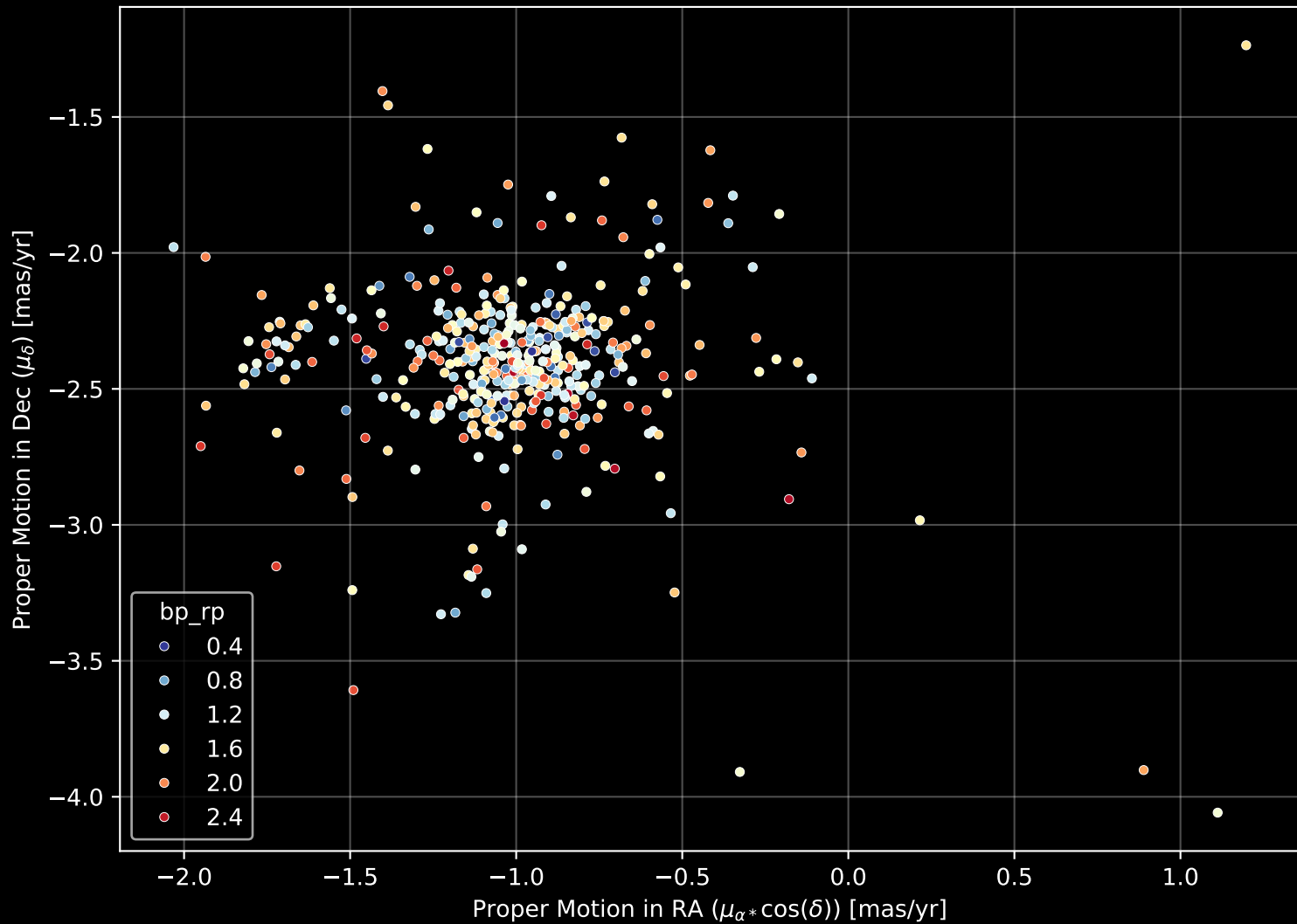
Gaia Cluster: [NGC_1750] Proper Motion Diagram (n= 433)
