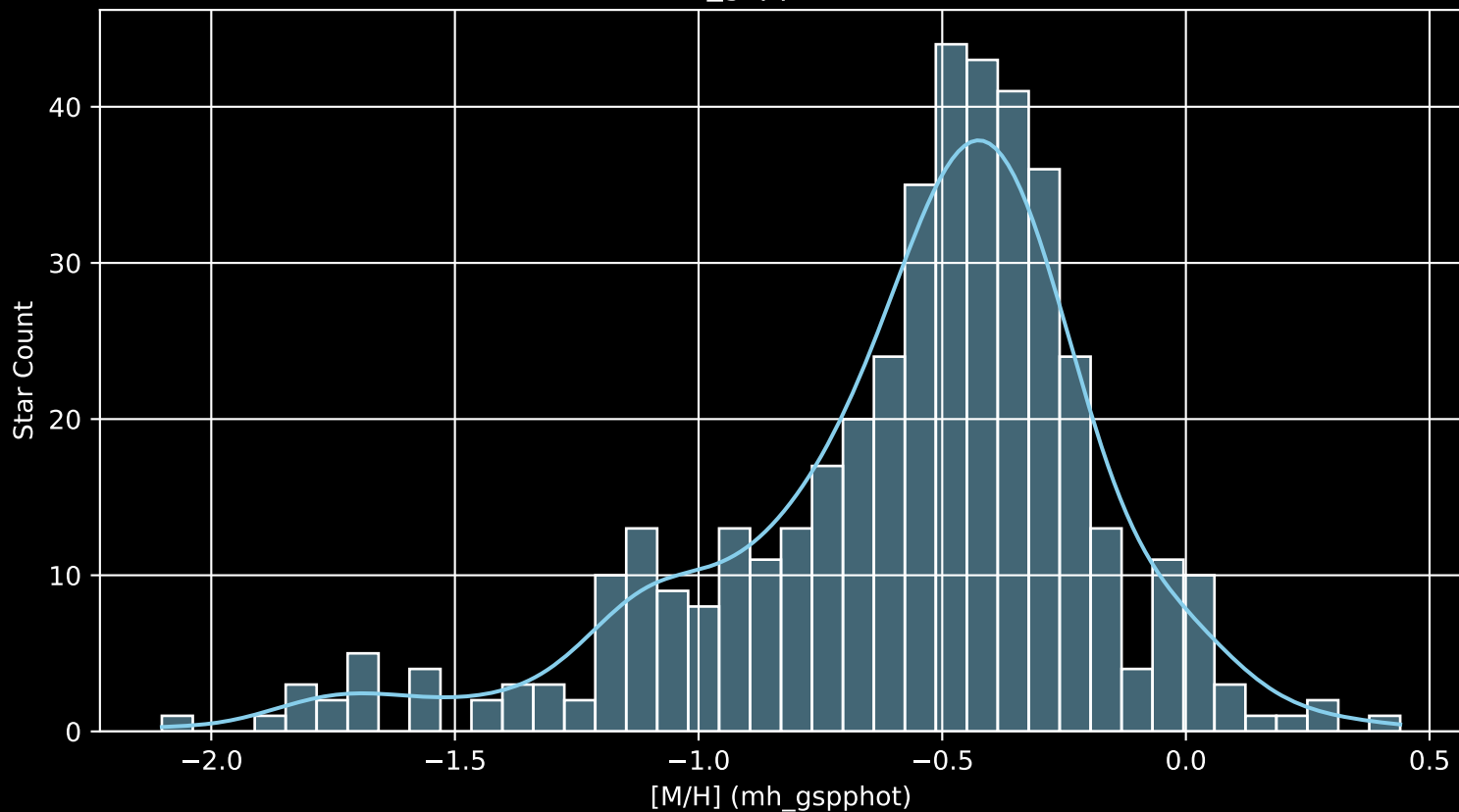
Gaia Cluster: [NGC_1750 [M/H] (mh_gspphot) (n= 433)
