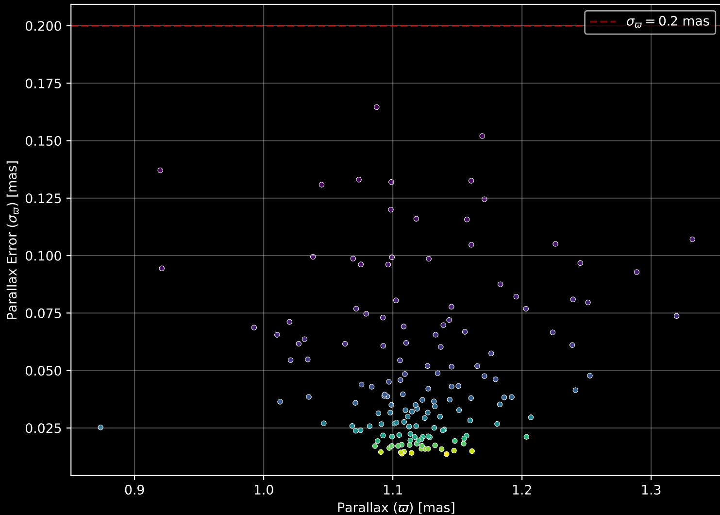
Gaia Cluster: [NGC_1758] Parallax Quality (n= 153)
