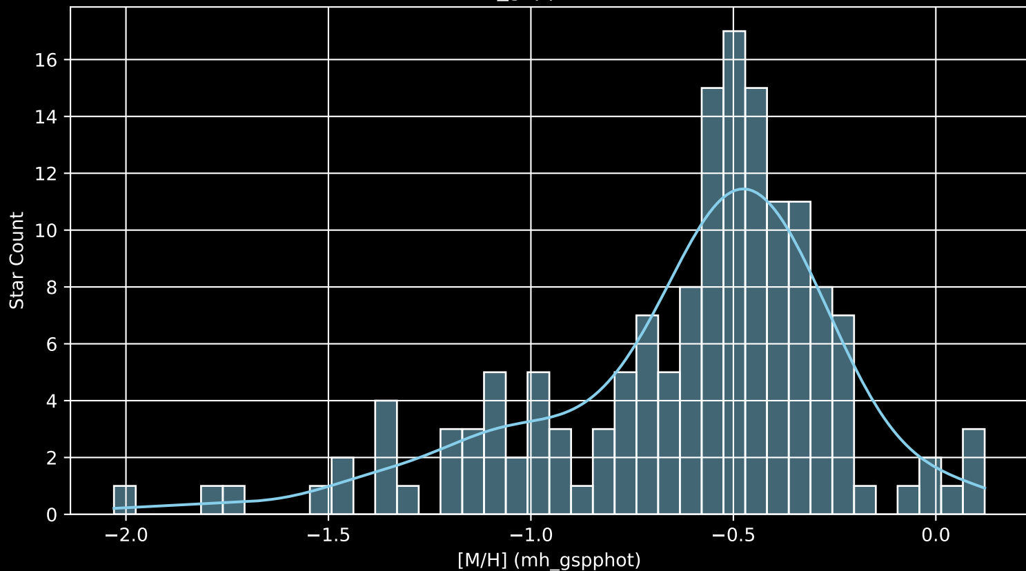
Gaia Cluster: [NGC_1758 [M/H] (mh_gspphot) (n= 153)
