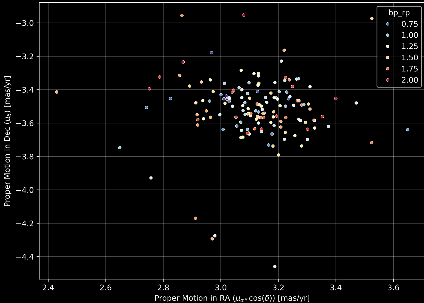
Gaia Cluster: [NGC_1758] Proper Motion Diagram (n= 153)
