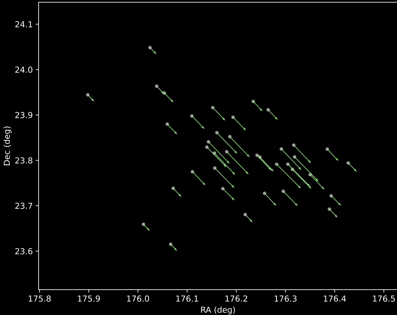
Gaia DR3 Cluster 5 Proper Motion Vectors (n=38)
