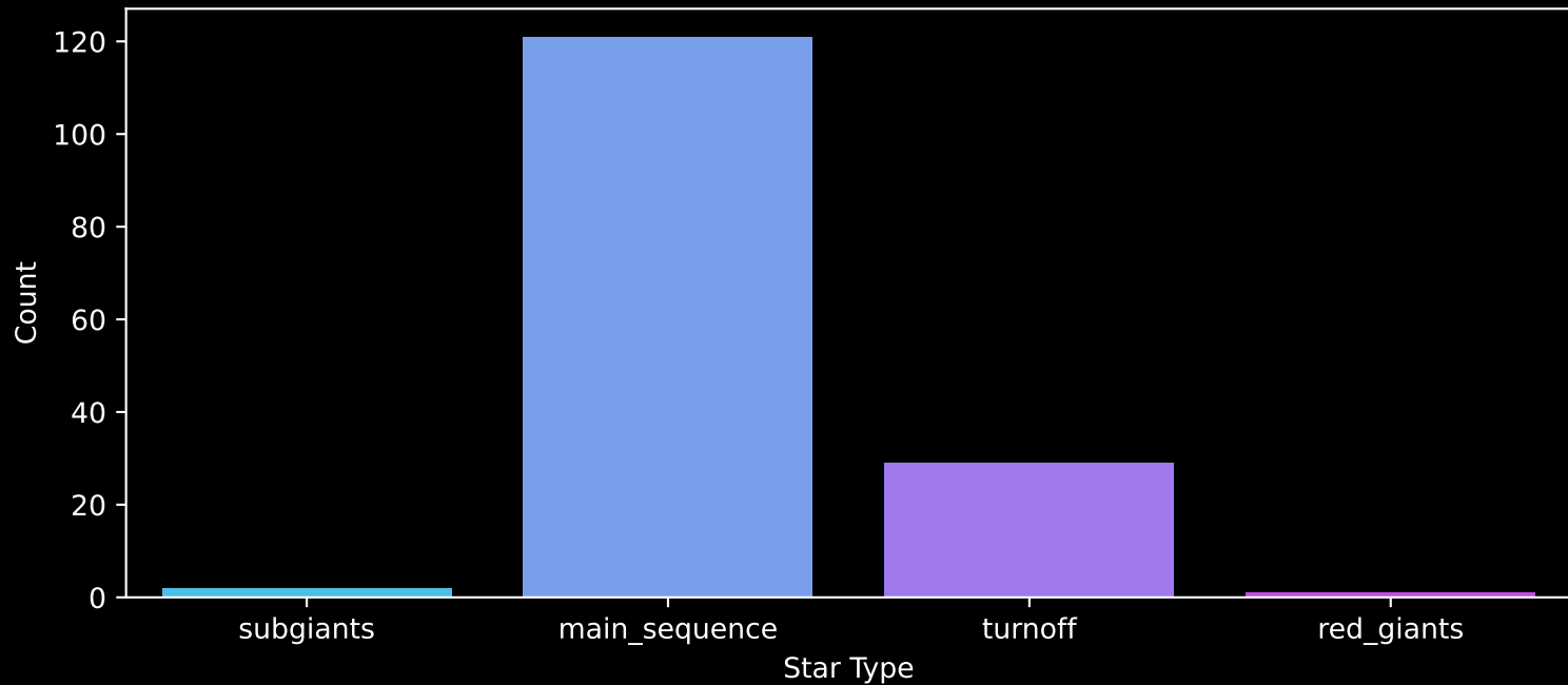
Gaia Cluster: [NGC_1758] Count plot of Star Type
