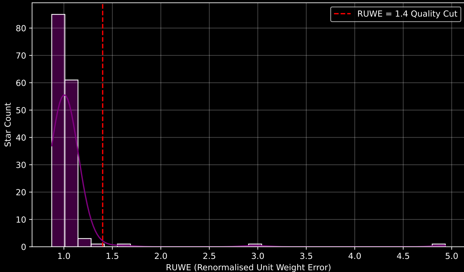
Gaia Cluster: [NGC_1758] RUWE Distribution (n= 153)
