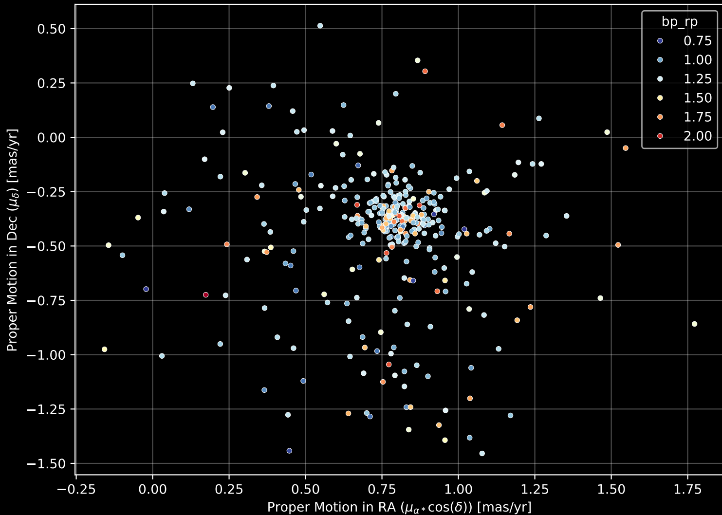
Gaia Cluster: [NGC_1798] Proper Motion Diagram (n= 349)
