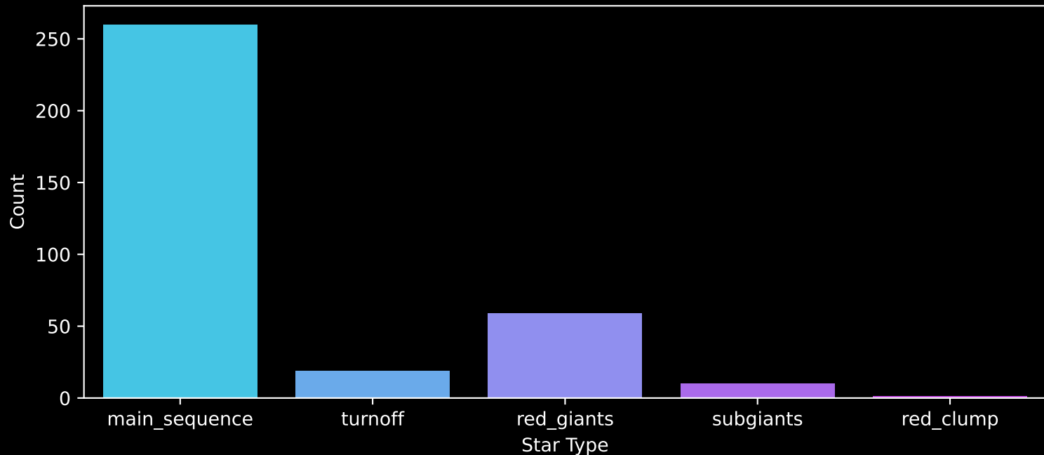
Gaia Cluster: [NGC_1798] Count plot of Star Type
