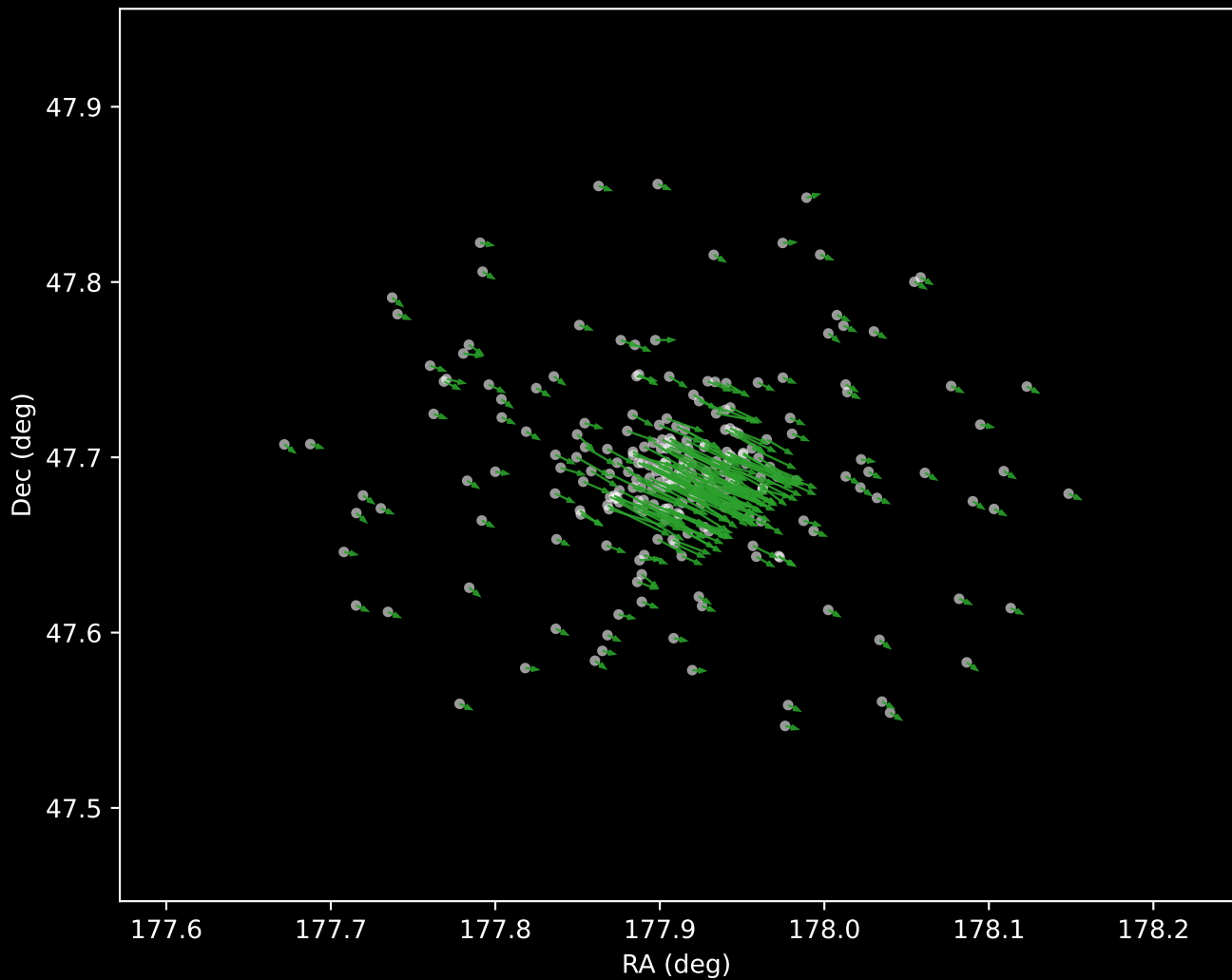
Gaia DR3 Cluster 4 Proper Motion Vectors (n=243)
