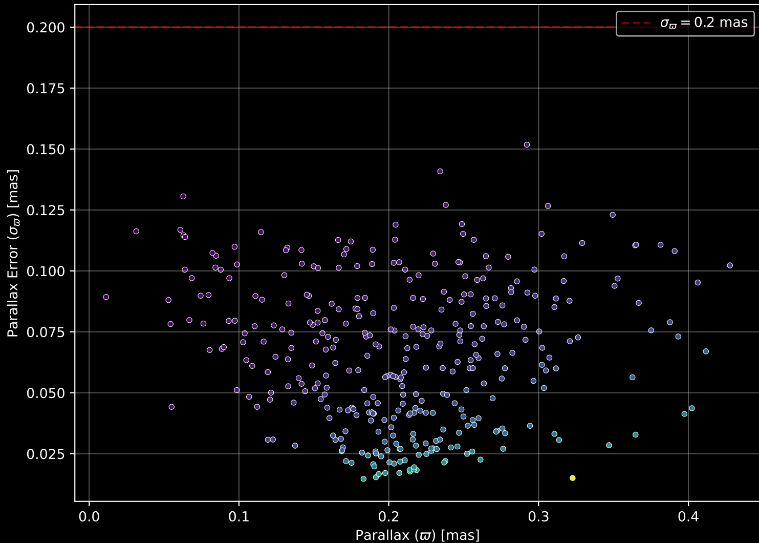
Gaia Cluster: [NGC_1798] Parallax Quality (n= 349)
