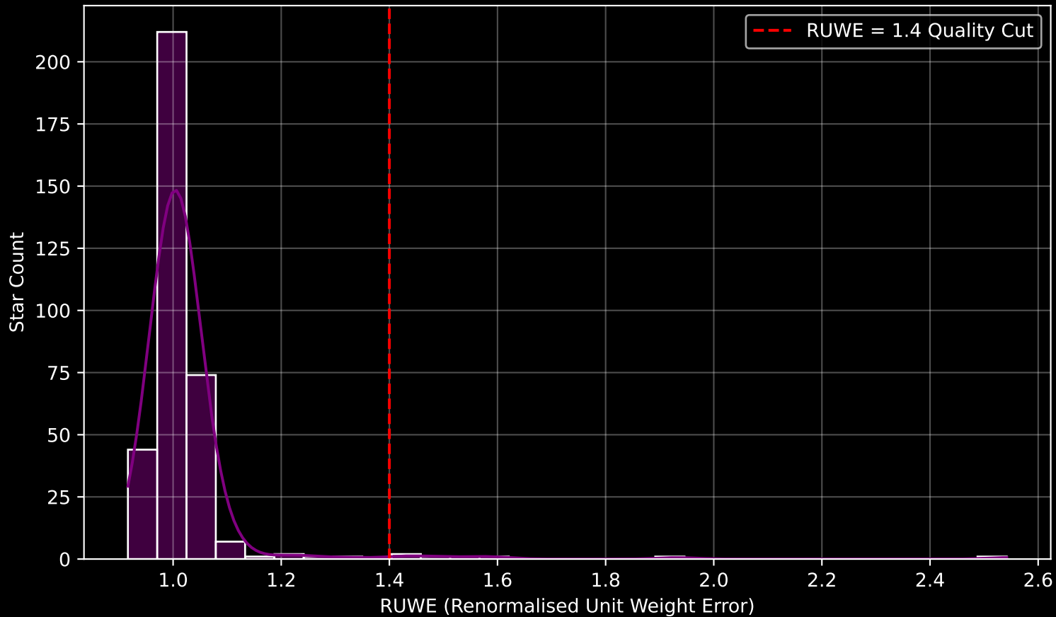
Gaia Cluster: [NGC_1798] RUWE Distribution (n= 349)
