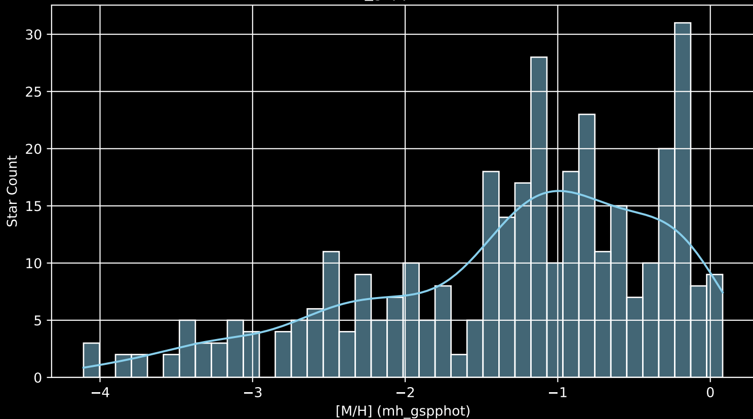
Gaia Cluster: [NGC_1798 [M/H] (mh_gspphot) (n= 349)
