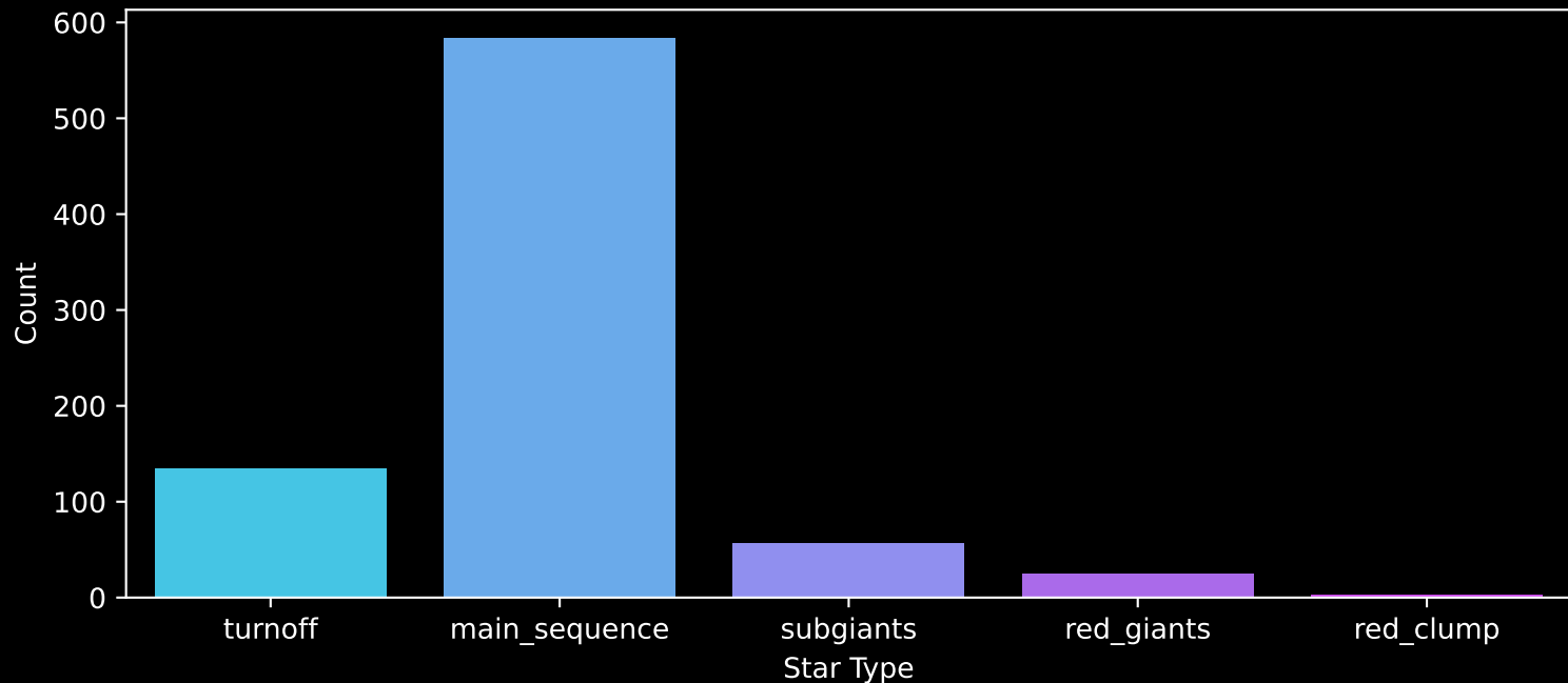
Gaia Cluster: [NGC_188] Count plot of Star Type
