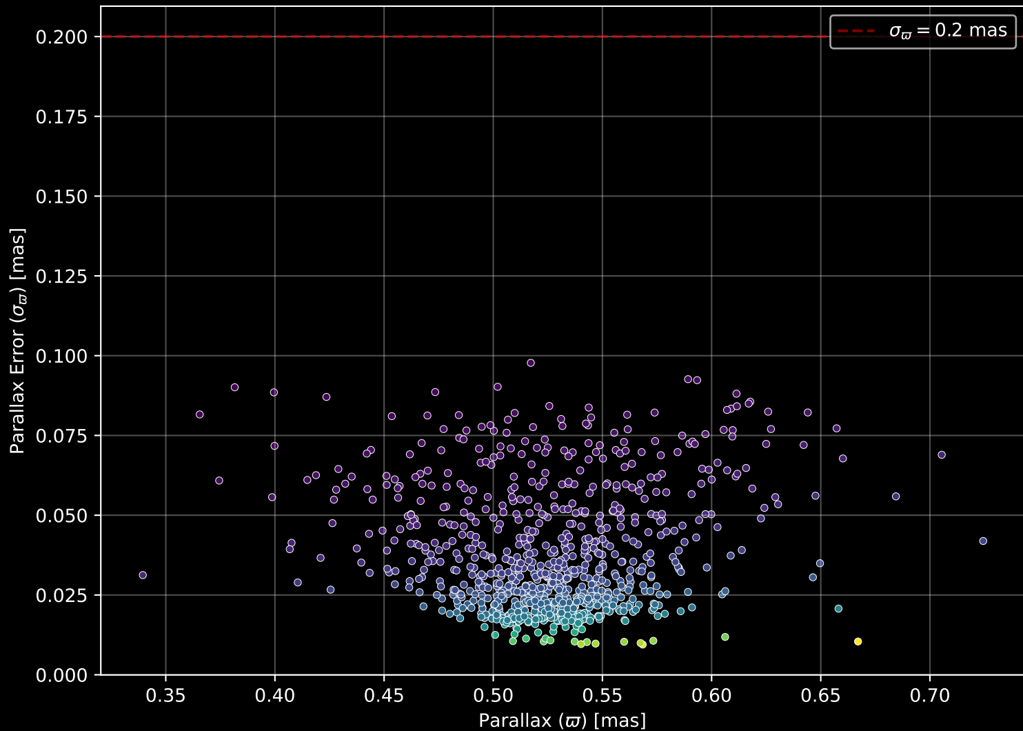
Gaia Cluster: [NGC_188] Parallax Quality (n= 804)
