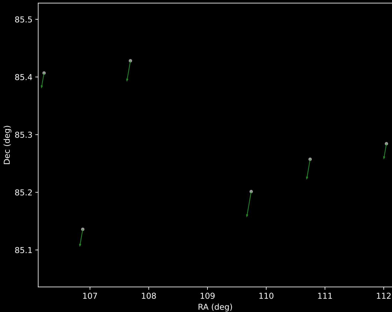
Gaia DR3 Cluster 4 Proper Motion Vectors (n=6)
