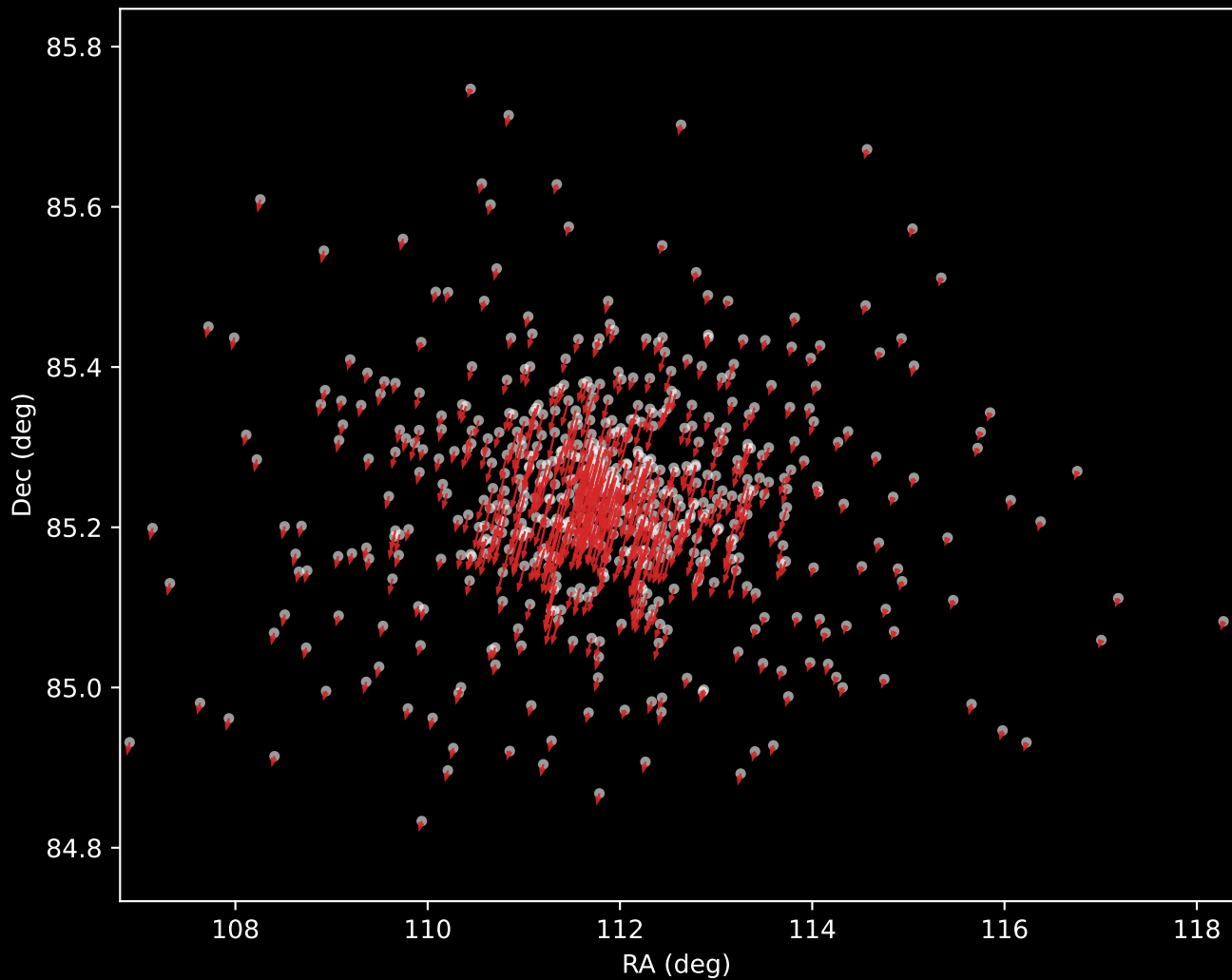
Gaia DR3 Cluster 6 Proper Motion Vectors (n=613)
