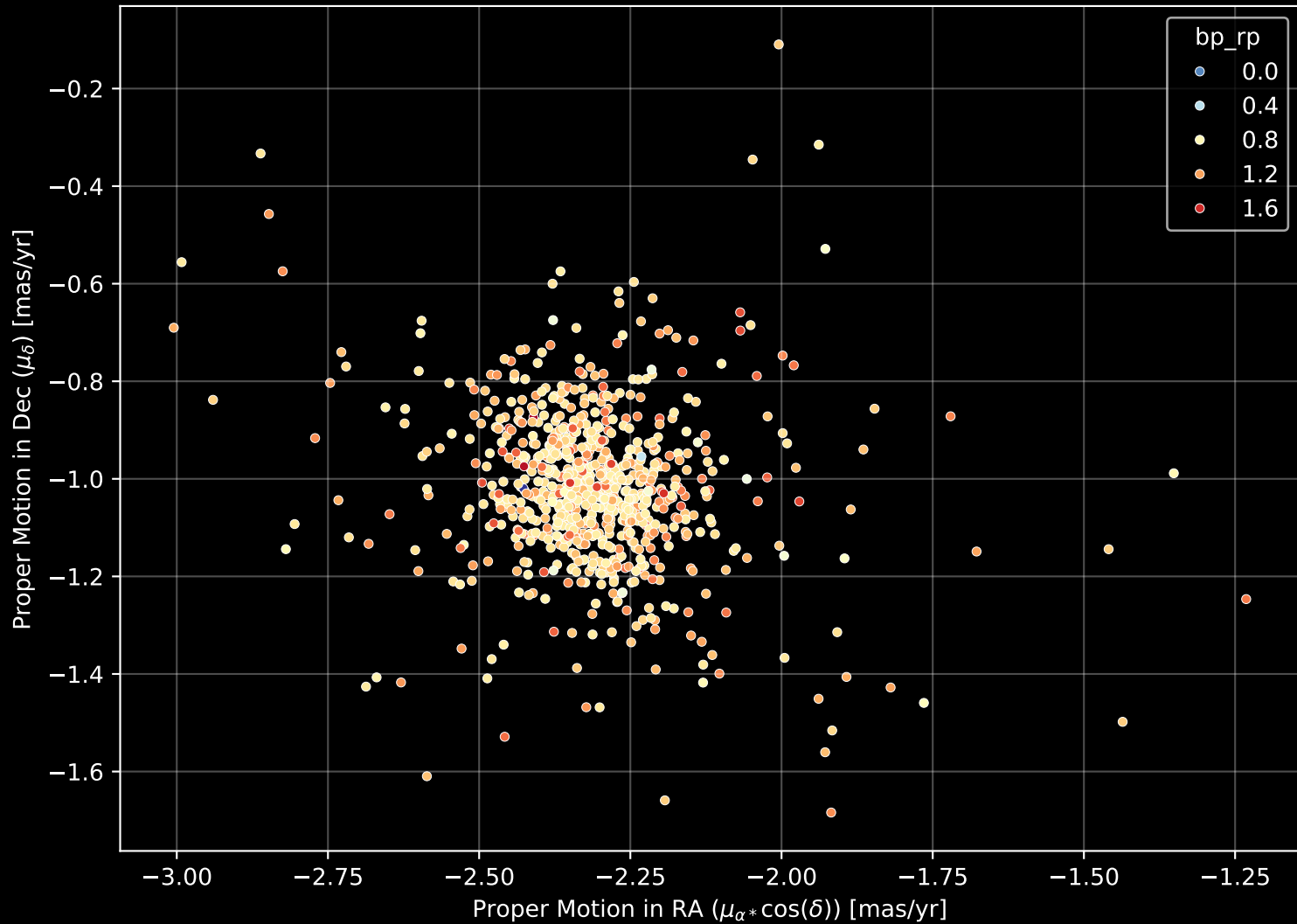
Gaia Cluster: [NGC_188] Proper Motion Diagram (n= 804)
