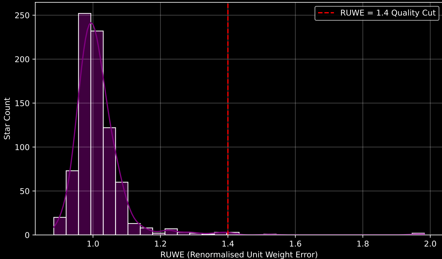
Gaia Cluster: [NGC_188] RUWE Distribution (n= 804)
