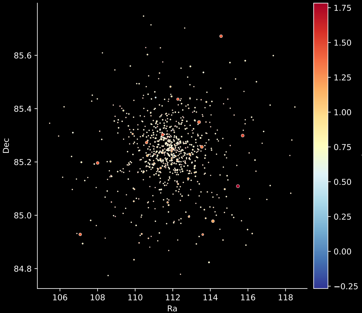
Gaia Cluster: [NGC_188] Stars: 804
