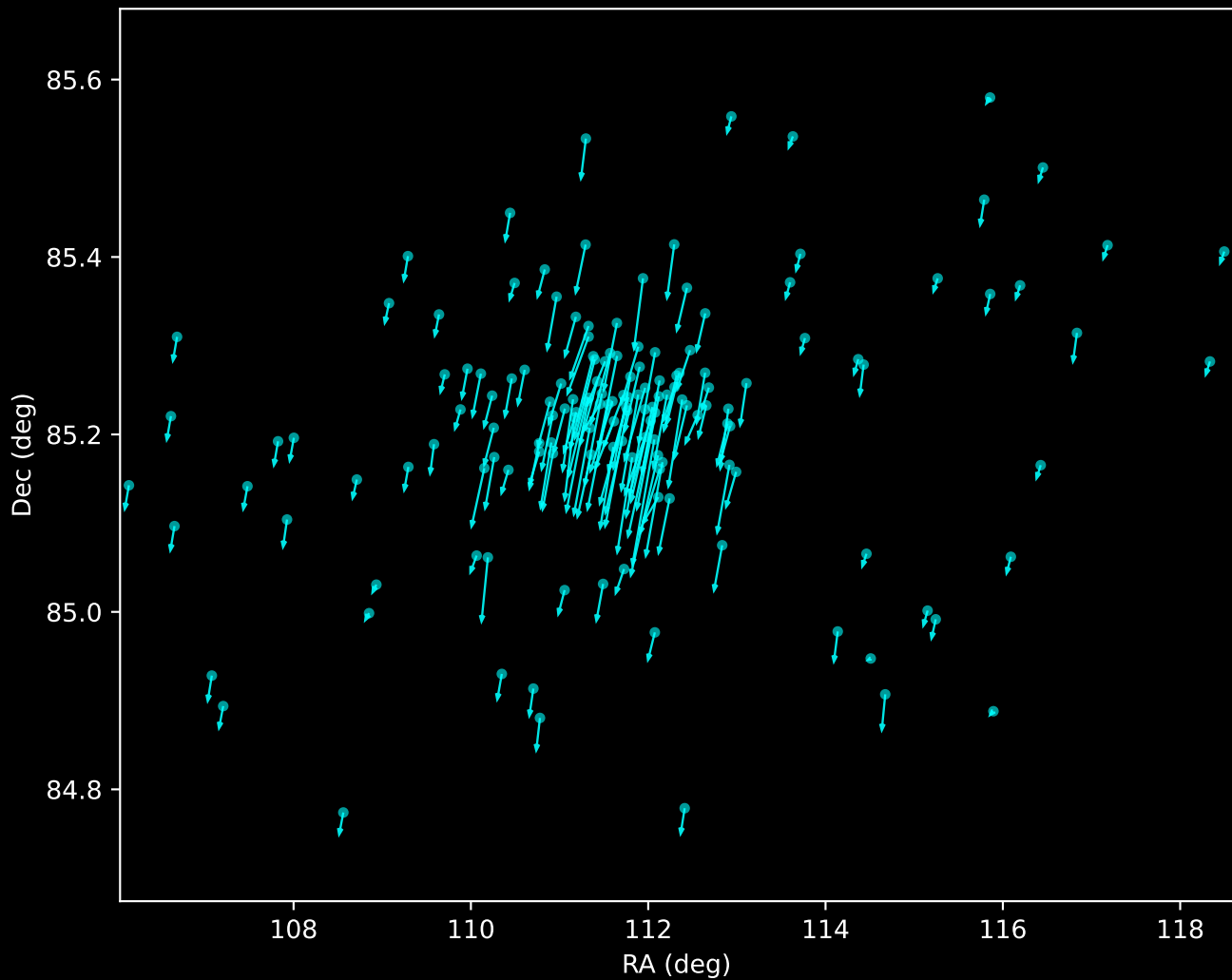
Gaia DR3 Noise Stream Proper Motion Vectors (n=150)
