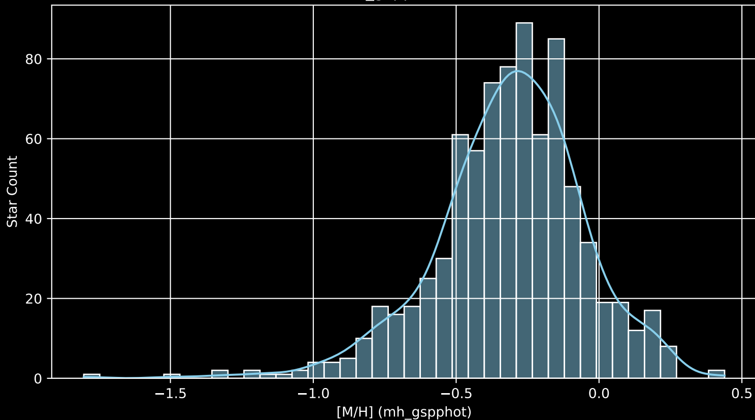
Gaia Cluster: [NGC_188 [M/H] (mh_gspphot) (n= 804)
