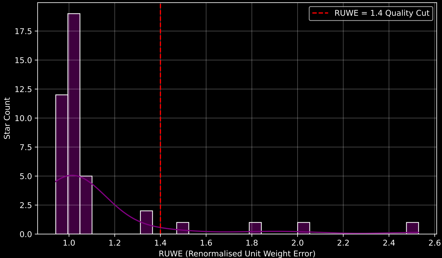
Gaia Cluster: [NGC_189] RUWE Distribution (n= 42)
