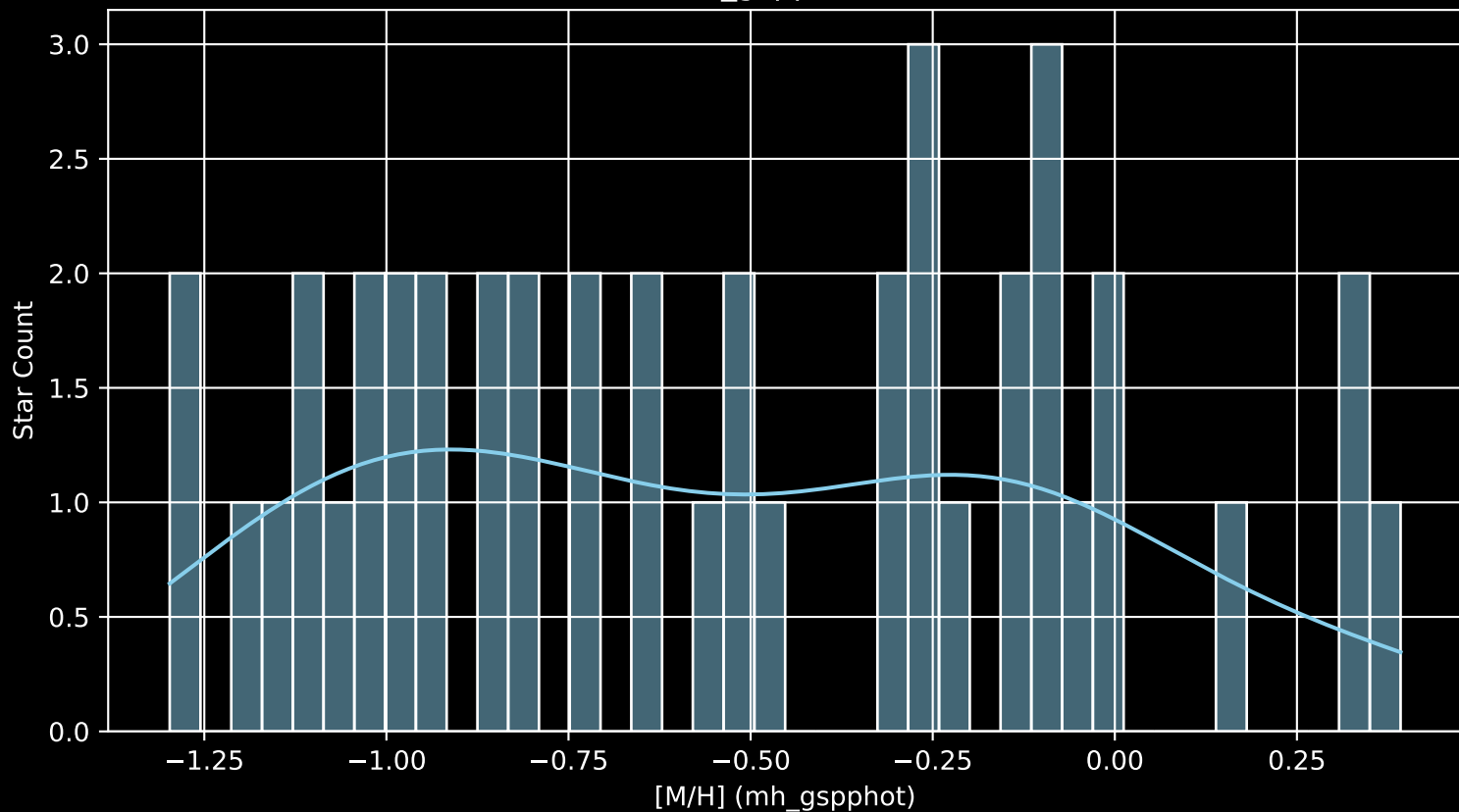
Gaia Cluster: [NGC_189 [M/H] (mh_gspphot) (n= 43)
