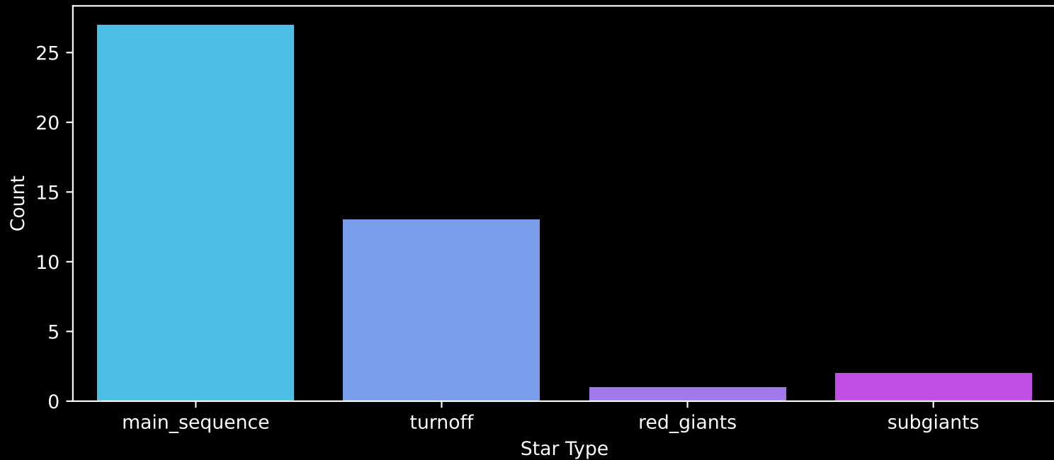
Gaia Cluster: [NGC_189] Count plot of Star Type
