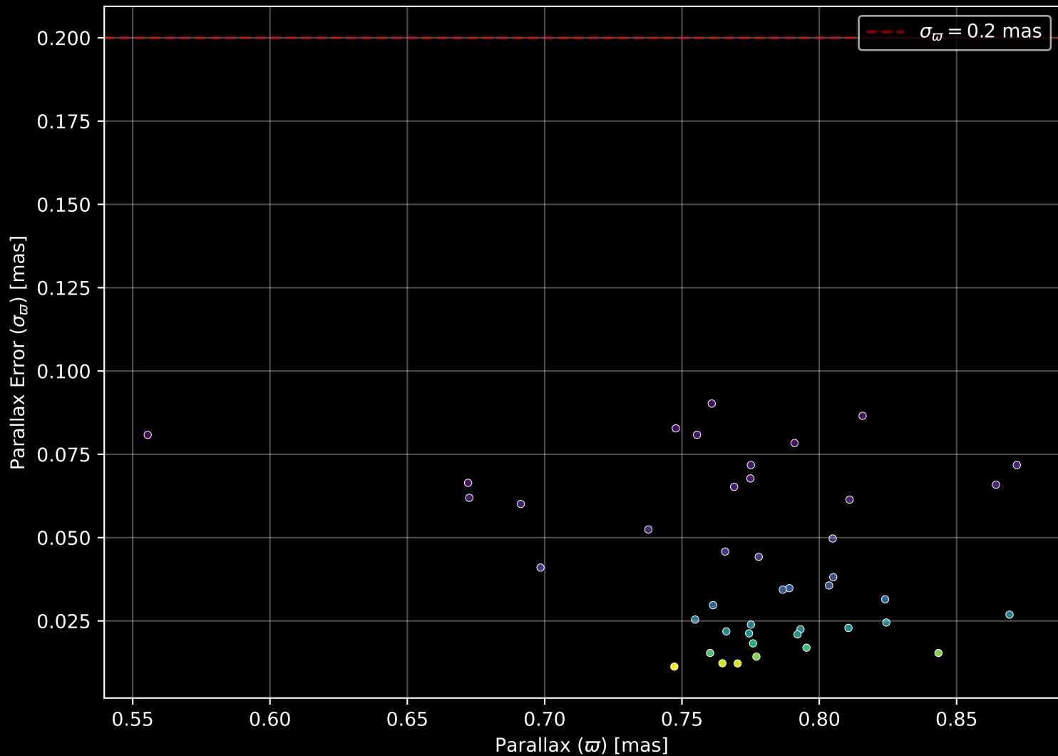
Gaia Cluster: [NGC_189] Parallax Quality (n= 43)
