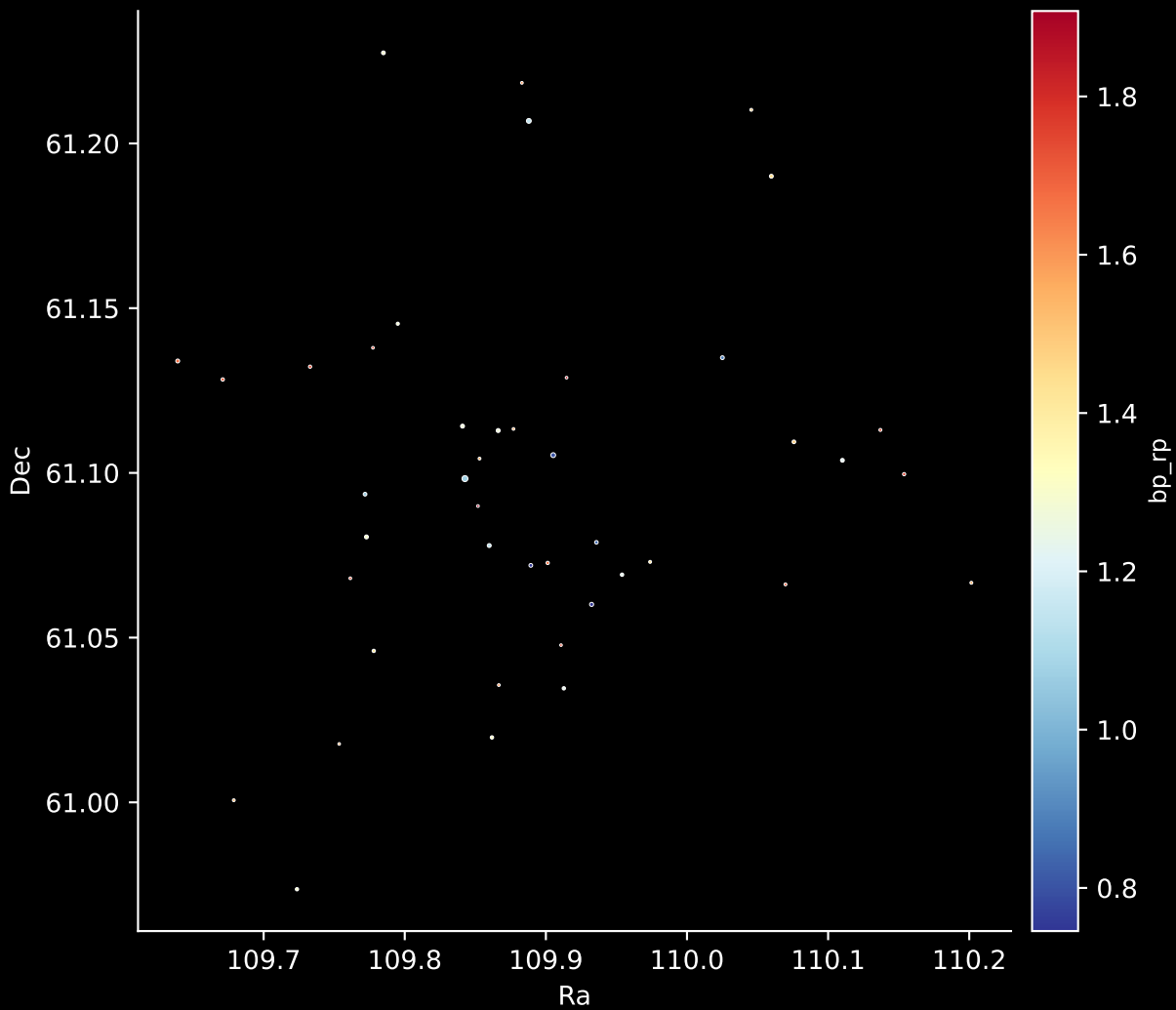
Gaia Cluster: [NGC_189] Stars: 43
