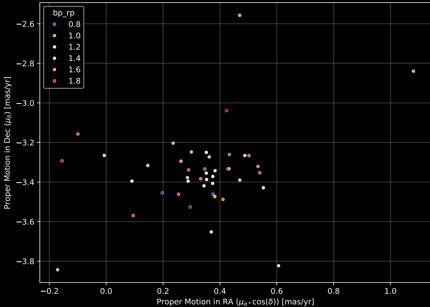
Gaia Cluster: [NGC_189] Proper Motion Diagram (n= 43)
