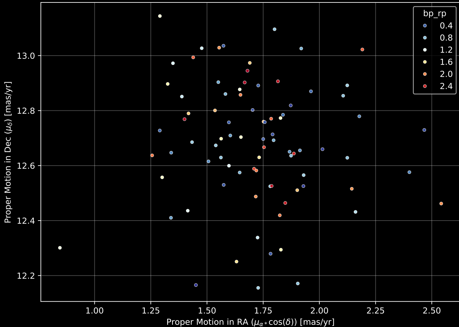
Gaia Cluster: [NGC_1901] Proper Motion Diagram (n= 85)
