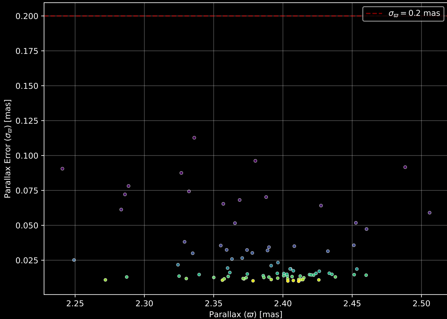
Gaia Cluster: [NGC_1901] Parallax Quality (n= 85)
