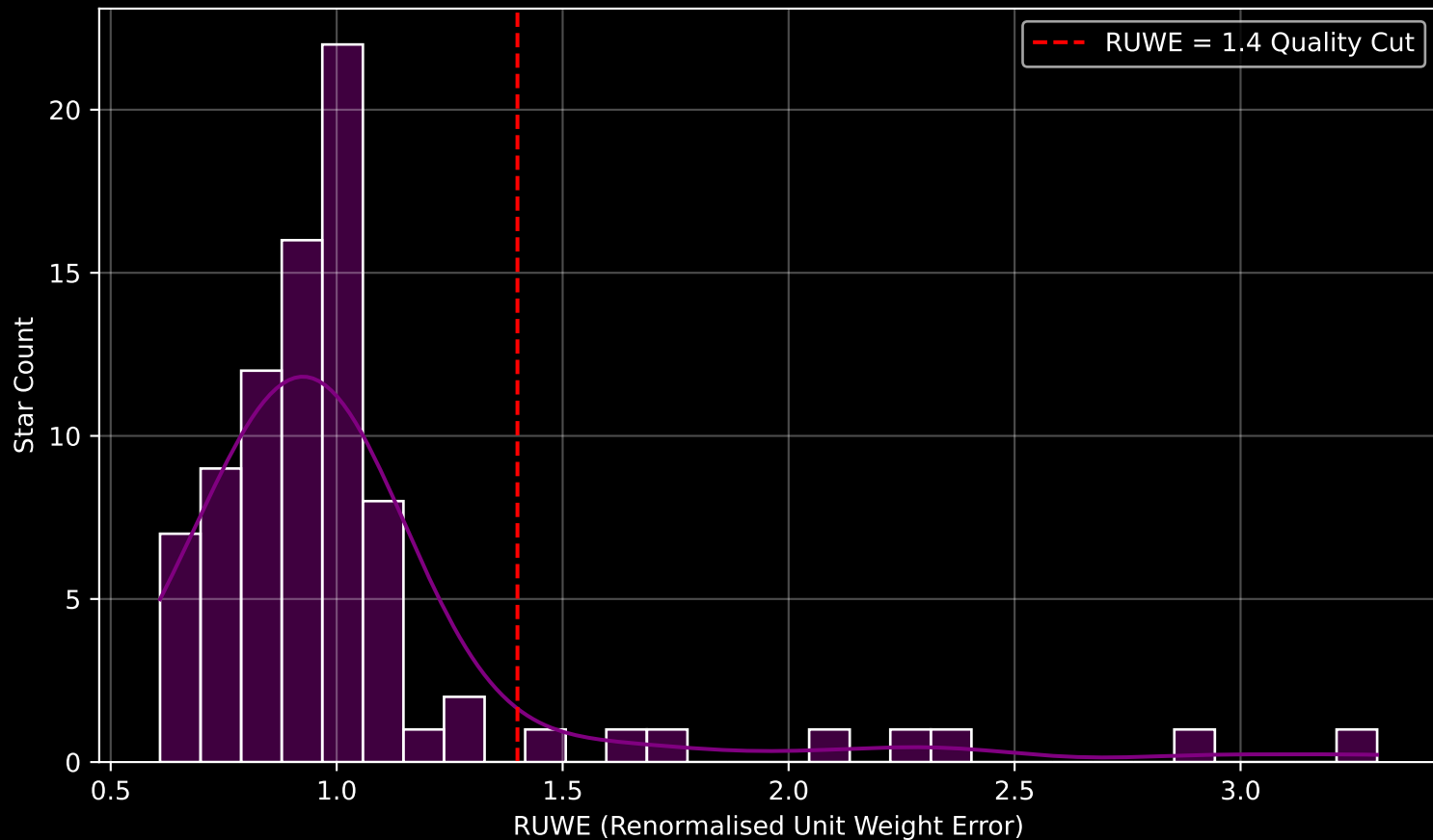
Gaia Cluster: [NGC_1901] RUWE Distribution (n= 85)
