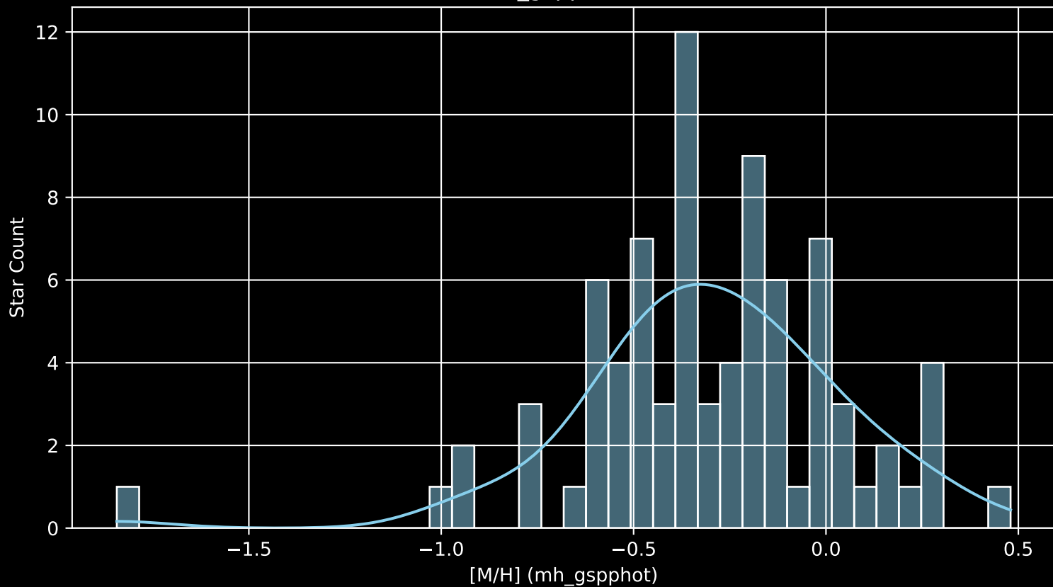
Gaia Cluster: [NGC_1901 [M/H] (mh_gspphot) (n= 82)
