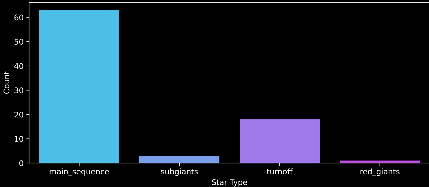
Gaia Cluster: [NGC_1901] Count plot of Star Type
