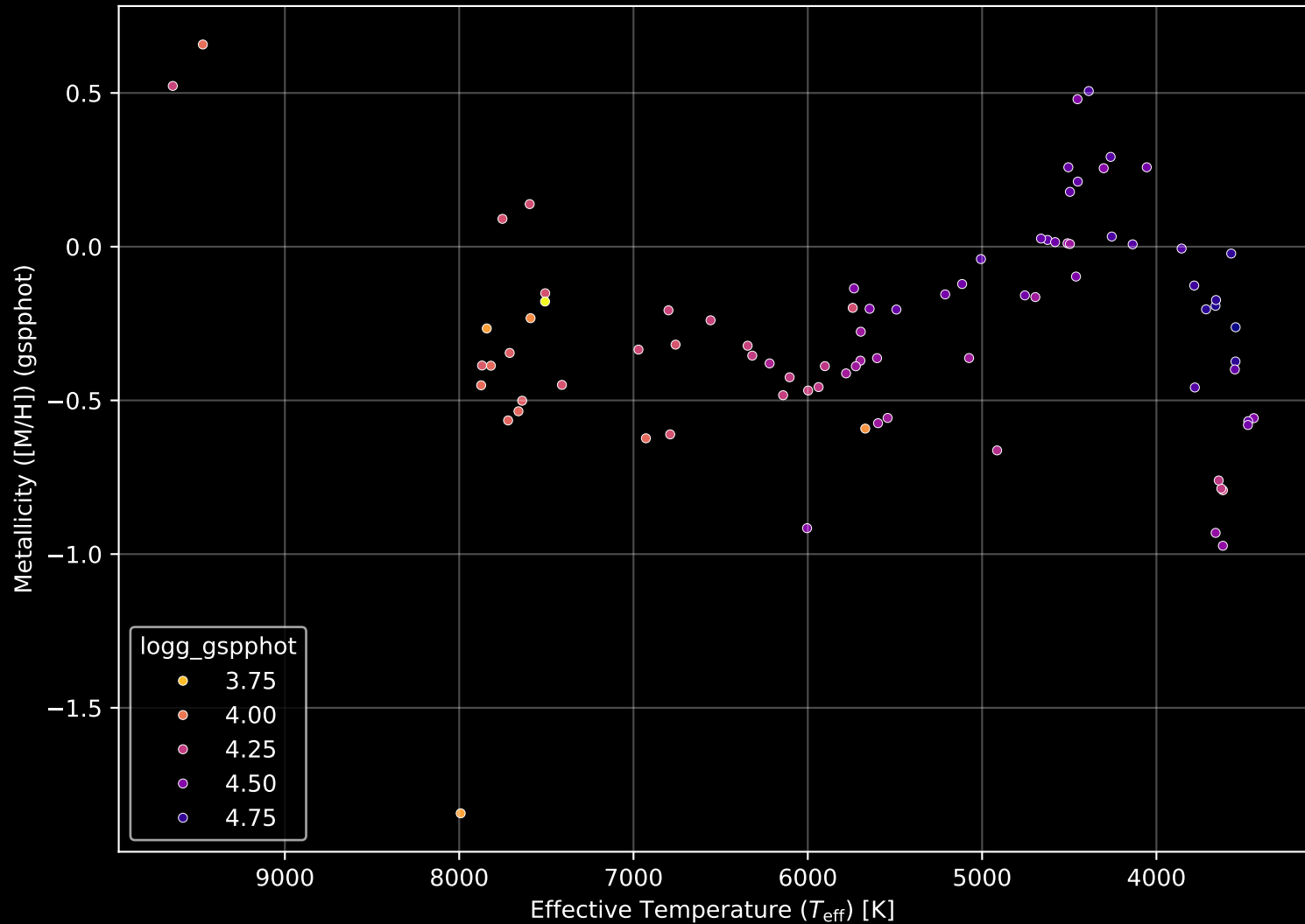
Gaia Cluster: [NGC_1901] Stellar Population Parameters (n= 85)
