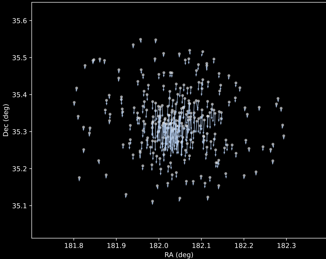
Gaia DR3 Cluster 1 Proper Motion Vectors (n=286)
