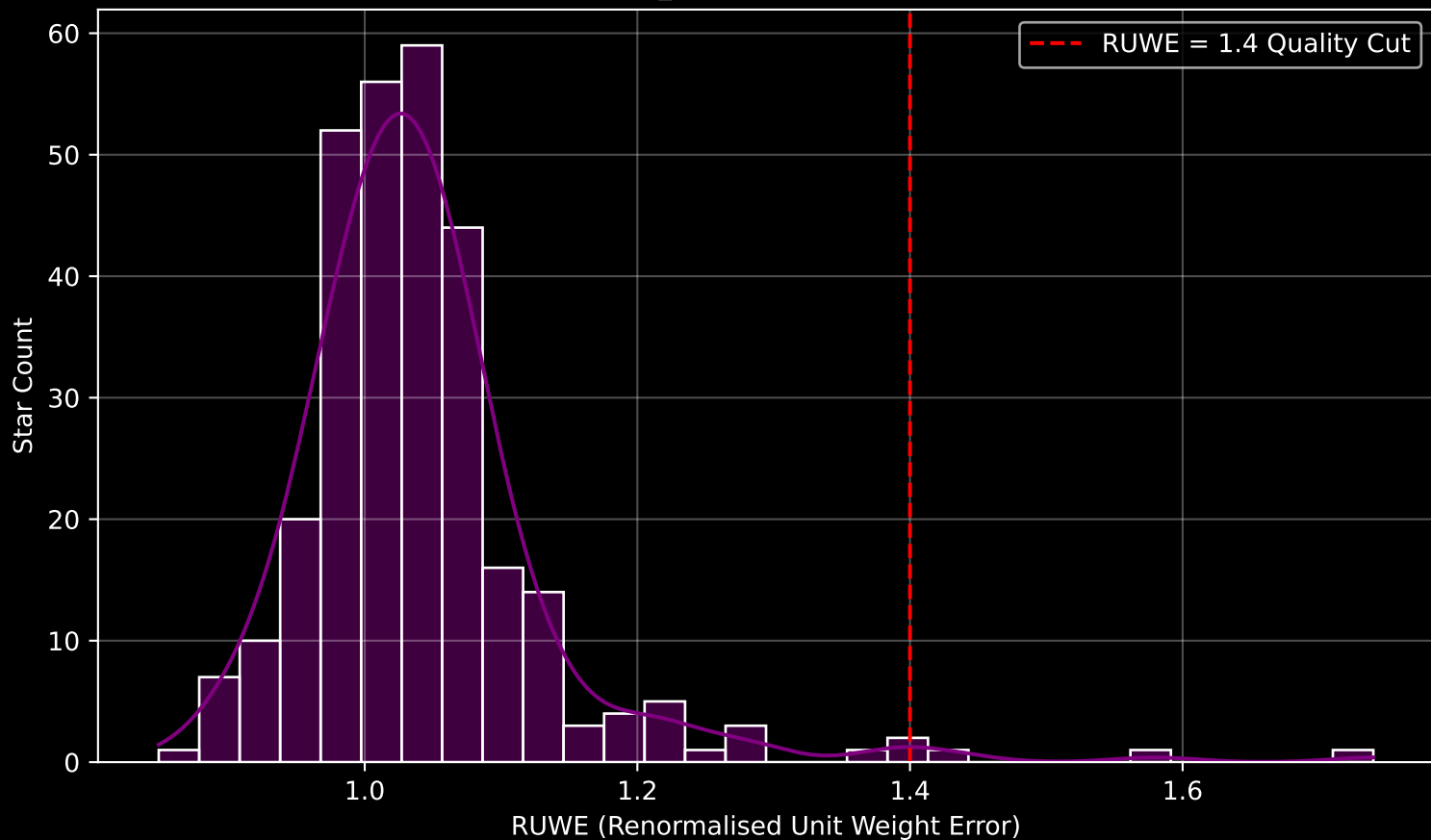
Gaia Cluster: [NGC_1907] RUWE Distribution (n= 301)
