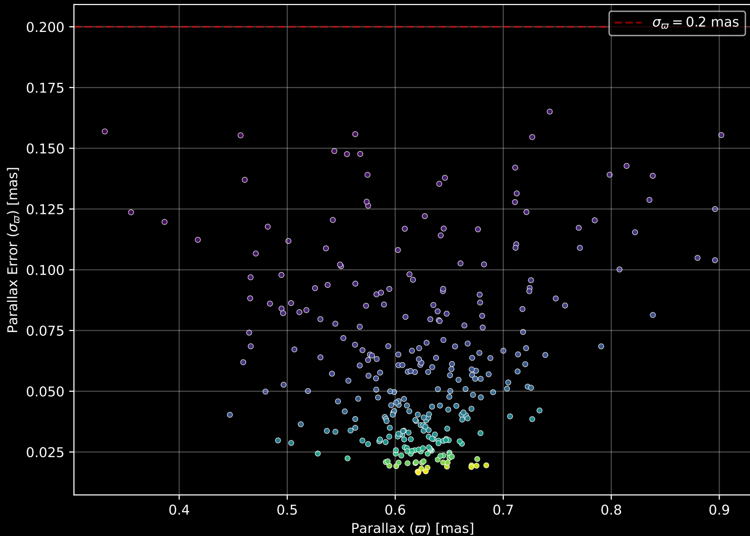
Gaia Cluster: [NGC_1907] Parallax Quality (n= 301)
