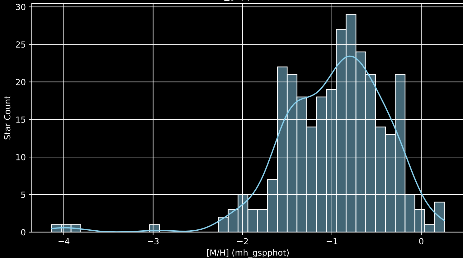
Gaia Cluster: [NGC_1907 [M/H] (mh_gspphot) (n= 301)
