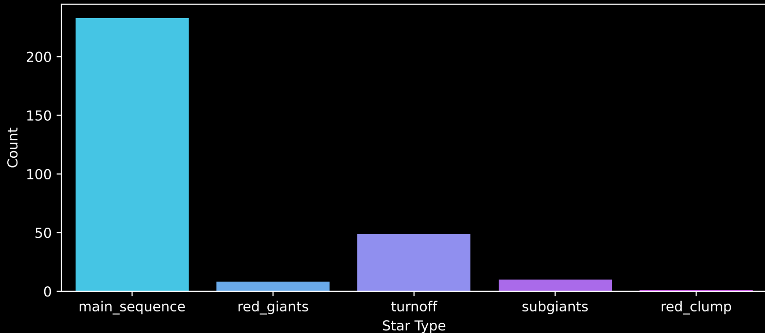
Gaia Cluster: [NGC_1907] Count plot of Star Type
