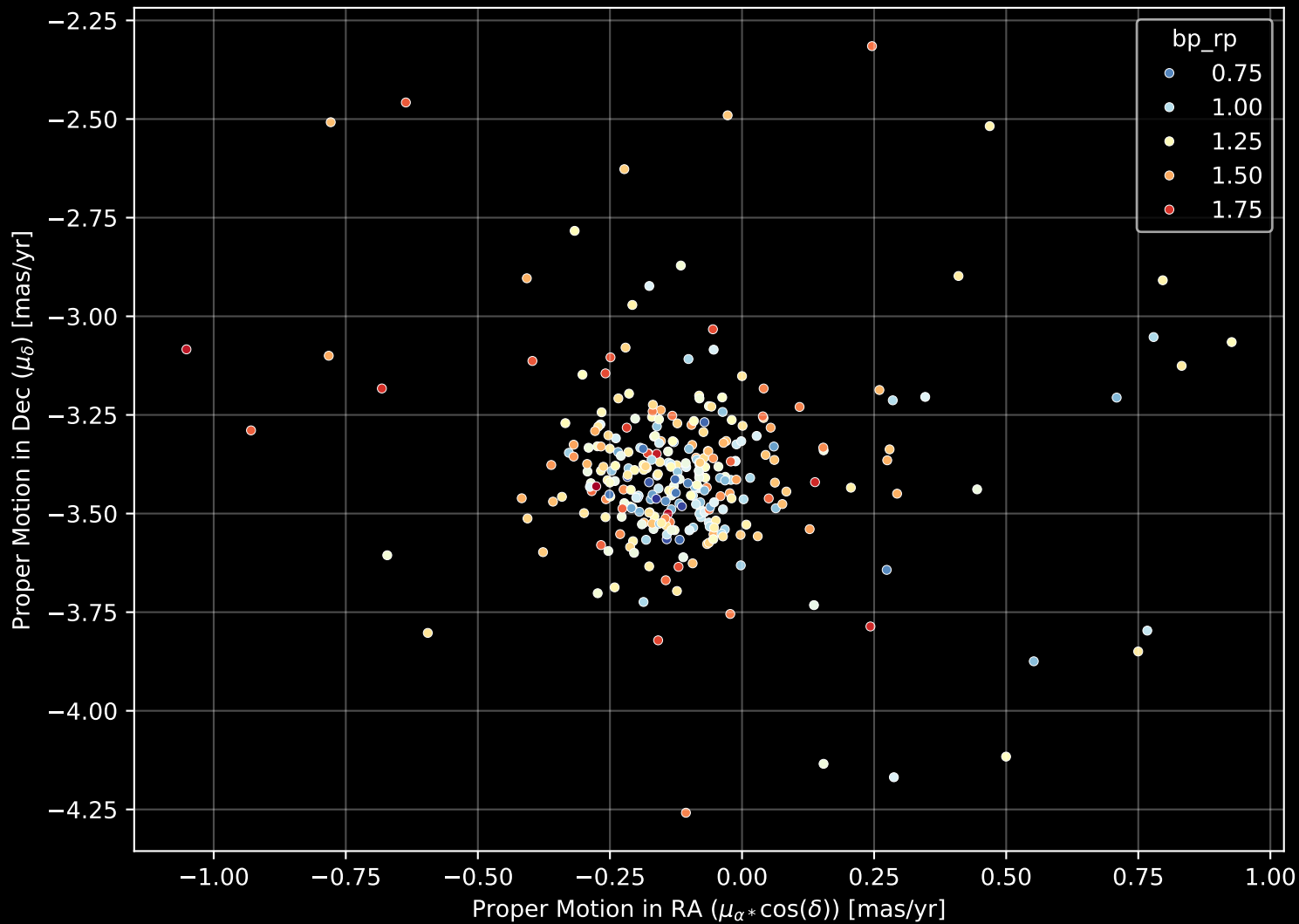
Gaia Cluster: [NGC_1907] Proper Motion Diagram (n= 301)
