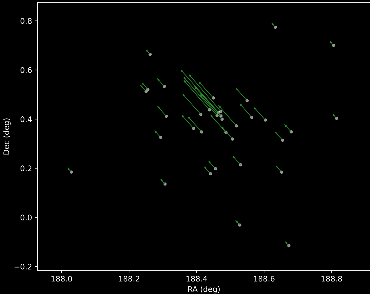
Gaia DR3 Cluster 24 Proper Motion Vectors (n=35)
