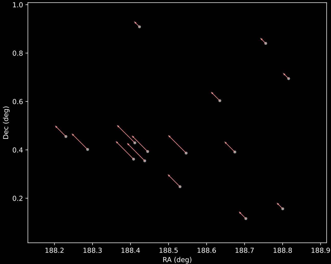
Gaia DR3 Cluster 27 Proper Motion Vectors (n=15)
