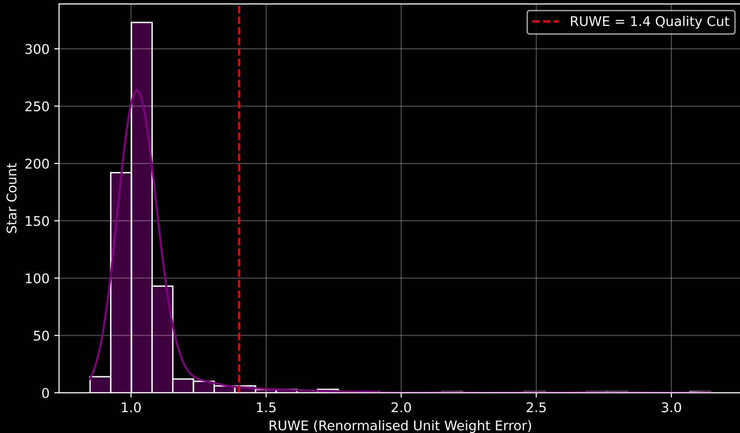
Gaia Cluster: [NGC_2112] RUWE Distribution (n= 672)
