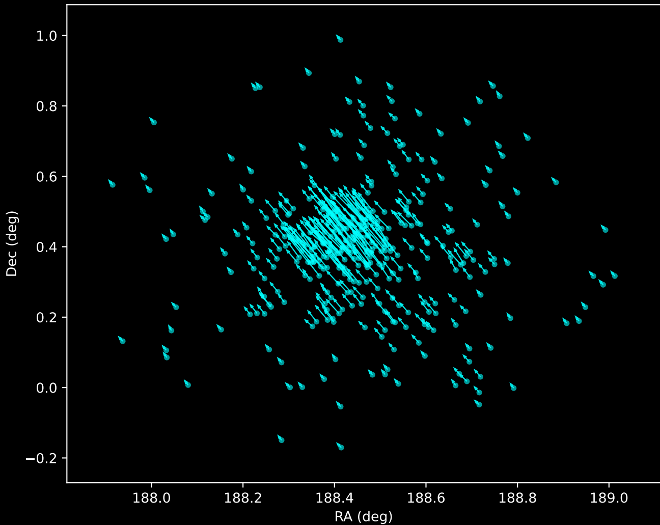
Gaia DR3 Noise Stream Proper Motion Vectors (n=343)
