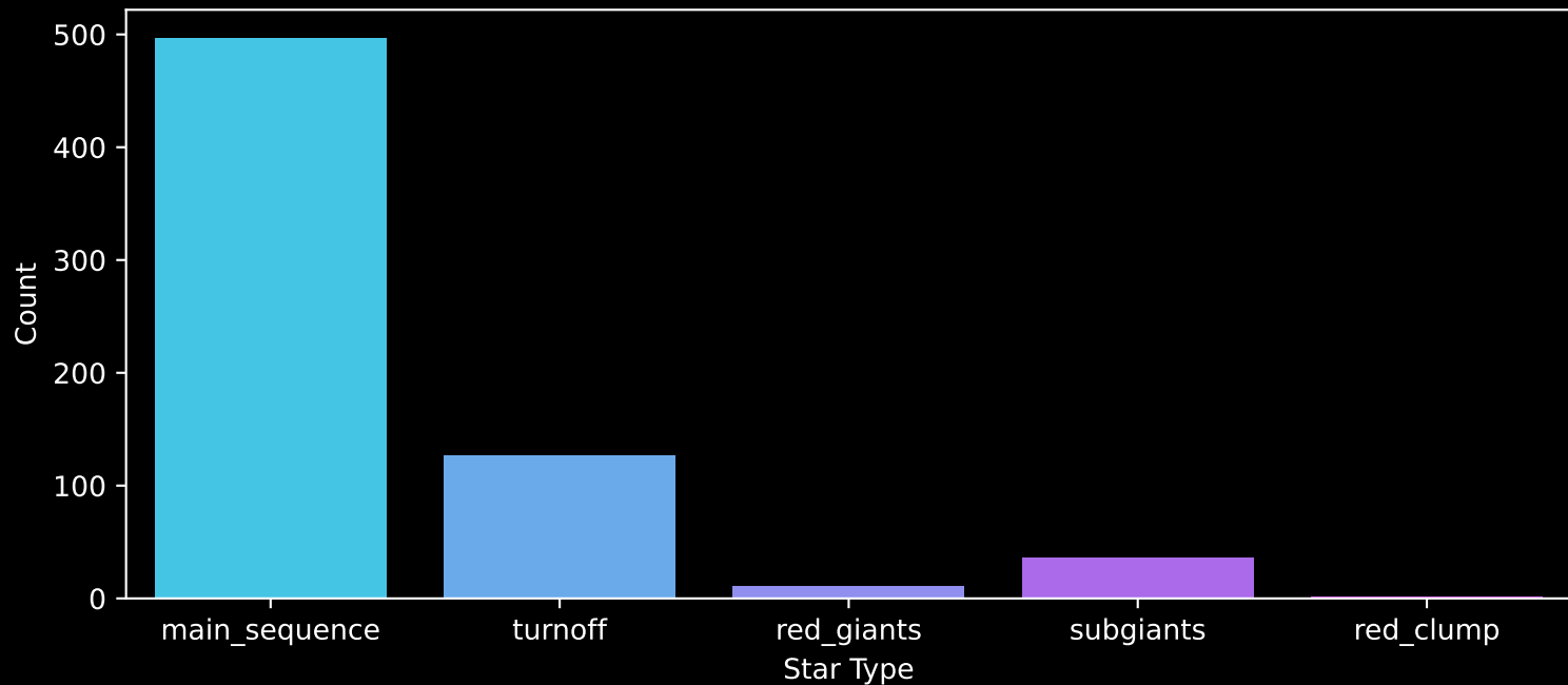
Gaia Cluster: [NGC_2112] Count plot of Star Type
