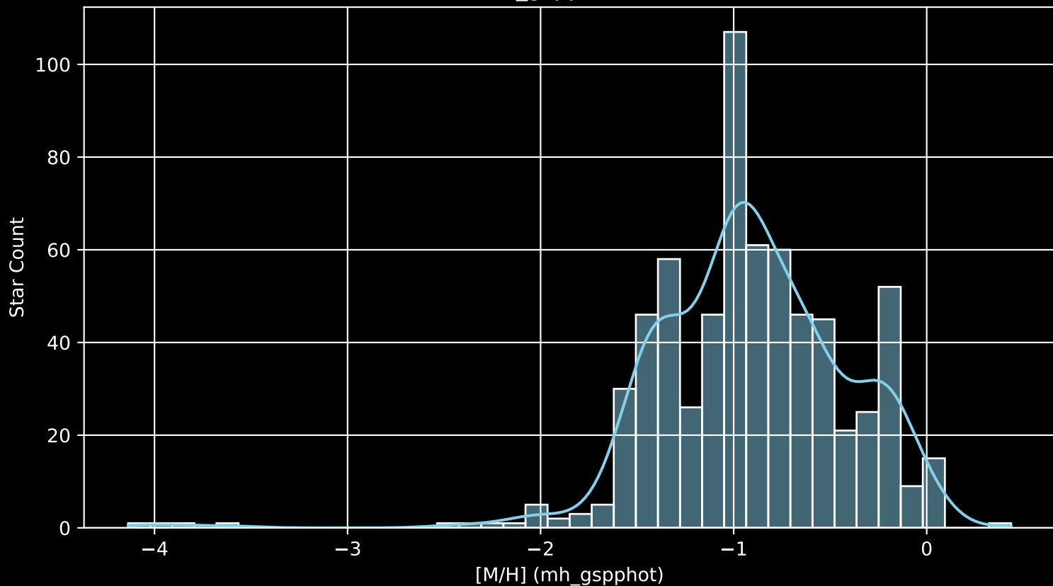
Gaia Cluster: [NGC_2112 [M/H] (mh_gspphot) (n= 671)
