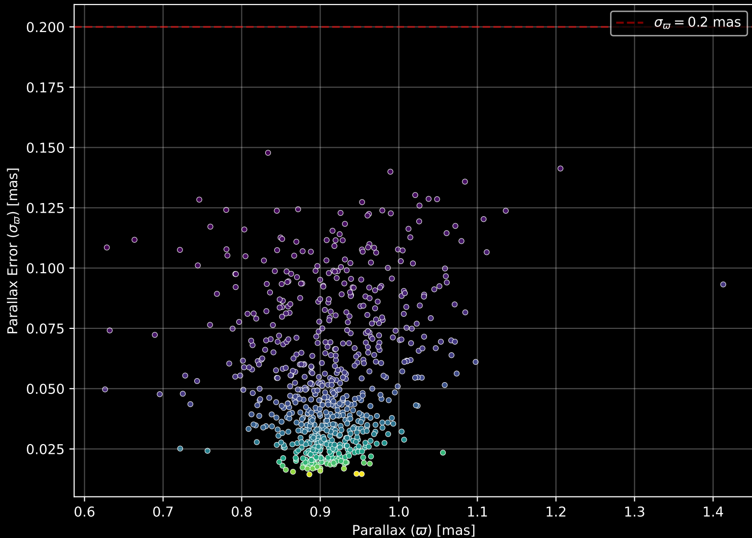
Gaia Cluster: [NGC_2112] Parallax Quality (n= 672)
