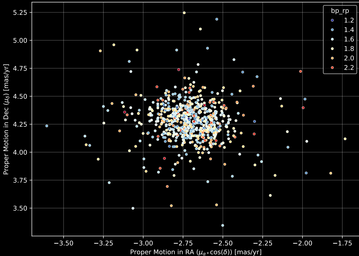
Gaia Cluster: [NGC_2112] Proper Motion Diagram (n= 672)
