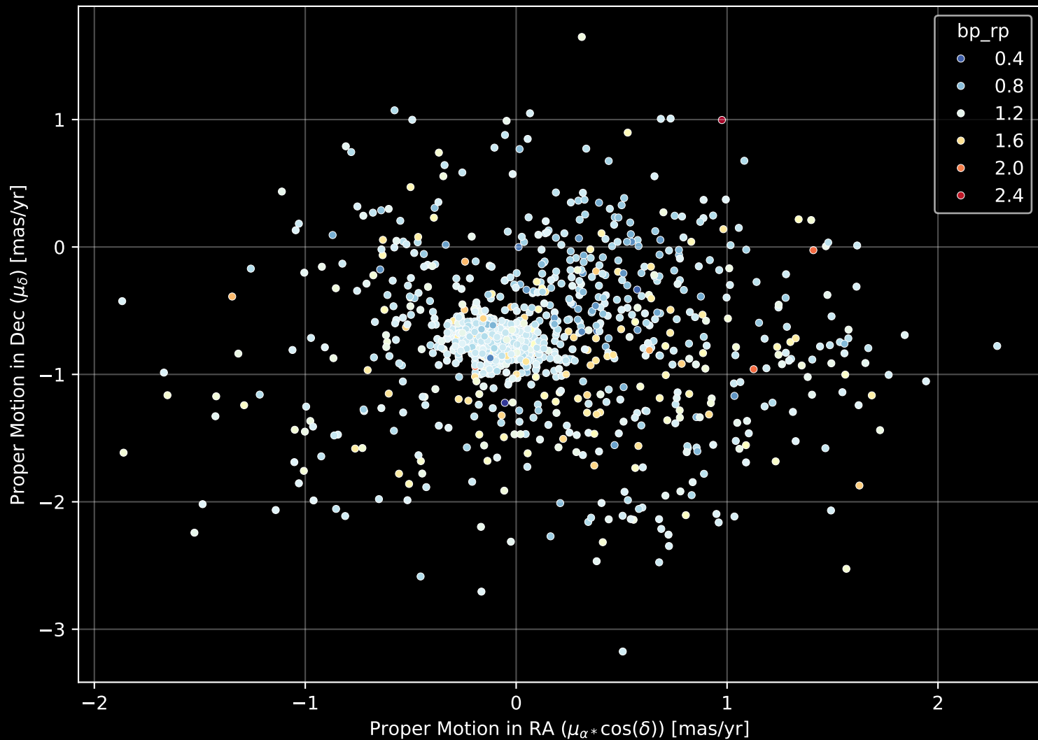
Gaia Cluster: [NGC_2141] Proper Motion Diagram (n= 1357)
