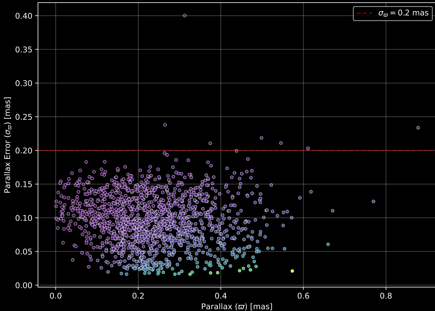
Gaia Cluster: [NGC_2141] Parallax Quality (n= 1357)
