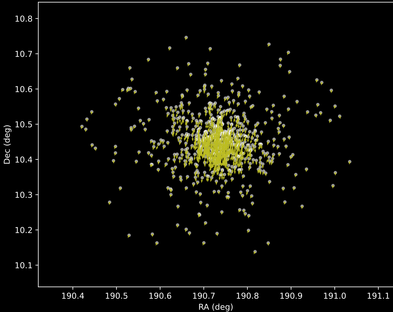
Gaia DR3 Cluster 36 Proper Motion Vectors (n=670)
