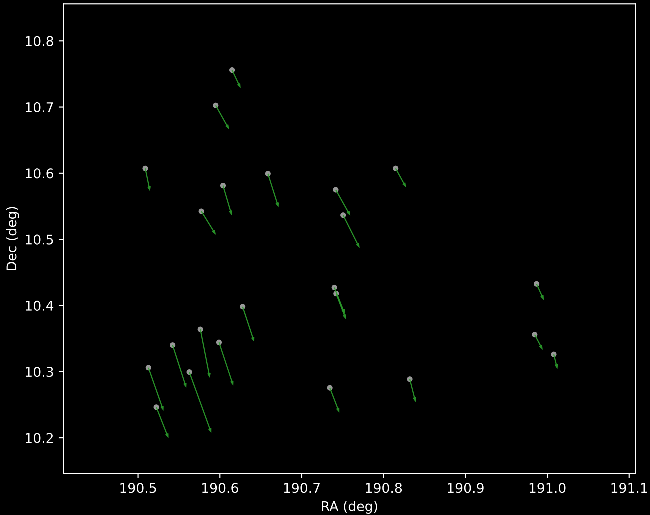
Gaia DR3 Cluster 4 Proper Motion Vectors (n=23)
