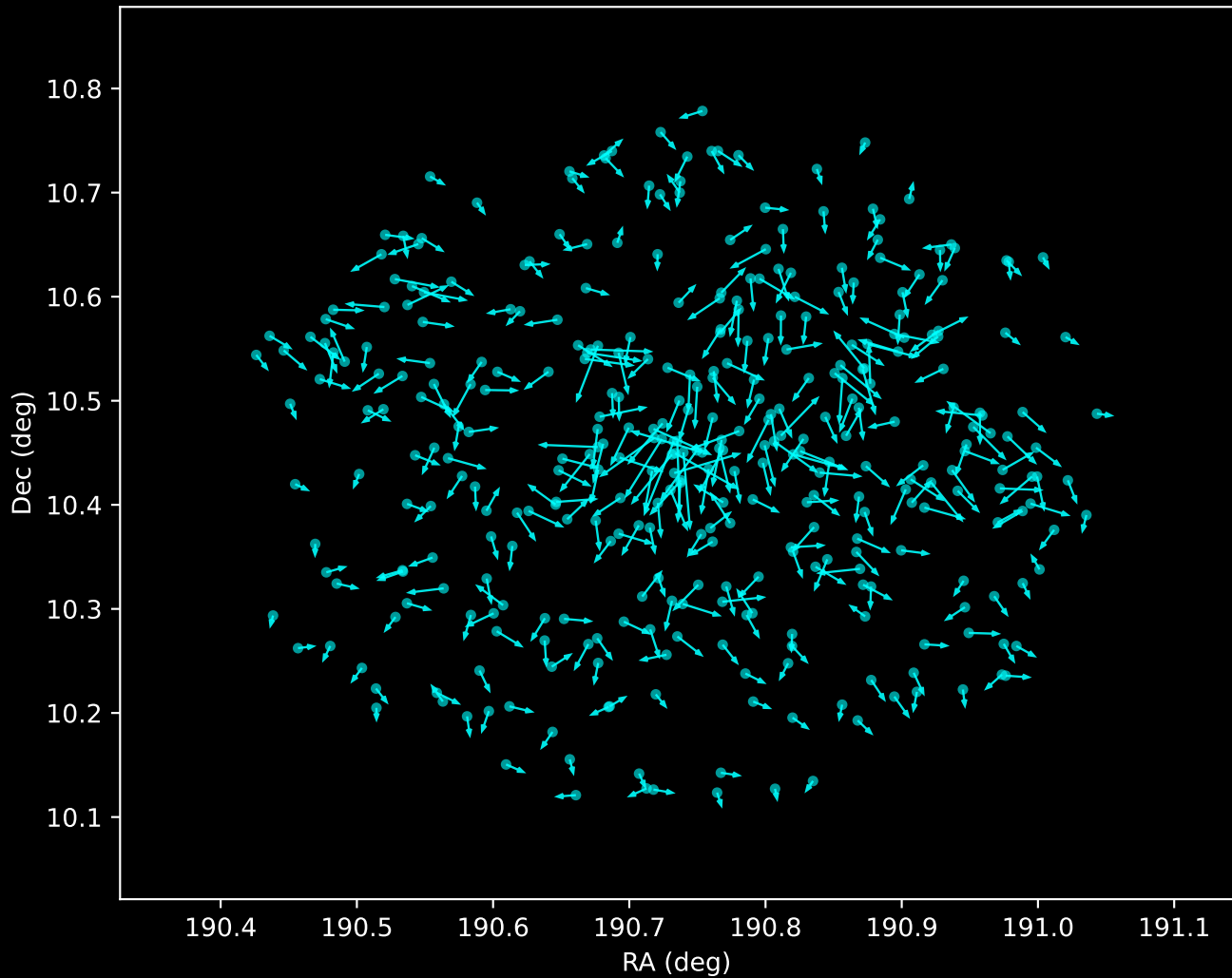
Gaia DR3 Noise Stream Proper Motion Vectors (n=358)
