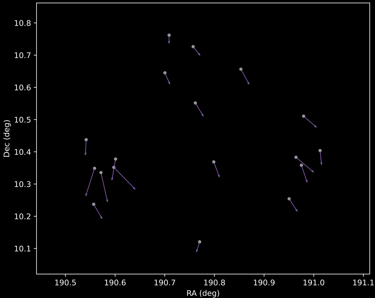
Gaia DR3 Cluster 28 Proper Motion Vectors (n=18)
