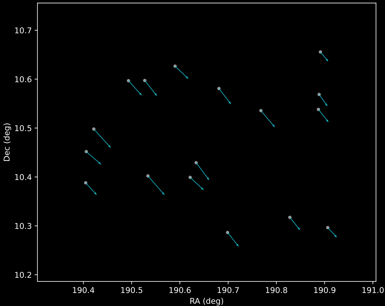
Gaia DR3 Cluster 18 Proper Motion Vectors (n=17)
