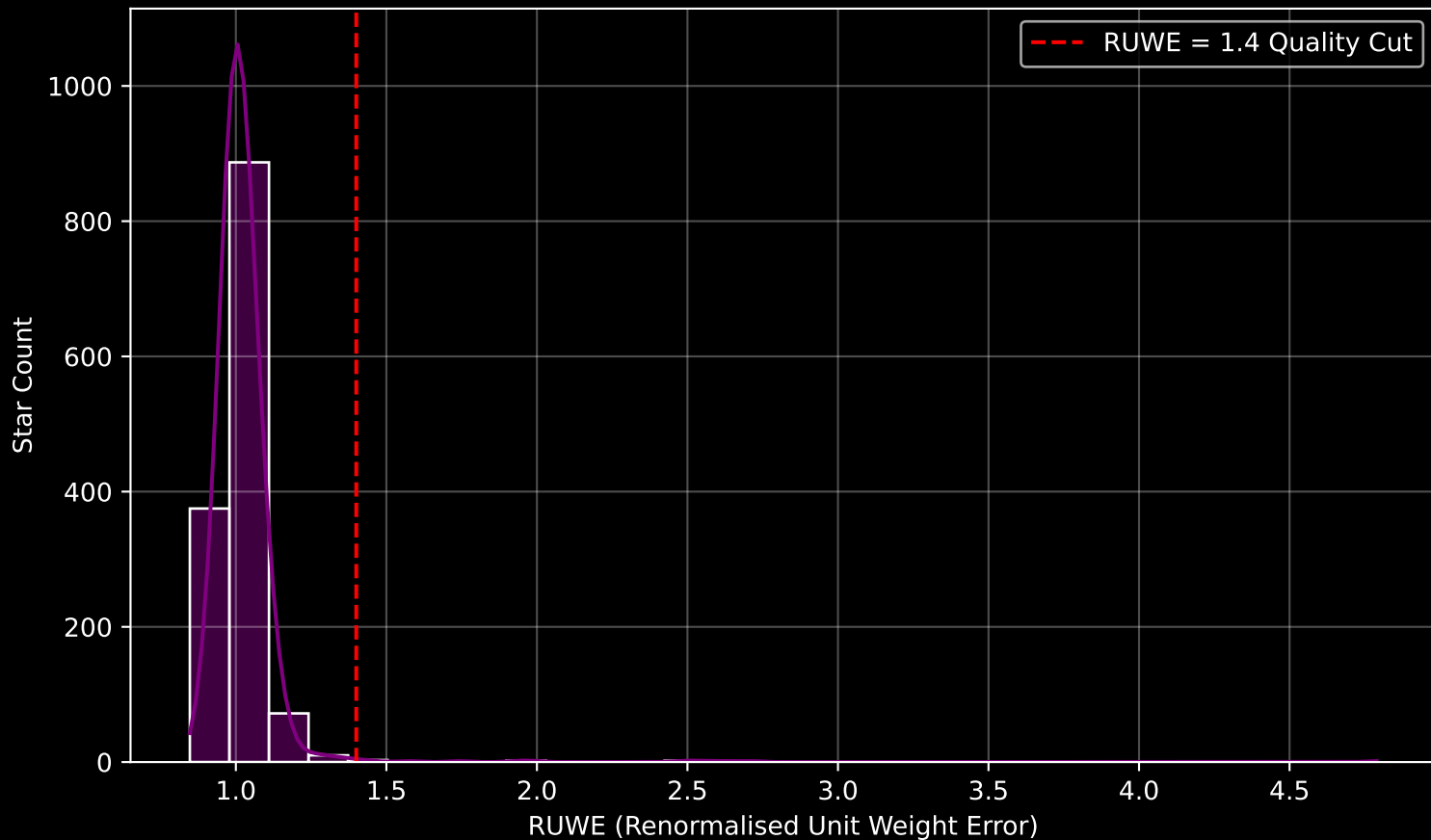
Gaia Cluster: [NGC_2141] RUWE Distribution (n= 1356)
