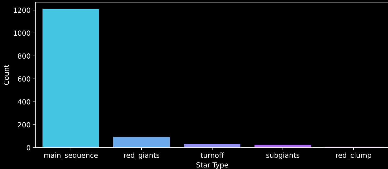
Gaia Cluster: [NGC_2141] Count plot of Star Type
