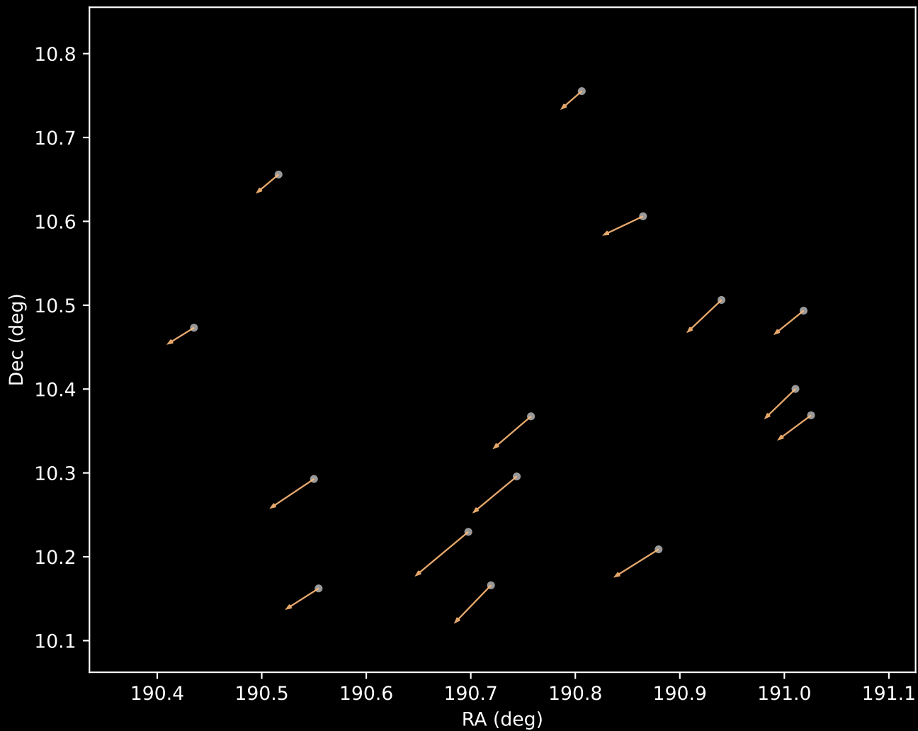
Gaia DR3 Cluster 23 Proper Motion Vectors (n=15)
