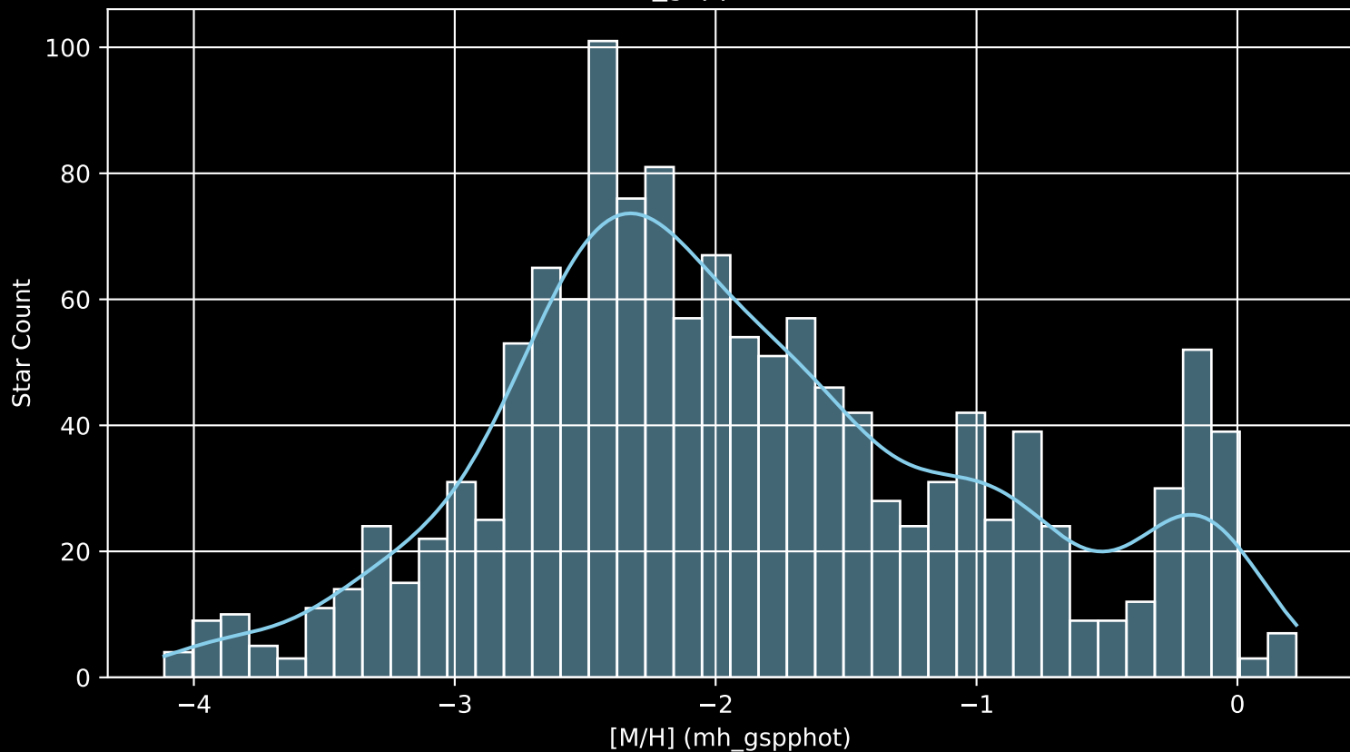
Gaia Cluster: [NGC_2141 [M/H] (mh_gspphot) (n= 1357)
