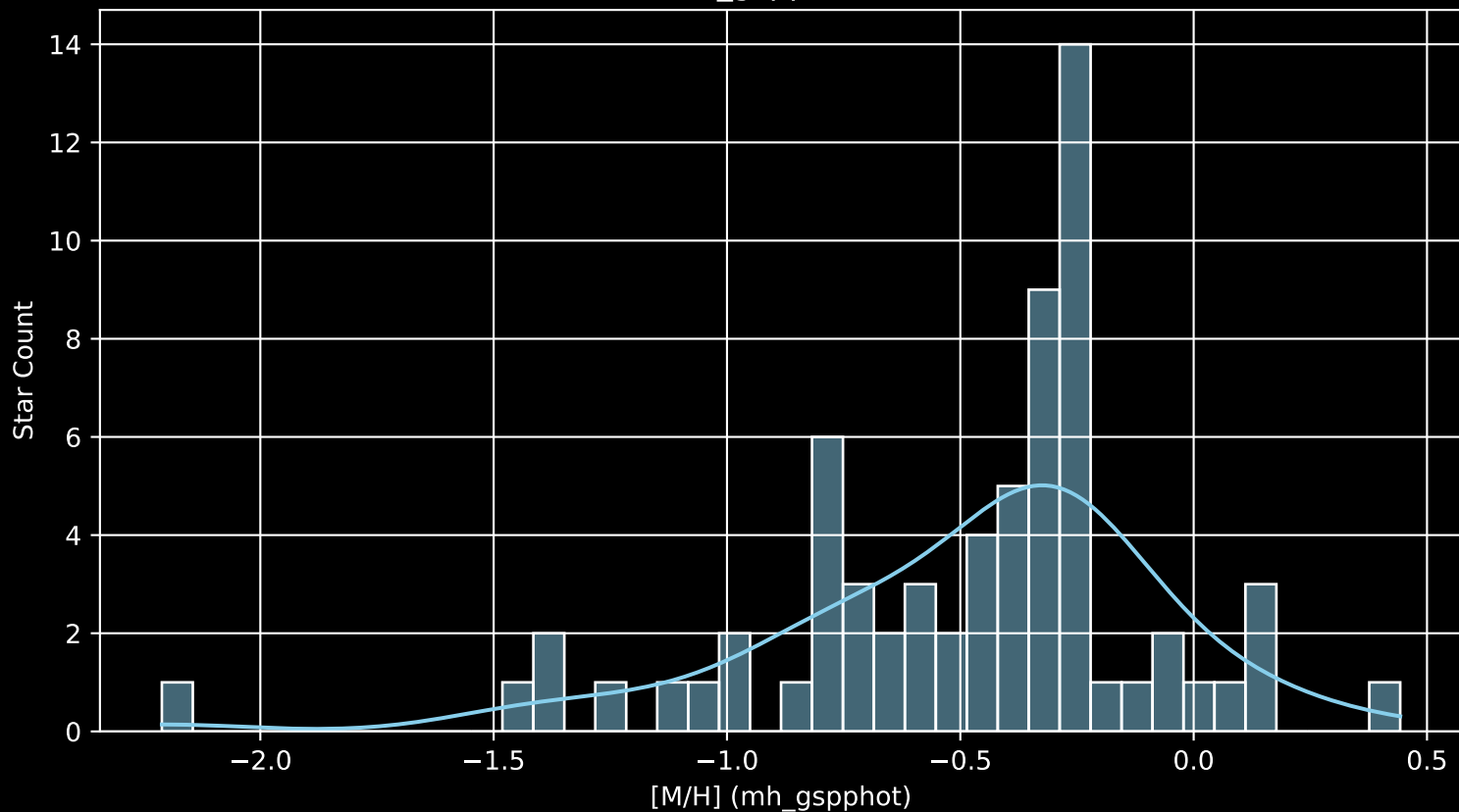
Gaia Cluster: [NGC_2183 [M/H] (mh_gspphot) (n= 68)
