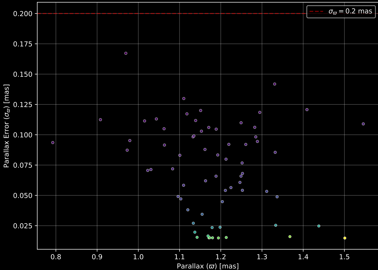
Gaia Cluster: [NGC_2183] Parallax Quality (n= 68)
