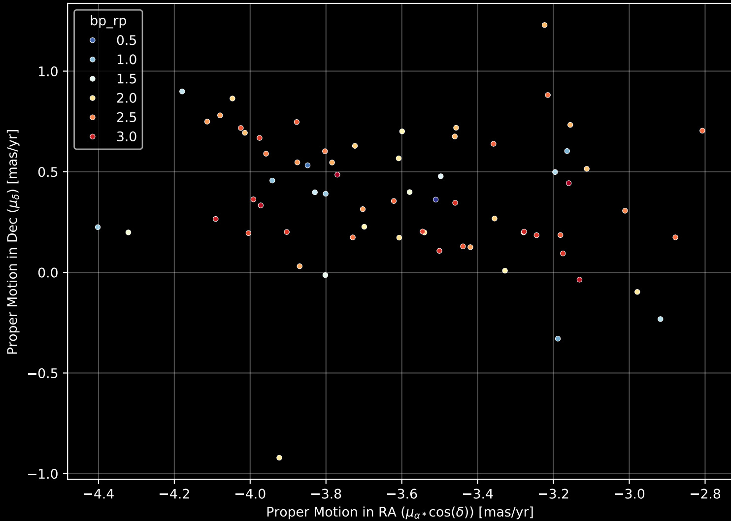
Gaia Cluster: [NGC_2183] Proper Motion Diagram (n= 68)
