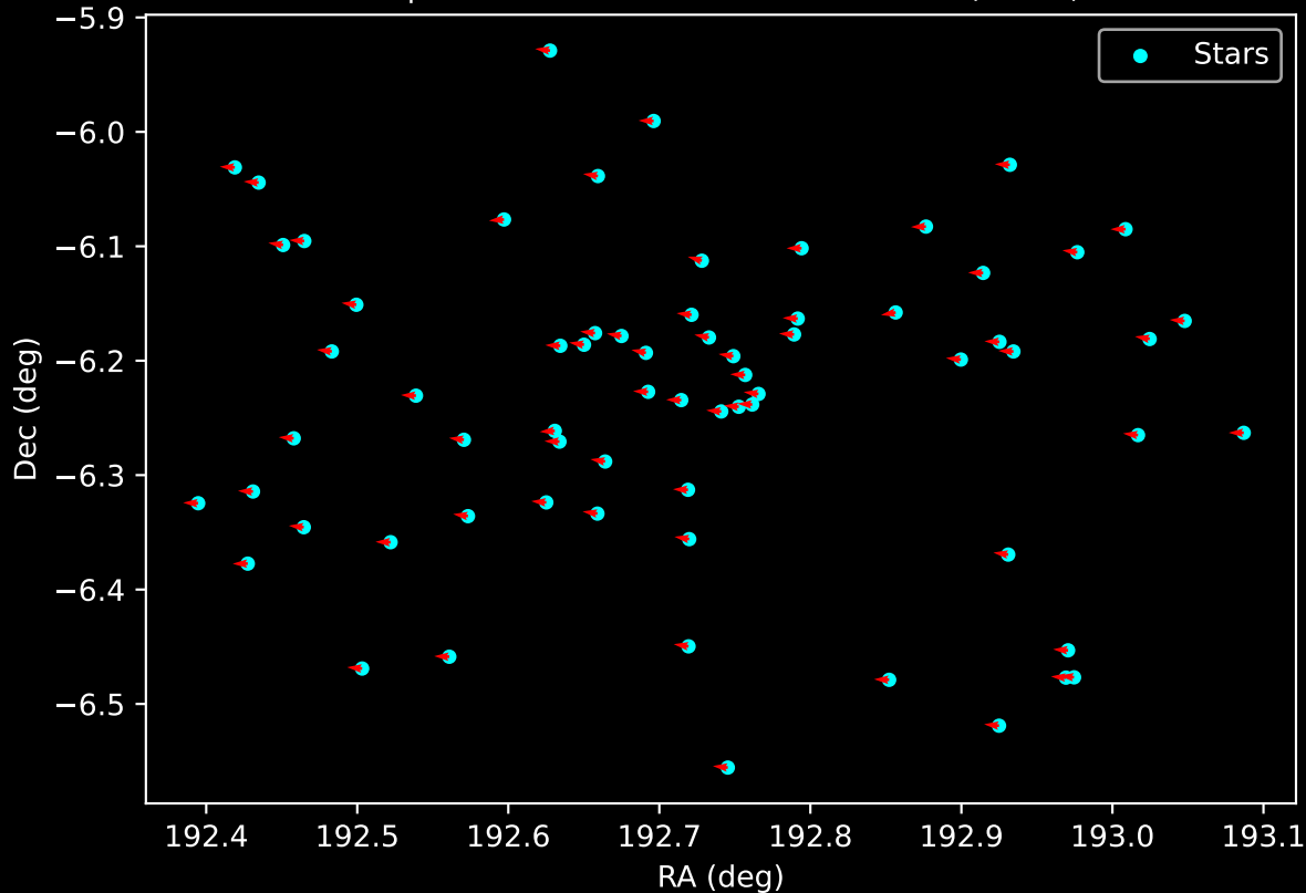
Gaia Cluster: [NGC_2183] Proper Motion Vectors for Gaia Star Field (n= 68)
