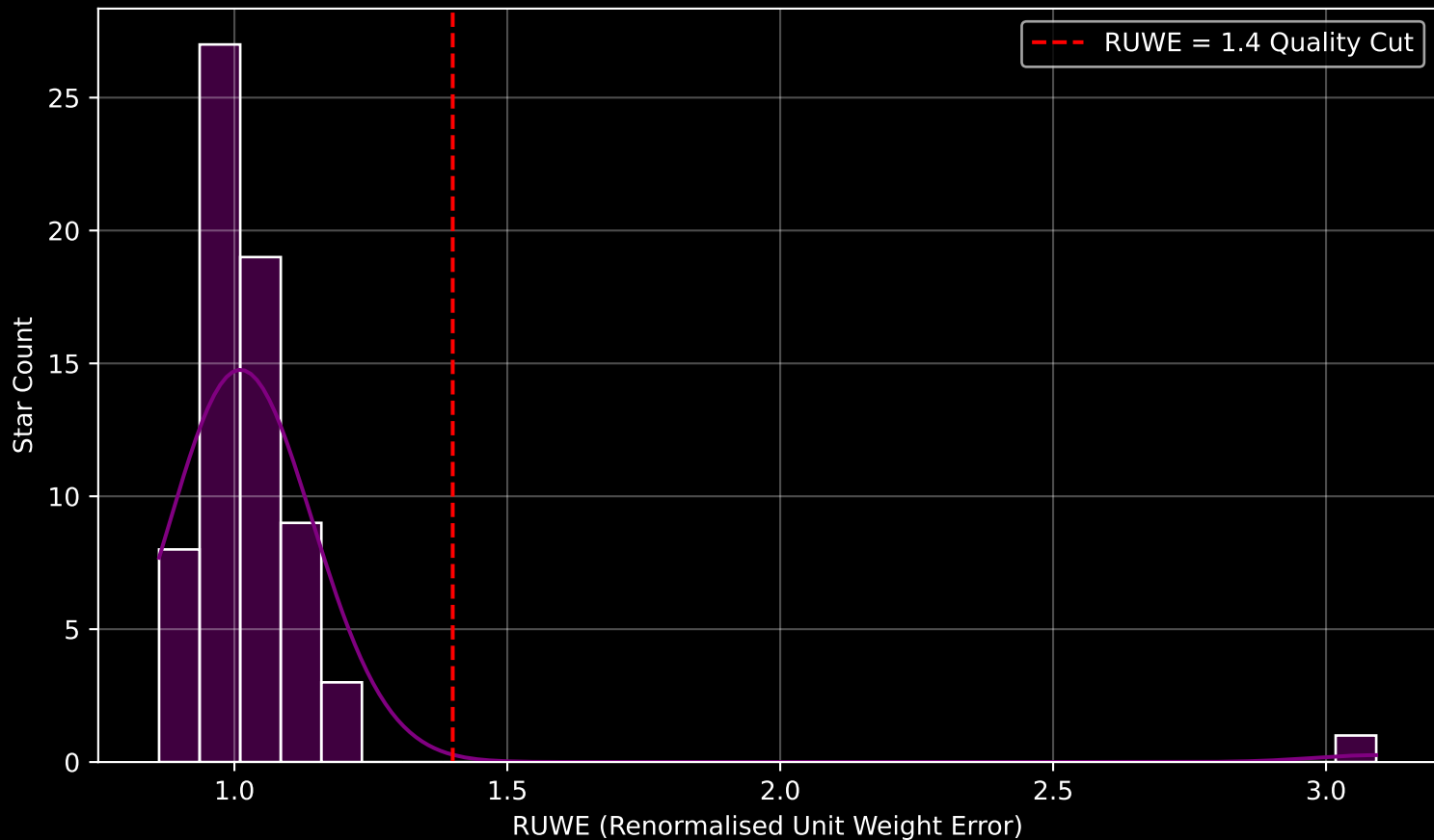
Gaia Cluster: [NGC_2183] RUWE Distribution (n= 67)
