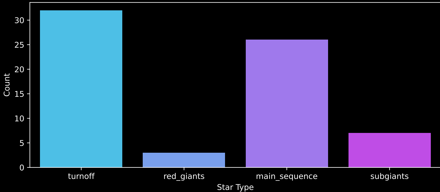
Gaia Cluster: [NGC_2183] Count plot of Star Type
