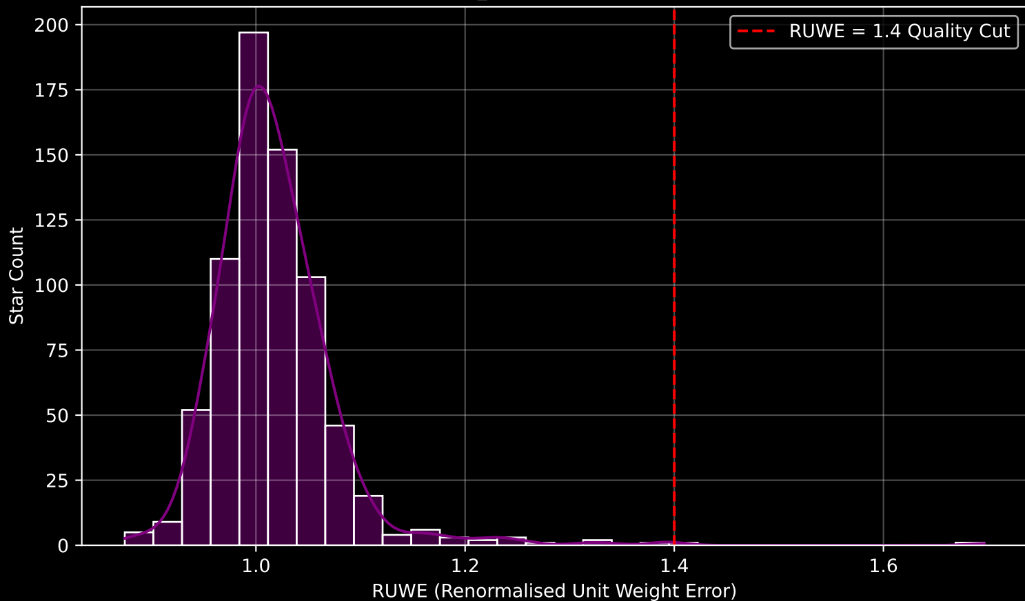
Gaia Cluster: [NGC_2204] RUWE Distribution (n= 717)
