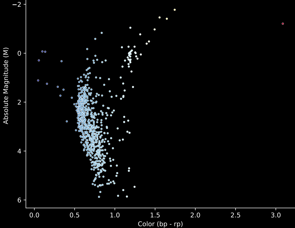
Gaia Cluster: [NGC 2204] Stars (n= 717) Hertzsprung-Russel Diagram
