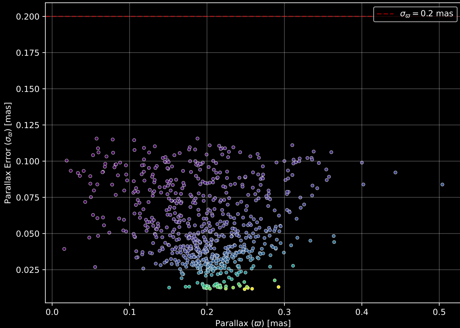
Gaia Cluster: [NGC_2204] Parallax Quality (n= 717)
