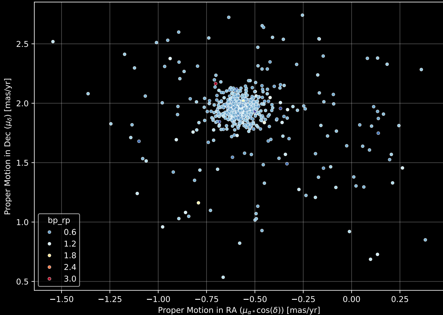
Gaia Cluster: [NGC_2204] Proper Motion Diagram (n= 717)
