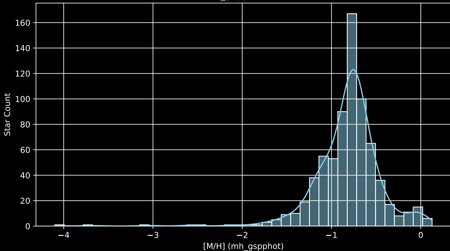
Gaia Cluster: [NGC_2204 [M/H] (mh_gspphot) (n= 716)
