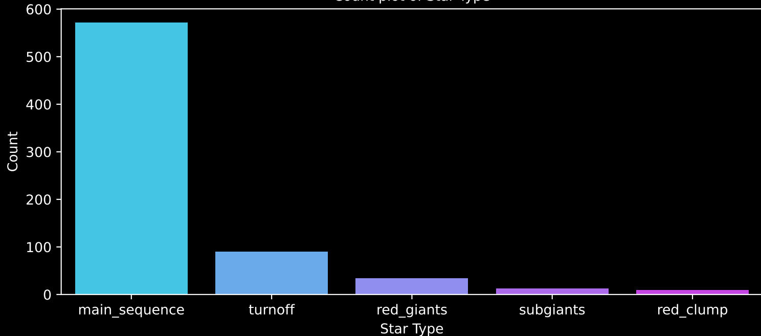
Gaia Cluster: [NGC_2204] Count plot of Star Type
