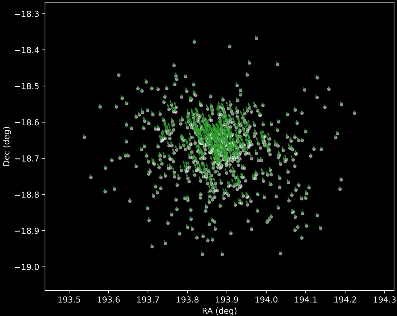
Gaia DR3 Cluster 4 Proper Motion Vectors (n=626)
