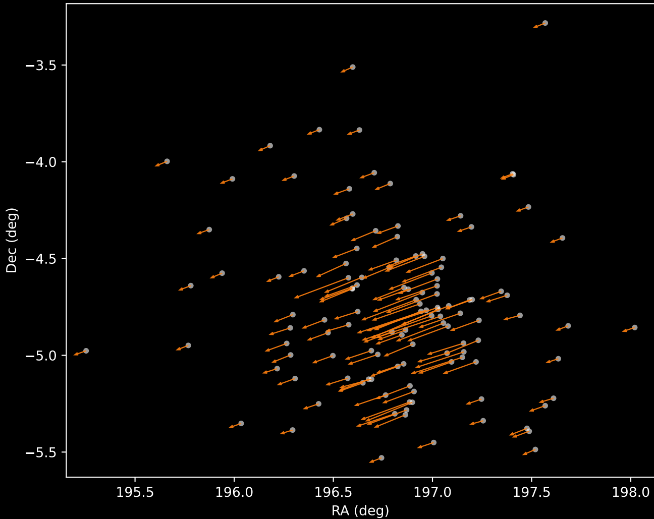
Gaia DR3 Cluster 2 Proper Motion Vectors (n=121)
