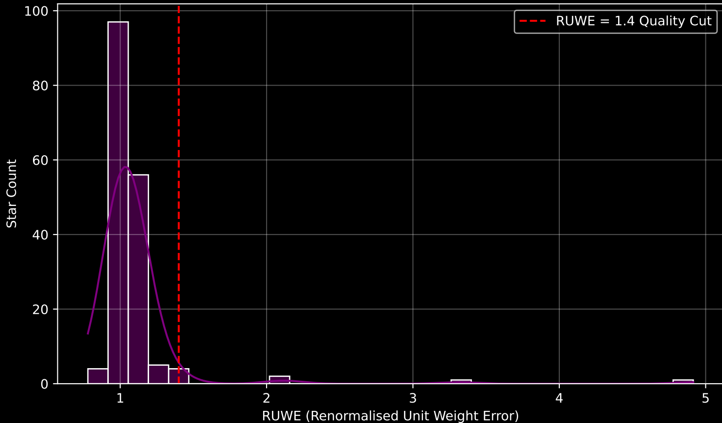
Gaia Cluster: [NGC_2232] RUWE Distribution (n= 170)
