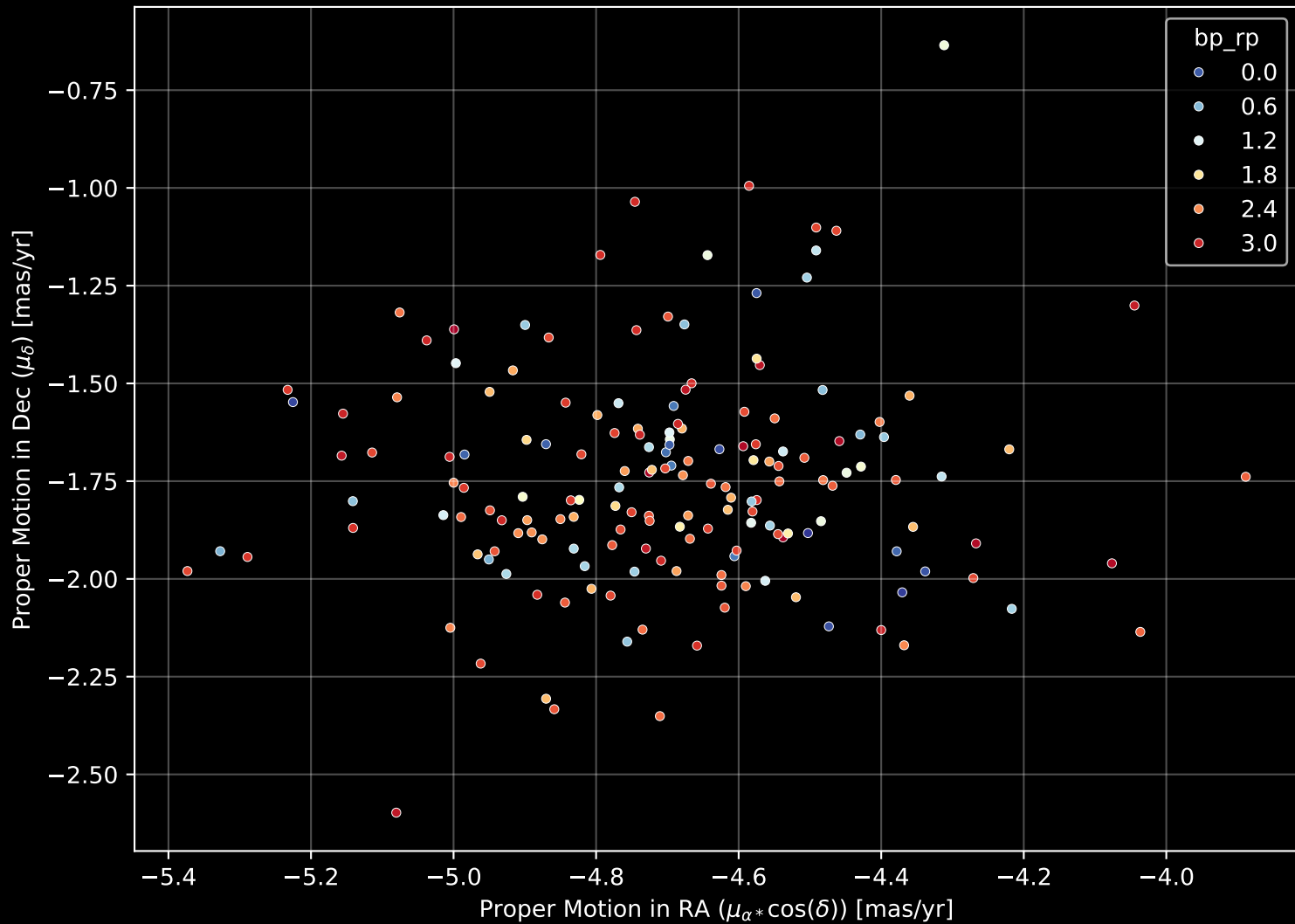
Gaia Cluster: [NGC_2232] Proper Motion Diagram (n= 171)
