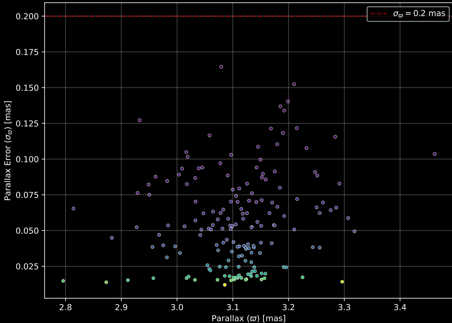
Gaia Cluster: [NGC_2232] Parallax Quality (n= 171)
