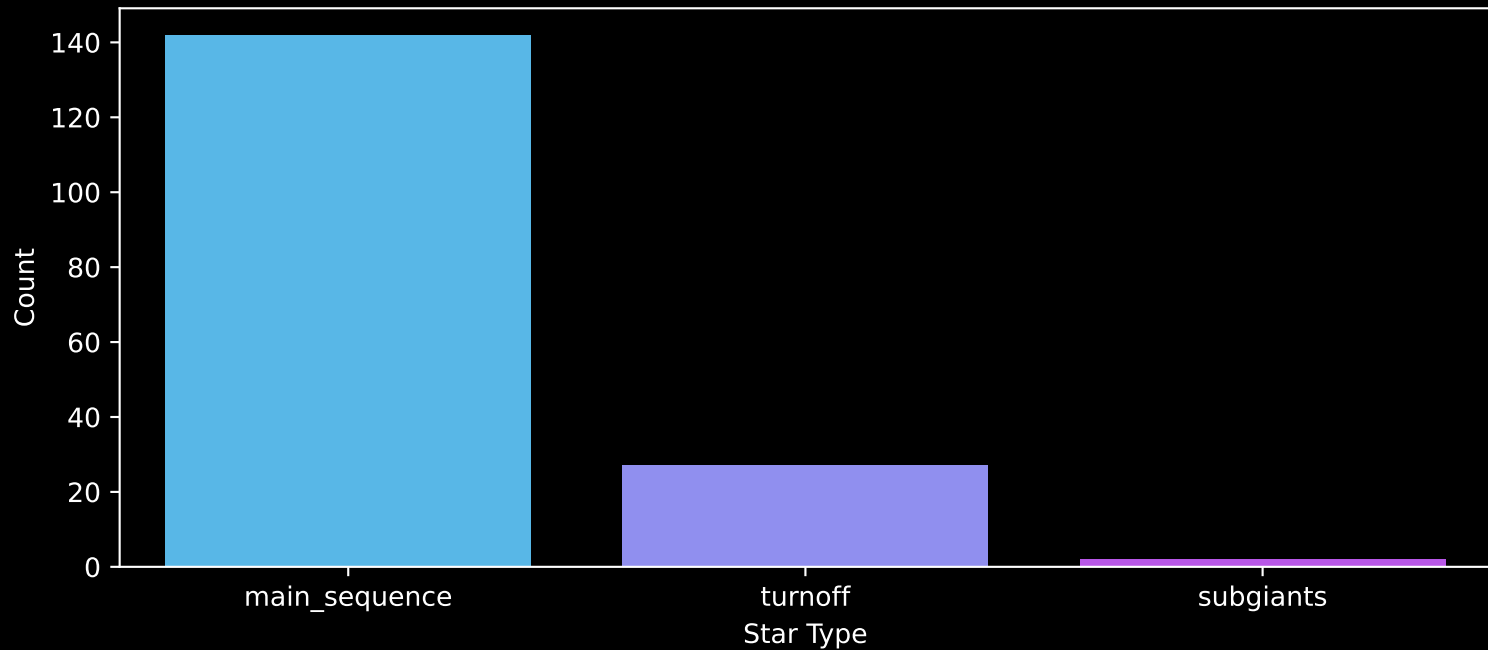
Gaia Cluster: [NGC_2232] Count plot of Star Type
