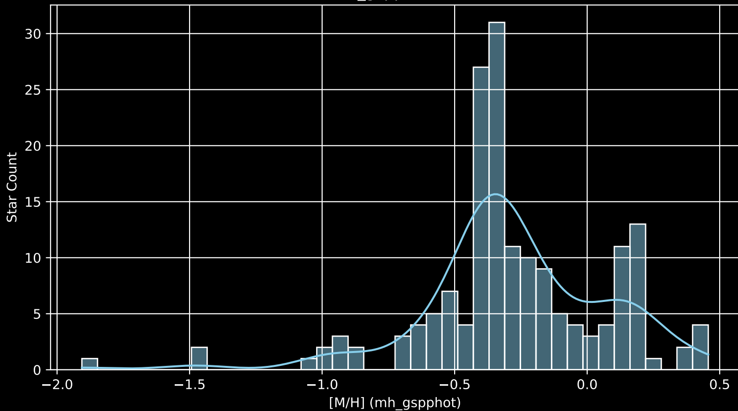
Gaia Cluster: [NGC_2232 [M/H] (mh_gspphot) (n= 169)
