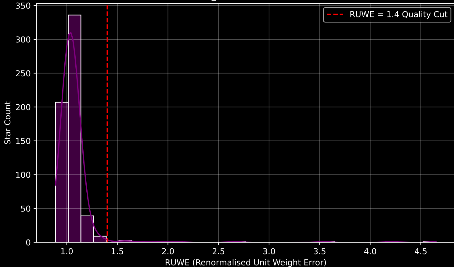
Gaia Cluster: [NGC_2236] RUWE Distribution (n= 601)
