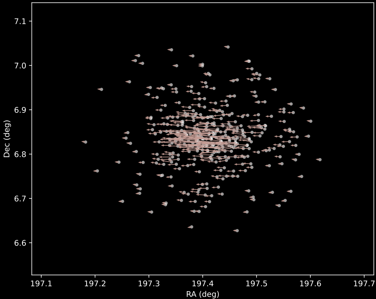
Gaia DR3 Cluster 11 Proper Motion Vectors (n=358)
