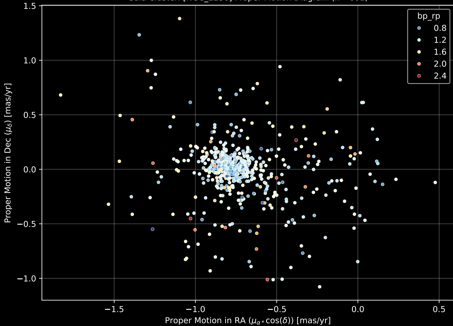
Gaia Cluster: [NGC_2236] Proper Motion Diagram (n= 601)
