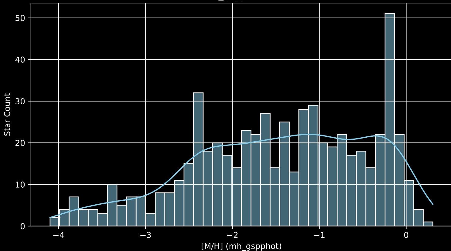
Gaia Cluster: [NGC_2236 [M/H] (mh_gspphot) (n= 601)
