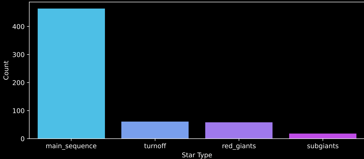
Gaia Cluster: [NGC_2236] Count plot of Star Type
