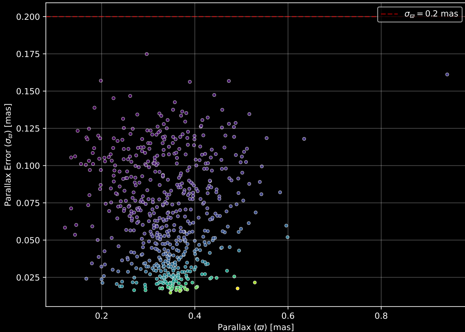
Gaia Cluster: [NGC_2236] Parallax Quality (n= 601)
