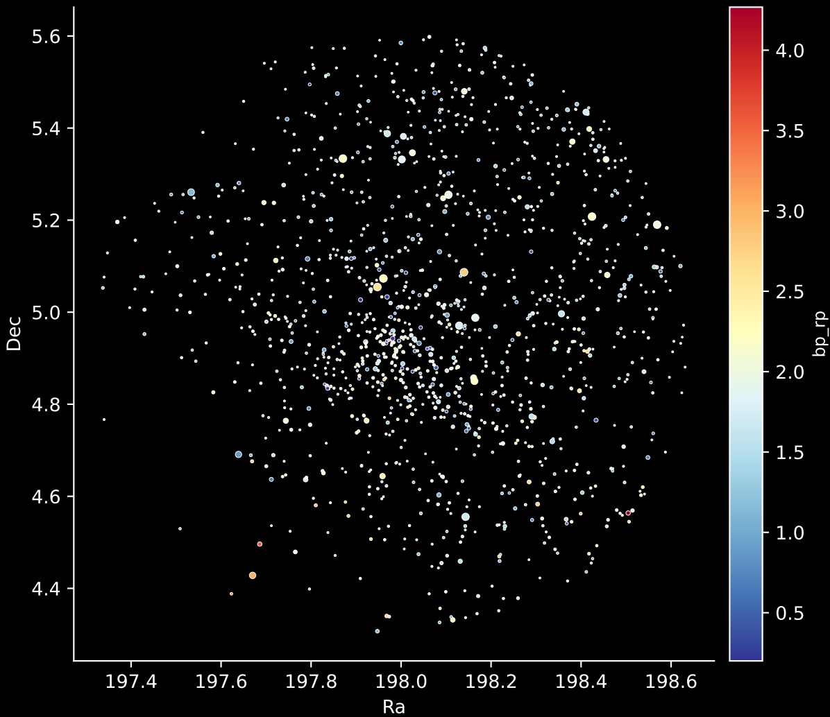
Gaia Cluster: [NGC_2244] Stars: 1320
