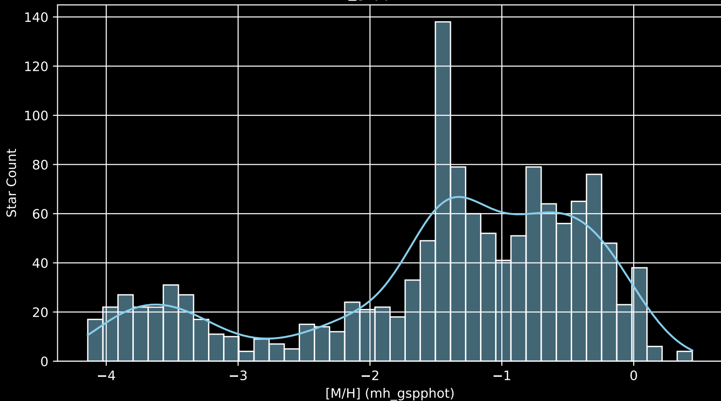
Gaia Cluster: [NGC_2244 [M/H] (mh_gspphot) (n= 1319)
