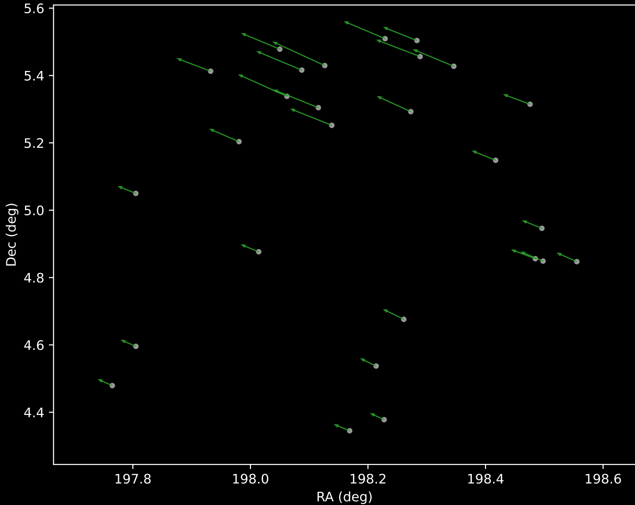
Gaia DR3 Cluster 44 Proper Motion Vectors (n=27)
