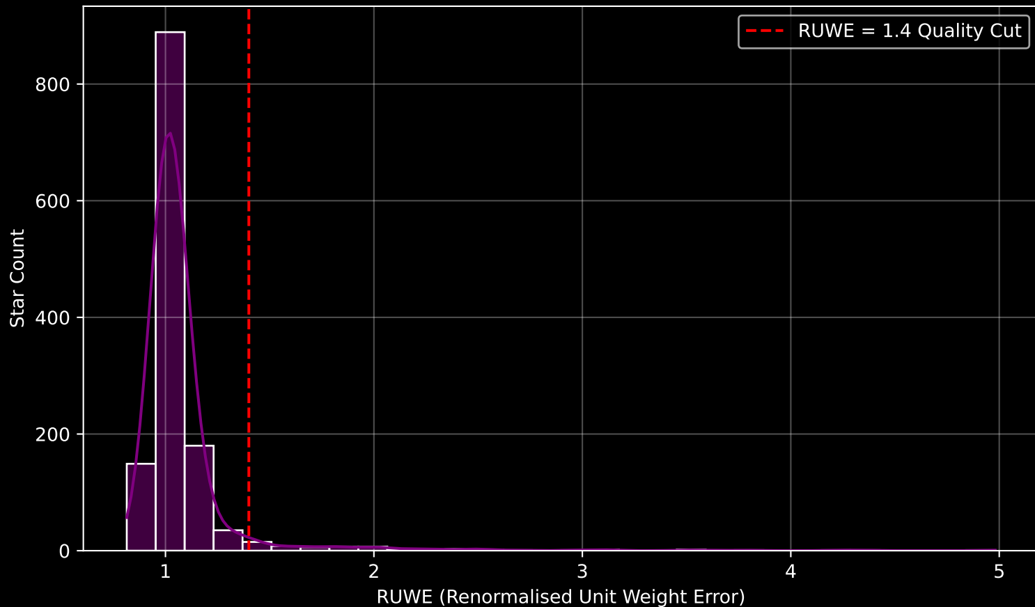
Gaia Cluster: [NGC_2244] RUWE Distribution (n= 1316)
