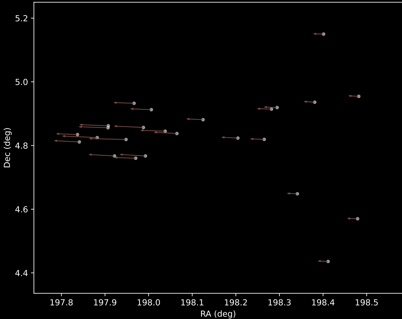
Gaia DR3 Cluster 70 Proper Motion Vectors (n=25)
