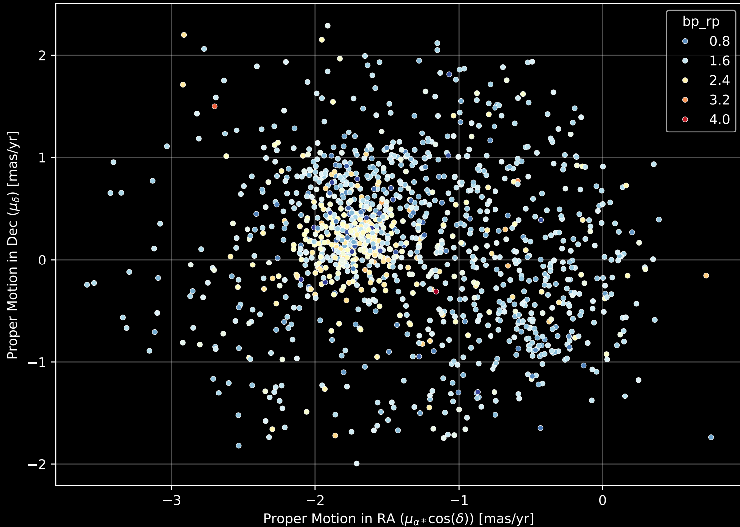
Gaia Cluster: [NGC_2244] Proper Motion Diagram (n= 1320)
