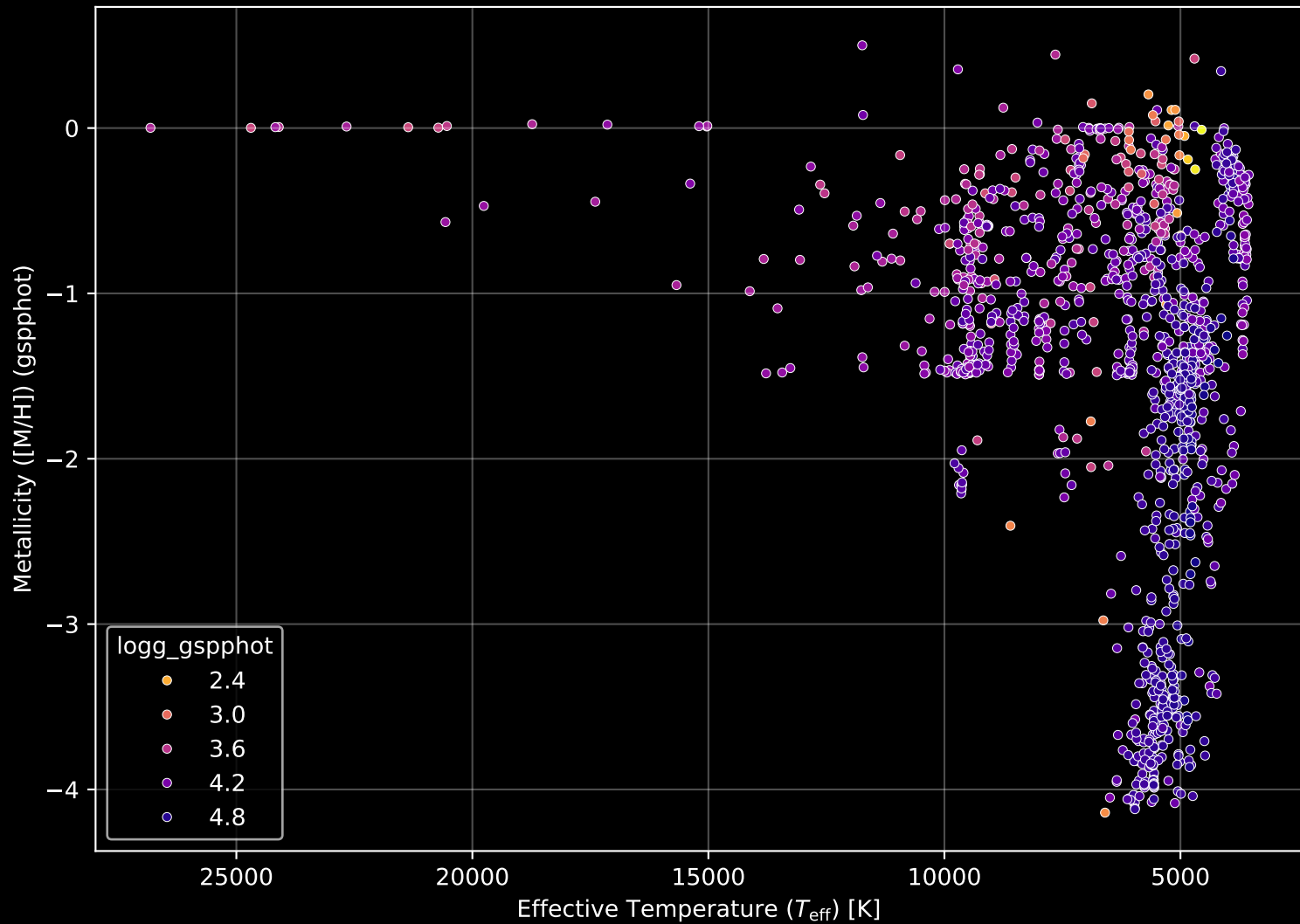
Gaia Cluster: [NGC_2244] Stellar Population Parameters (n= 1320)
