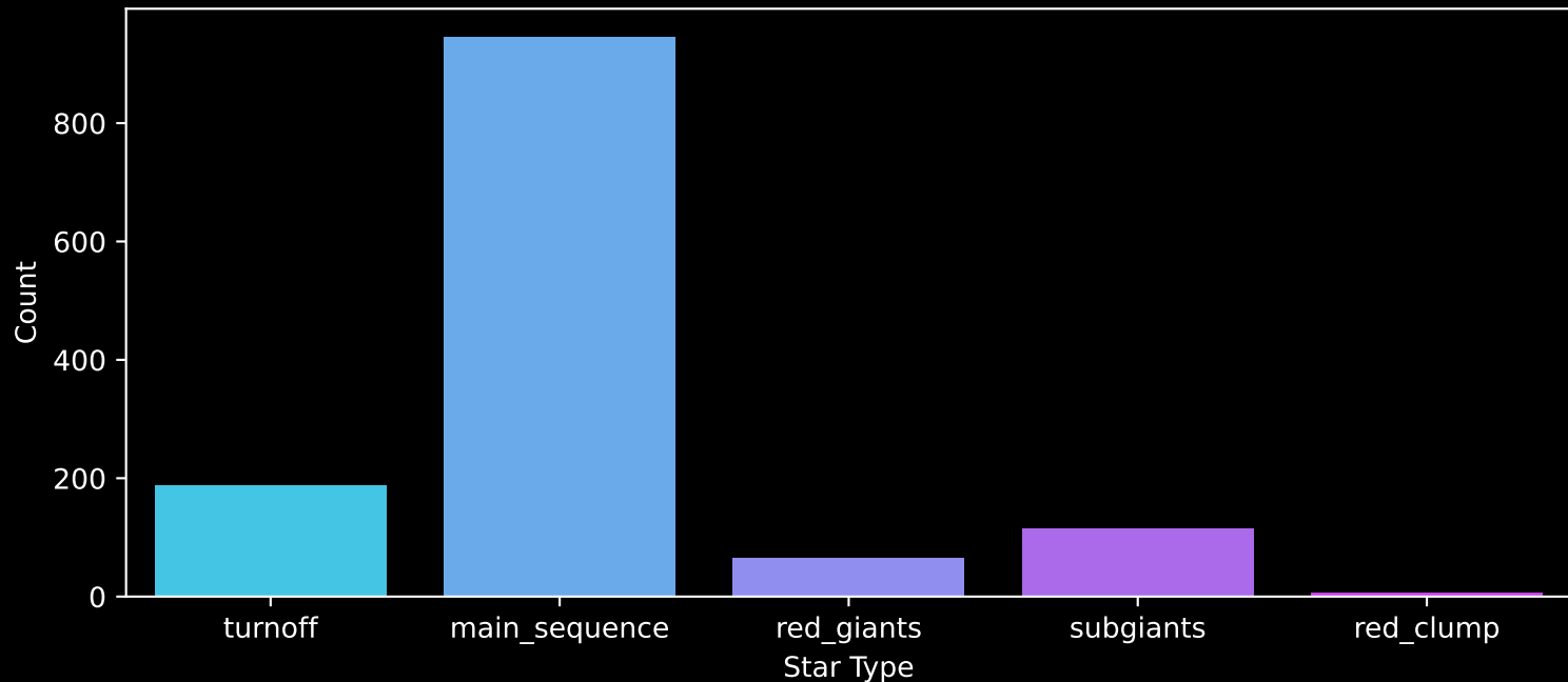
Gaia Cluster: [NGC_2244] Count plot of Star Type
