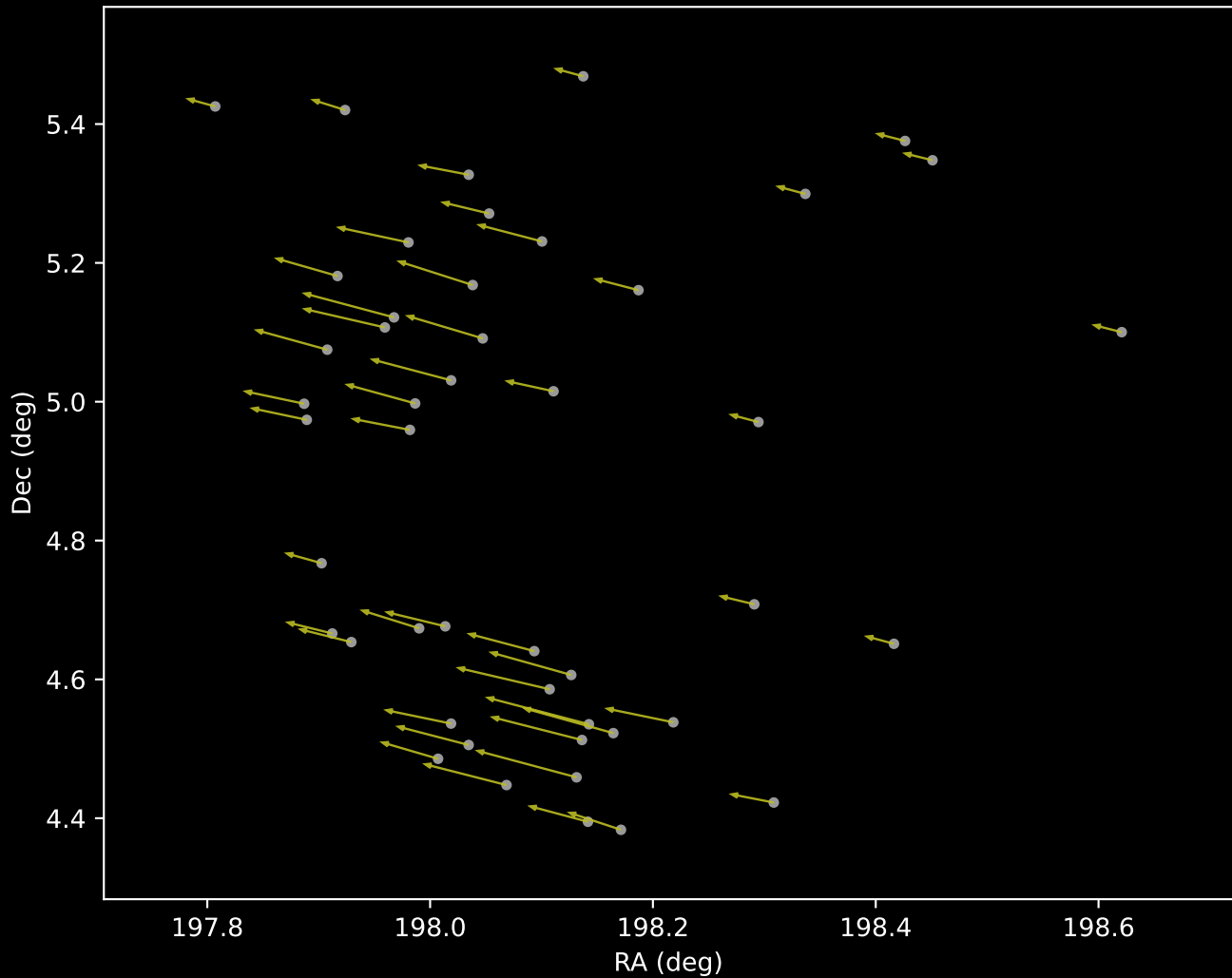
Gaia DR3 Cluster 56 Proper Motion Vectors (n=47)
