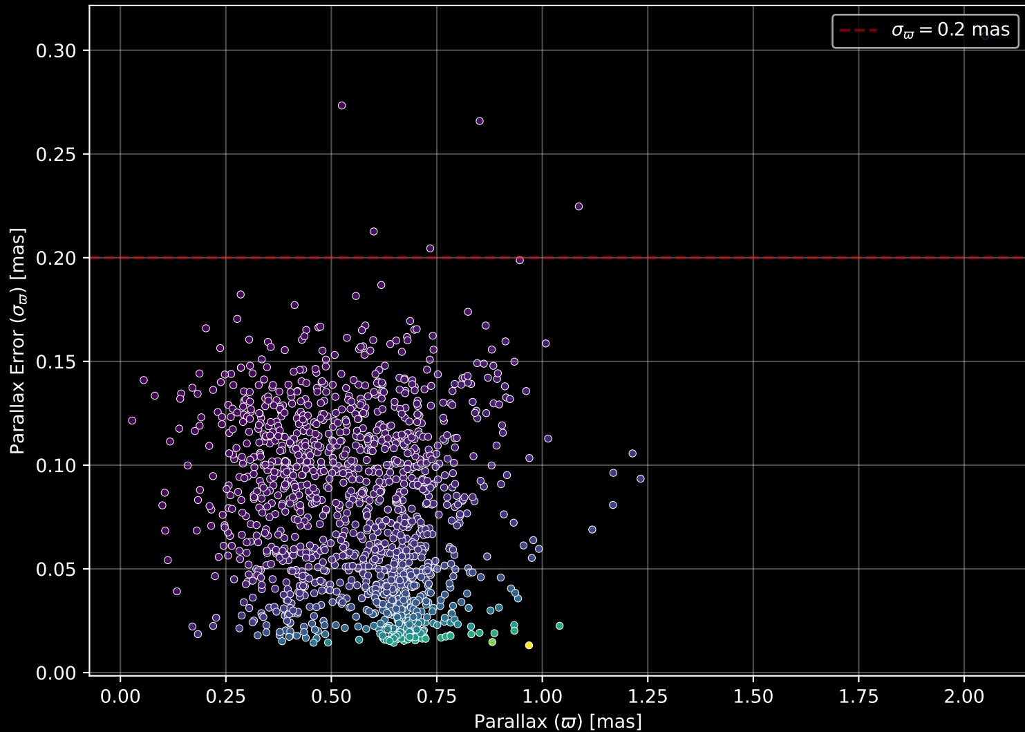
Gaia Cluster: [NGC_2244] Parallax Quality (n= 1320)
