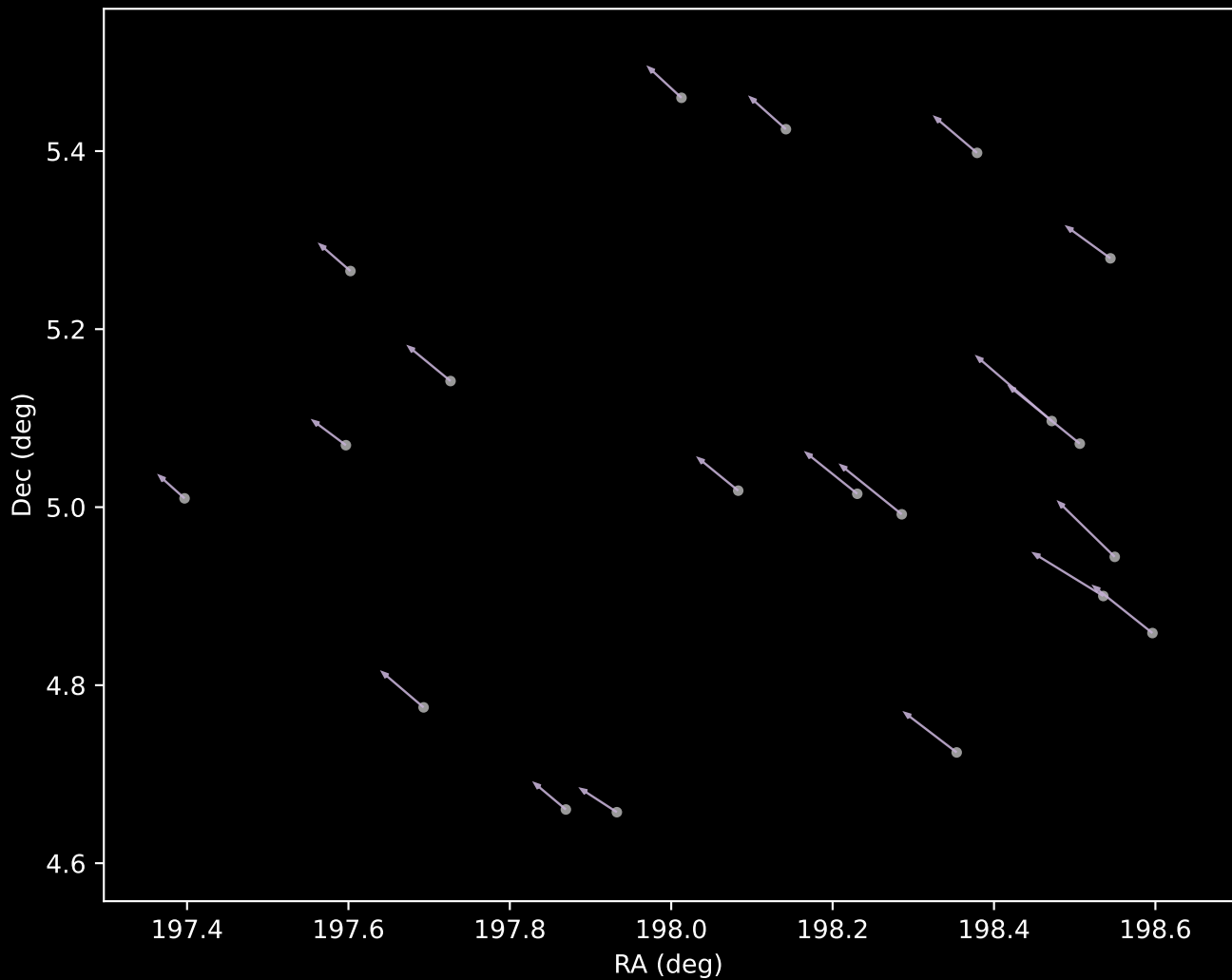
Gaia DR3 Cluster 29 Proper Motion Vectors (n=20)
