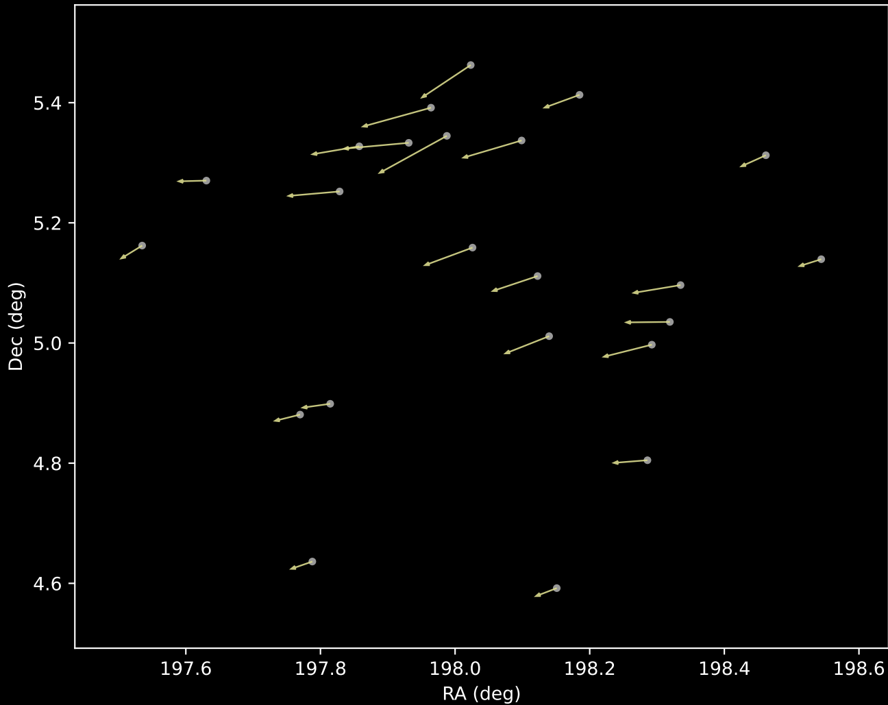
Gaia DR3 Cluster 37 Proper Motion Vectors (n=23)
