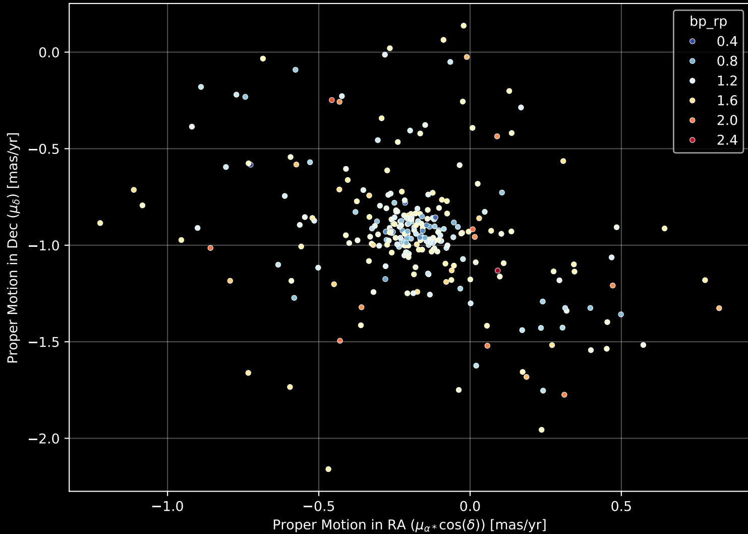
Gaia Cluster: [NGC_2254] Proper Motion Diagram (n= 277)
