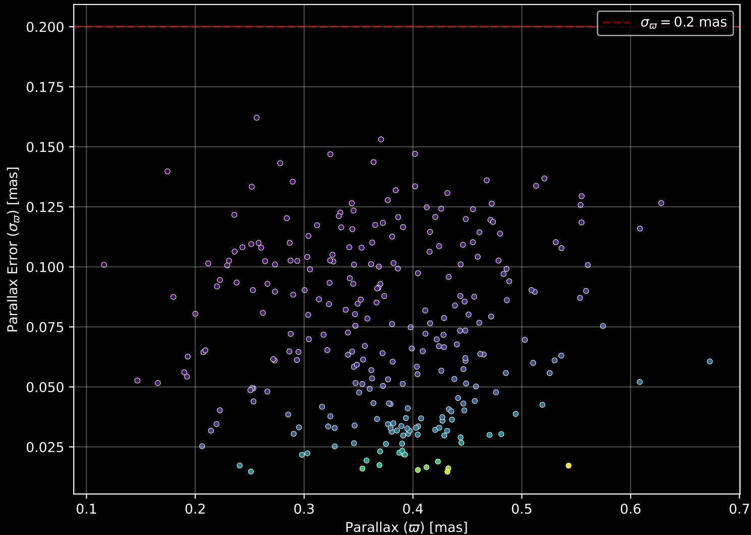
Gaia Cluster: [NGC_2254] Parallax Quality (n= 277)
