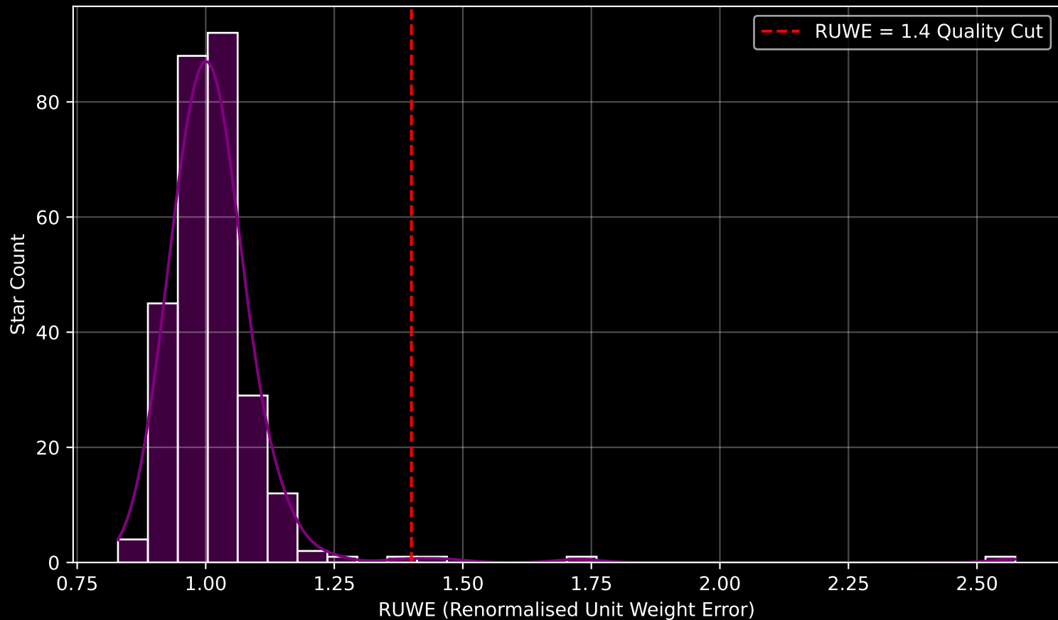
Gaia Cluster: [NGC_2254] RUWE Distribution (n= 277)
