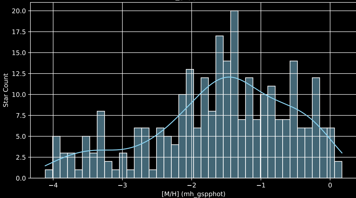
Gaia Cluster: [NGC_2254 [M/H] (mh_gspphot) (n= 277)
