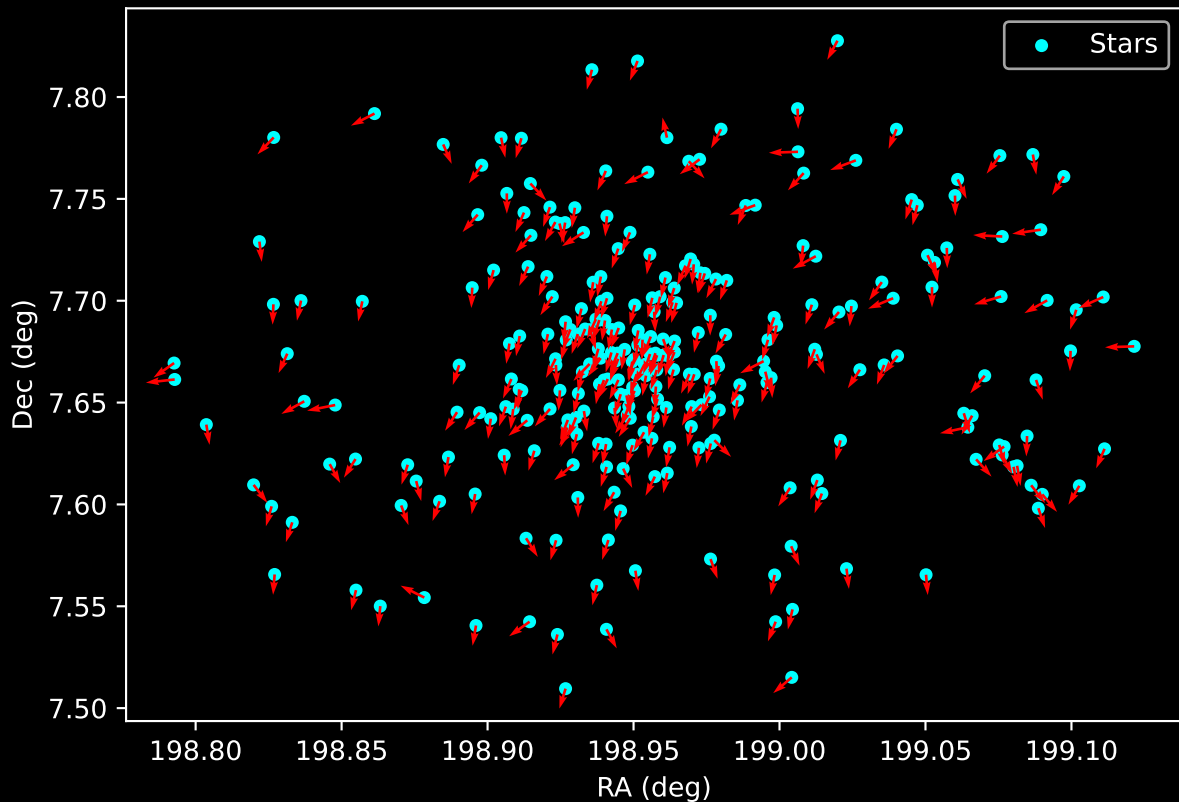
Gaia Cluster: [NGC_2254] Proper Motion Vectors for Gaia Star Field (n= 277)
