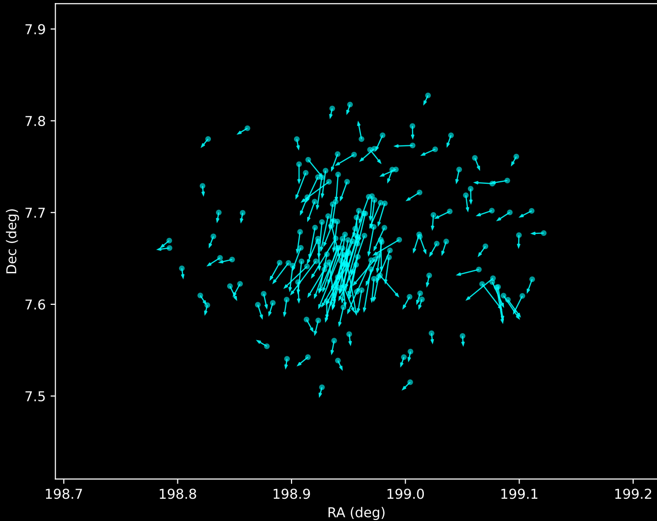
Gaia DR3 Noise Stream Proper Motion Vectors (n=170)
