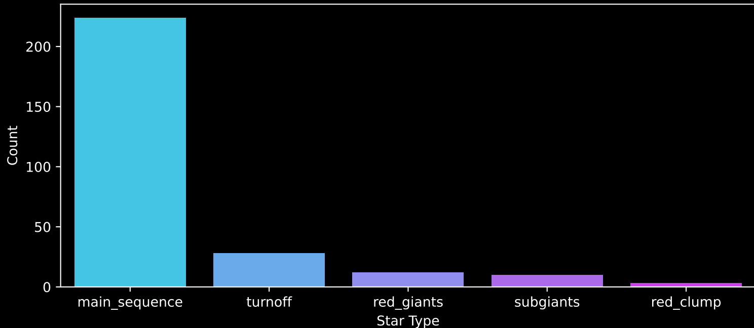
Gaia Cluster: [NGC_2254] Count plot of Star Type
