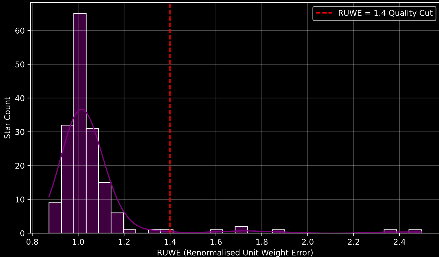
Gaia Cluster: [NGC_2259] RUWE Distribution (n= 167)
