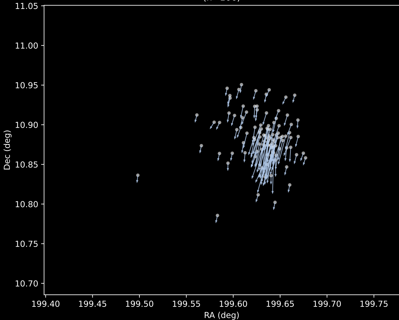
Gaia DR3 Cluster 1 Proper Motion Vectors (n=106)
