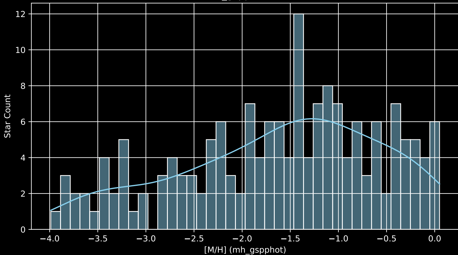
Gaia Cluster: [NGC_2259 [M/H] (mh_gspphot) (n= 167)
