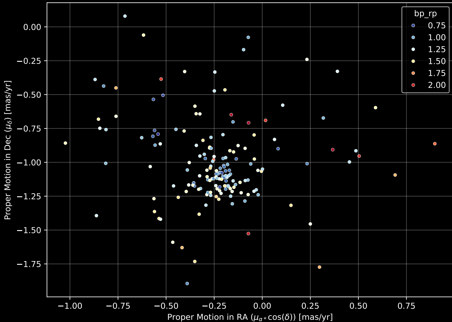
Gaia Cluster: [NGC_2259] Proper Motion Diagram (n= 167)
