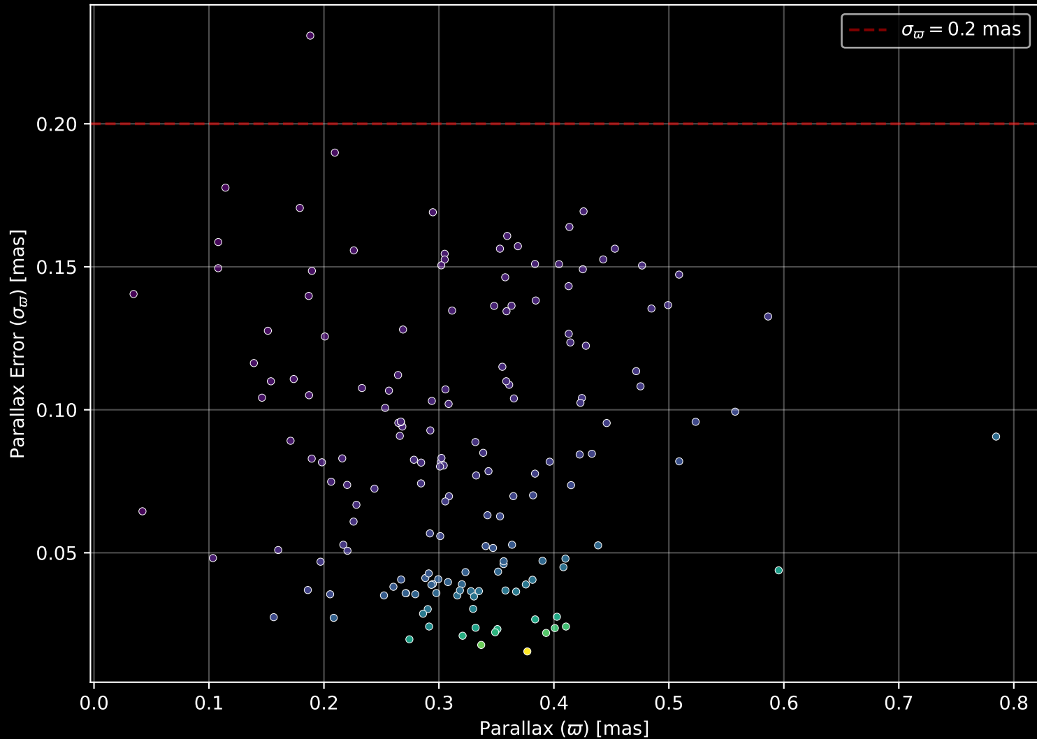
Gaia Cluster: [NGC_2259] Parallax Quality (n= 167)
