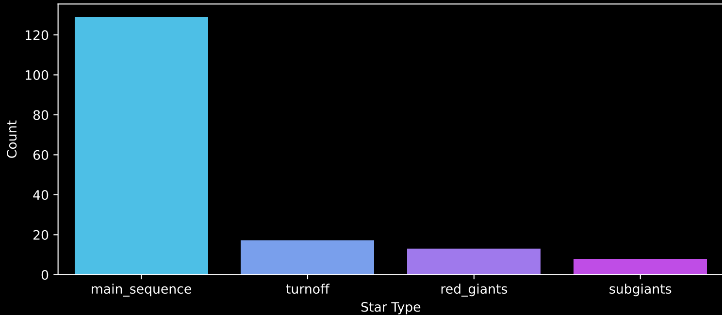
Gaia Cluster: [NGC_2259] Count plot of Star Type
