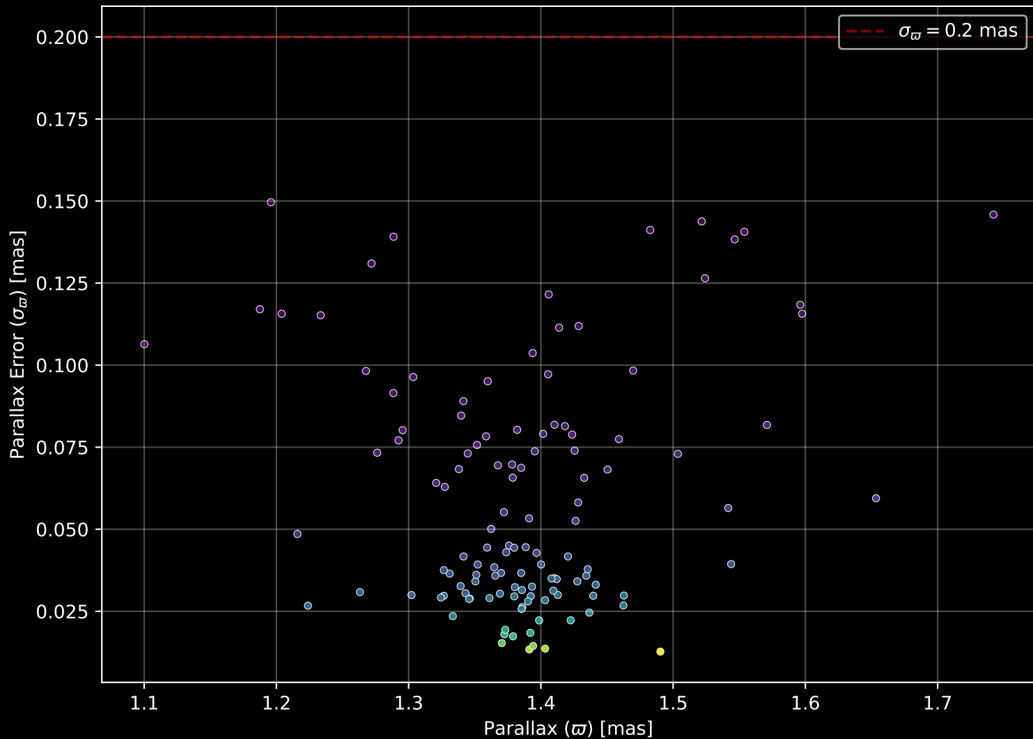
Gaia Cluster: [NGC_2264] Parallax Quality (n= 124)
