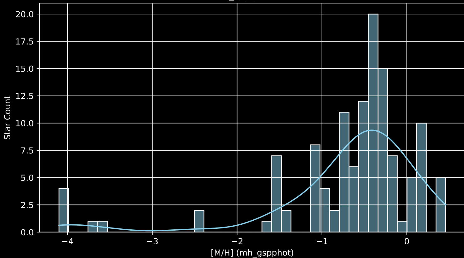
Gaia Cluster: [NGC_2264 [M/H] (mh_gspphot) (n= 124)
