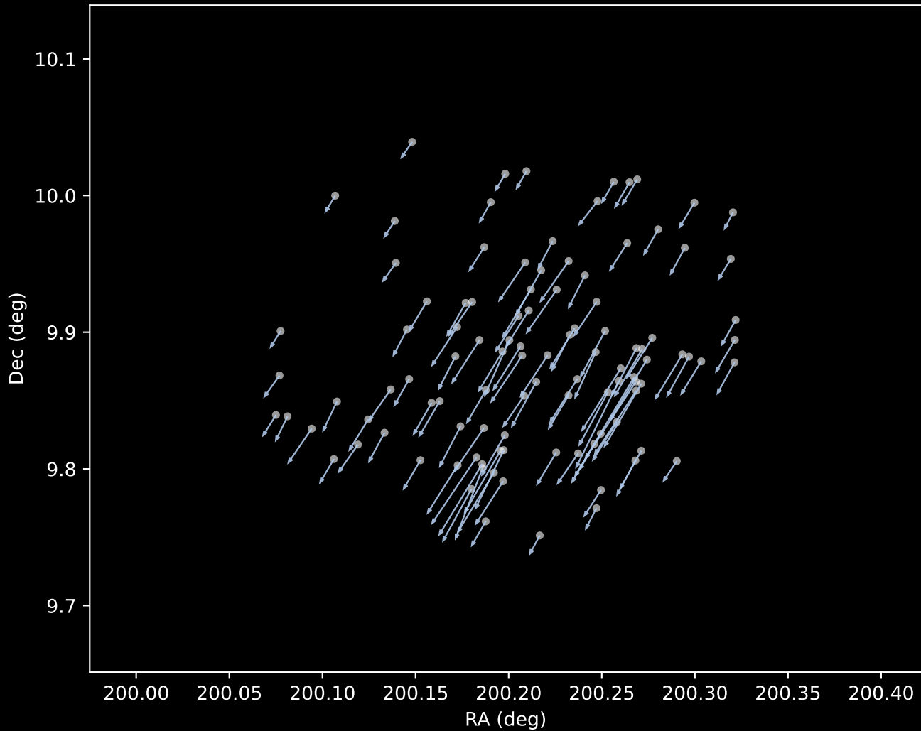
Gaia DR3 Cluster 1 Proper Motion Vectors (n=105)
