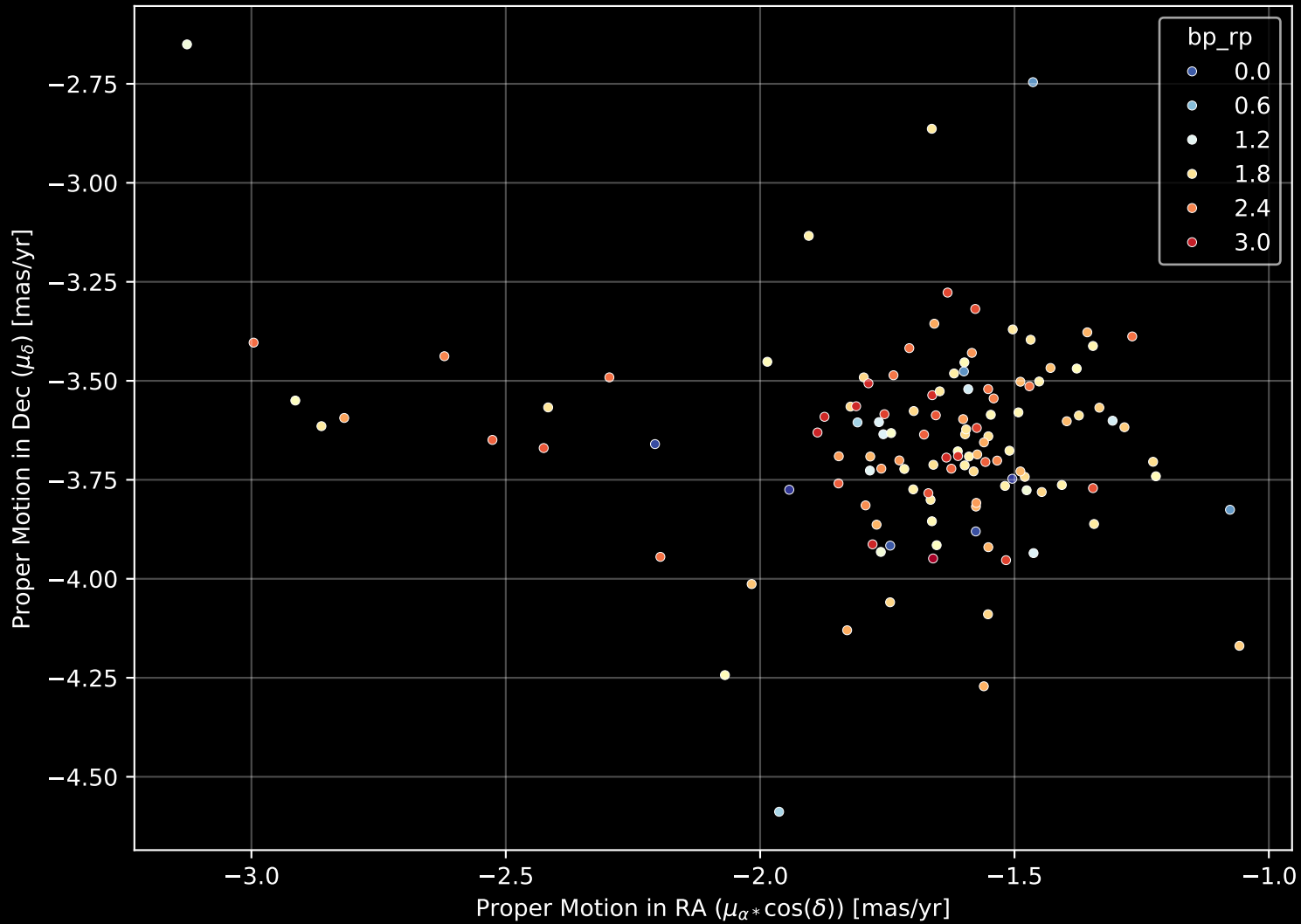
Gaia Cluster: [NGC_2264] Proper Motion Diagram (n= 124)
