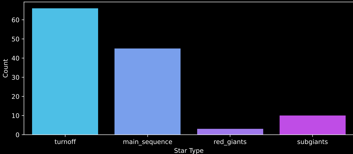
Gaia Cluster: [NGC_2264] Count plot of Star Type
