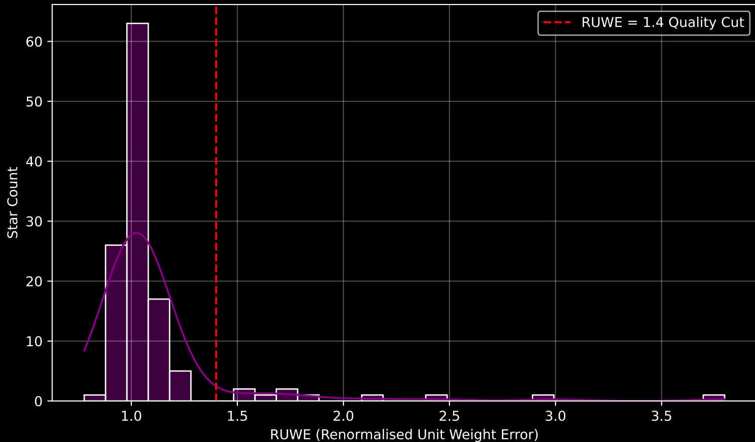
Gaia Cluster: [NGC_2264] RUWE Distribution (n= 122)
