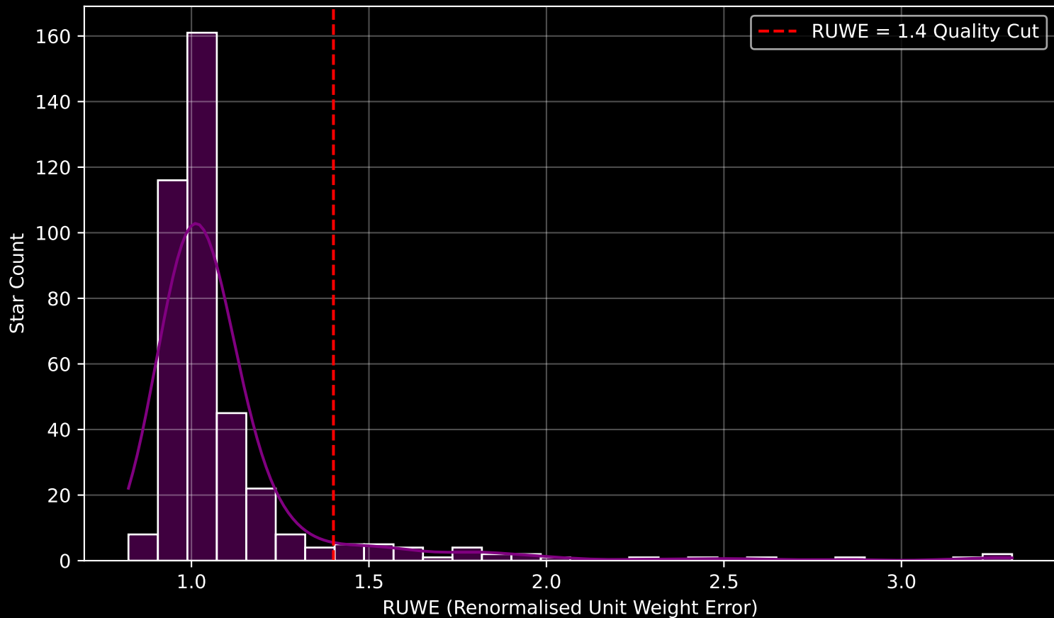
Gaia Cluster: [NGC_2281] RUWE Distribution (n= 395)
