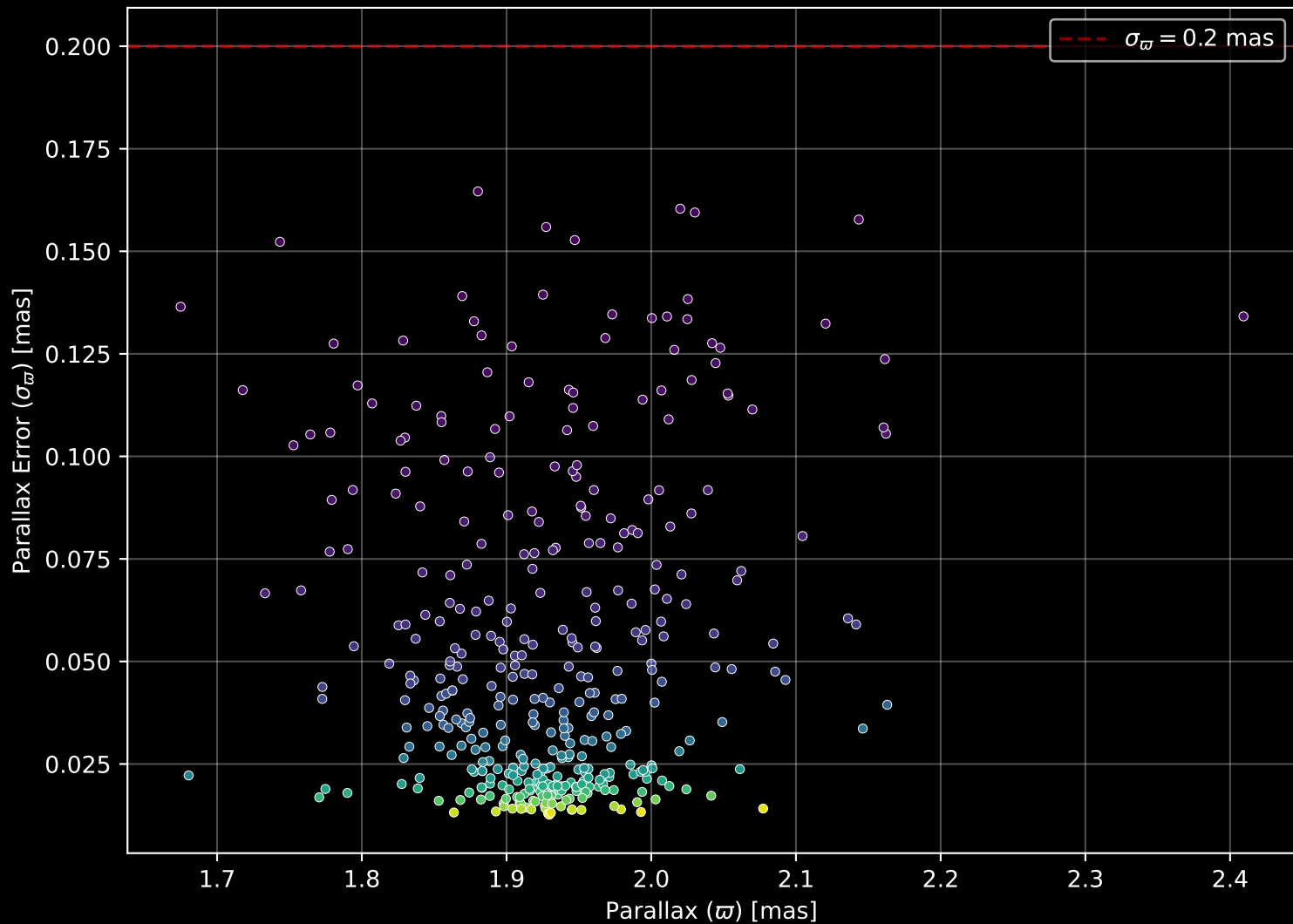
Gaia Cluster: [NGC_2281] Parallax Quality (n= 395)
