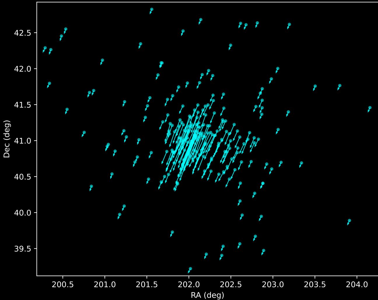
Gaia DR3 Noise Stream Proper Motion Vectors (n=221)
