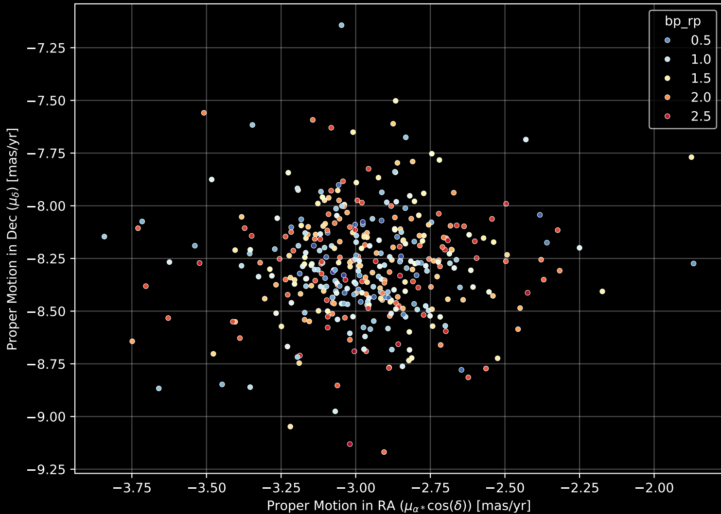
Gaia Cluster: [NGC_2281] Proper Motion Diagram (n= 395)
