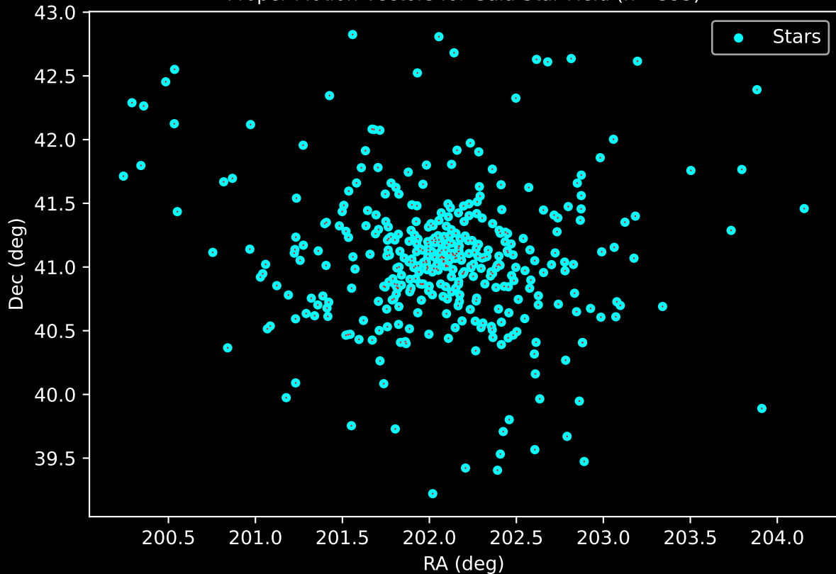
Gaia Cluster: [NGC_2281] Proper Motion Vectors for Gaia Star Field (n= 395)
