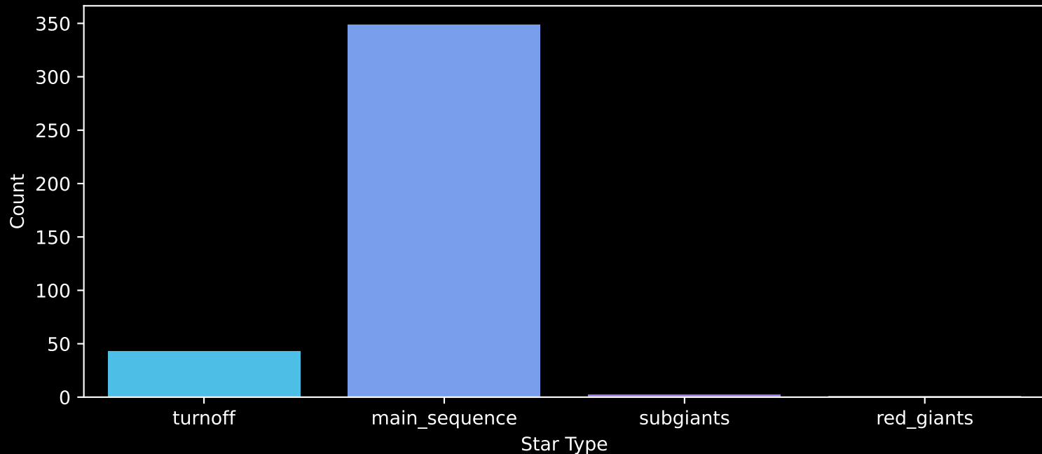
Gaia Cluster: [NGC_2281] Count plot of Star Type
