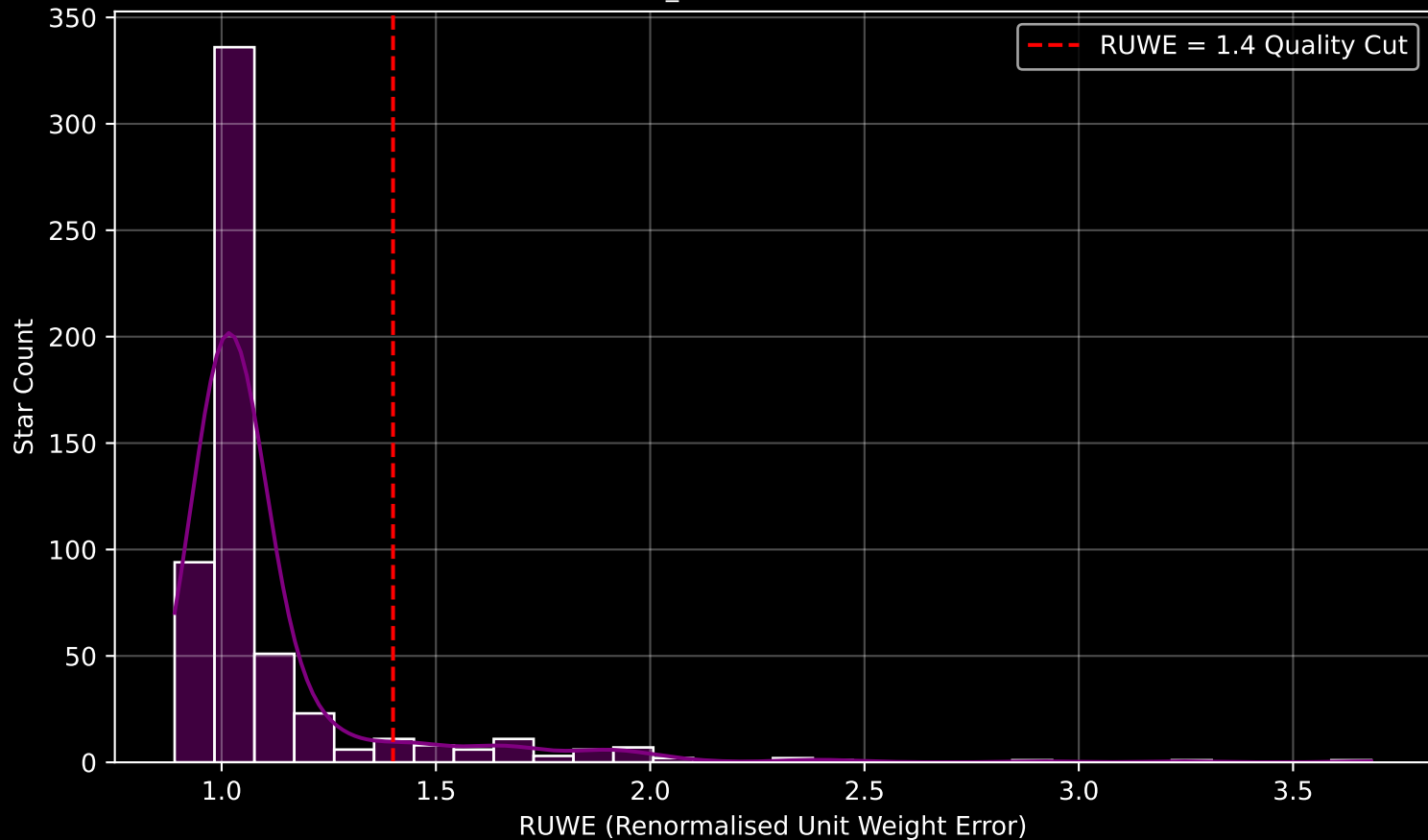
Gaia Cluster: [NGC_2287] RUWE Distribution (n= 570)
