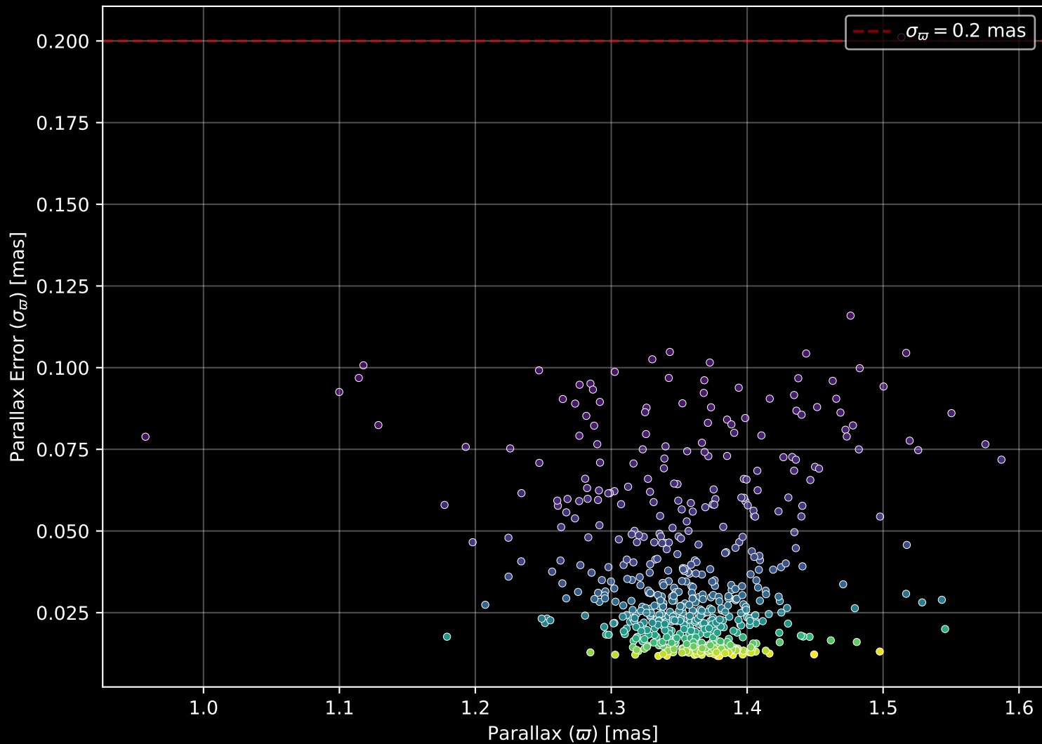
Gaia Cluster: [NGC_2287] Parallax Quality (n= 574)
