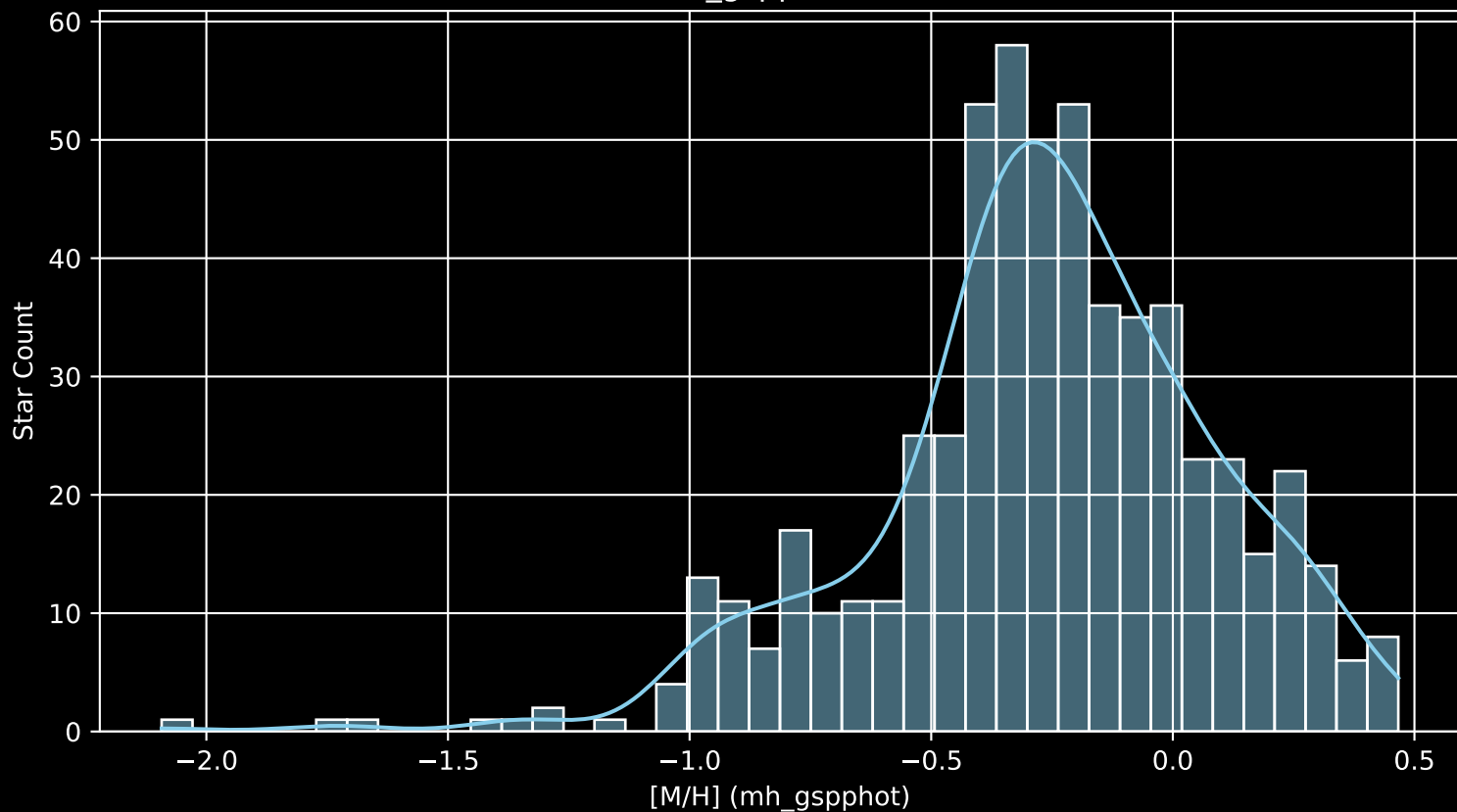
Gaia Cluster: [NGC_2287 [M/H] (mh_gspphot) (n= 574)
