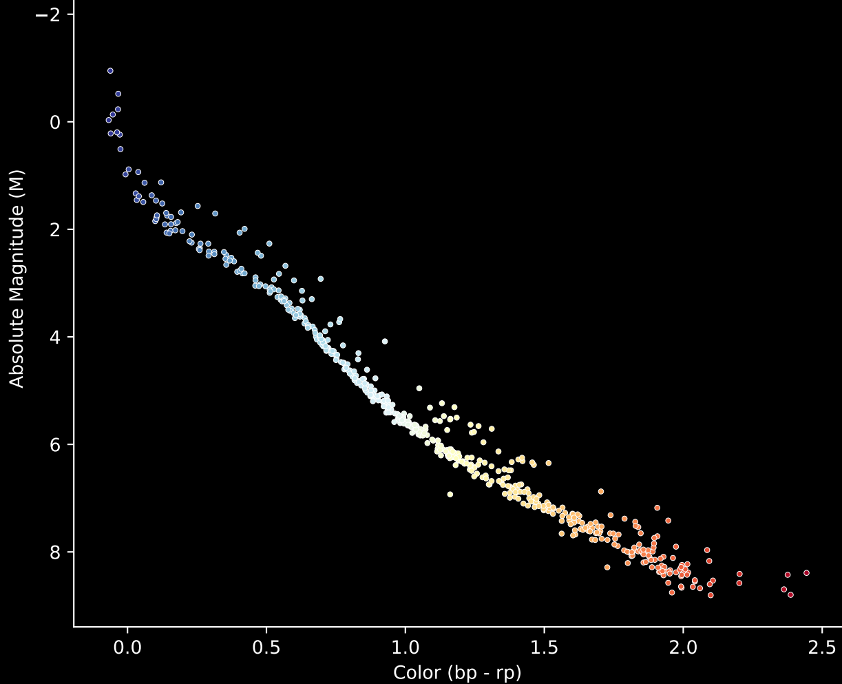
Gaia Cluster: [NGC 2287] Stars (n= 574) Hertzsprung-Russel Diagram
