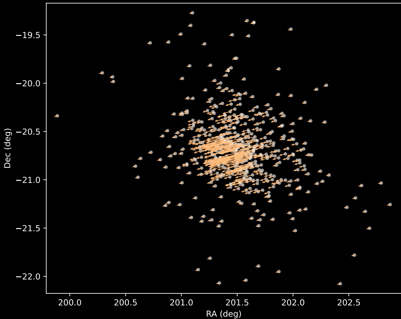
Gaia DR3 Cluster 3 Proper Motion Vectors (n=503)
