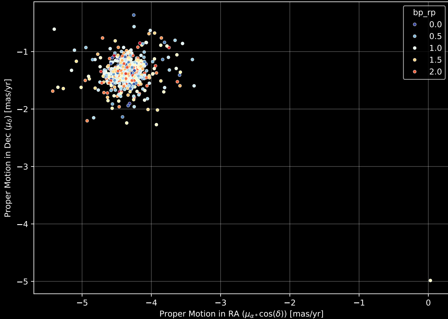
Gaia Cluster: [NGC_2287] Proper Motion Diagram (n= 574)
