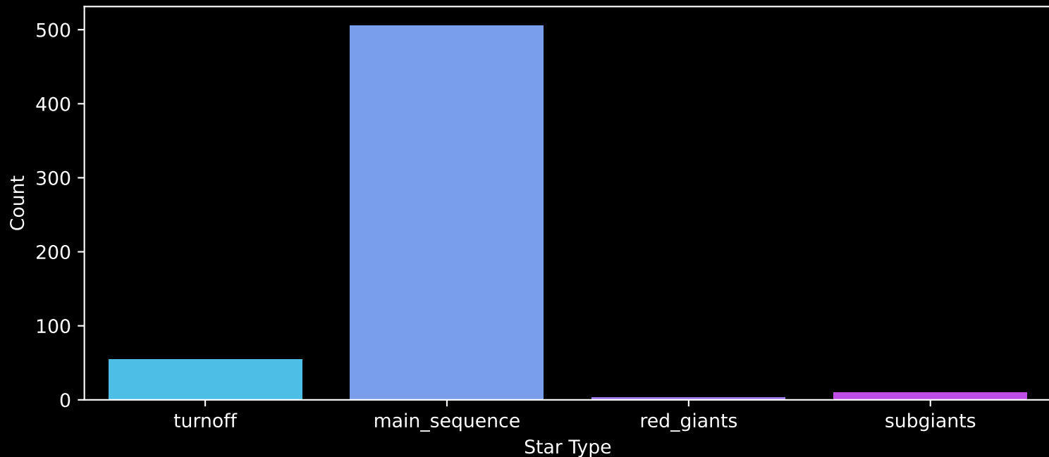
Gaia Cluster: [NGC_2287] Count plot of Star Type
