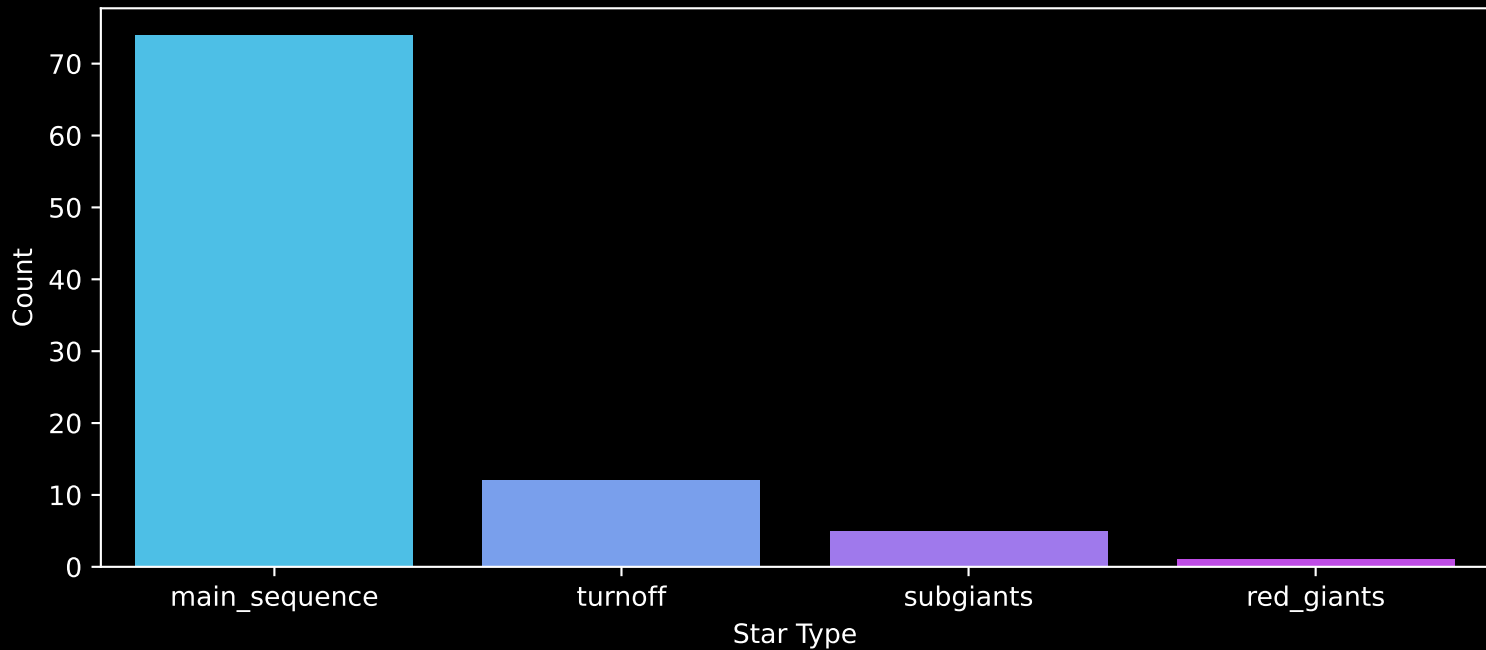
Gaia Cluster: [NGC_2302] Count plot of Star Type
