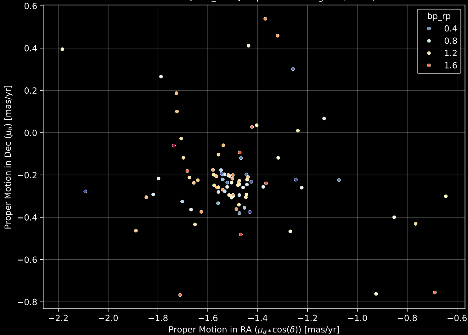
Gaia Cluster: [NGC_2302] Proper Motion Diagram (n= 92)
