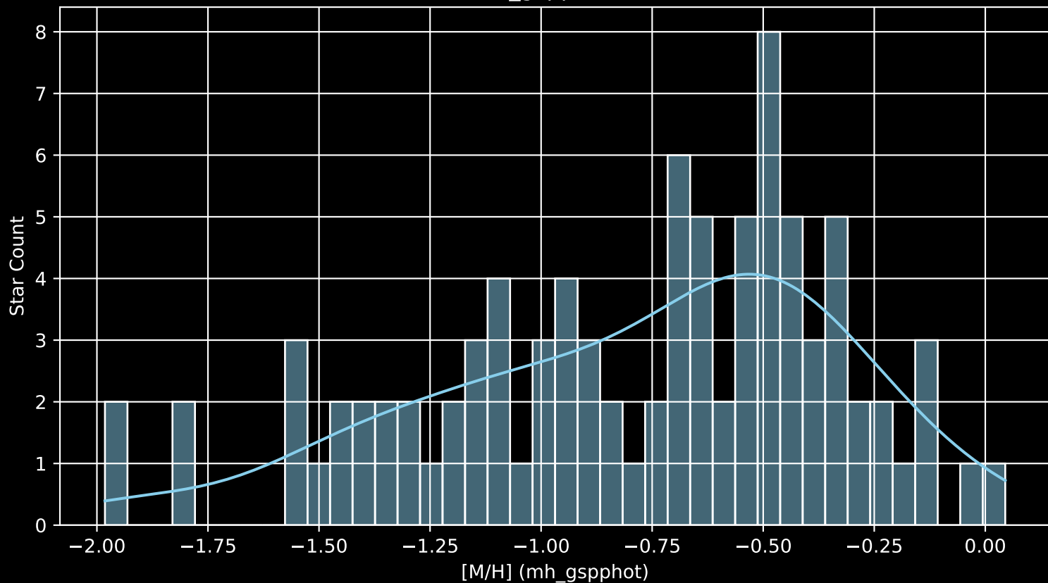
Gaia Cluster: [NGC_2302 [M/H] (mh_gspphot) (n= 91)
