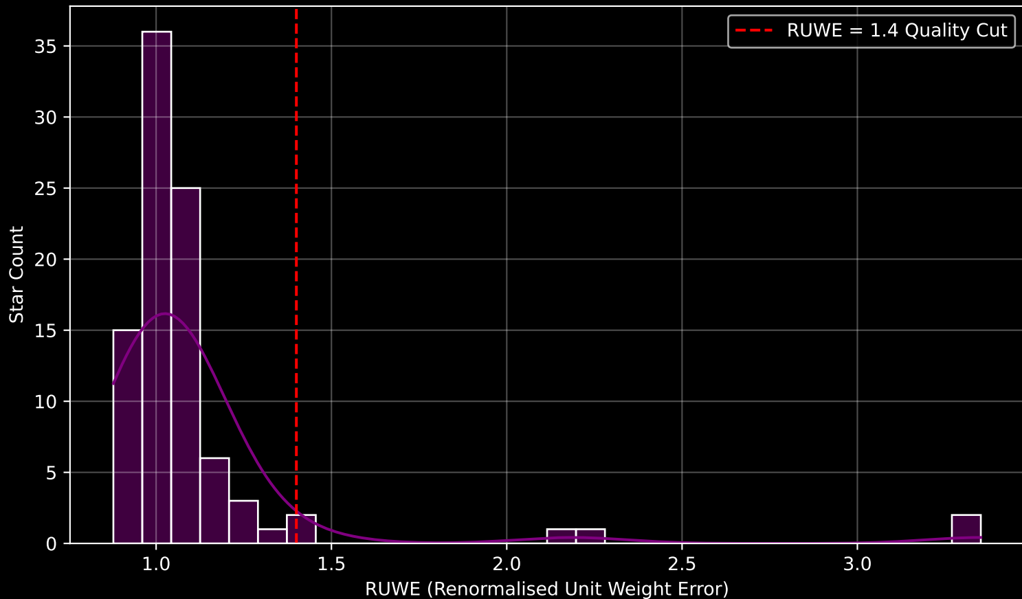
Gaia Cluster: [NGC_2302] RUWE Distribution (n= 92)
