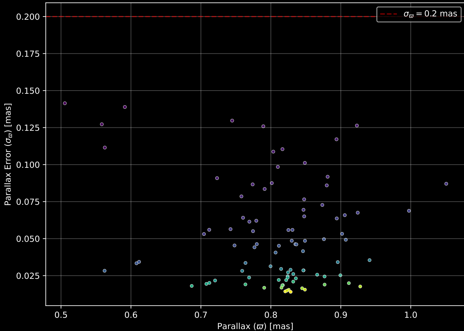
Gaia Cluster: [NGC_2302] Parallax Quality (n= 92)
