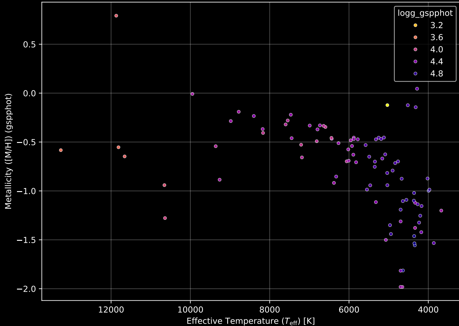
Gaia Cluster: [NGC_2302] Stellar Population Parameters (n= 92)
