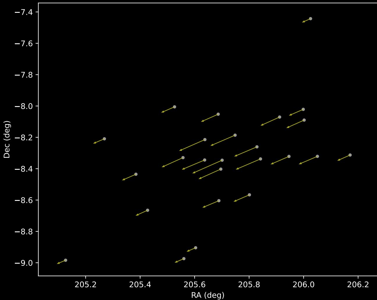
Gaia DR3 Cluster 56 Proper Motion Vectors (n=25)
