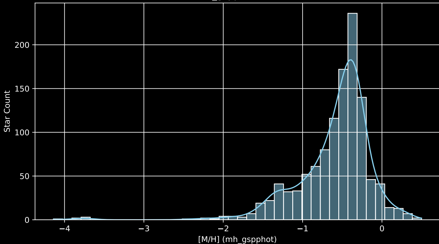
Gaia Cluster: [NGC_2323 [M/H] (mh_gspphot) (n= 1156)
