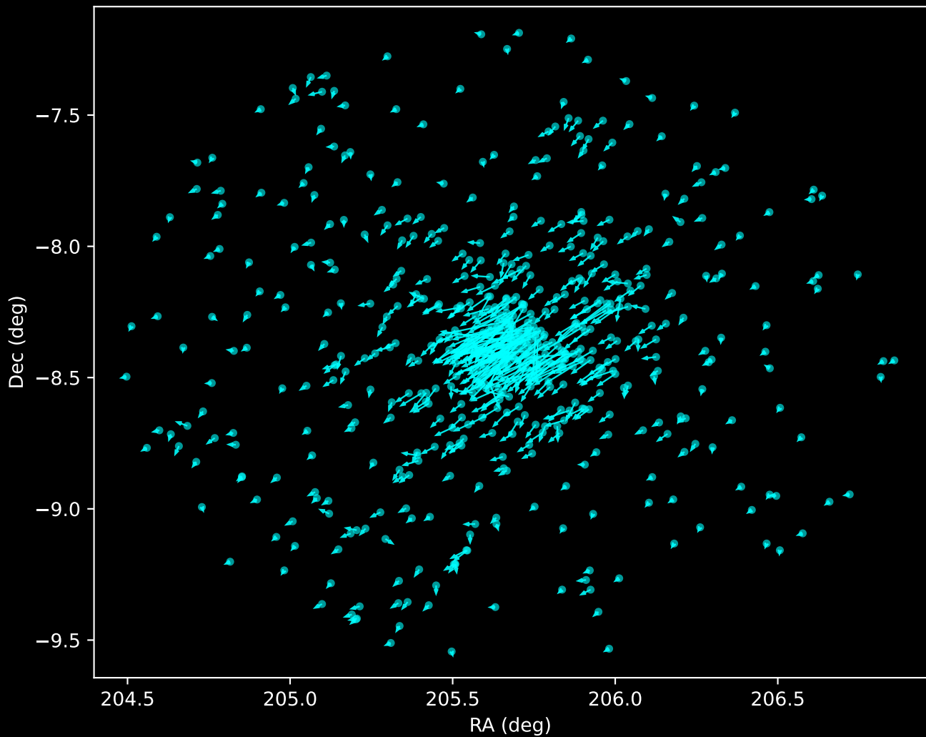
Gaia DR3 Noise Stream Proper Motion Vectors (n=562)
