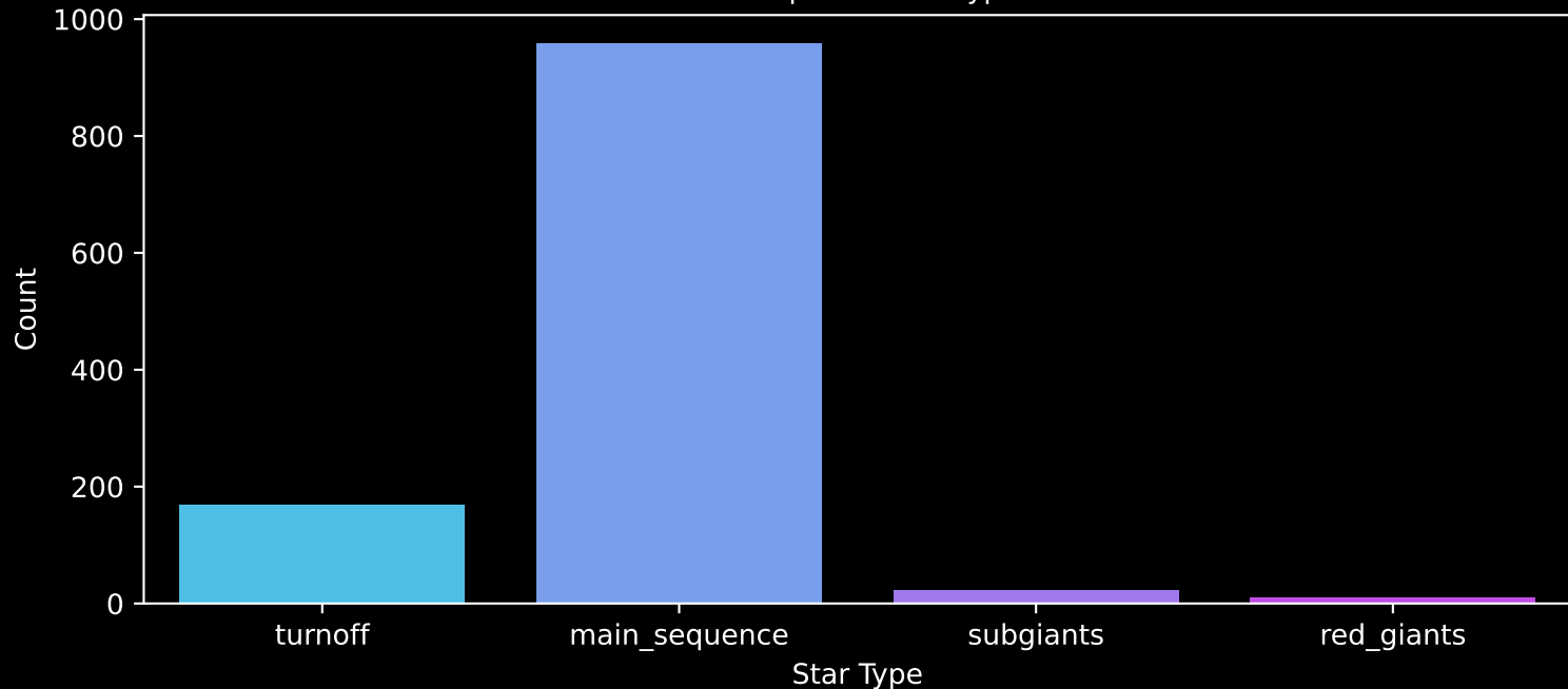
Gaia Cluster: [NGC_2323] Count plot of Star Type
