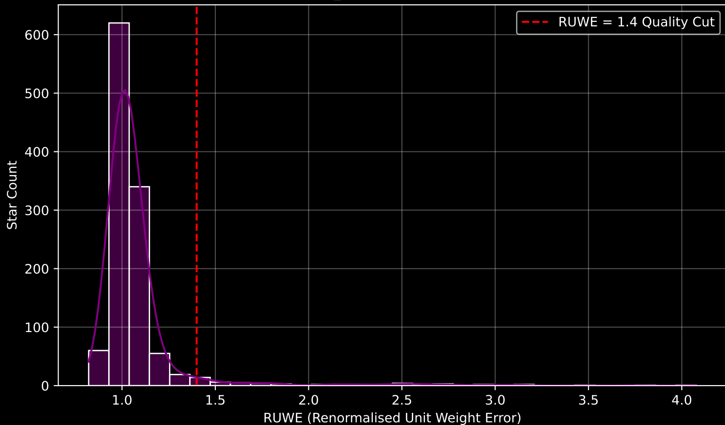
Gaia Cluster: [NGC_2323] RUWE Distribution (n= 1150)
