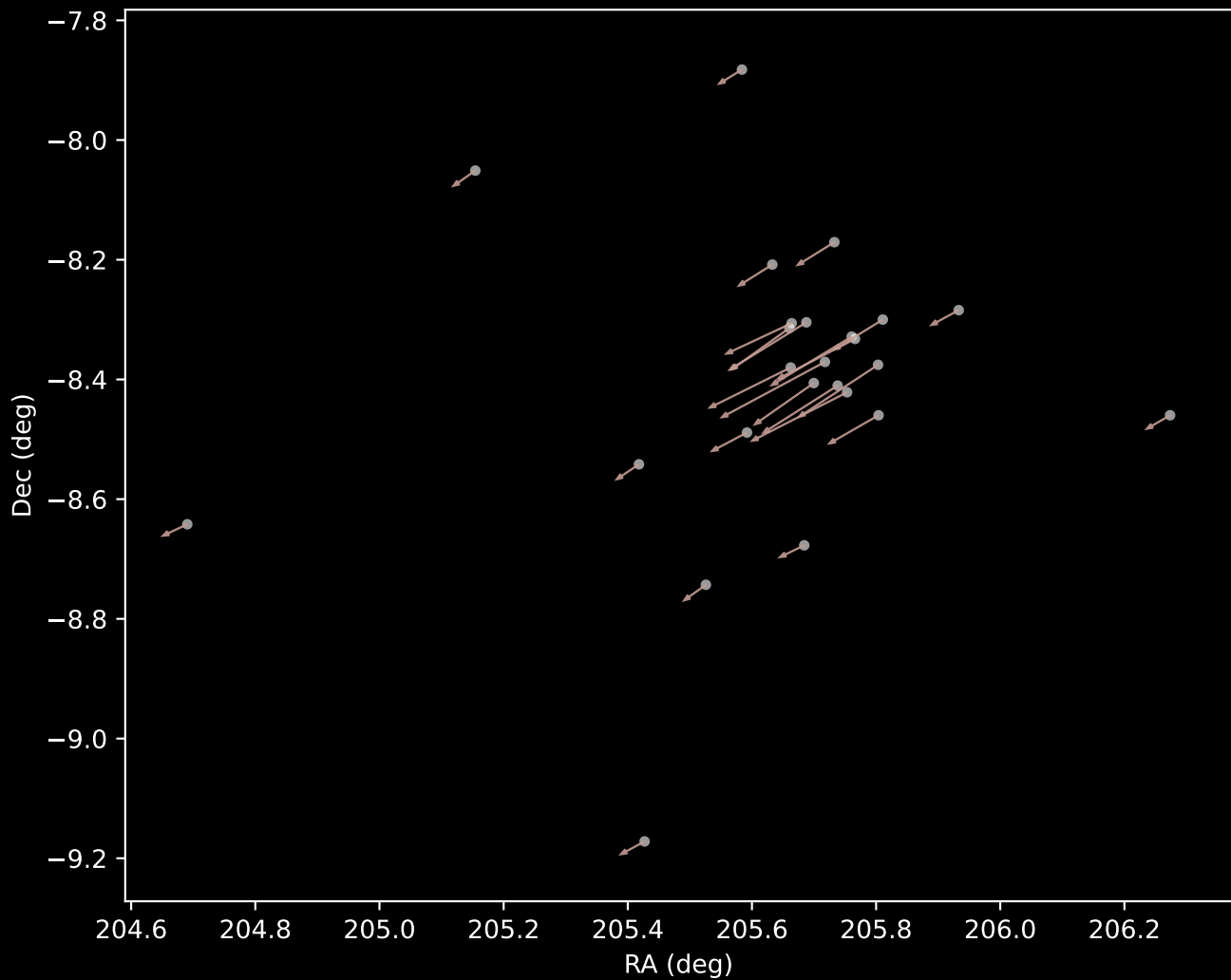
Gaia DR3 Cluster 31 Proper Motion Vectors (n=25)
