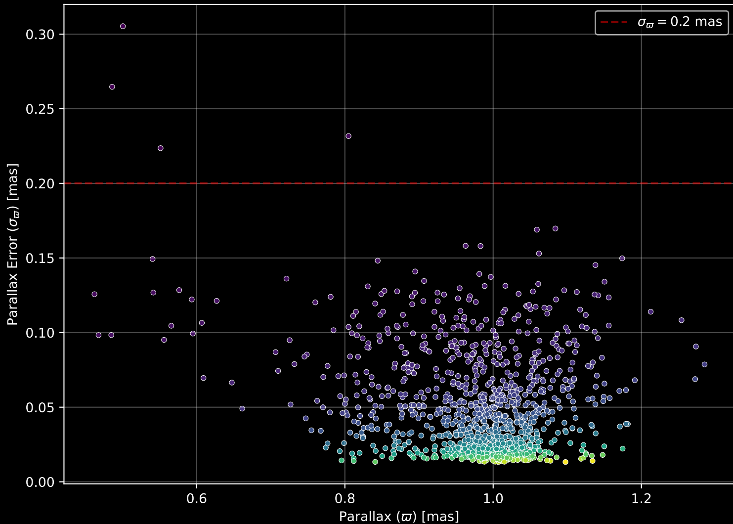
Gaia Cluster: [NGC_2323] Parallax Quality (n= 1160)
