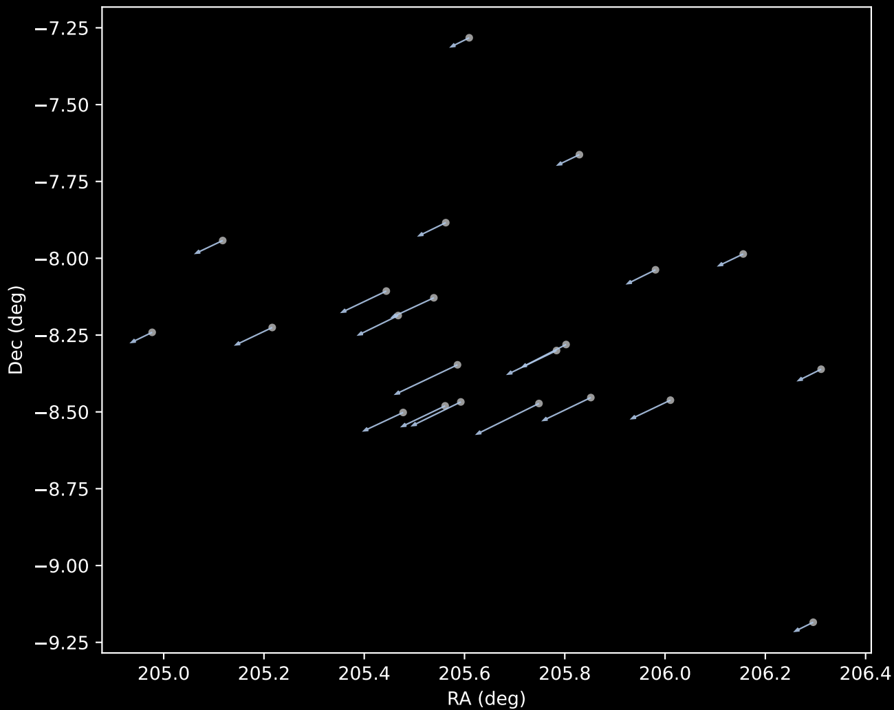
Gaia DR3 Cluster 41 Proper Motion Vectors (n=22)
