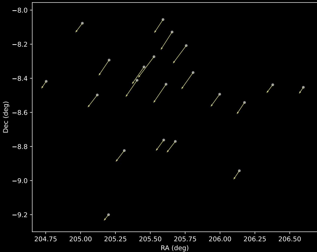
Gaia DR3 Cluster 37 Proper Motion Vectors (n=21)
