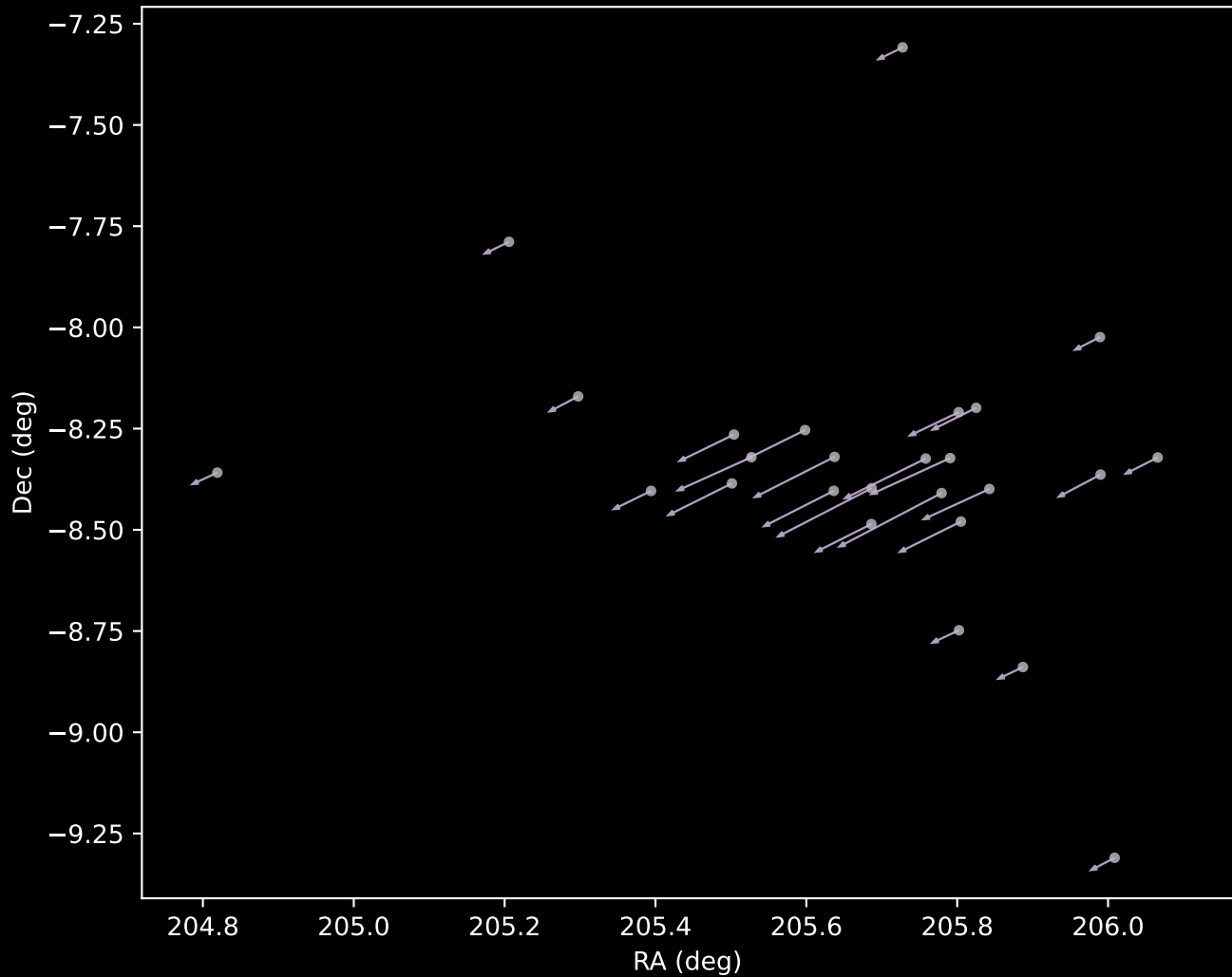
Gaia DR3 Cluster 49 Proper Motion Vectors (n=26)
