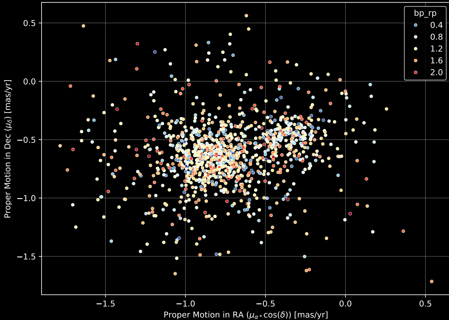
Gaia Cluster: [NGC_2323] Proper Motion Diagram (n= 1160)
