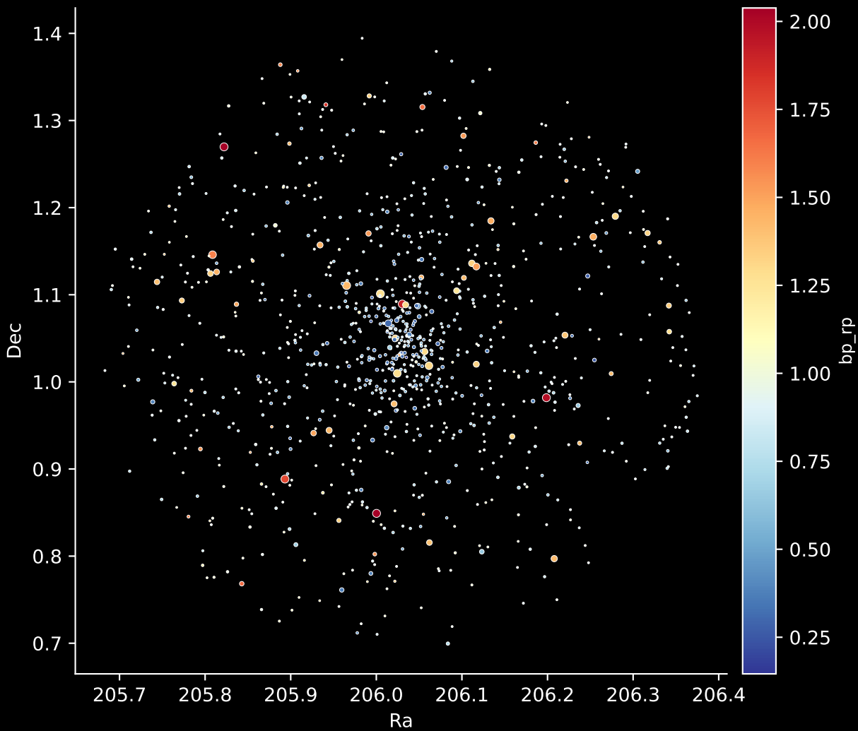
Gaia Cluster: [NGC_2324] Stars: 995
