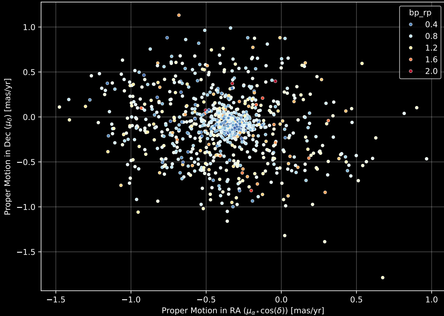
Gaia Cluster: [NGC_2324] Proper Motion Diagram (n= 995)
