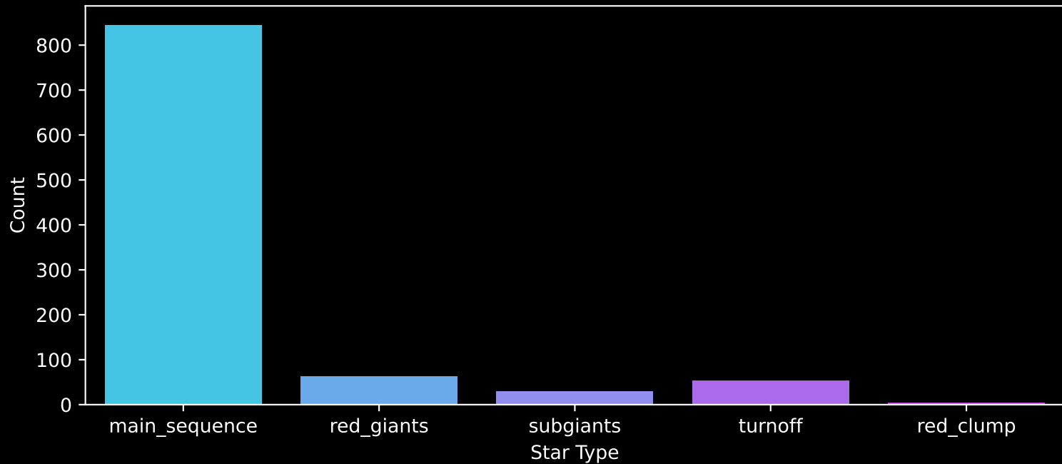
Gaia Cluster: [NGC_2324] Count plot of Star Type
