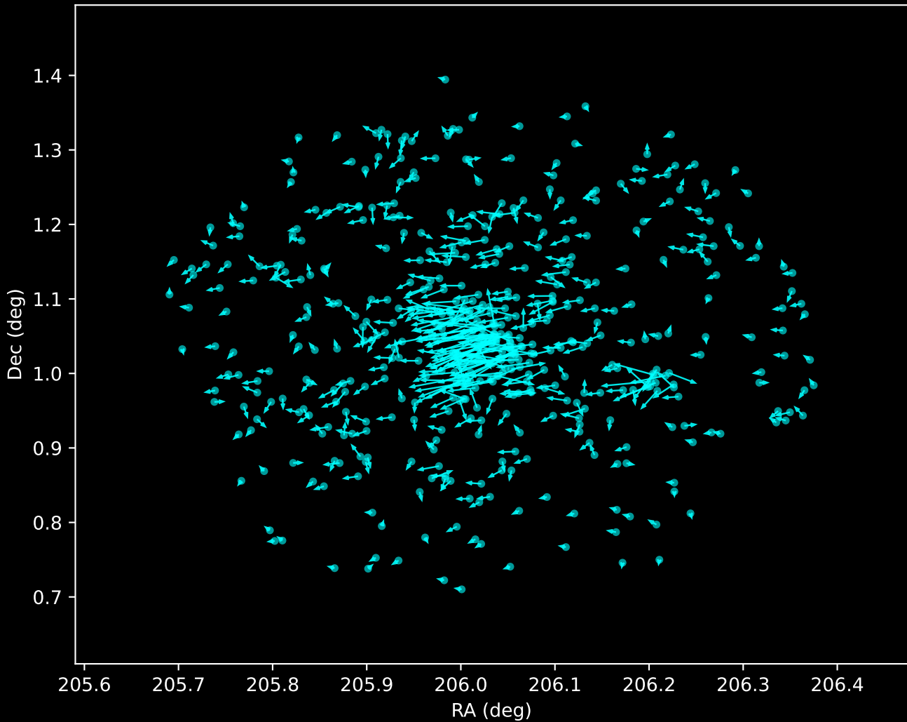
Gaia DR3 Noise Stream Proper Motion Vectors (n=496)
