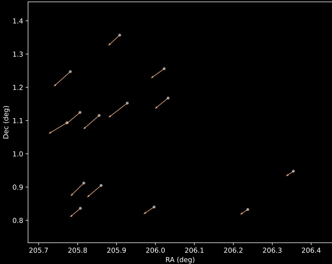
Gaia DR3 Cluster 23 Proper Motion Vectors (n=14)
