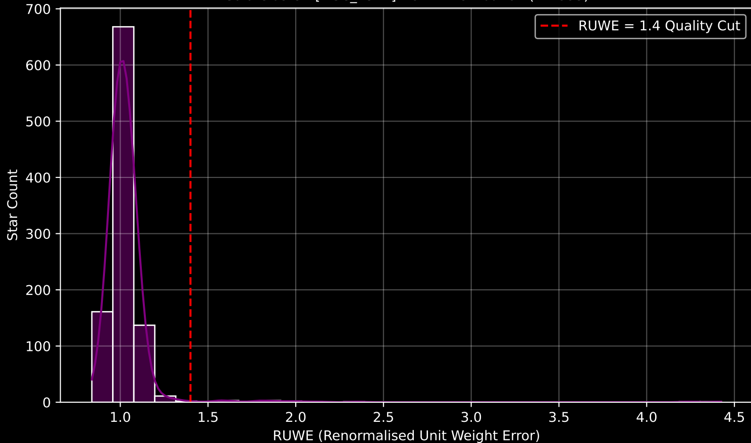
Gaia Cluster: [NGC_2324] RUWE Distribution (n= 993)
