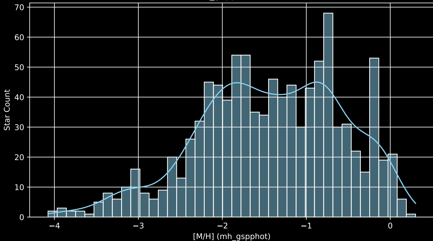
Gaia Cluster: [NGC_2324 [M/H] (mh_gspphot) (n= 995)
