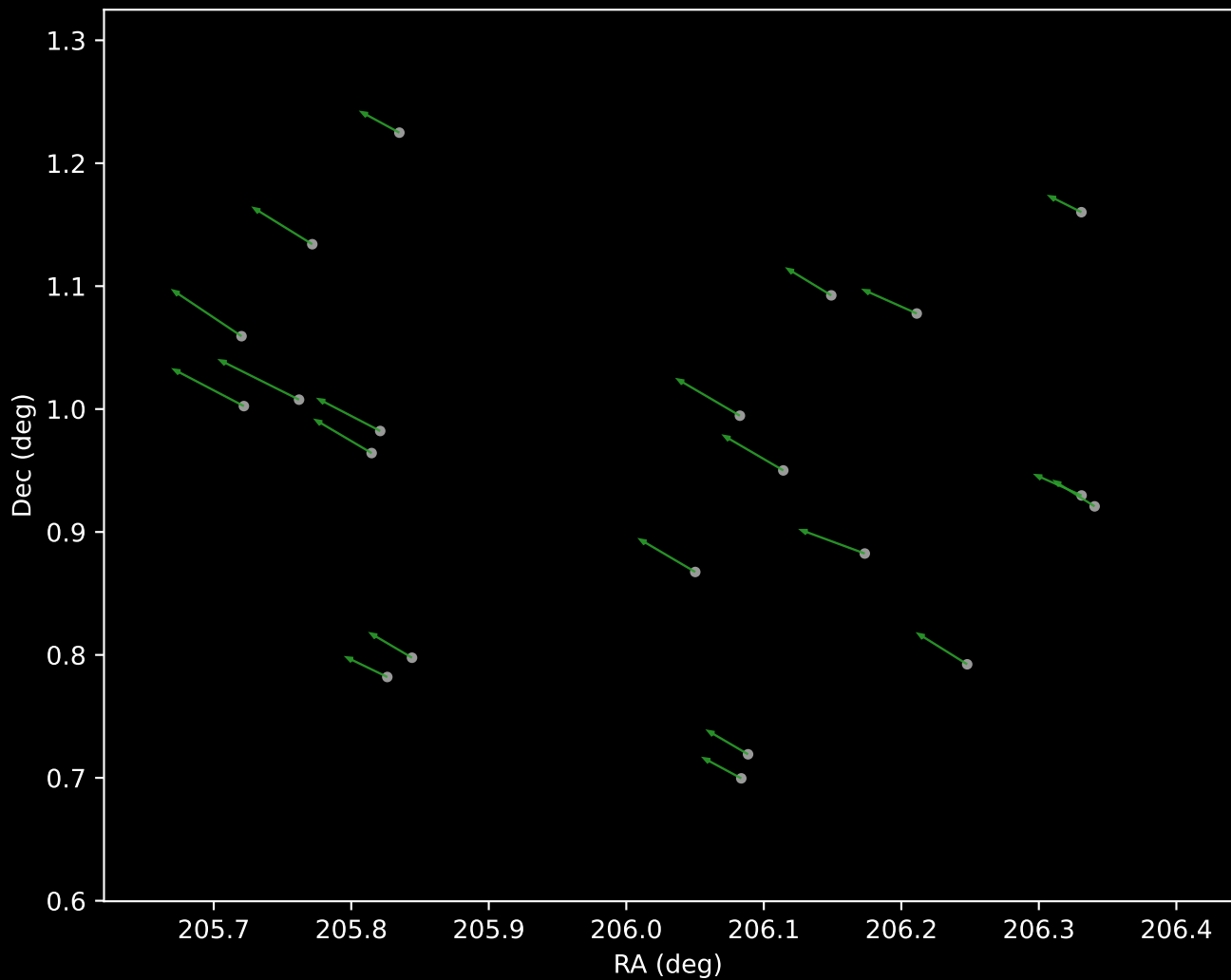
Gaia DR3 Cluster 24 Proper Motion Vectors (n=21)
