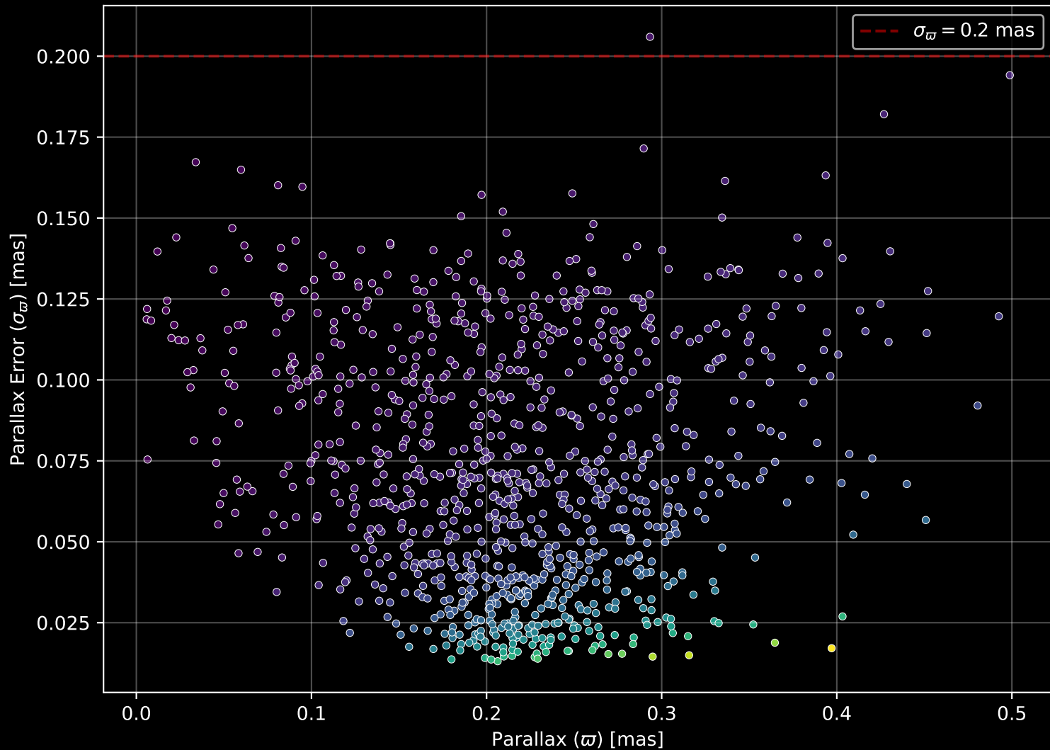
Gaia Cluster: [NGC_2324] Parallax Quality (n= 995)
