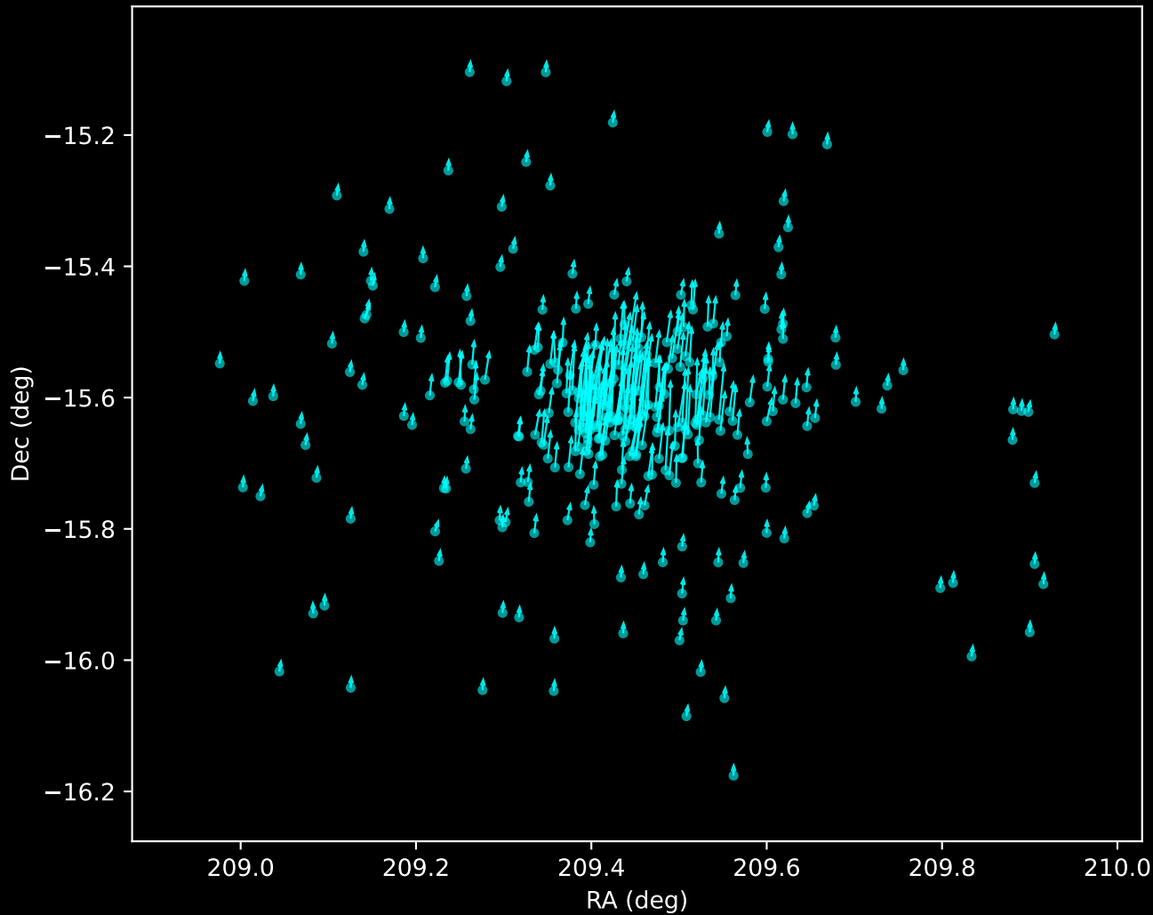
Gaia DR3 Noise Stream Proper Motion Vectors (n=310)
