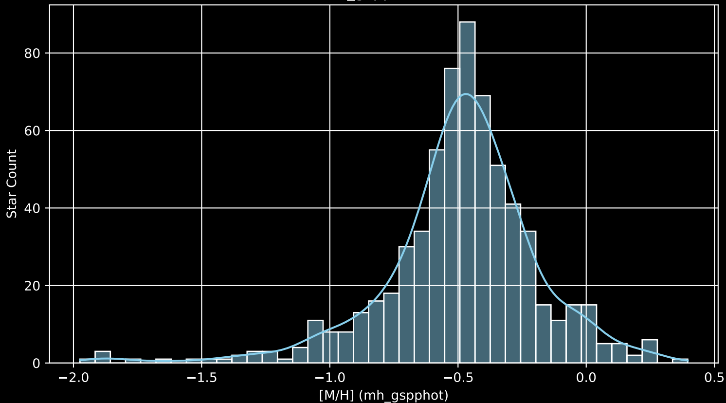
Gaia Cluster: [NGC_2360 [M/H] (mh_gspphot) (n= 649)
