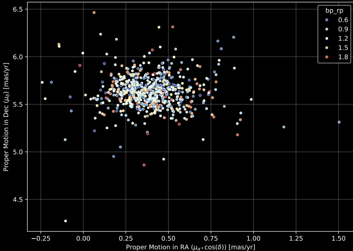
Gaia Cluster: [NGC_2360] Proper Motion Diagram (n= 650)
