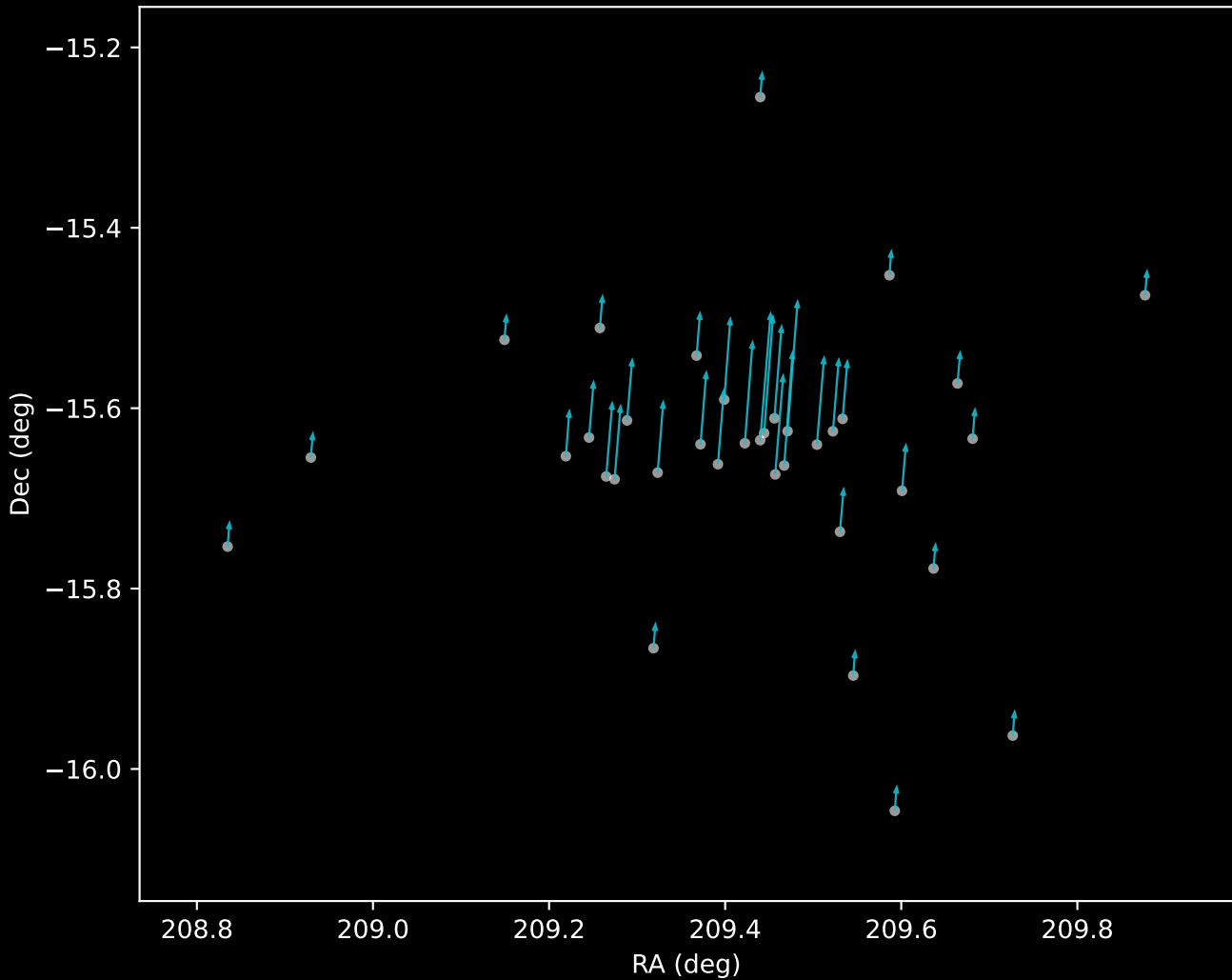
Gaia DR3 Cluster 18 Proper Motion Vectors (n=36)
