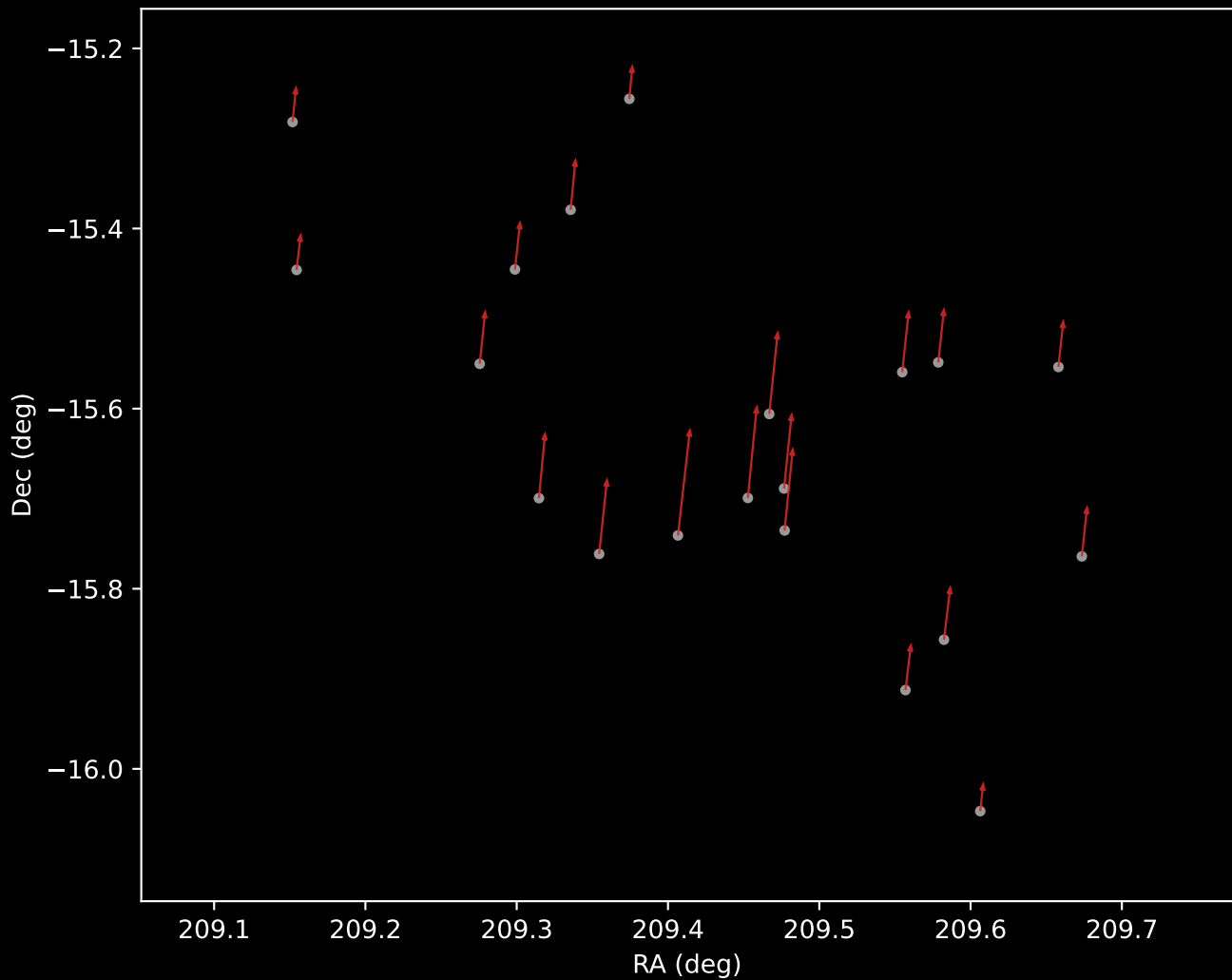
Gaia DR3 Cluster 26 Proper Motion Vectors (n=20)
