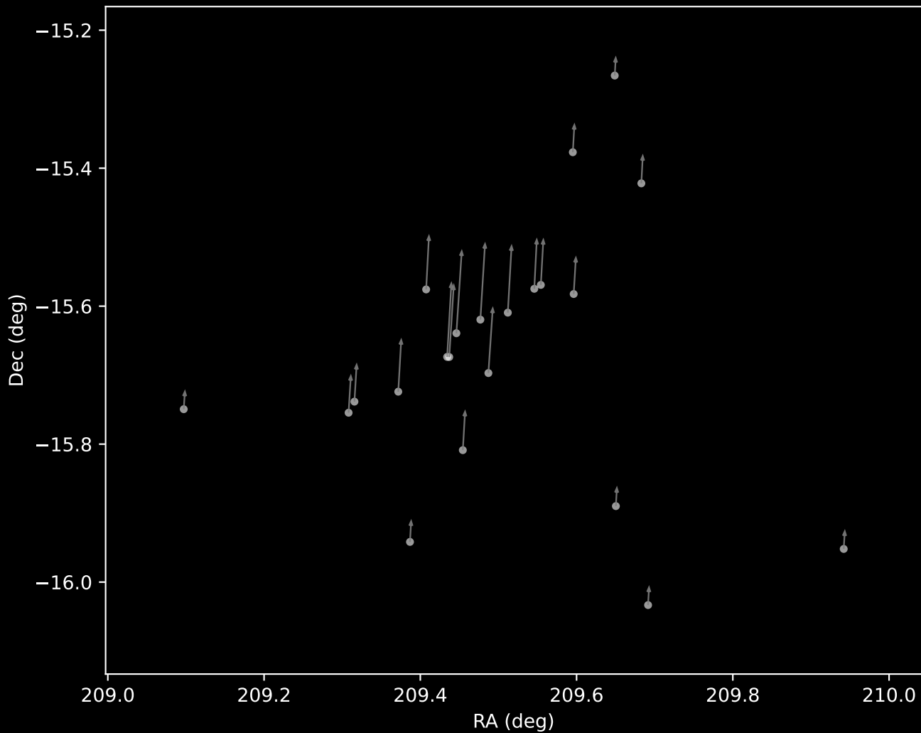
Gaia DR3 Cluster 14 Proper Motion Vectors (n=22)
