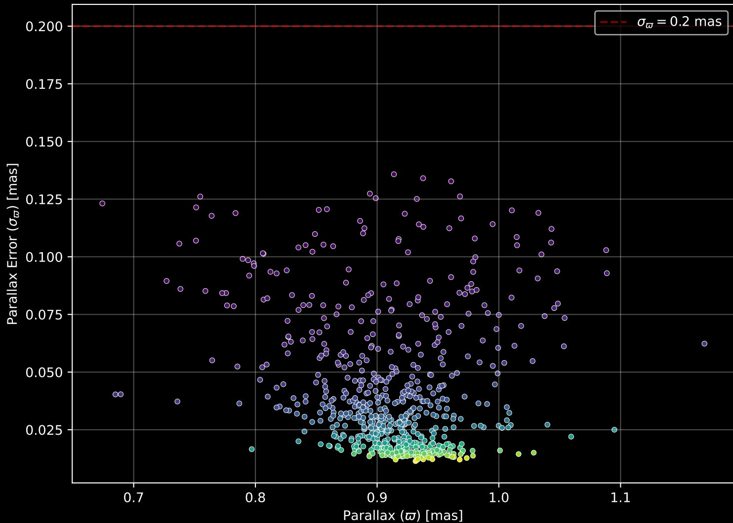
Gaia Cluster: [NGC_2360] Parallax Quality (n= 650)
