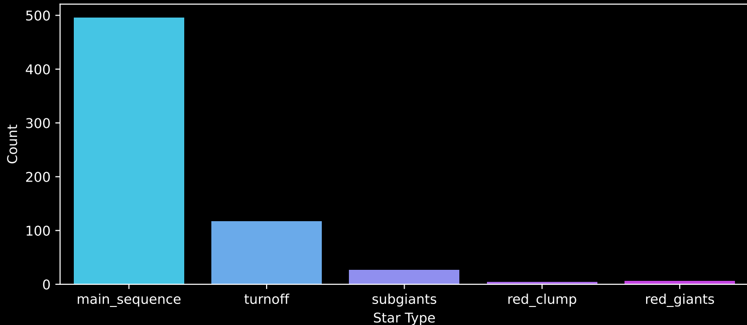
Gaia Cluster: [NGC_2360] Count plot of Star Type
