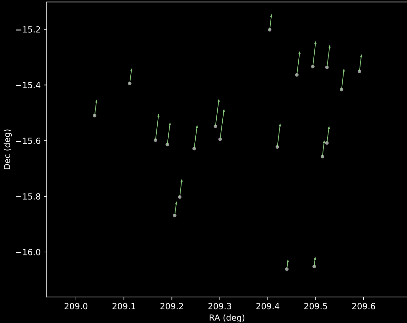
Gaia DR3 Cluster 25 Proper Motion Vectors (n=20)
