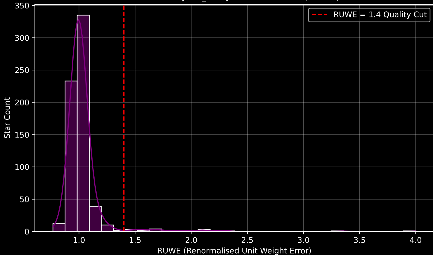
Gaia Cluster: [NGC_2360] RUWE Distribution (n= 650)
