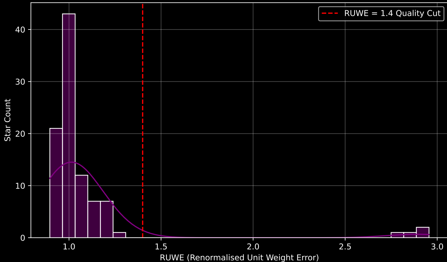
Gaia Cluster: [NGC_2374] RUWE Distribution (n= 95)
