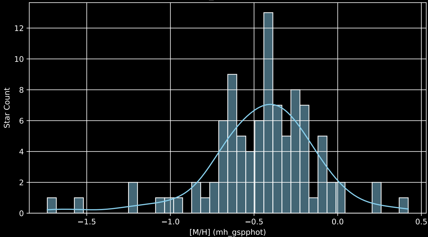
Gaia Cluster: [NGC_2374 [M/H] (mh_gspphot) (n= 95)
