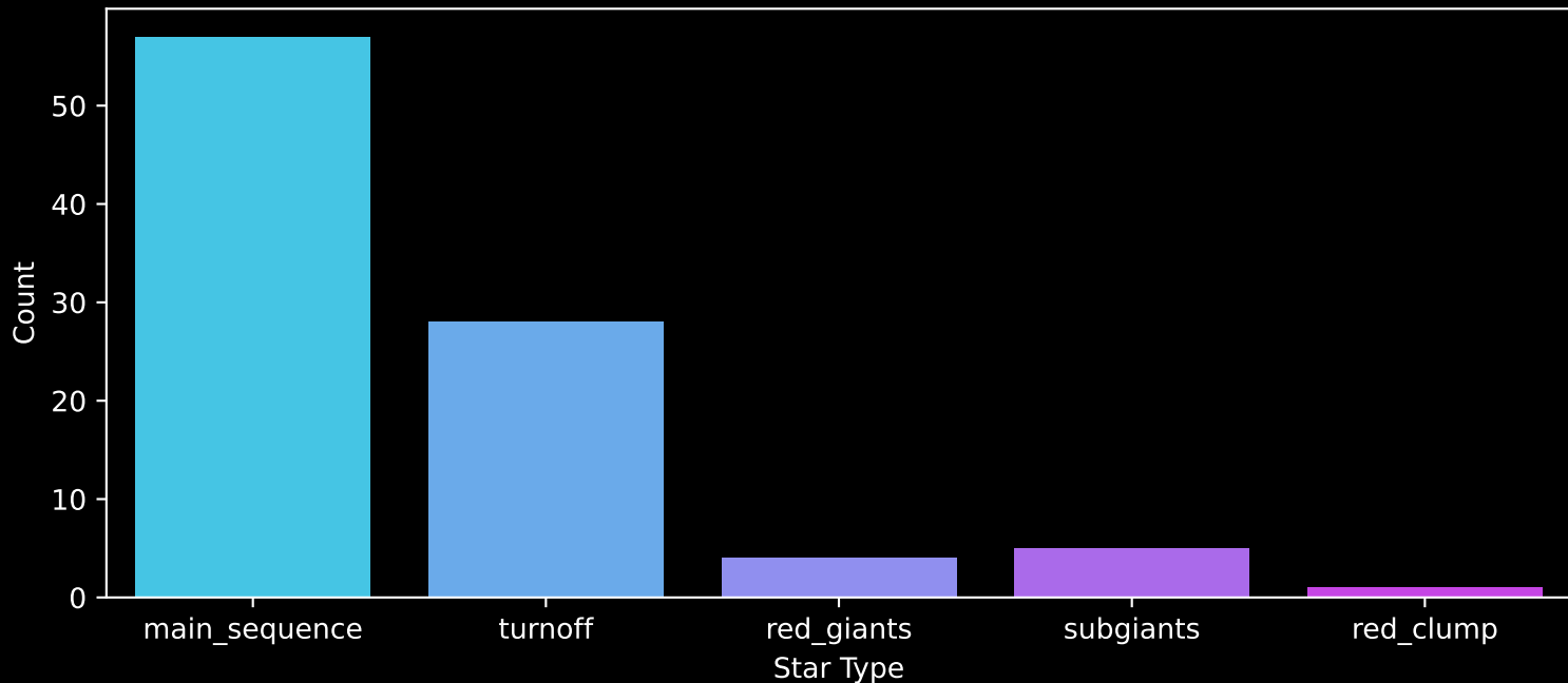
Gaia Cluster: [NGC_2374] Count plot of Star Type
