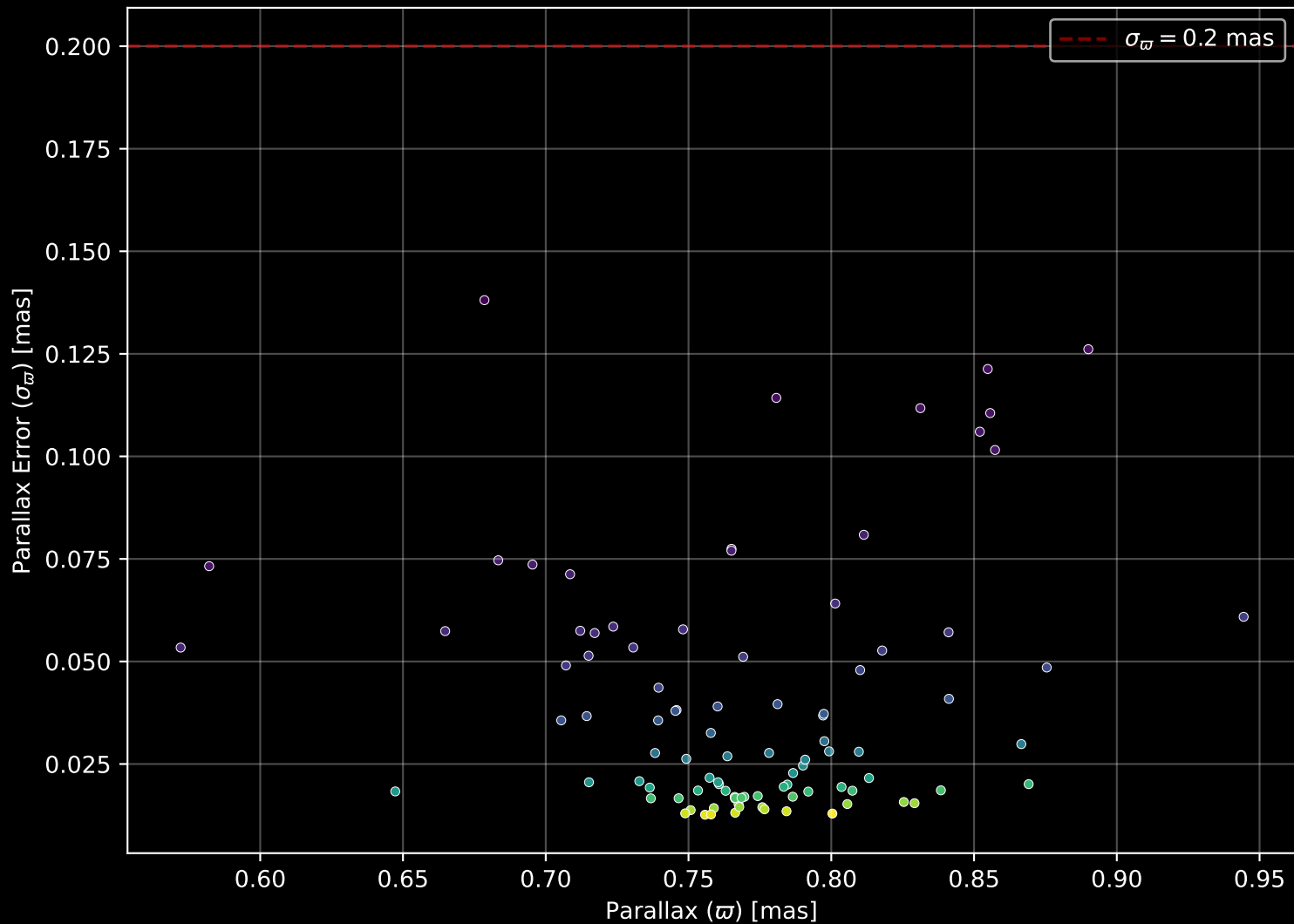
Gaia Cluster: [NGC_2374] Parallax Quality (n= 95)
