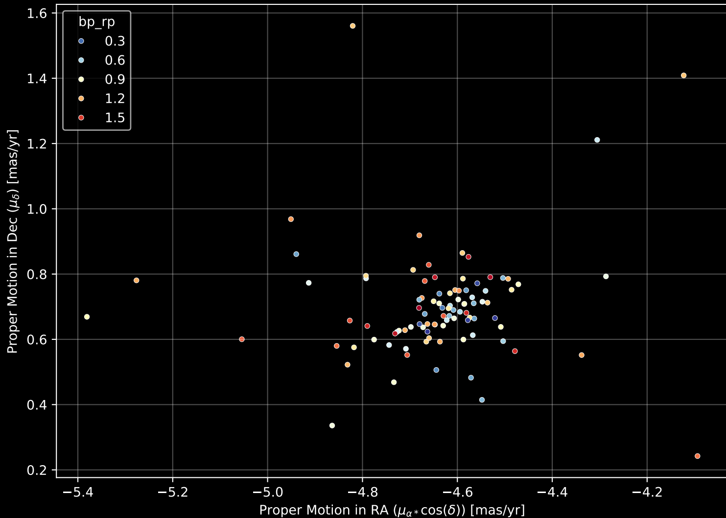
Gaia Cluster: [NGC_2374] Proper Motion Diagram (n= 95)
