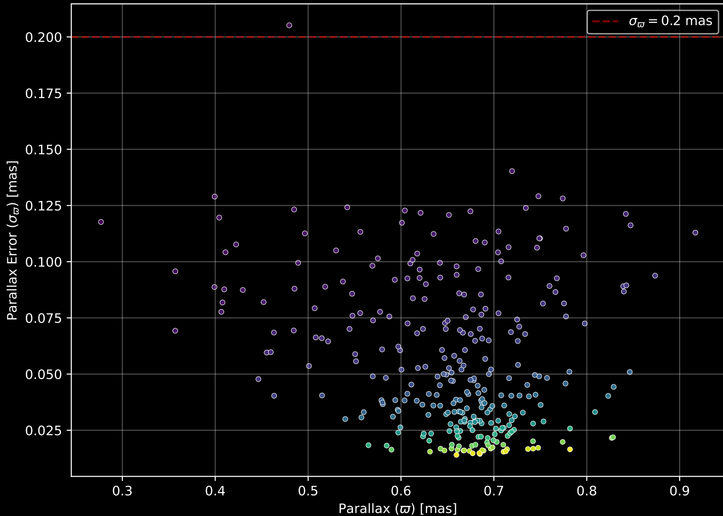
Gaia Cluster: [NGC_2396] Parallax Quality (n= 301)
