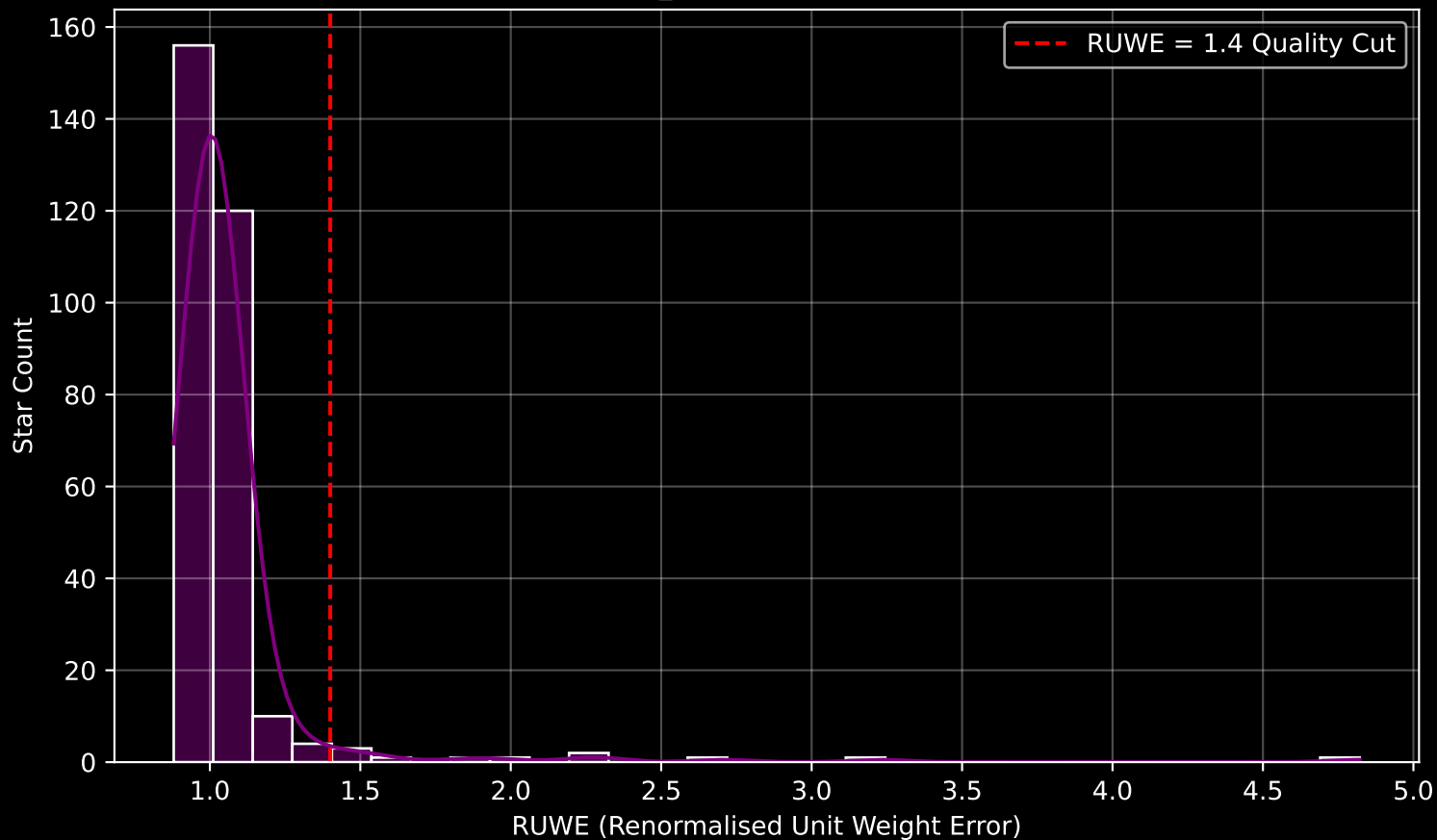
Gaia Cluster: [NGC_2396] RUWE Distribution (n= 301)
