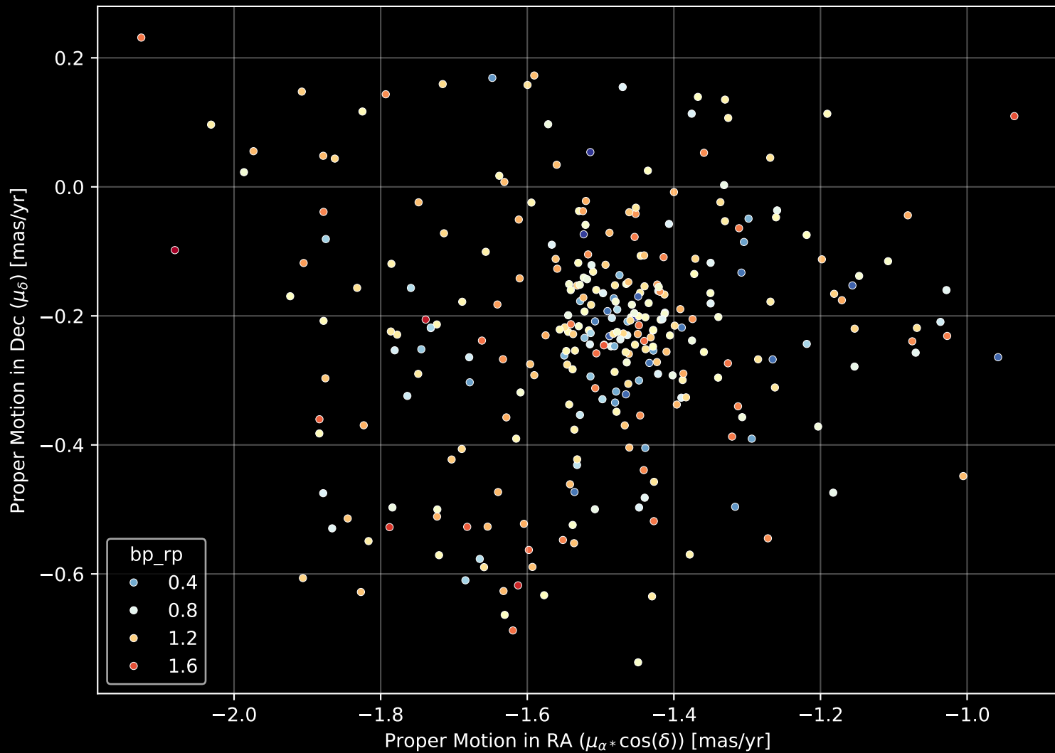
Gaia Cluster: [NGC_2396] Proper Motion Diagram (n= 301)
