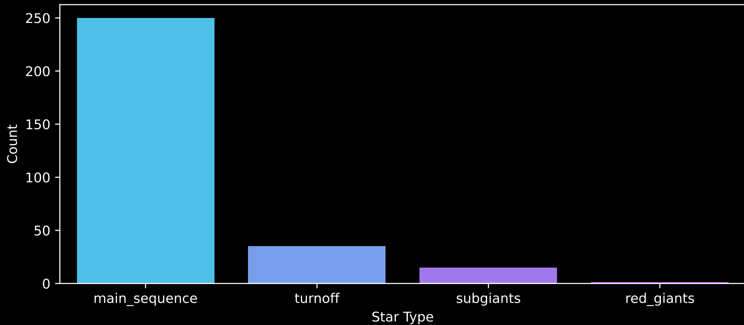
Gaia Cluster: [NGC_2396] Count plot of Star Type
