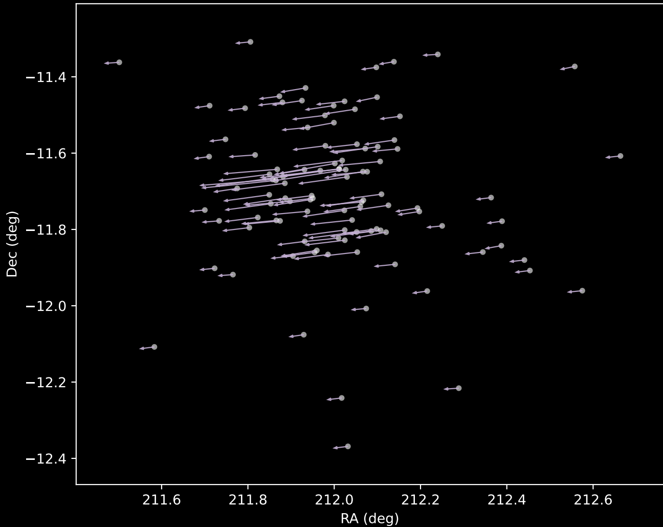
Gaia DR3 Cluster 9 Proper Motion Vectors (n=103)
