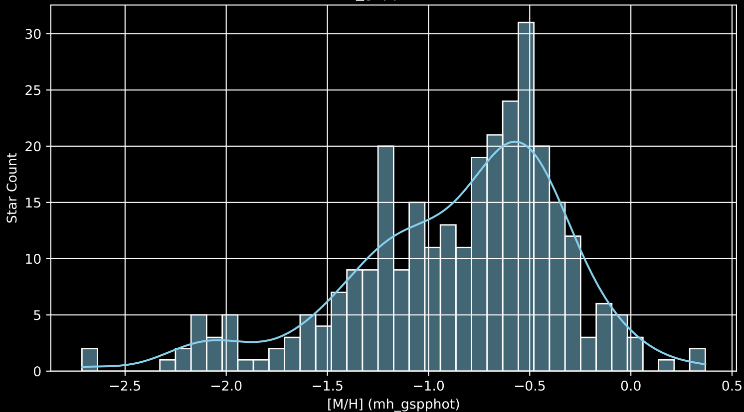
Gaia Cluster: [NGC_2396 [M/H] (mh_gspphot) (n= 300)
