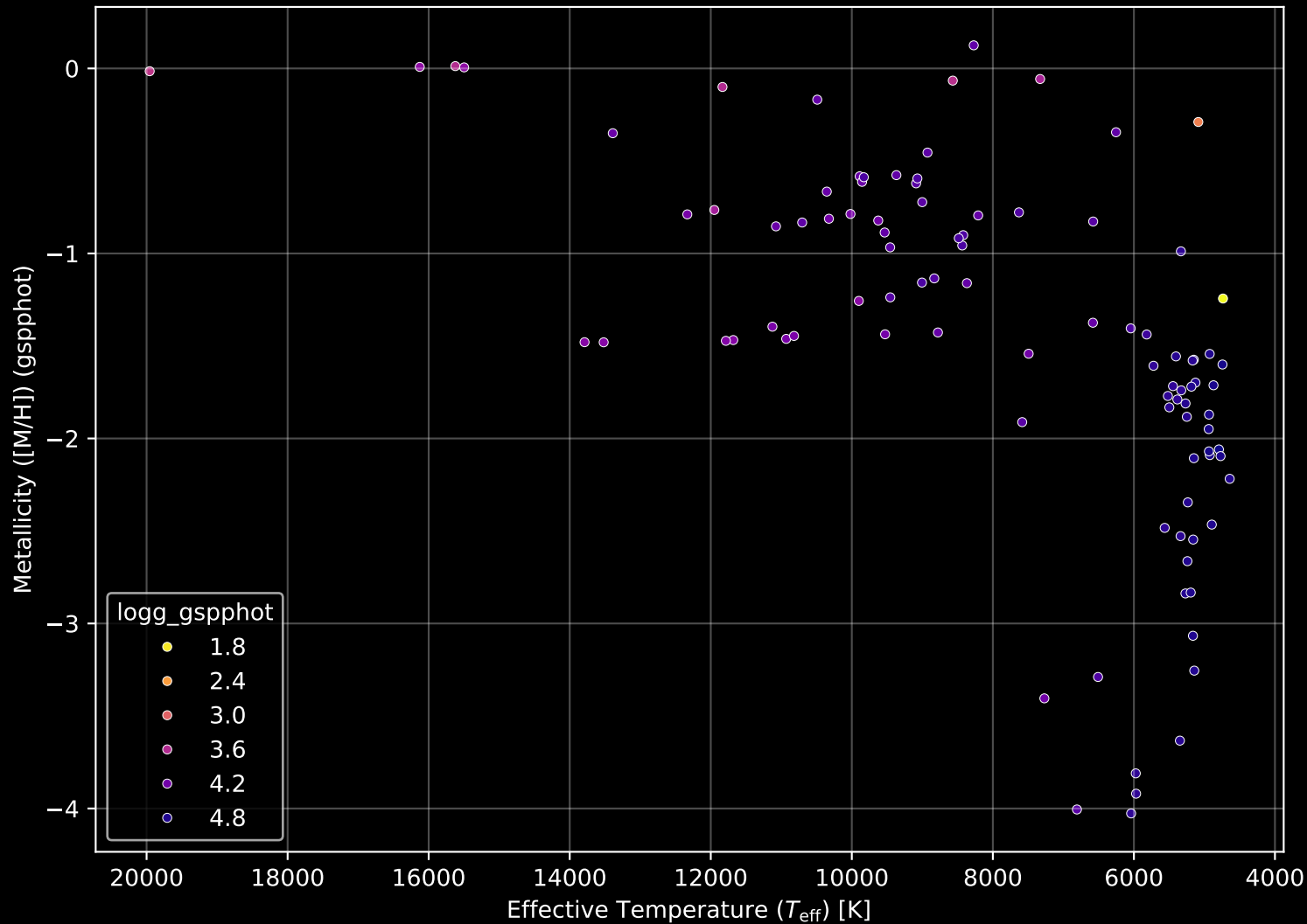
Gaia Cluster: [NGC_2401] Stellar Population Parameters (n= 98)
