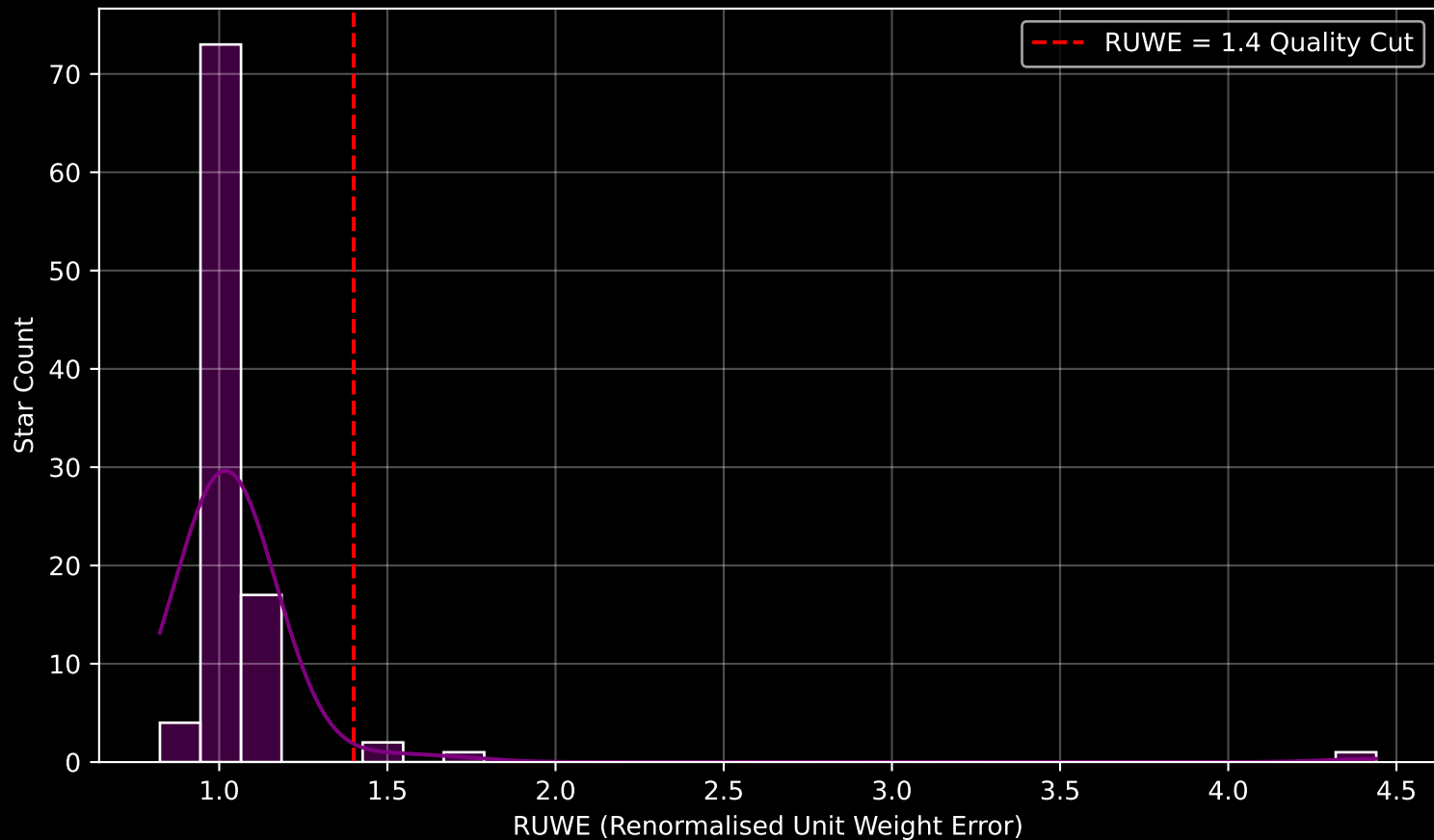
Gaia Cluster: [NGC_2401] RUWE Distribution (n= 98)
