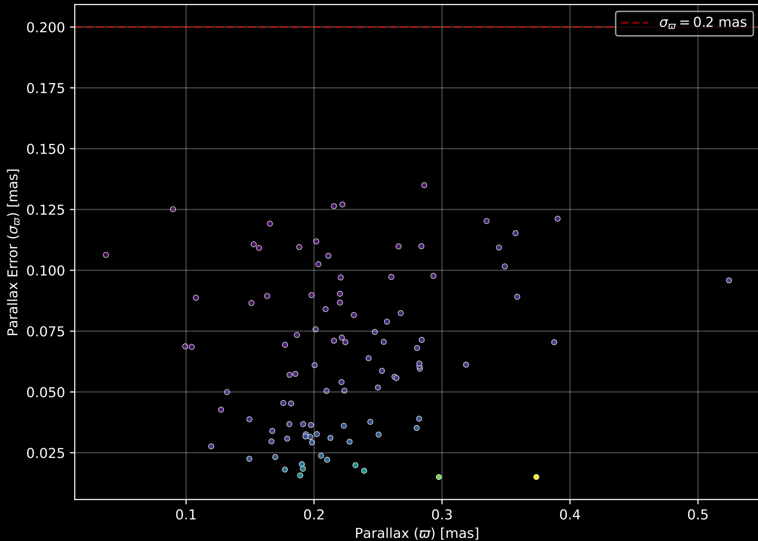
Gaia Cluster: [NGC_2401] Parallax Quality (n= 98)
