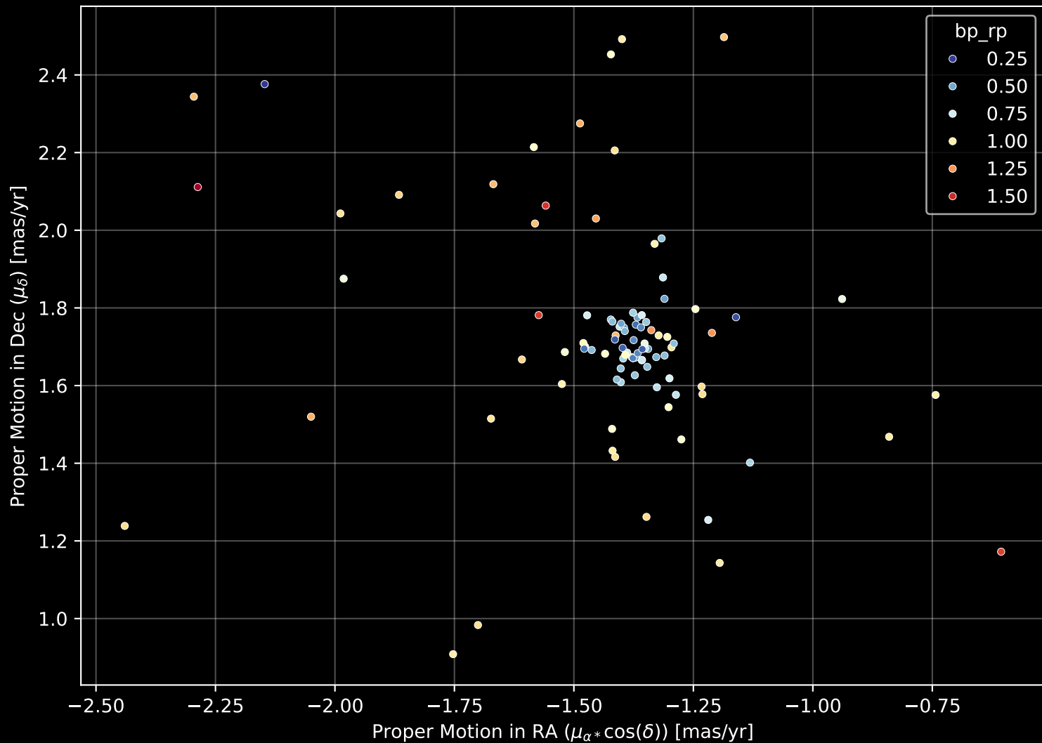
Gaia Cluster: [NGC_2401] Proper Motion Diagram (n= 98)
