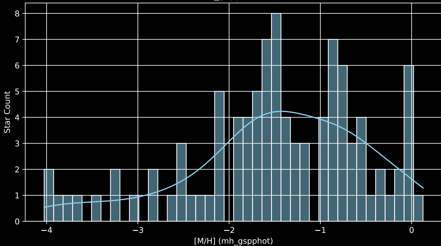
Gaia Cluster: [NGC_2401 [M/H] (mh_gspphot) (n= 98)
