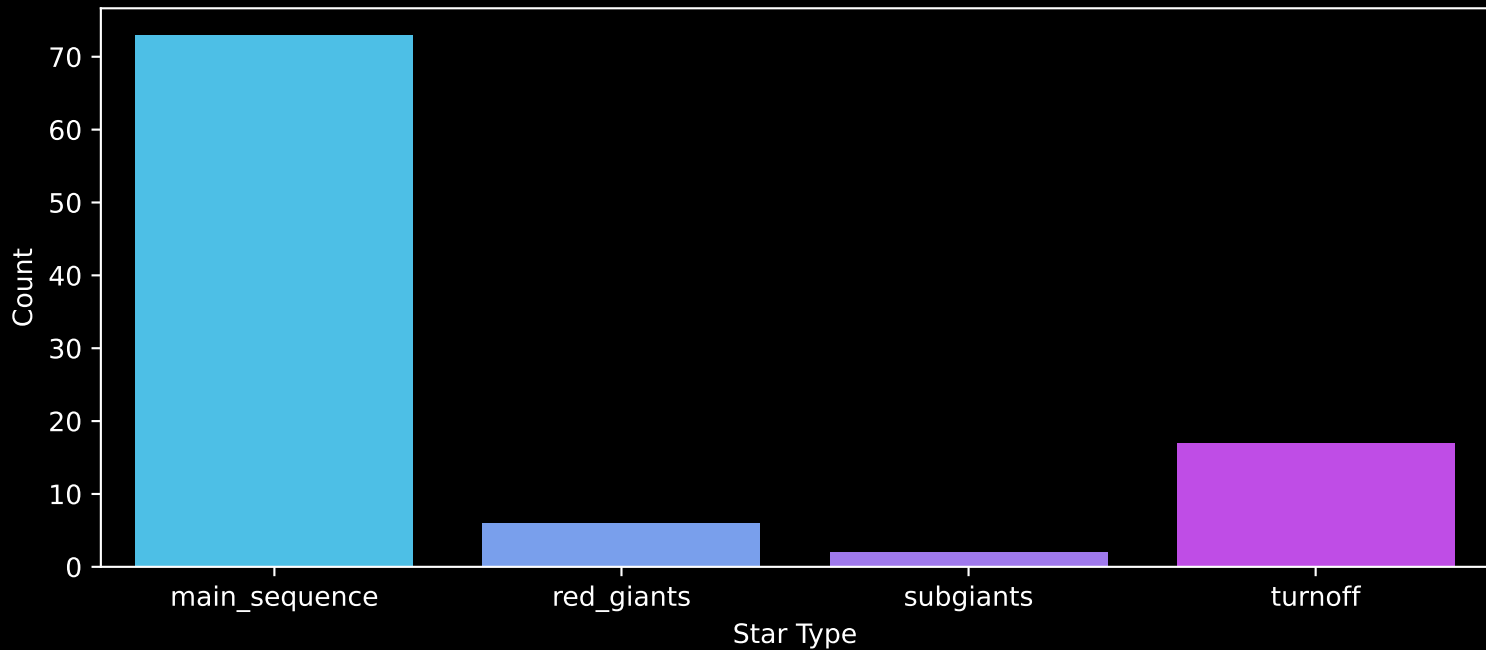
Gaia Cluster: [NGC_2401] Count plot of Star Type
