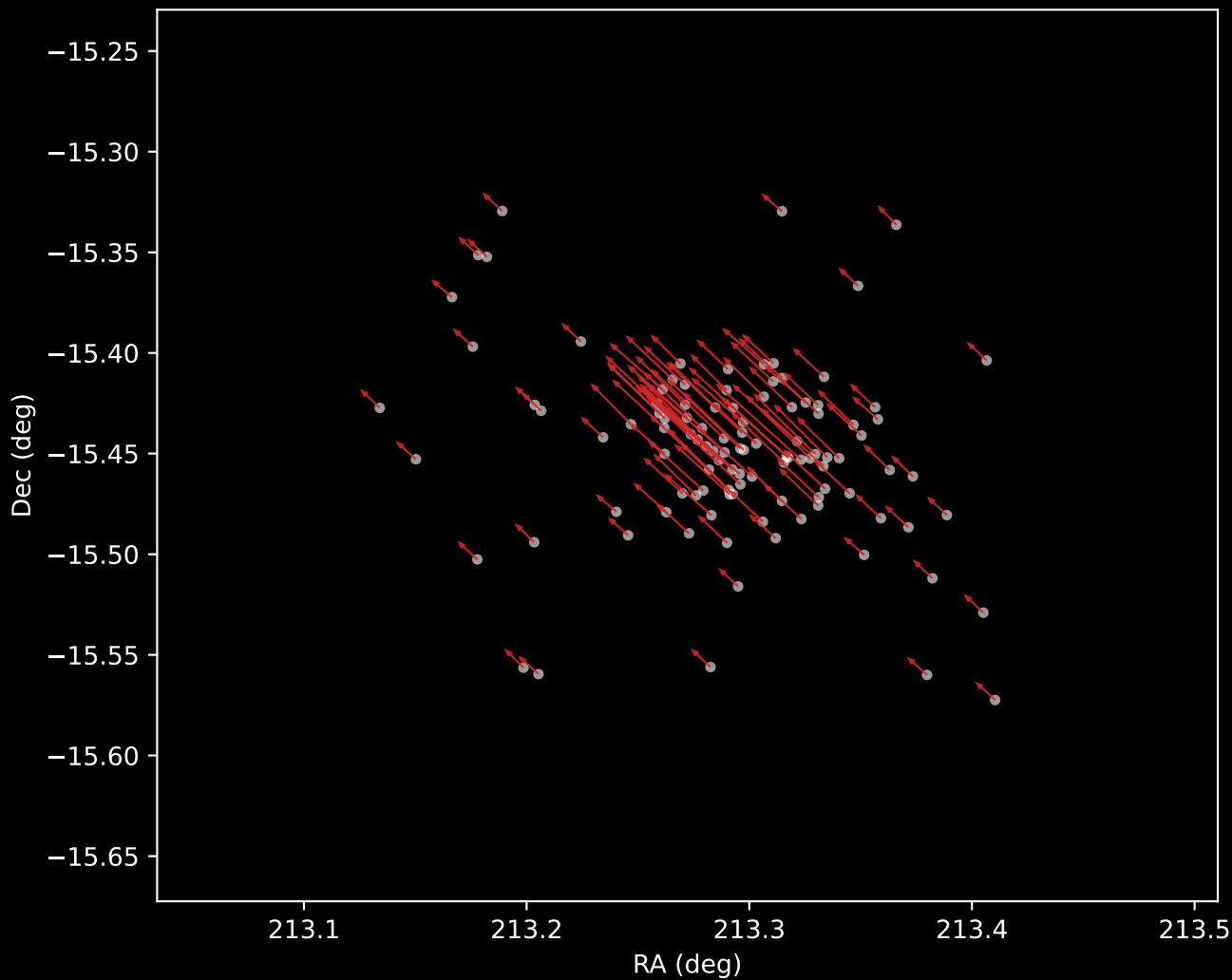
Gaia DR3 Cluster 6 Proper Motion Vectors (n=109)
