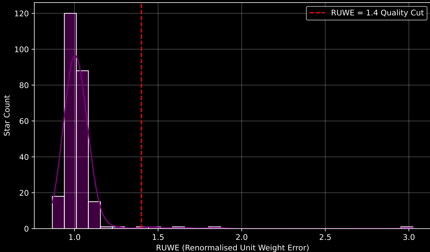
Gaia Cluster: [NGC_2414] RUWE Distribution (n= 248)
