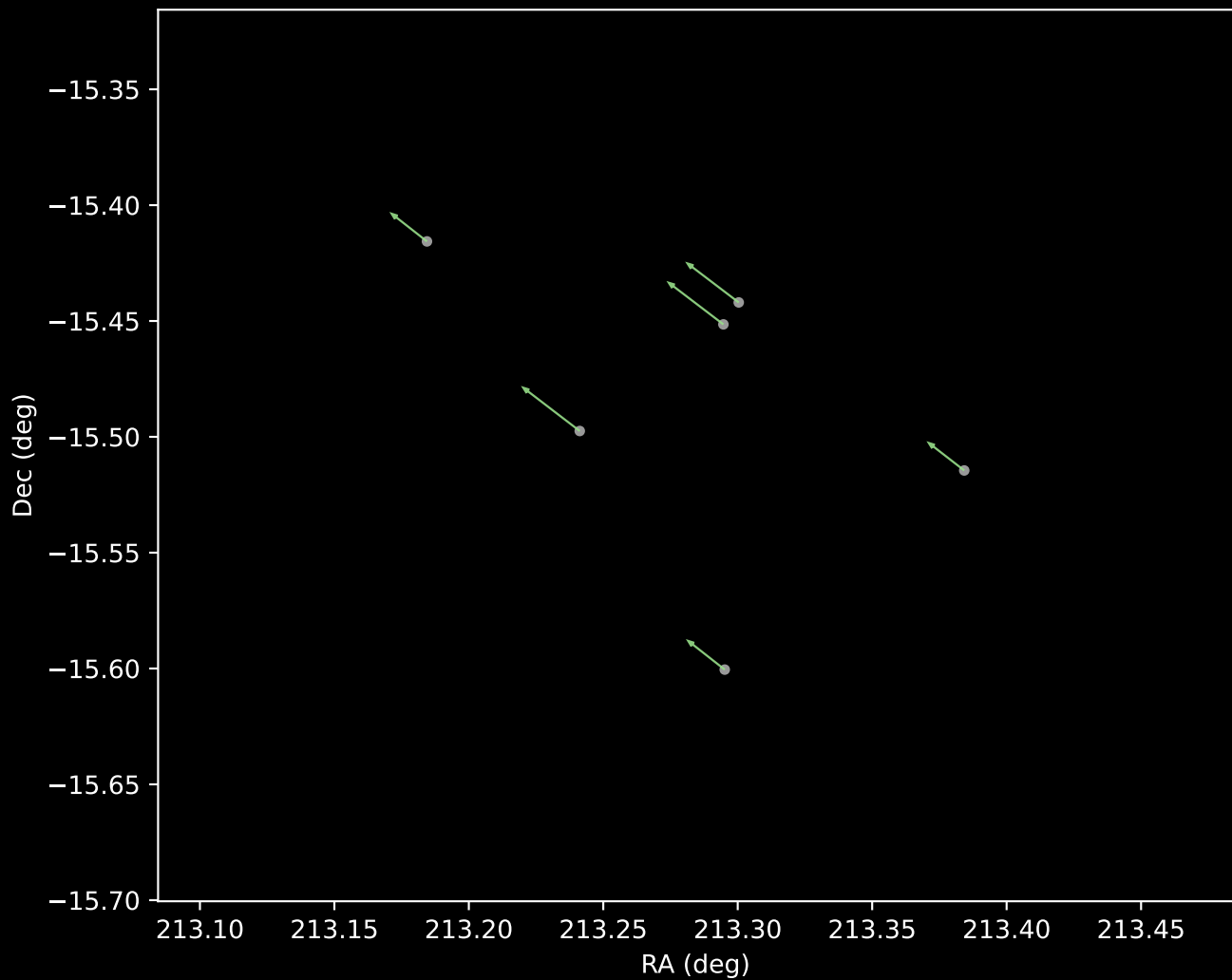
Gaia DR3 Cluster 5 Proper Motion Vectors (n=6)
